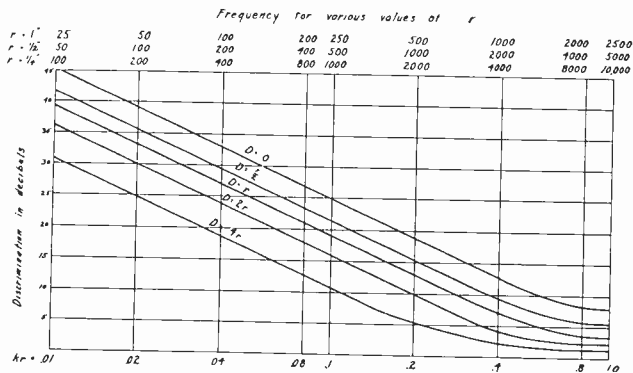
Fig. 6—Theoretical discrimination against random sounds for various spacings D of openings to front and back of diaphragm, and for various distances r from point source.
