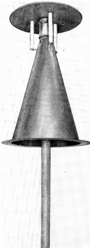
Fig. 5—Discone antenna for cutoff frequency of 90 megacycles.
