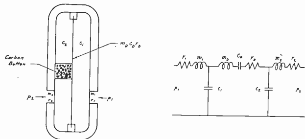
Fig. 9—Diagram of differential microphone and its equivalent acoustic-mechanical circuit.
