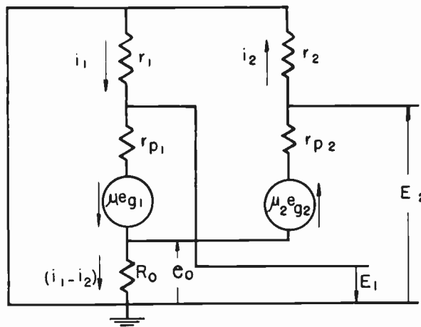
Fig. 4—Equivalent linear-tube-parameter circuit of common-cathode-impedance self-balancing inverter.
