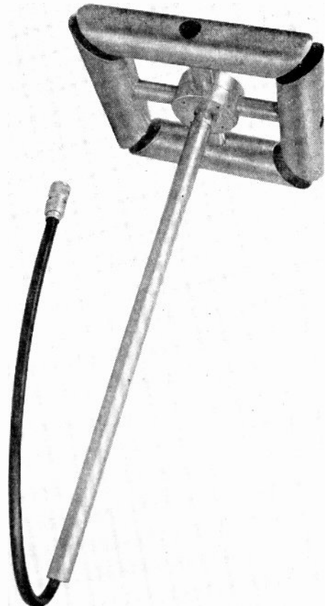
Fig. 6—Coaxially fed loop antenna for 550 megacycles.
