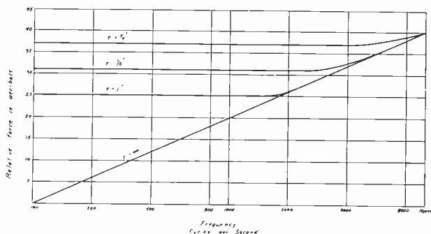
Fig. 7—Force available for actuating diaphragm.
