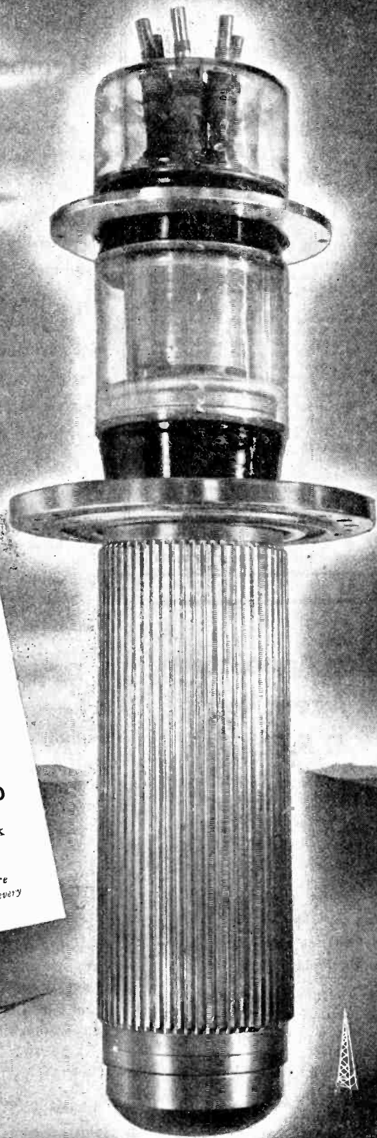
Federal 134 Transmitting Tube, 200 KW oscillator and amplifier; length, 34- \frac{1}{8} ".
