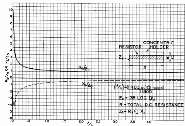
Fig. 10—Impedance of short-circuited transmission line. R/Z_0 = 10.0 .
