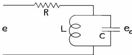
Fig. 6—Resistance-inductance-capacitance circuit.
