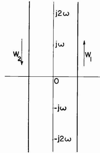
Fig. 1—One path of integration employed in the inverse transform.
