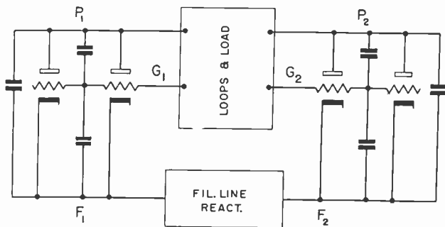
Fig. 3—Equivalent circuit of transmitting tube.
