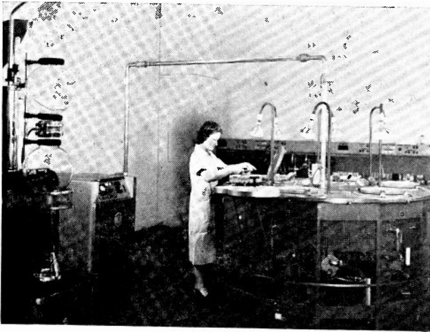
Fig. 10—A circular table with six drying chambers. This equipment dries 2000 bottles per hour. The infrared lamps prevent condensation on the cold lids of the vacuum chambers.
