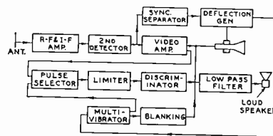
Fig. 14—Pulsed frequency-modulation receiver.
