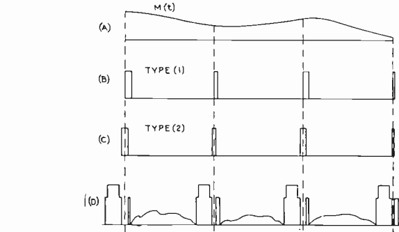
Fig. 4—Width-modulated duplex wave forms.
