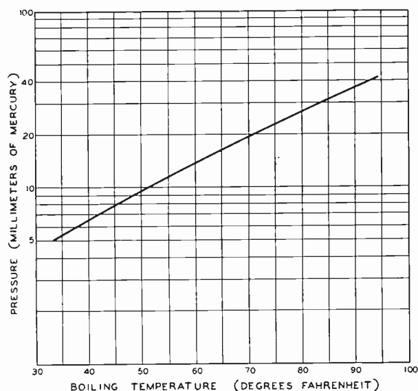
Fig. 2—Boiling temperature versus pressure.
