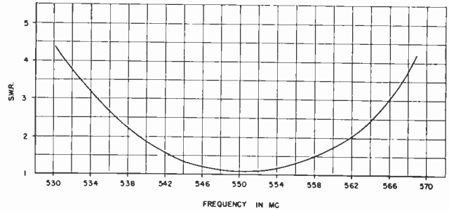
Fig. 10—Characteristic curve of frequency versus standing-wave ratio for a square loop. Four elements of 2-inch cross section; loop diameter, 8\frac{1}{2} inches.
