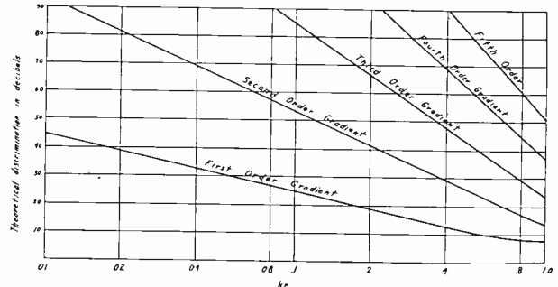
Fig. 10—Theoretical discrimination of pressure gradient microphones of various orders.
