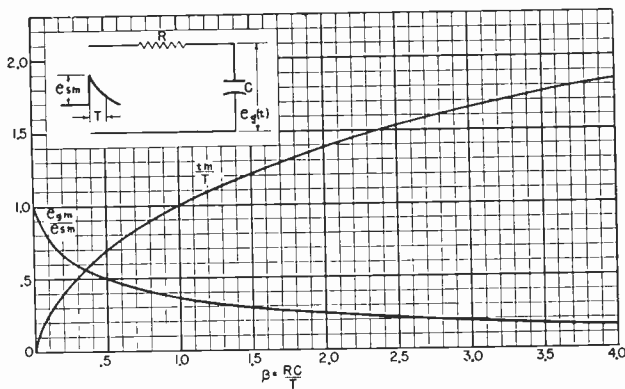
Fig. 12—The ratios ( t_m/T ) and ( e_{gm}/e_{sm} ) as functions of \beta = RC/T for an exponential pulse.
