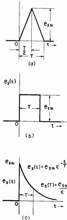
Fig. 4—Grid-signal pulses.
