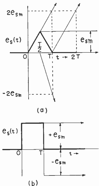
Fig. 5—Components of the triangular and square pulses.
