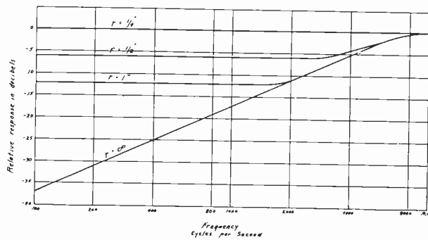
Fig. 8—Theoretical response at various distances r from source for microphones having a flat response 1/4 inch from source.
