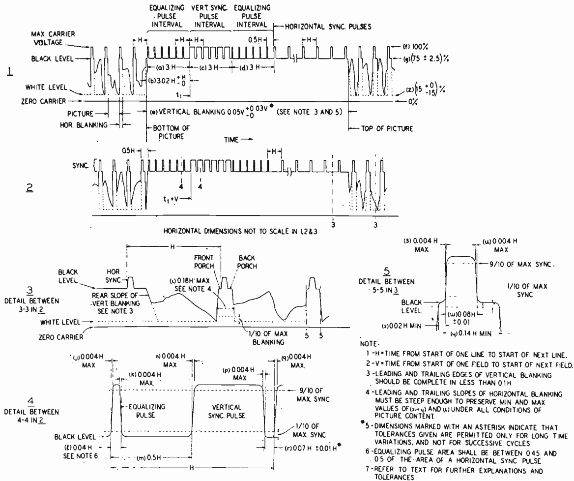
Fig. 1—Television synchronizing wave form.
