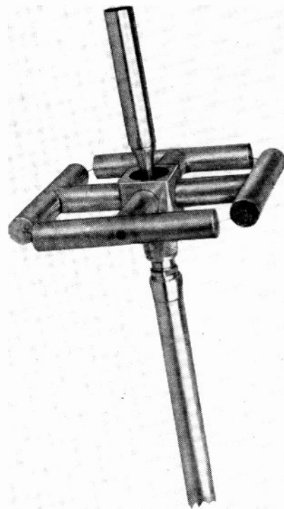
Fig. 14—Type III antenna for an operating frequency of 1200 megacycles.
