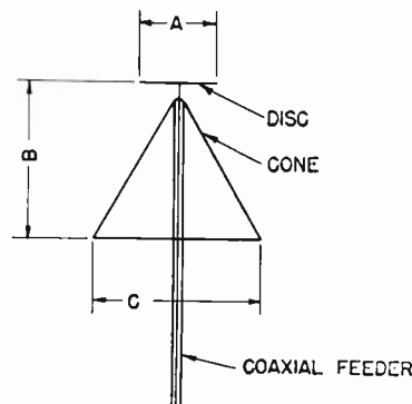
Fig. 1—Schematic diagram of the Discone antenna.
