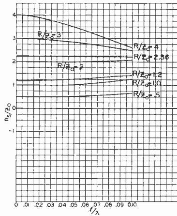
Fig. 11—Resistance of short-circuited transmission line. All slopes are zero at l/\lambda=0 . For R/Z_0 = \sqrt{3} , curvature is zero at l/\lambda=0 .
