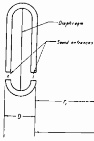
Fig. 3—Relative source and microphone locations used in calculation of discrimination of microphone with distance D between sound entrances.
