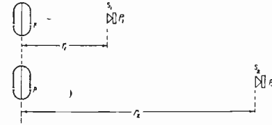
Fig. 2—Relative source and microphone locations used in calculating discriminations.
