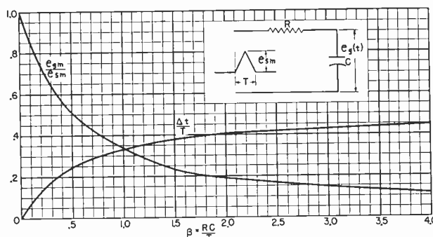
Fig. 7—The ratios ( e_{gm}/e_{sm} ) and ( \Delta t/T ) as functions of \beta = RC/T for a triangular pulse.
