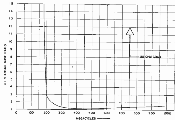
Fig. 3—Mismatch versus frequency of Discone antenna for a cutoff of 200 megacycles.
