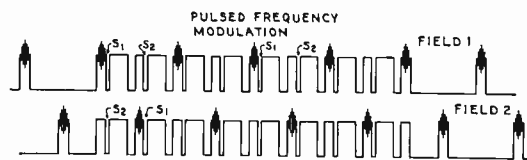
Fig. 12—Modification of television wave form for pulsed frequency modulation on line-synchronizing pulses.
