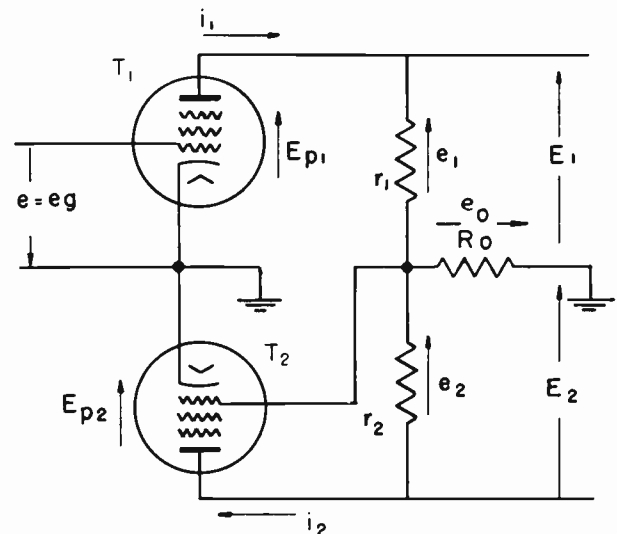
Fig. 1—Equivalent signal-voltage circuit of common-plate-impedance self-balancing inverter.
