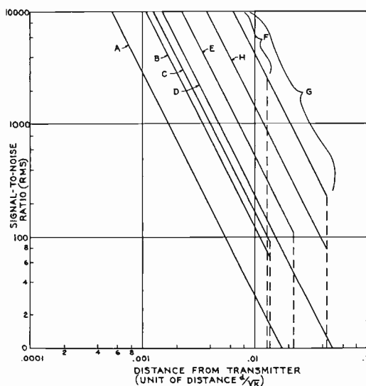
Fig. 15—Signal-to-noise ratios for sound transmission. A = amplitude-modulated pulses B = width-modulated pulses (symmetrical) C = width-modulated pulses (dissymmetrical) D = standard amplitude modulation E = pulsed frequency modulation ( f_d = 150 kilocycles) F = pulsed frequency modulation ( f_d = 1200 kilocycles) G = standard frequency modulation ( f_d = 150 kilocycles) H = standard frequency modulation ( f_d = 50 kilocycles; bandwidth = 150 kilocycles).
