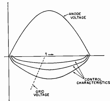
Fig. 2—Grid-control curves of Fig. 1 for a sinusoidal anode voltage.
