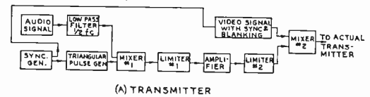
(A) TRANSMITTER
