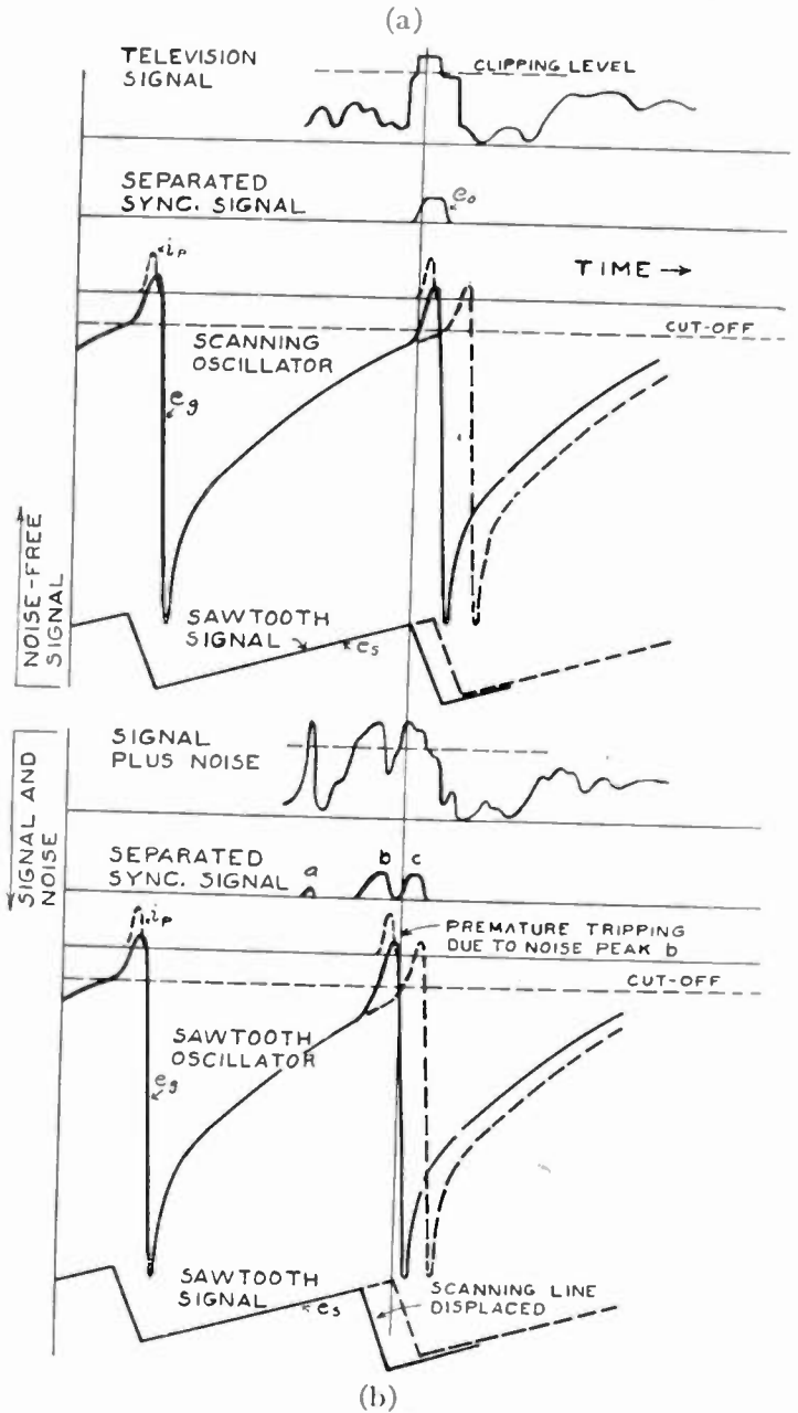
(a)—Operation of scanning oscillator. (b)—Operation of scanning oscillator when noise is present.
