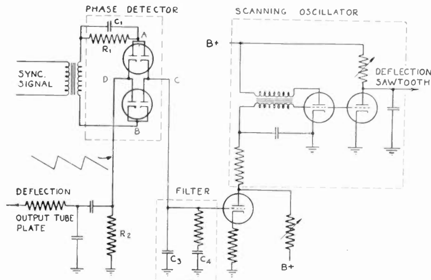
Fig. 10—Four-diode automatic frequency- and phase-controlled circuit.
