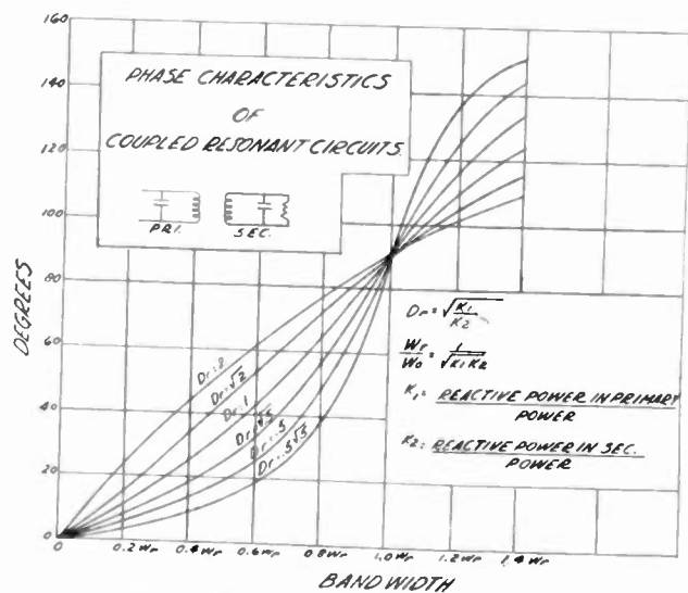
Fig. 3—Phase characteristics of coupled resonant circuits.
