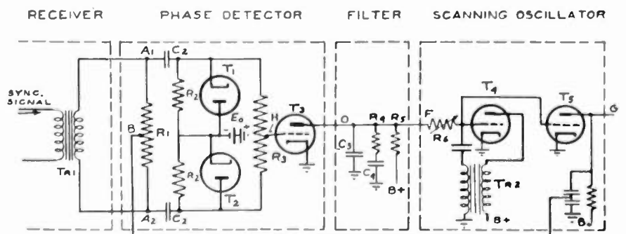
Fig. 5—Automatic frequency- and phase-controlled circuit.
