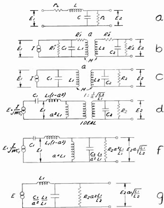
Fig. 1—Equivalent circuits for coupled resonant circuits.
