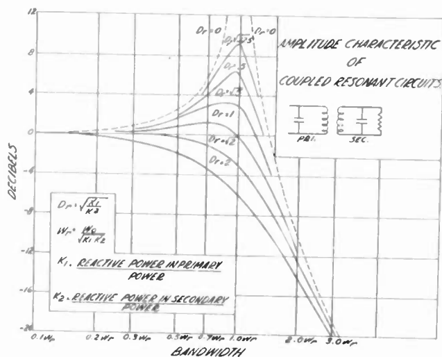
Fig. 2—Coupled resonant circuits for transmitters.
