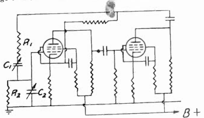
Fig. 1.—Typical circuit of a resistance-capacitance-tuned oscillator.
