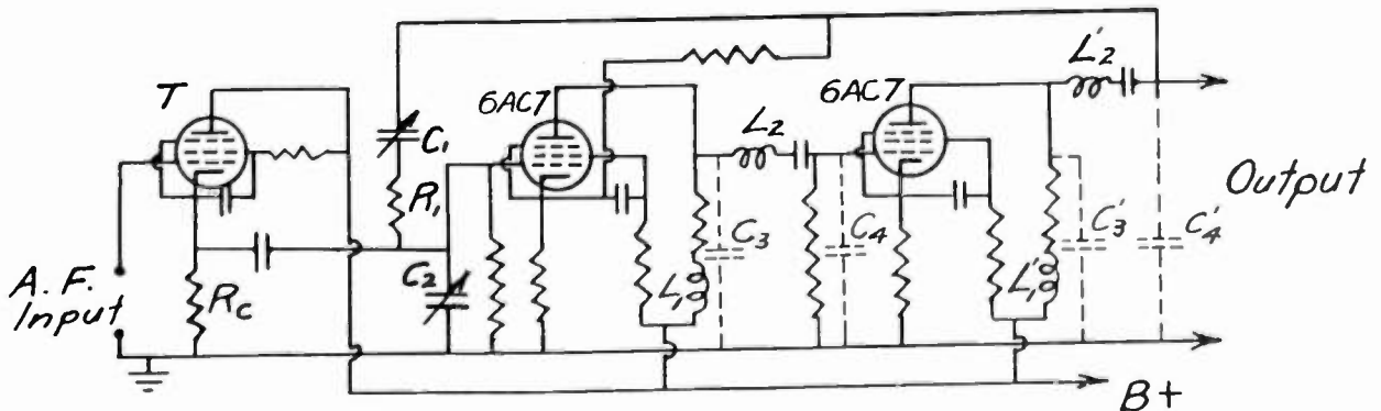
Fig. 2.—Circuit diagram of a frequency-modulated resistance-capacitance oscillator.
