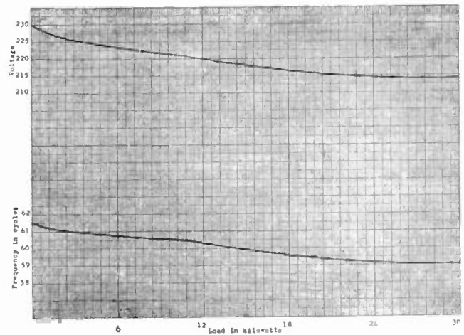
Fig. 3—Voltage and frequency change as plant load is increased from no load to full load.
