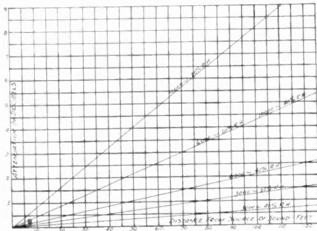
Fig. 6—Attenuation of sound due to absorption in air at 70 degrees Fahrenheit and relative humidities indicated on curves.
