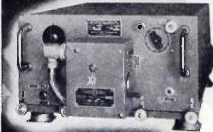
The "BENDIX" RTA-1 Communication Unit, which combines 10 crystal-controlled receiver and transmitter channels with integral power supply into one compact, light-weight unit.
