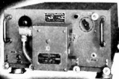
The "BENDIX" RTA-1 Communication Unit, which combines 10 crystal-controlled receiver and transmitter channels with integral power supply into one compact, light-weight unit.
