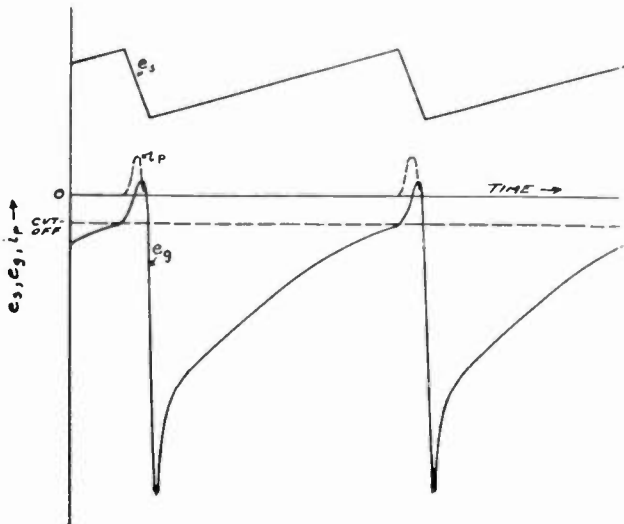
Fig. 2—Operation of the scanning oscillator.
