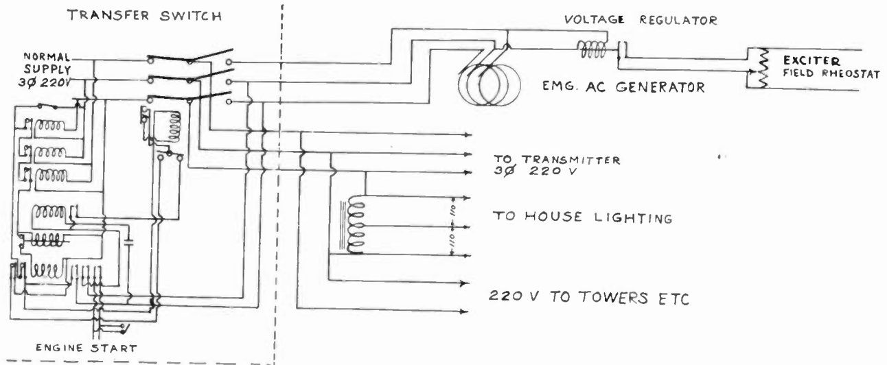
Fig. 1—Transfer switch and connections to generator and building wiring.
