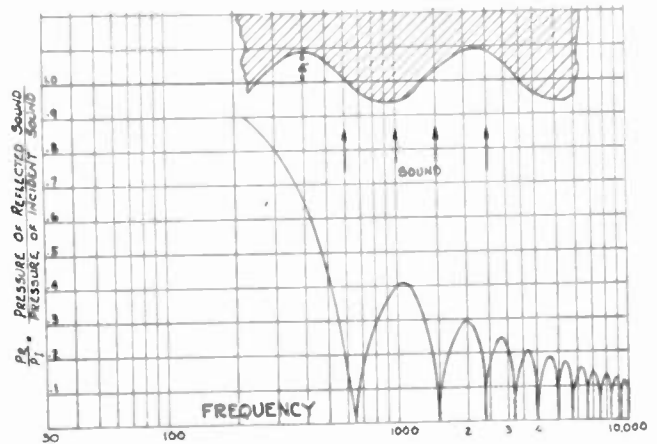
Fig. 9—Sound-reflection characteristic from a rigid non-porous wall of sinusoidal contour.
