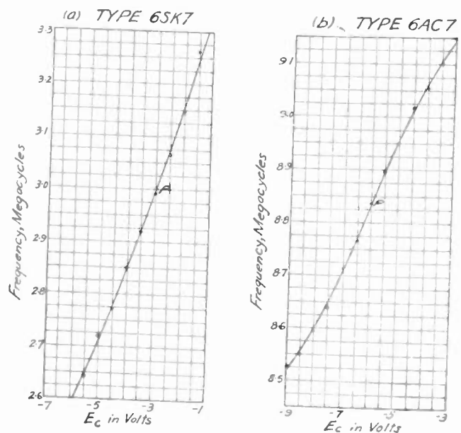
Fig. 3.—Oscillator frequency as a function of grid voltage of the resistance tube. Note that E_c is the battery bias only.
