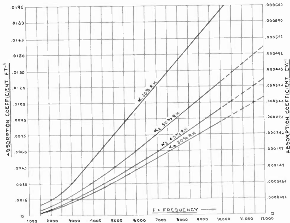
Fig. 2—Absorption characteristic of sound in air for various degrees of relative humidity.
