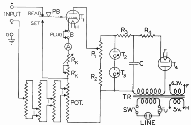
Fig. 3—The practical vacuum-tube voltmeter circuit.
