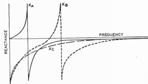
Fig. 8—Reactance curves for Pierce-type oscillator.
