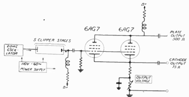
Fig. 11—Block diagram of square-wave generator.
