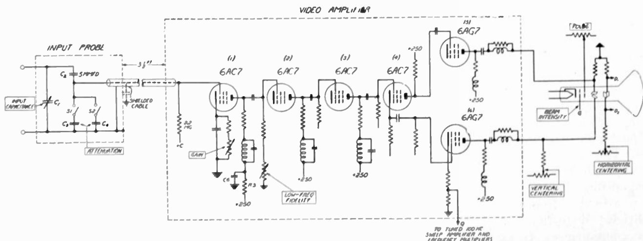
Fig. 5—Simplified circuit diagram of probe, video amplifier, and cathode-ray tube in the square-wave oscilloscope.
