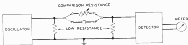
Fig. 2—Resistance method for measuring Q of crystal.
