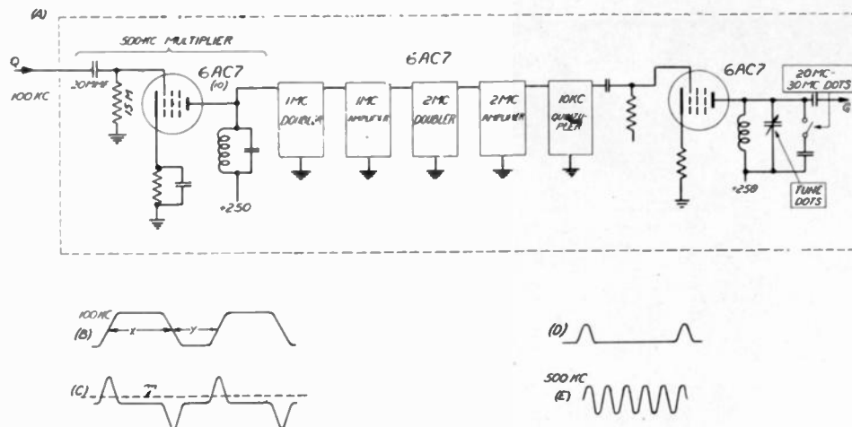
Fig. 8—(A) Dotter circuit of square-wave oscillograph. (B) Square-wave signal at point Q . (C) Differentiated signal at grid of 500-kilocycle multiplier tube. (D) Plate current of multiplier tube. (E) Output voltage of 500-kilocycle multiplier.
