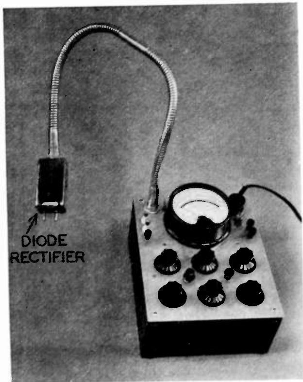
Fig. 4—Experimental model of the vacuum-tube voltmeter.
