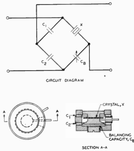
Fig. 16—Crystal bridge.
