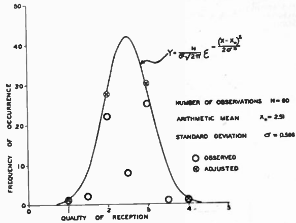
Fig. 3—The data of Fig. 2 expressed in the form of a frequency-distribution curve.
