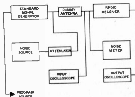
Fig. 1—Block diagram of the apparatus used in the tests.
