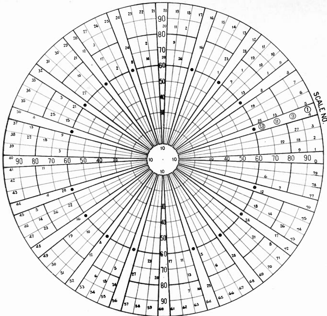
Fig. 12—Chart for square-wave synthesis.
