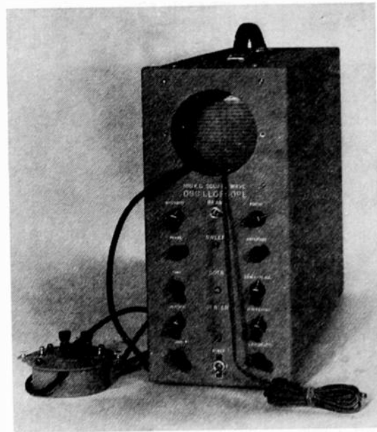
Fig. 4—Square-wave oscilloscope and probe.
