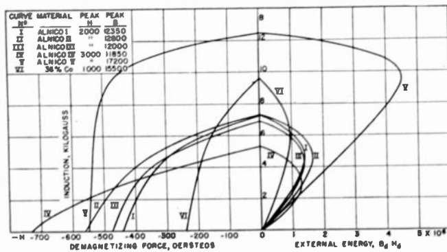
Fig. 5—Demagnetization and energy curves of alnico type of permanent magnets.
