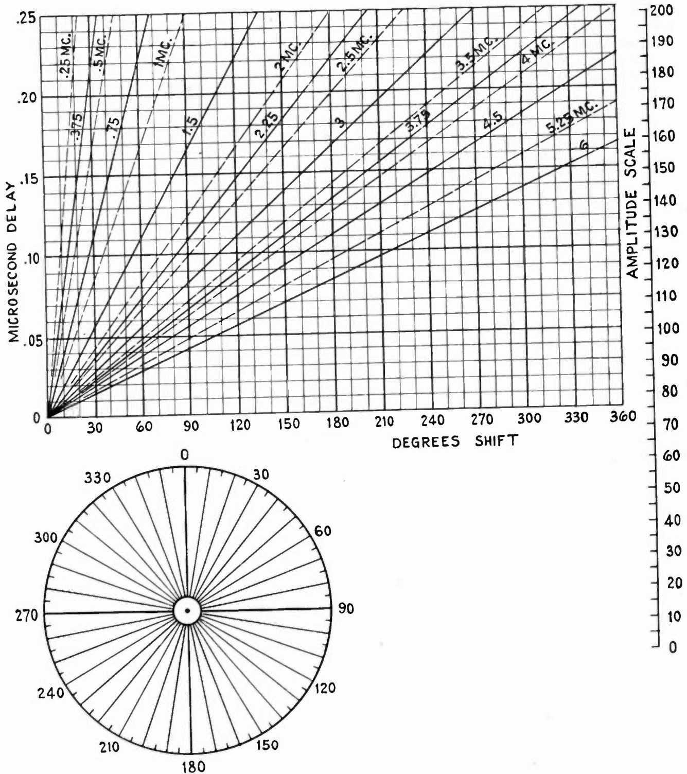
Fig. 5—Chart for square-wave analysis.
