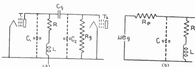
(a) Compensated resistance-capacitance amplifier. (b) Equivalent circuit for high frequencies.
