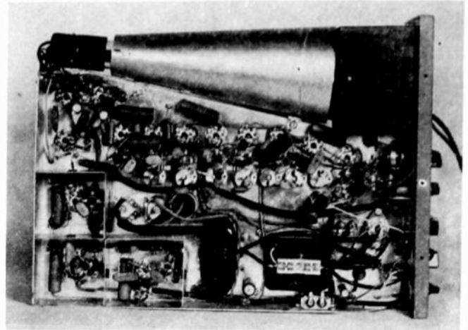
Fig. 10—Chassis of the square-wave oscillograph.
