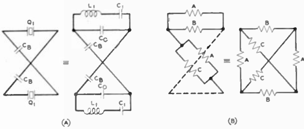
Fig. 11—Use of crystal in bridge circuit.
