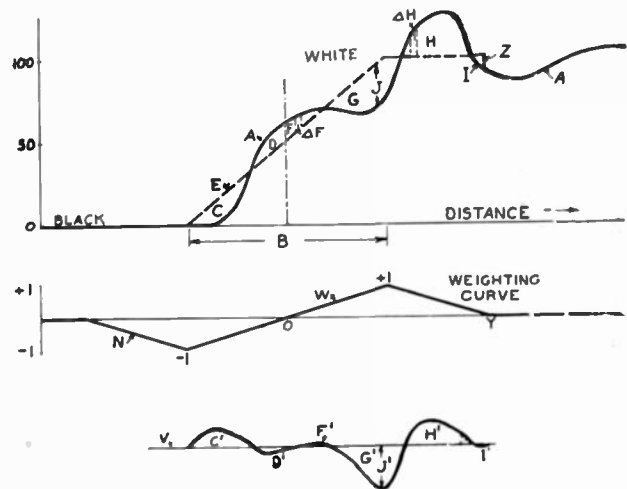
Fig. 19—Linear transition E is equivalent to A. By Condition 2, the algebraic sum of areas C, D, F, G, H, and I is zero. By condition 1, the sum of weighted areas C, D, F, etc., shown at C', D', F', etc., is zero
