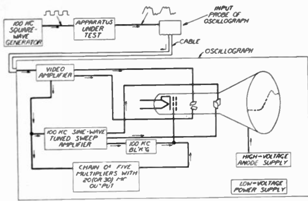
Fig. 2—Block diagram of a typical test arrangement showing the square-wave generator, apparatus under test, and the square-wave oscilloscope. Internal components of the oscilloscope also appear in block form.
