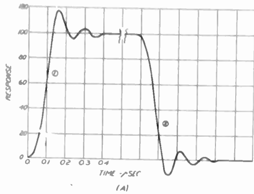
(A) Square-wave response of generator and oscillograph only.
