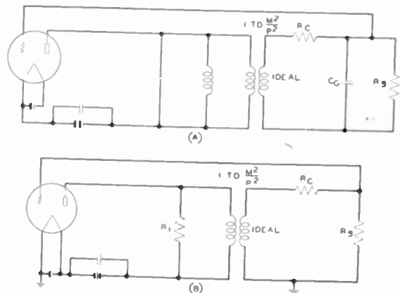
Fig. 10—Impedances at crystal resonance for phase-reversing oscillator.
