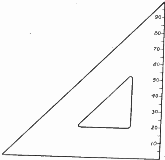
Fig. 15—Calibrated triangle 8 for reading contributions of harmonics from synthesis charts.
