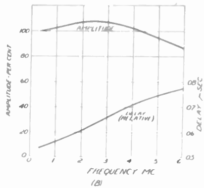
(B) Combined amplitude and delay characteristics of generator and oscillograph according to chart analysis of rising trace in (A).
