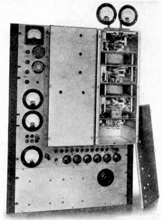
Fig. 21—Photograph of crystal oscillator and amplifier.
