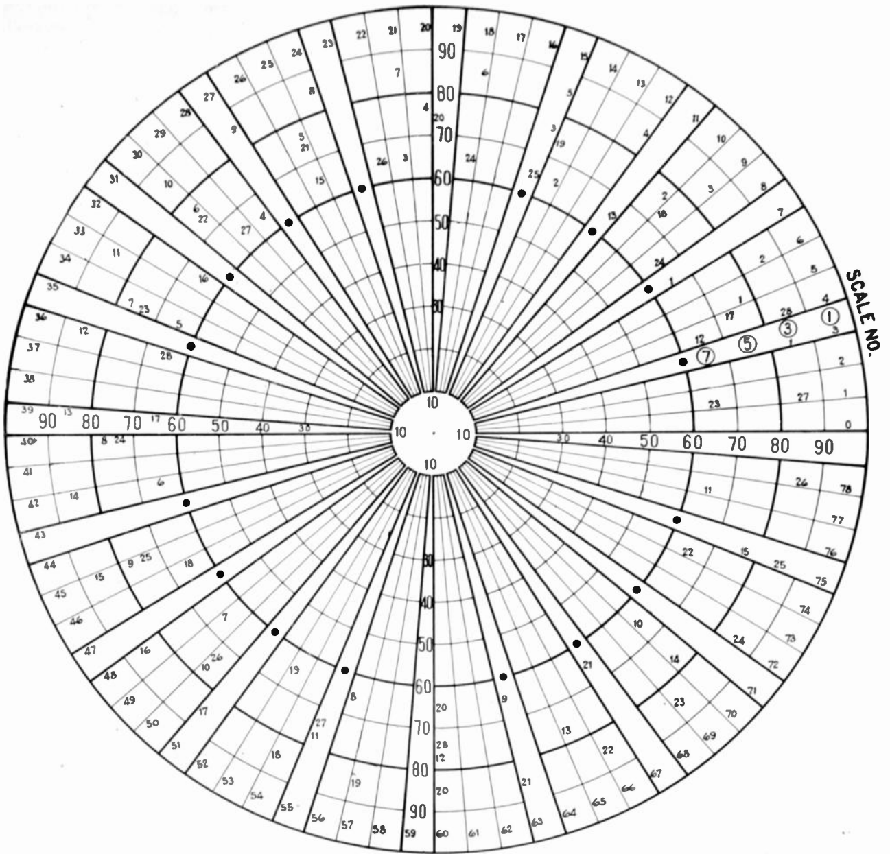
Fig. 11—Chart for square-wave synthesis.
