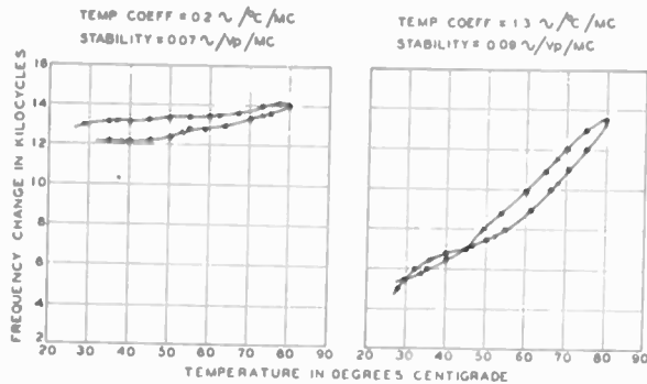
Fig. 19—Frequency change as a function of temperature.
