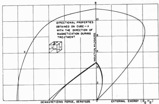
Fig. 6—Directional properties of alnico V.
