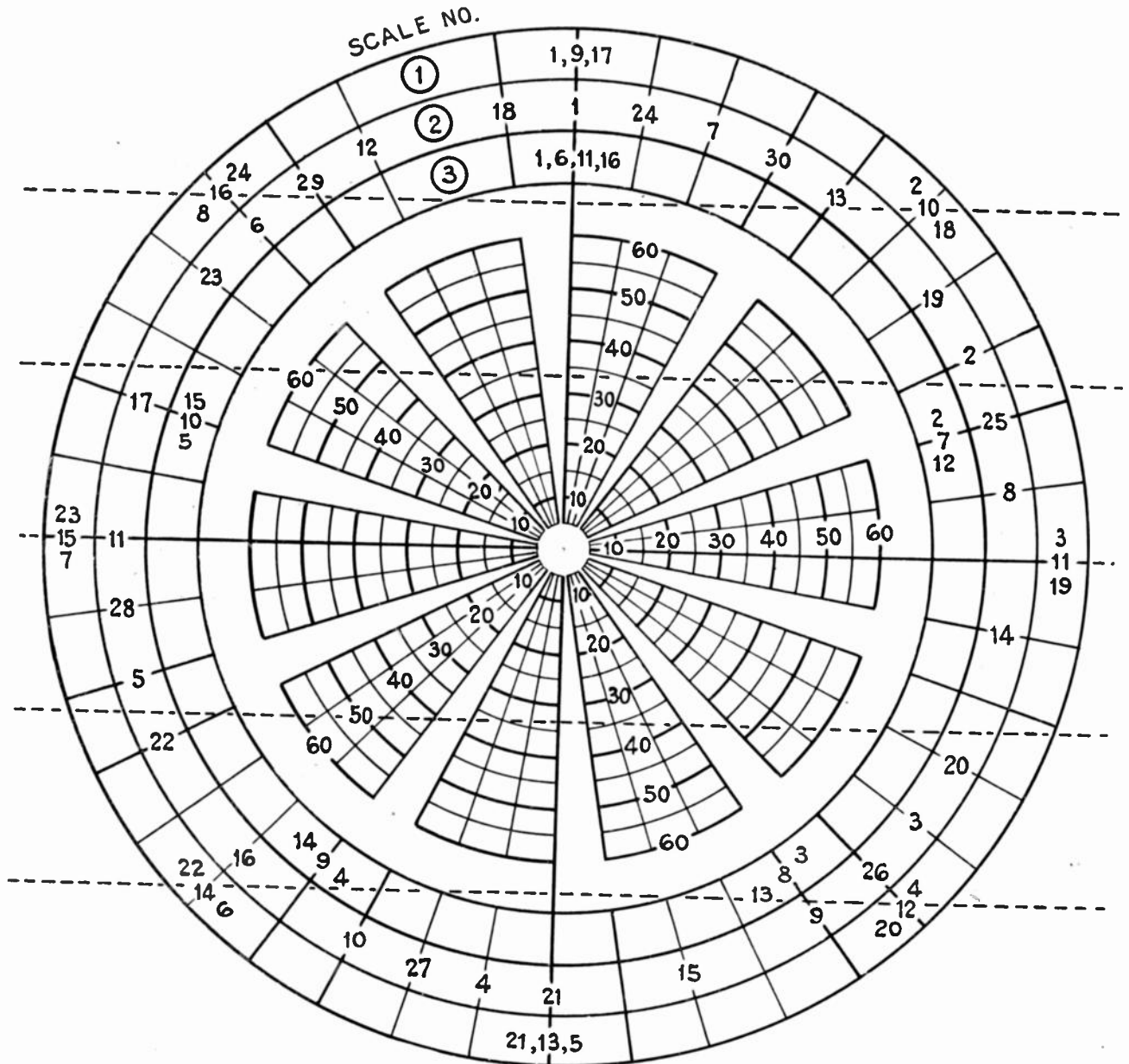
Fig. 4—Chart for square-wave analysis.
