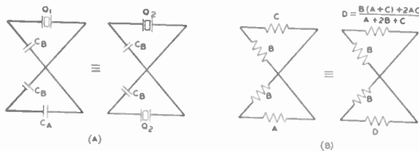
Fig. 13—Equivalence between balanced and unbalanced lattice networks.
