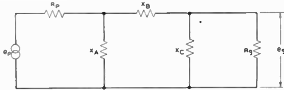
Fig. 7—Equivalent circuit of Pierce-type oscillator.
