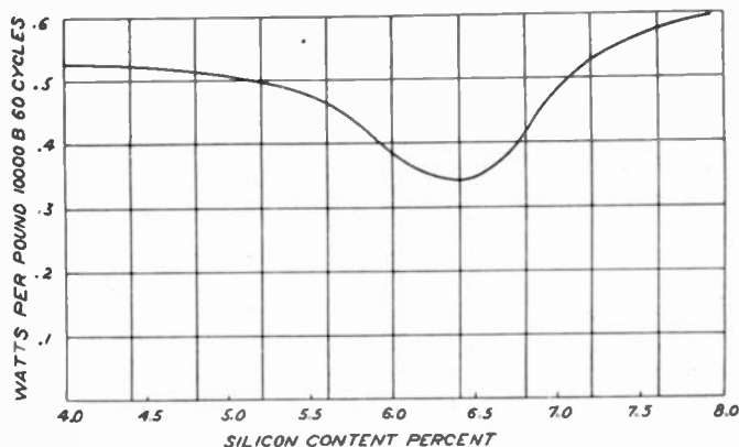
Fig. 1—Effect of silicon content on watt loss.
