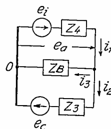
Fig. 2—Simplified diagram for calculating the input voltage of the auxiliary amplifier. The impedance Z_3 in this figure is equal to (Z_3+Z') in Fig. 1.
