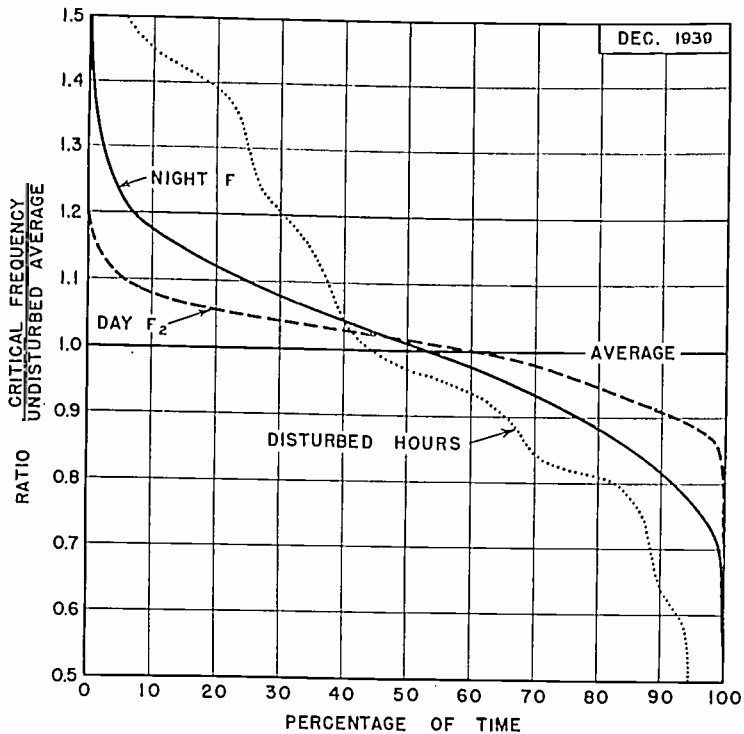
Fig. 3—Distribution of F- and F 2 -layer ordinary-wave critical frequencies (and approximately of maximum usable frequencies) about monthly average. Abscissas show percentages of time for which the ratio of the critical frequency to the undisturbed average exceeded the values given by the ordinates. The solid-line graph is for 403 undisturbed night hours of observation; the dashed graph is for 208 undisturbed day hours of observation; the dotted graph is for 69 disturbed hours of observation: listed in Table I.
