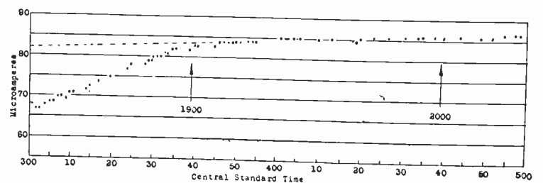
Fig. 3—Microamperes versus C.S.T. on May 11, 1939, for declination -20 degrees. Hours right ascension indicated by arrows. P marks the plane of the Milky Way. Galactic longitude for this declination is 337.2 degrees. The at first rapid, and later gradual, increase of reading is due to the warming up of the equipment.
