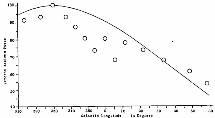
Fig. 4—Intensity versus Galactic longitude l . Circles indicate measured points. Solid line computed from equation (7).
