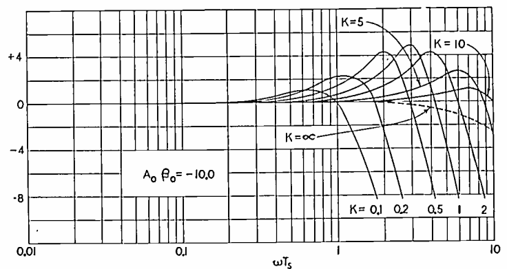
Fig. 11—High-frequency response, feedback factor -10.0 .
