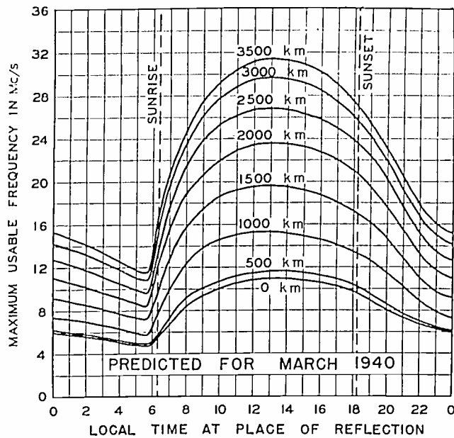
Fig. 4—Predicted maximum usable frequencies for dependable radio transmission via the regular layers, average for undisturbed days, for March, 1940.
