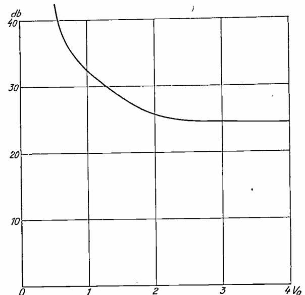
Fig. 10—Reduction of the "klirr-factor" with the arrangement shown in Fig. 4.
