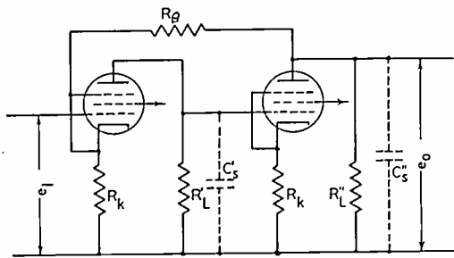
Fig. 8—Schematic circuit of two-stage feedback amplifier valid for the high-frequency region.
