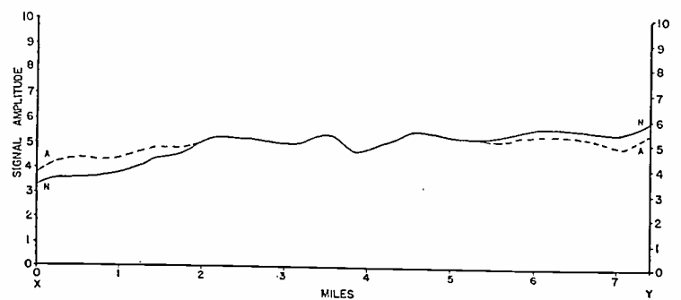
Fig. 4—Sector X-Y of A and N field-strength contours 52 miles from the 63,000-kilocycle transmitter. (Actual.)
