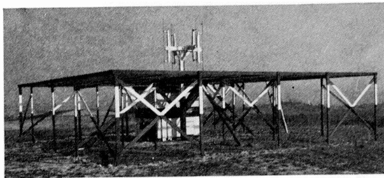
Fig. 7—Final design of the ultra-high-frequency radio-range station.
