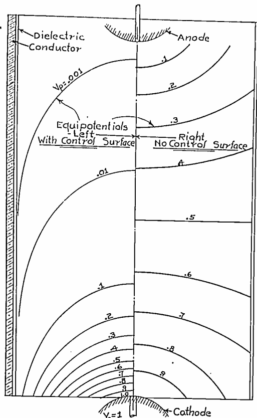
Fig. 6—Equipotentials in cylinder-plane section on axis; right of center line, no control surface. Left of center line, with control surface.
