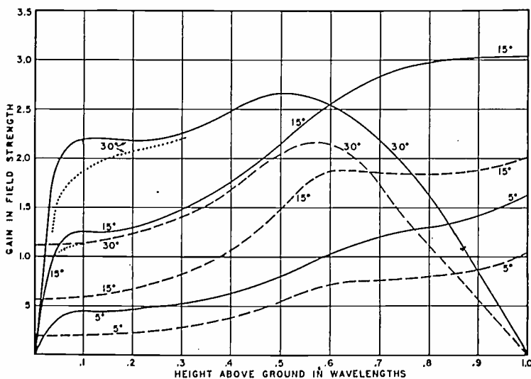
Fig. 6—The effect of height above ground on the gain of two horizontal out-of-phase elements with a spacing of one-eighth wavelength is shown by the solid curves. The gain of a single horizontal half-wave antenna is shown by the dashed curves. The gain is given for vertical angles of 5, 15, and 30 degrees and is referred to a half-wave antenna in free space. Perfectly conducting ground is assumed.
