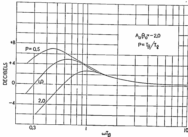
Fig. 2—Low-frequency response, feedback factor -2.0.
