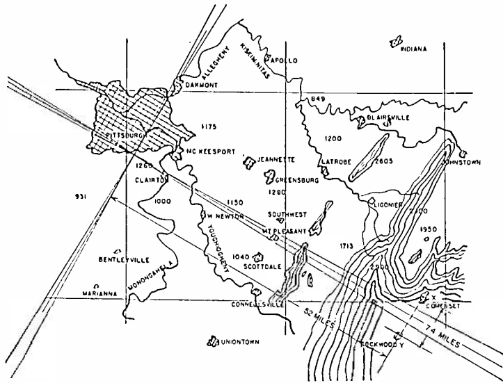
Fig. 1—Course orientation of both Pittsburgh range stations. (254 and 63,000 kilocycles.)
