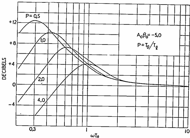
Fig. 3—Low-frequency response, feedback factor -5.0.
