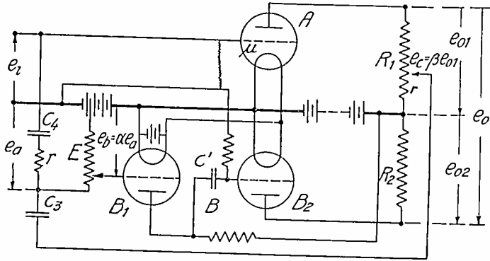
Fig. 4—Arrangement for distortion-free voltage amplification, A = main amplifier, B = auxiliary amplifier.
