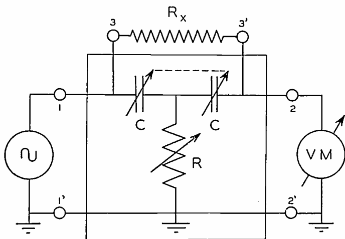
Fig. 1—Bridged-T resistance-measuring network.
