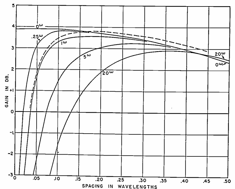
Fig. 5—Gain of two out-of-phase elements in free space as a function of spacing for various loss resistances.
