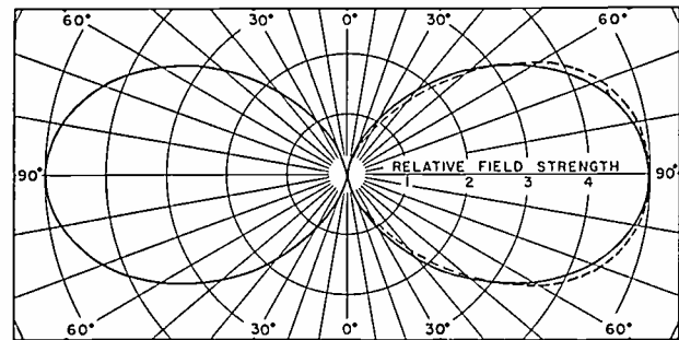
Fig. 2—Horizontal radiation pattern of a two-element array of the type shown in Fig. 1A. The elements of the antenna are horizontal and the maximum radiation is broadside to the array. The spacing S is one-eighth wavelength. The solid curve is computed and the dashed curve measured.
