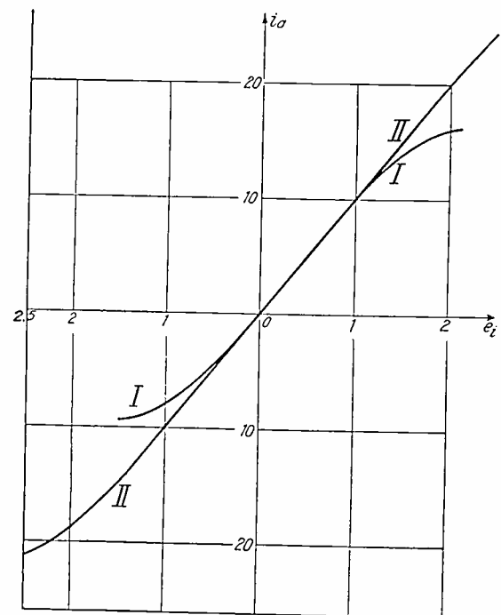
Fig. 8—Curve I shows the main-amplifier characteristic: 10e_i + e_i^2 - e_i^3 and curve II the resulting characteristic: 10e_i + (e_i^2 - e_i^3)^3/10^3 .
