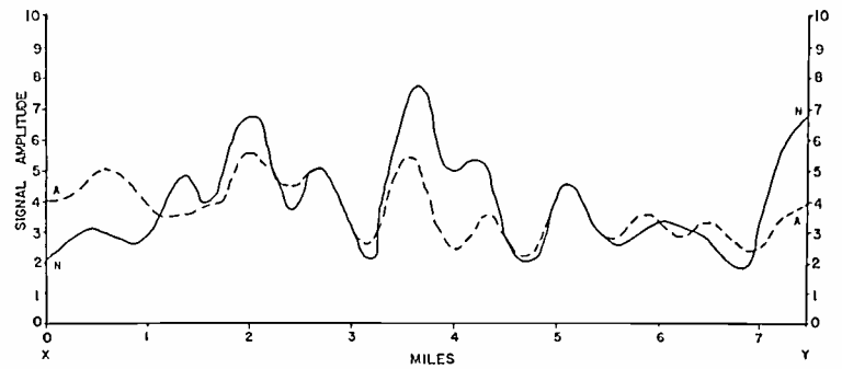
Fig. 3—Sector X-Y of A and N field-strength contours 52 miles from the 254-kilocycle transmitter. (Actual.)
