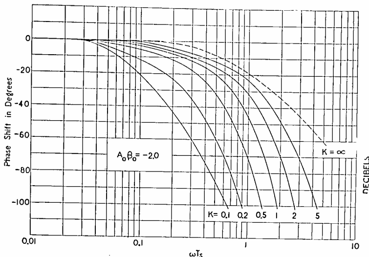
Fig. 12—High-frequency phase shift, feedback factor -2.0 .
