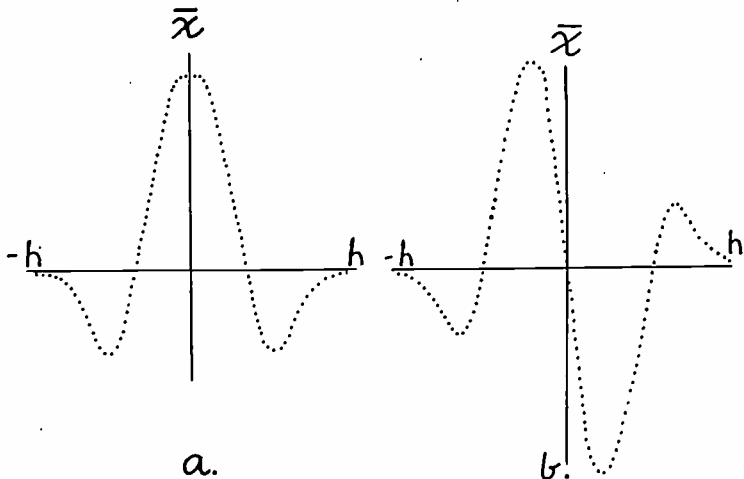
Fig. 1—Possible field distributions along one wire of a parallel line due to a coupled oscillator. a. Direct or cosine symmetrical curve. b. Inverted or sine symmetrical curve.
