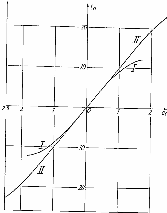
Fig. 7—Curve I shows the main-amplifier characteristic: 10e_i - e_i^3 , and curve II the resulting characteristic: 10e_i - (1/10^3)e_i^9 .
