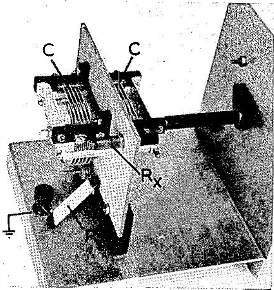
Fig. 3—Bridged-T resistance-measuring set.
