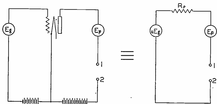
Fig. 1—Circuits which are assumed to have equivalent impedances at terminals 1 and 2.
