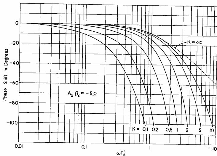
Fig. 13—High-frequency phase shift, feedback factor -5.0 .
