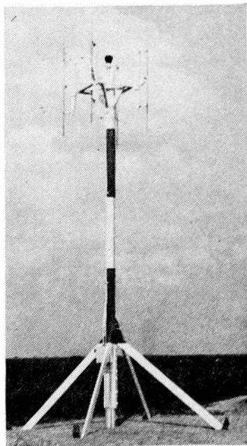
Fig. 5—Preliminary design of the ultra-high-frequency radio-range transmitting antenna.
