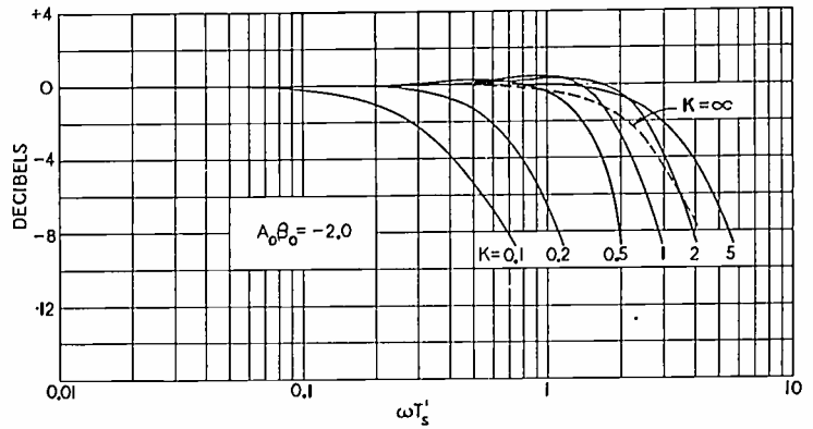
Fig. 9—High-frequency response, feedback factor -2.0 .
