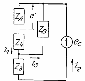
Fig. 3—Simplified diagram for calculating the magnitude of the feedback. Z_3 in this figure is equal to (Z_3+Z') in Fig. 1.
