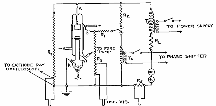
Fig. 2—Diagram of connections.
