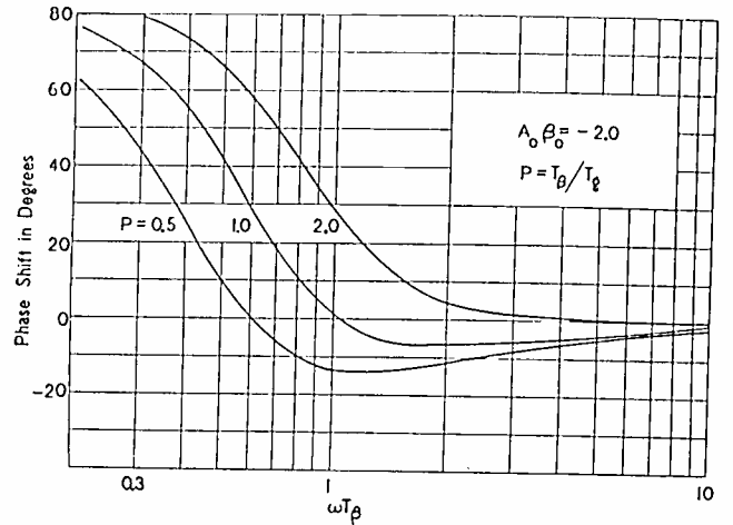
Fig. 5—Low-frequency phase shift, feedback factor -2.0.
