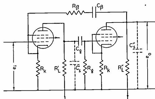
Fig. 1—A schematic wiring diagram of a typical output amplifier and driver having feedback applied across two stages.
