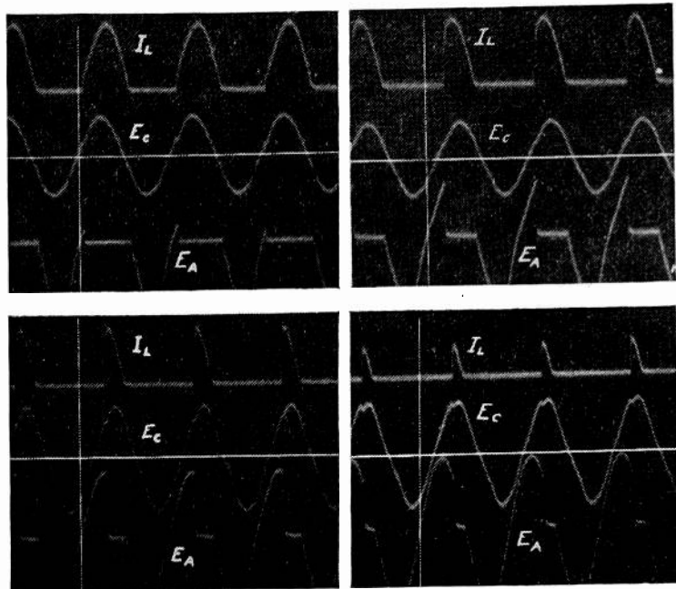
Fig. 5—Oscillograms of voltage and current relations. I_L = average current through rectifier. E_C = control voltage. E_A = voltage across rectifier.
