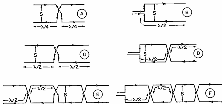
Fig. 1—Six types of "flat-top beam" antennas.
