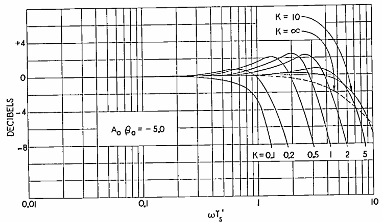
Fig. 10.—High-frequency response, feedback factor -5.0 .
