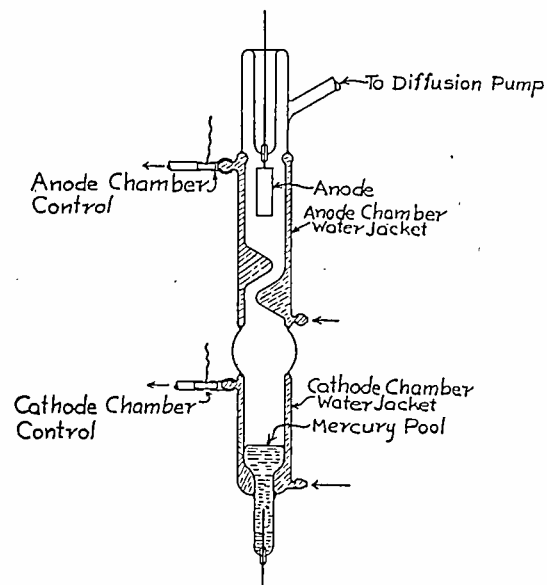
Fig. 9—Sectional view of surface-controlled rectifier having independent temperature control of anode and cathode chambers.
