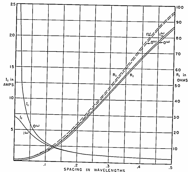
Fig. 4—Current and resistance of each element of an array of two out-of-phase elements as a function of spacing.
