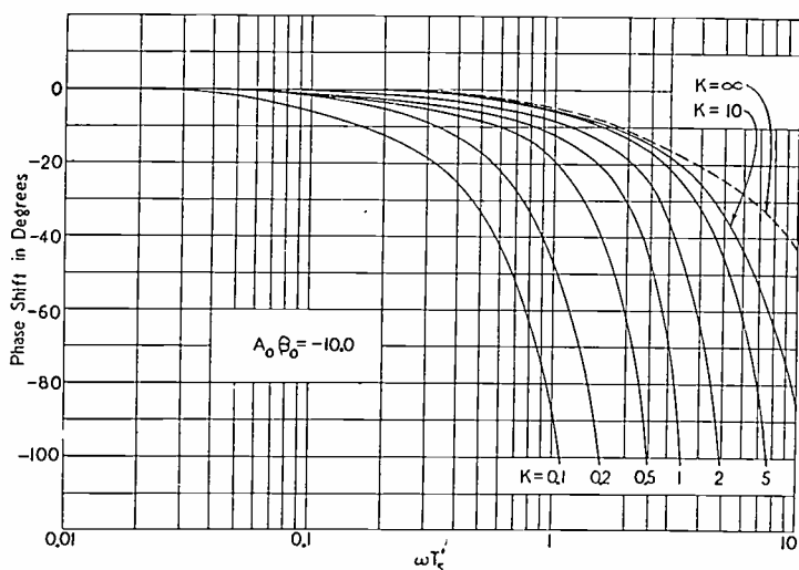
Fig. 14—High-frequency phase shift, feedback factor -10.0 .
