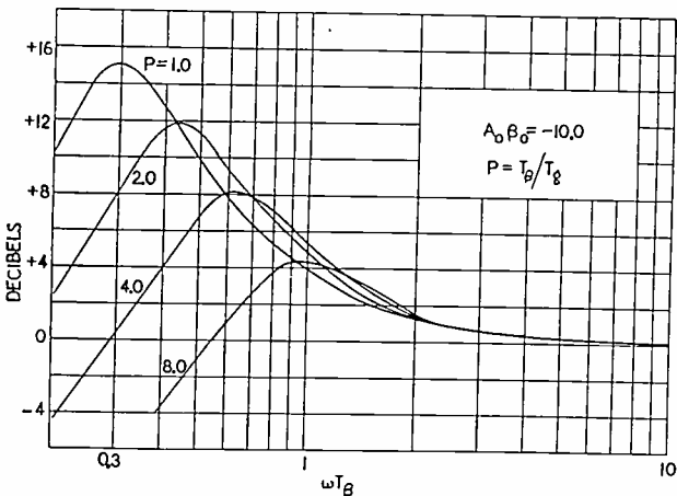
Fig. 4—Low-frequency response, feedback factor -10.0.
