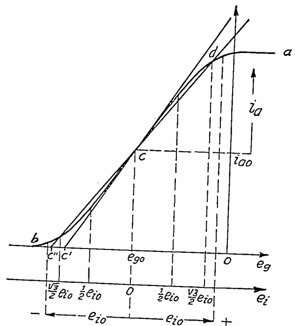
Fig. 5—Characteristic of the main amplifier.
