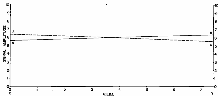
Fig. 2—Sector X-Y of A and N field-strength contours 52 miles from the range transmitter. (Theoretical.)
