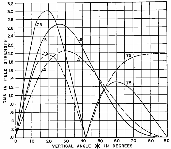
Fig. 7—The gain of an array of two horizontal out-of-phase elements over a half-wave antenna in free space for various vertical angles is shown by the solid curves. The gain of a single horizontal half-wave antenna is shown by the dashed curves. The gains are given for antenna heights of 0.5 and 0.75 wavelength above ground. The array spacing is one-eighth wavelength.
