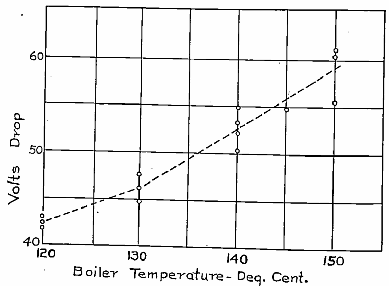
Fig. 4—Voltage drop versus boiler temperature for average current of 30 amperes, rectifier of Fig. 1.
