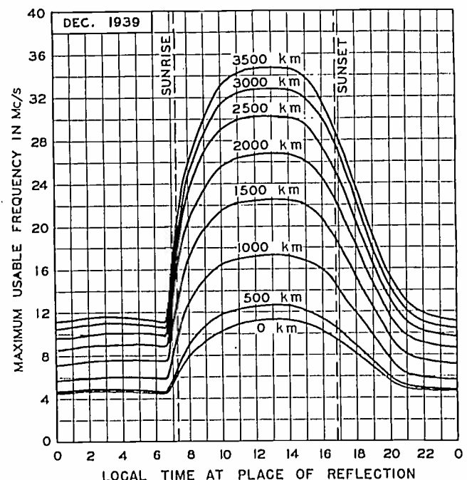
Fig. 2—Maximum usable frequencies for dependable radio transmission via the regular layers, average for undisturbed days for December, 1939.
