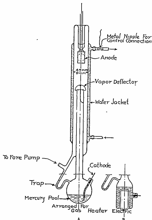
Fig. 1—Sectional view of Cordes-type surface-controlled mercury-pool rectifier.
