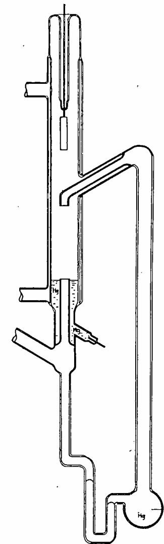
Fig. 8—Sectional view of jet-type surface-controlled rectifier.
