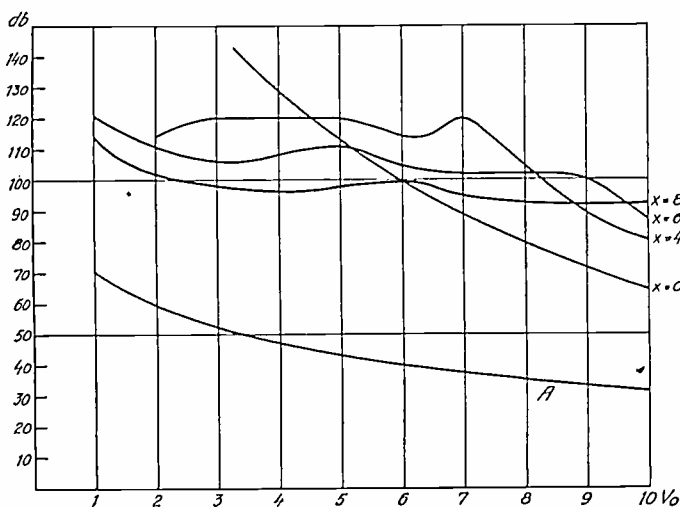
Fig. 9—Value of the "klirr-factor" for the resulting amplification, given in decibels below the linearly amplified fundamental note (a_1 - x a_3) V_0 \sin \omega t .
