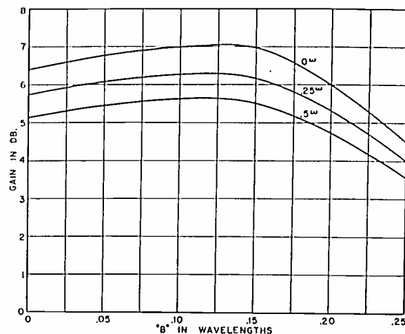
Fig. 10—Effect of variation of B on the gain of the four-element array for loss resistances of 0, 0.25, and 0.5 ohm. The value of A is 0.25 wavelength.
