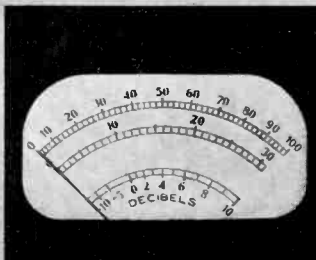
Illuminated linear meter with auxiliary db scale
