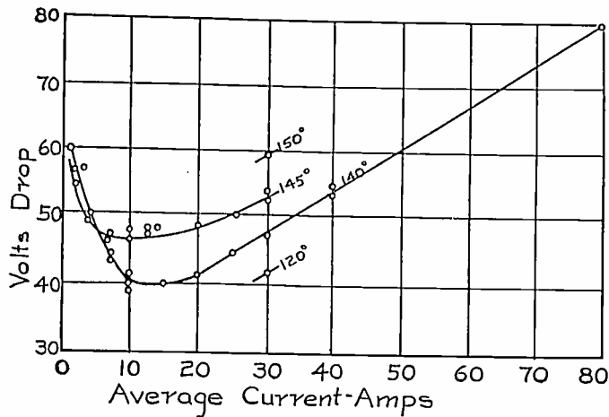
Fig. 3—Voltage drop through the rectifier of Fig. 1 versus average current for several boiler temperatures.
