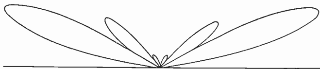
Fig. 6—Field in a vertical plane radiated from a 63-megacycle range antenna array 3\lambda/2 above a typical earth.
