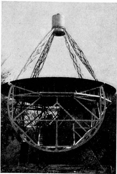
Fig. 1—Antenna system used for the investigation of cosmic static.
