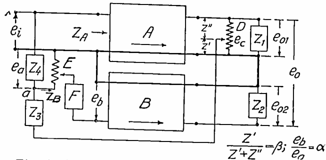
Fig. 1—Principle schematically. A = main amplifier, B = auxiliary amplifier.
