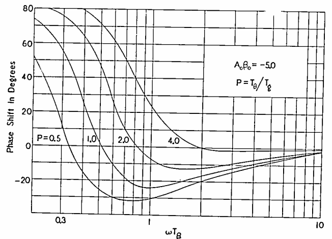
Fig. 6—Low-frequency phase shift, backfeed factor -0.5.
