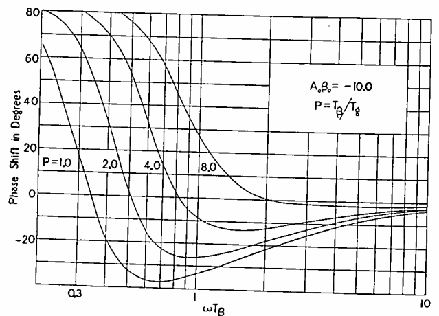
Fig. 7—Low-frequency phase shift, feedback factor -10.0.
