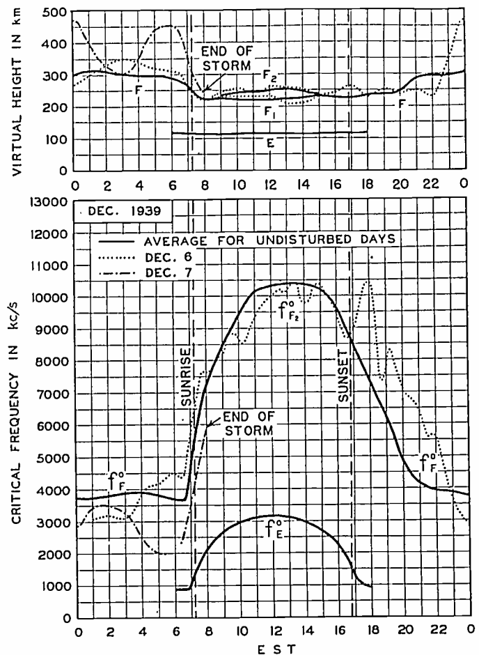
Fig. 1—Virtual heights and critical frequencies of the ionospheric layers, December, 1939. The solid-line graphs are the averages for the undisturbed days; the dotted-line graphs are for the ionospheric storm day of December 6, and the dot-dashed graphs for December 7. Reflections were too diffuse for critical-frequency measurements at 0000 December 6 and 0600 December 7.
