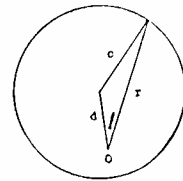
Fig. 6—Plan view of the Milky Way. Earth and sun at point O.
