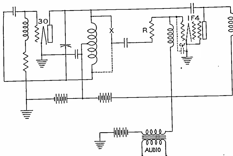
Fig. 2—Experimental frequency modulator
