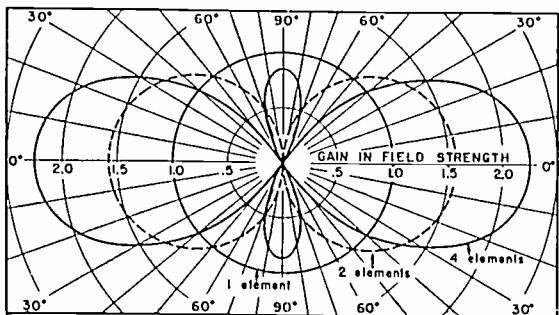
Fig. 9—Free-space radiation patterns of one-, two-, and four-element arrays, all having the same power input. The patterns are shown in the plane perpendicular to the elements.
