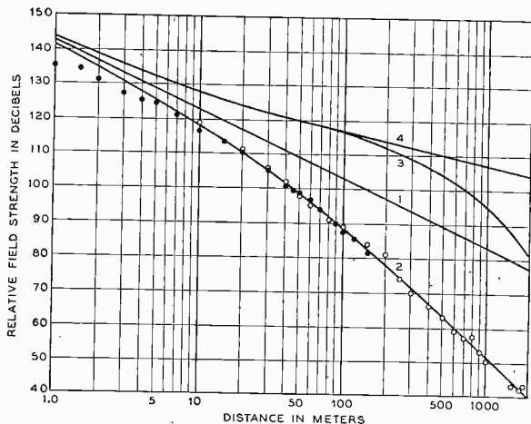
Fig. 3—Variation of received field strength with distance. Curve (1) is plot of equation (1) showing the inverse distance field that would result from propagation over plane earth of perfect conductivity. Curve (2) is a plot of equation showing the variation of the received field strength according to Weyl and Norton. Curves (3) and (4) are plots of equation (3) showing the variation of the received field strength according to Sommerfeld and Rolf. Curves (2) and (3) are based on a dielectric constant of 82.1, a conductivity of 4.05 \times 10^8 electrostatic units and a wave length of two meters. Curve (4) is for a perfect dielectric. The experimental points were obtained on a wave length of two meters with loaded quarter-wave doublets whose mid-points were 0.52 and 0.60 meter above the surface of the water. The solid circles represent measurements made with two boats and the open circles represent measurements made with one boat.
