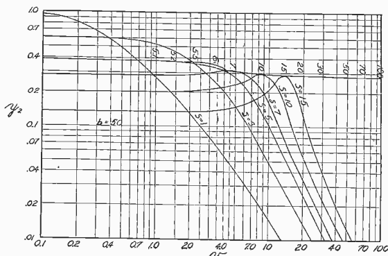
Fig. 5—Universal resonance curves for a circuit resistance ratio of 49.98:1.
