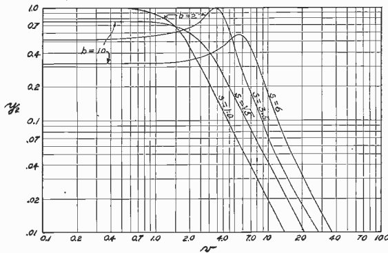
Fig. 7—Comparisons of curves having different values of s and b .
