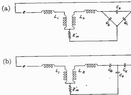
Fig. 2(a)—Coupled pair with capacitance between the high potential sides of the windings.
