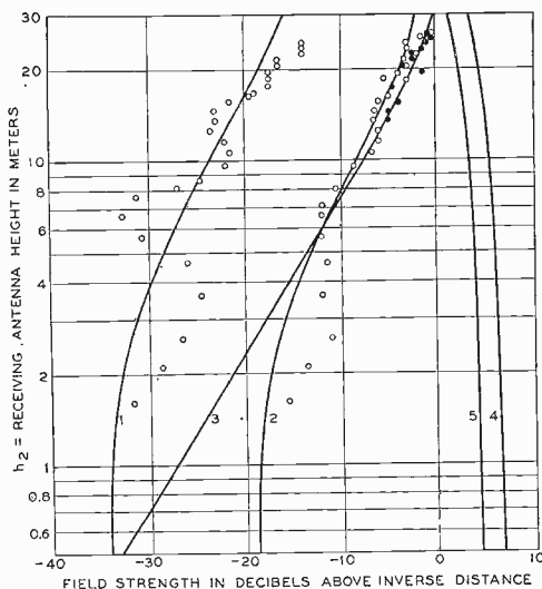
Fig. 5—Variation of received field strength with antenna height. Path length, 1800 meters. Curves (1) and (2) are plots of equation (9) for h_1 equal to 2.5 and 24.8 meters, respectively, which apply to vertical polarization if there is no surface wave. Curve (3) is a plot of equation (9) for h_1 = 24.8 meters which applies to horizontal polarization. Curves (4) and (5) are plots of the surface wave given by equation (8) for h_1 equal to 2.5 and 24.8 meters, respectively. The two sets of open circles represent experimental data taken on vertical polarization with h_1 equal to 2.5 and 24.8 meters, respectively. The solid circles represent experimental data taken on horizontal polarization with h_1 = 24.8 meters.
