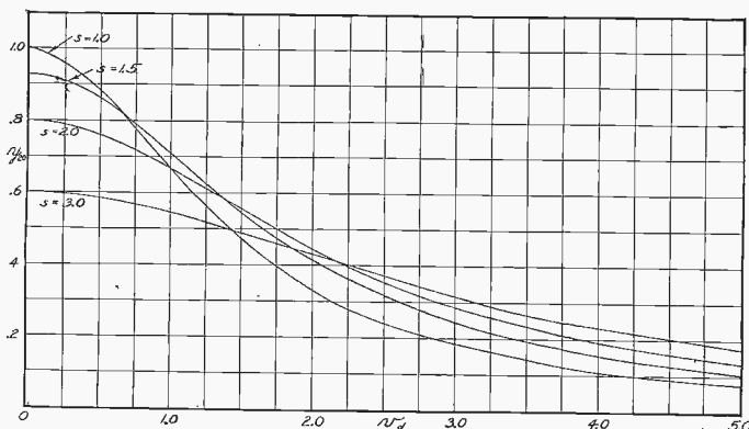
Fig. 19—Curves of gain at the center of the passed band versus the detuning parameter in the case of equal circuit resistances.
