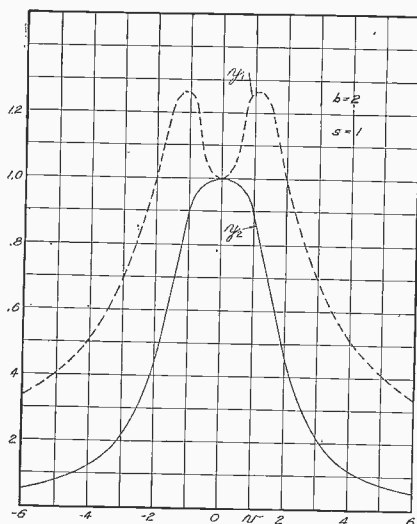
Fig. 13—Comparison of primary and secondary currents for the case of equal circuit resistances and critical coupling.
