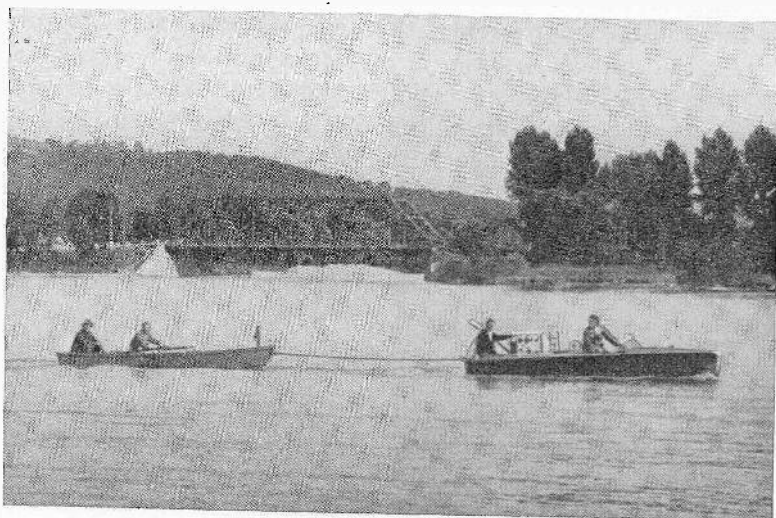
Fig. 1—Experimental arrangement for determining the variation of the received field strength with distance.
