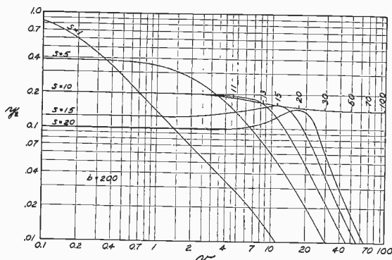
Fig. 6—Universal resonance curves for a circuit resistance ratio of 200:1.
