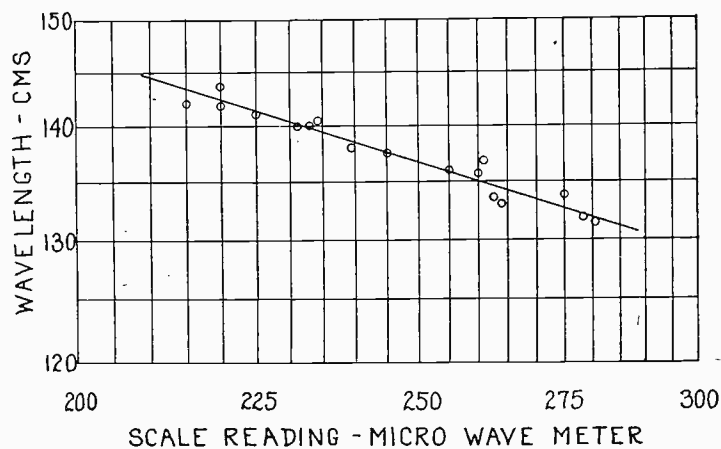
Fig. 4—Calibration curve of microwave meter.
