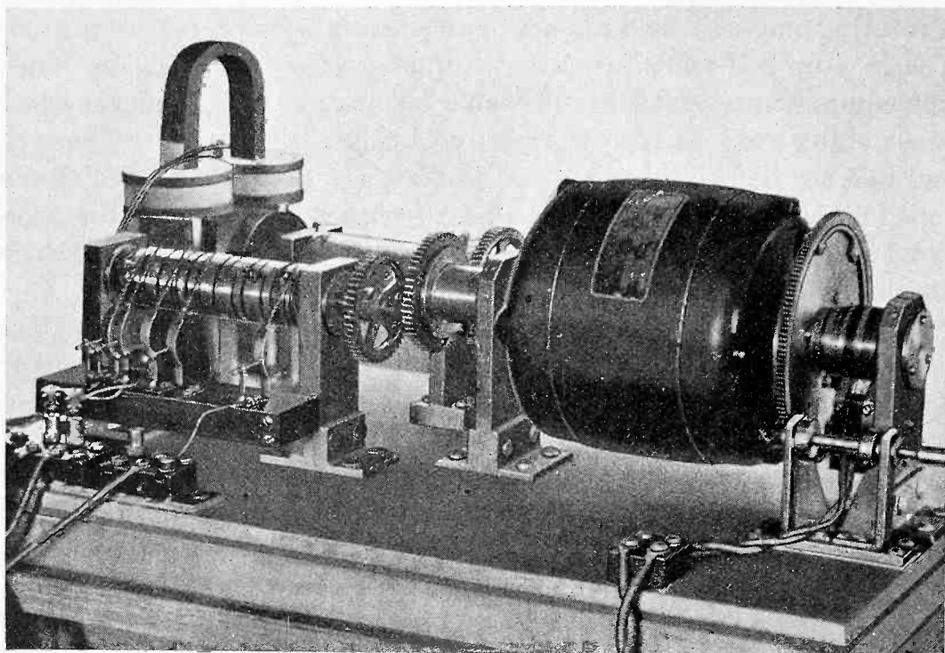
Fig. 14—The synchronizing-commutating unit used in pulse reception. Synchronization is accomplished manually by turning the synchronous motor frame. The sweep circuit is controlled by the "magnetic switch." The outputs from two or three receivers are switched by the drum type commutator.
