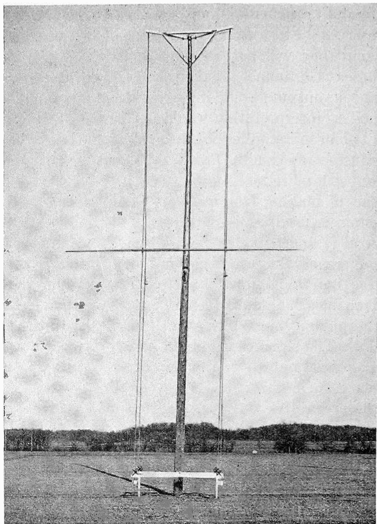
Fig. 7—Horizontal antenna with tackle for varying the height, mounted on a pole 92 feet high. The antenna is attached to the counterweighted boom which is suspended from an endless rope. The structure permits the use of an antenna 20 meters long.
