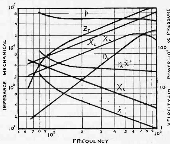
Fig. 1—Characteristics of a cone loud speaker.
