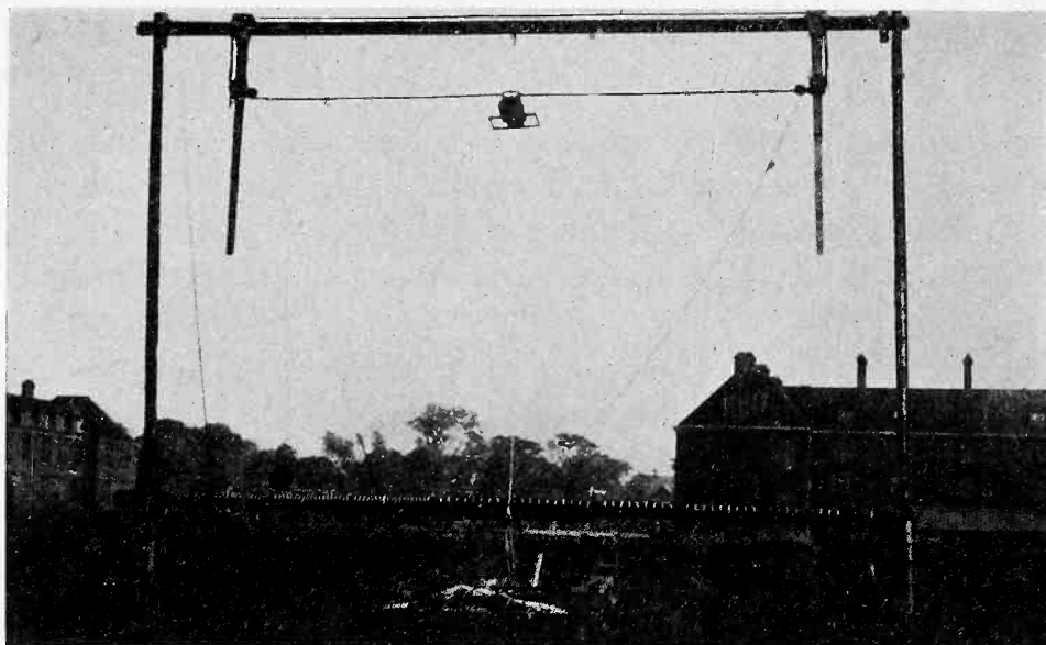
Fig. 10—View of the adjustable frame aerial used for the reflection experiments.
