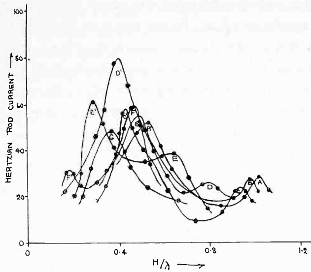
Fig. 12—Radiation measurements.
