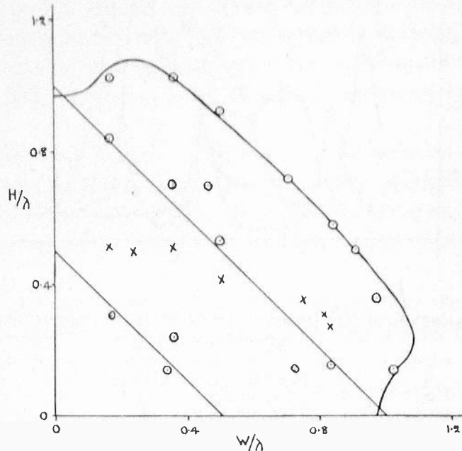
Fig. 8—Comparison of the experimental results with the theoretical curves of Fig. 1.
