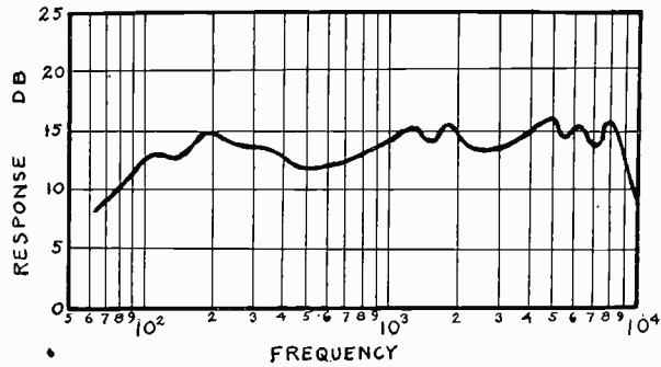
Fig. 9—Response frequency characteristic of the wide range loud speaker sound pressure on the axis of the cone at 10 feet in free space.
