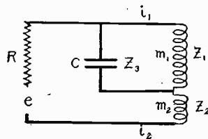
Fig. 4—Electrical circuit of the voice coil system.
