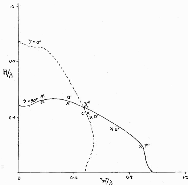
Fig. 15—Graphs showing the theoretical dimensions of a frame for the reception and reradiation of waves reflected off the ground.
