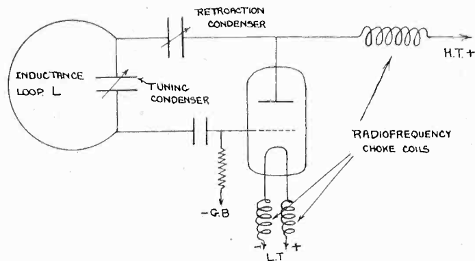
Fig. 3—Circuit diagram of the short-wave transmitter used.
