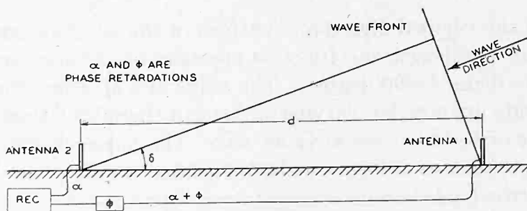
Fig. 11—Similarly spaced antennas used in the phase method. The phase shift \phi is obtained with a variable phase changer.
