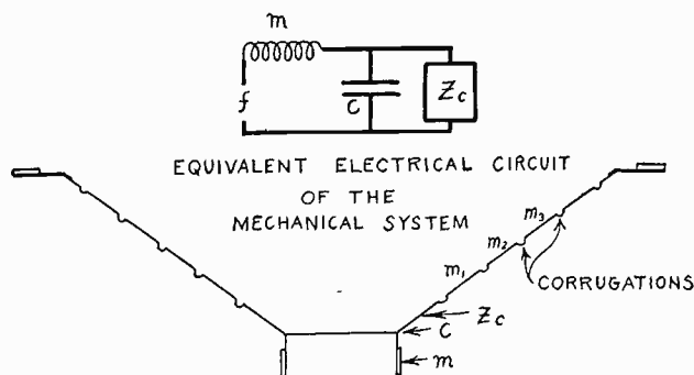
Fig. 2—Mechanical system consisting of a voice coil of mass m , compliance c , and cone impedance Z_c .
