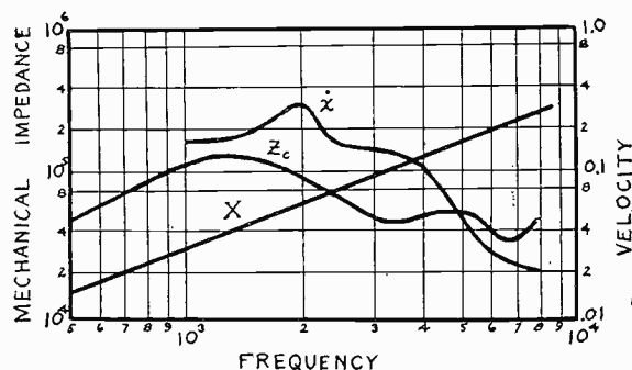
Fig. 3—Characteristics of a cone and a simple driving system.
