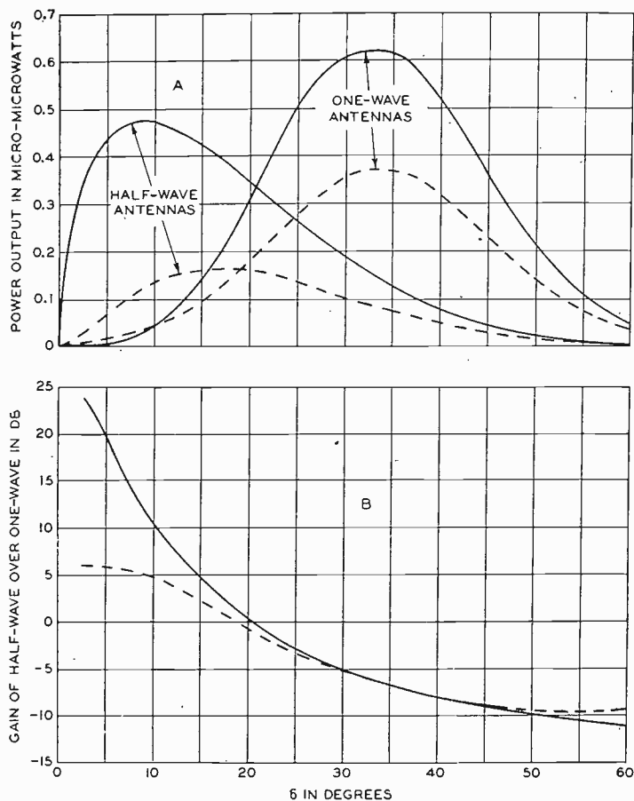
Fig. 4—A shows vertical directional patterns of half-wave and one-wave vertical antennas. The solid curves are for ocean water (dielectric constant = 80, conductivity = 4 \times 10^{-11} e.m.u.). The broken curves are for Holmdel ground (dielectric constant = 25, conductivity = 1.3 \times 10^{-13} e.m.u.). The wavelength is assumed to be 25 meters and the incident field intensity one microvolt per meter. In B the ratio of power expressed as a gain is plotted for the two types of ground. The angle \delta is measured from the horizontal. The lower ends of the antennas are assumed to be in close proximity to the ground.
