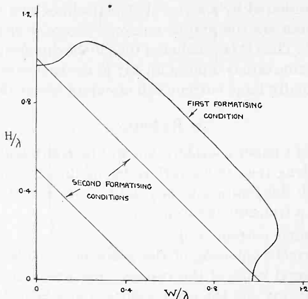
Fig. 1—Graph showing the theoretical dimensions of a transmitting frame for maximum current.
