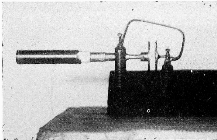
Fig. 3—Photograph of microwave meter.
