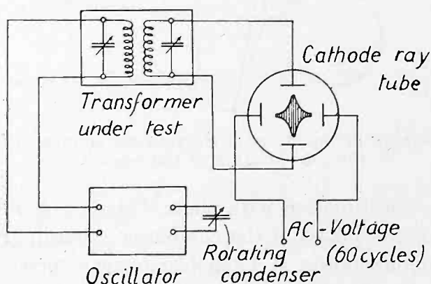
Fig. 1—Device for showing resonance curves with the cathode ray tube.
