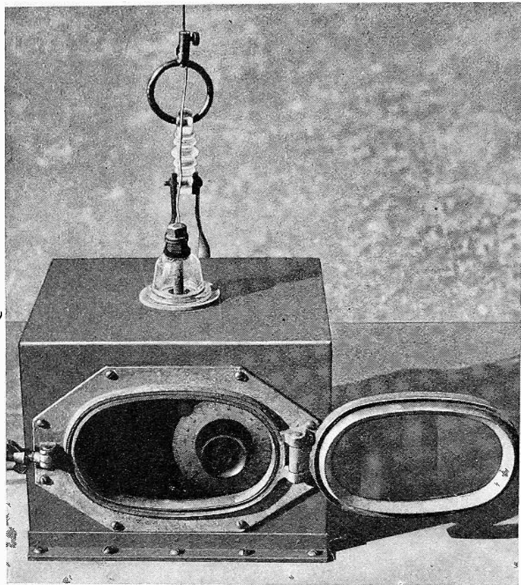
Fig. 9—Terminating equipment used to connect a vertical antenna to the buried concentric transmission line.
