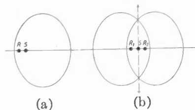
Fig. 1—(a) Propagation of transmitting dipole S and reflector R . (b) Propagation diagram of transmitting dipole S with two reflectors.
