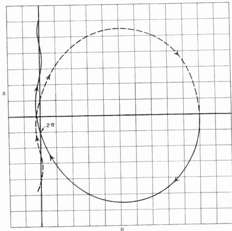
Fig. 13—Modification of Fig. 12 produced by added inductance.
