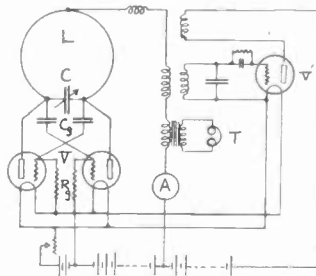
Fig. 1—Circuit of superregenerative wave meter. C_0 = 0.0001 microfarad, R_0 = 1 megohm.
