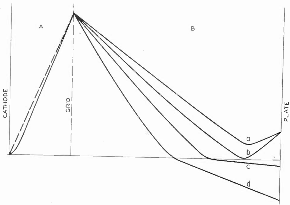
Fig. 9—Potential distributions in positive grid triodes.
