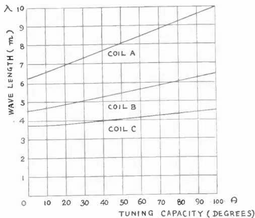
Fig. 2—Calibration curve of wave meter.
