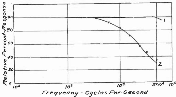
Fig. 3—1. Vacuum photocell and amplifier. 2. Calculated relative input impedance when total shunt capacitance is 274 micromicrofarads. x. Experimental check, same capacitance.
