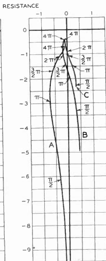
Fig. 16— R_0 - X_0 diagram for positive grid, slightly negative plate triode, without cathode space charge.
