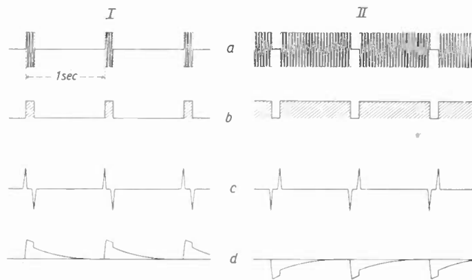
Fig. 13—Method of visual indication.
