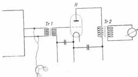
Fig. 11—Circuit of simultaneous acoustic and visual indication.
