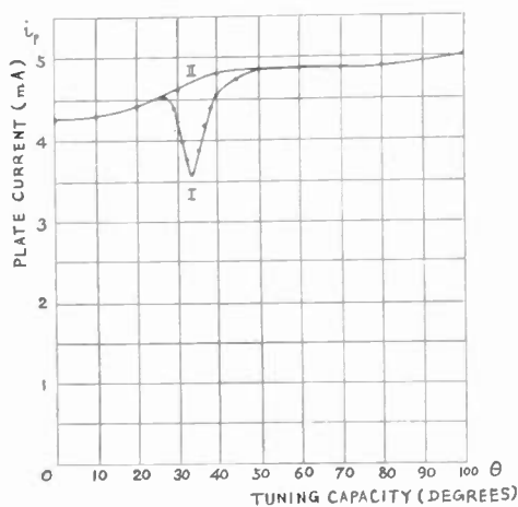
Fig. 3—Resonance curve of wave meter.
