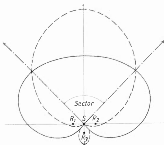
Fig. 10—Same beacon as in Fig. 9. Reflectors R_1 and R_2 keyed simultaneously for marking a sector.
