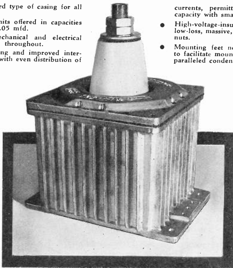
C-D BOMBARDER CAPACITOR TYPE 75A
