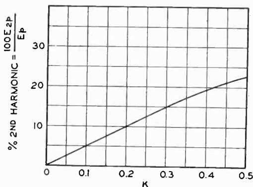
Fig. 9—Harmonic distortions occurring in the detection of a 100 per cent modulated weak signal in the presence of a strong unmodulated carrier.
