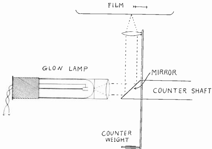
Fig. 6—Optical system. Portable recorder.
