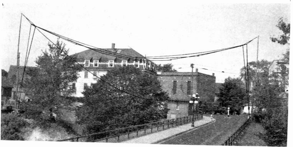
Fig. 1a—Transmitter location and antenna structures at Portsmouth Navy Yard (Kittery, Maine).
