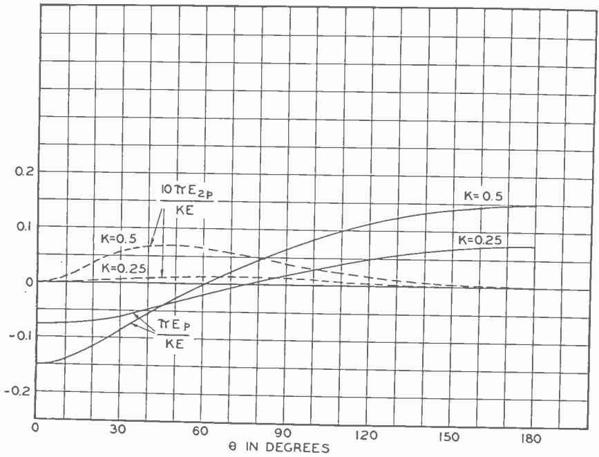
Fig. 3—Conditions are the same as in Fig. 2, except that the weaker carrier is modulated 30 per cent.
