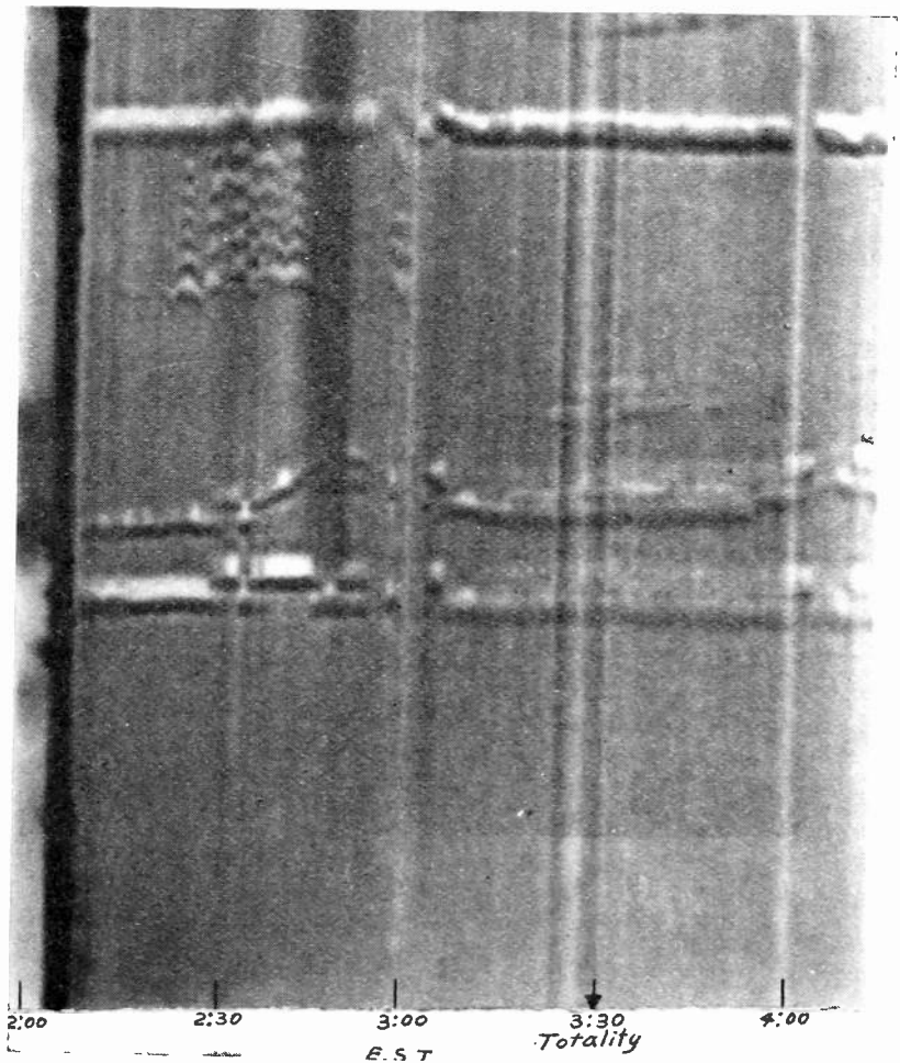
Fig. 6—Photographic record as observed at Seabrook Beach, New Hampshire, showing layer height variations on 3492.5 and 4550 kilocycles during eclipse.
