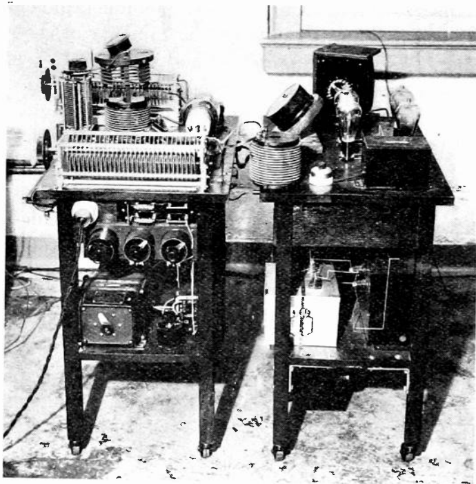
Fig. 8—Transmitting equipment used at Portsmouth.
