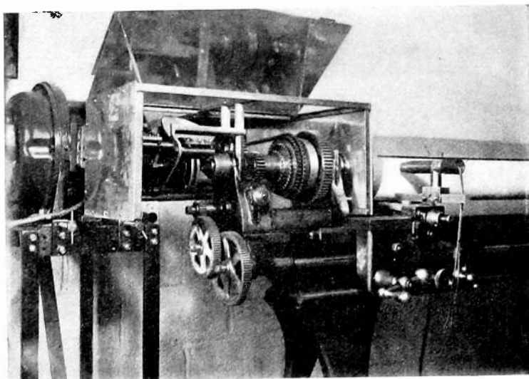
Fig. 3—Gear box. Rotating drum recorder.
