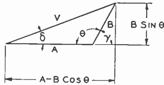
Fig. 1—Two waves of amplitudes A and B , respectively, and differing in phase by an angle \gamma , may be combined into a single wave of amplitude V and of phase angle \delta , as here indicated.
