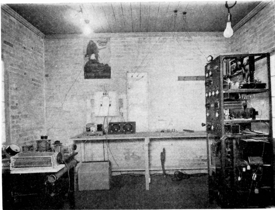
Fig. 1b—Inside view of building housing transmitters. 500-watt (modified) Navy transmitter is shown on right; 250-watt transmitter on left.
