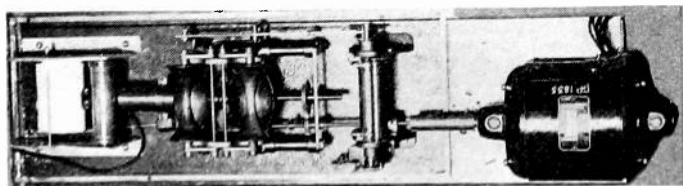
Fig. 5—Top view of portable recorder. Photographic tape has been removed in order to show the interior mechanism.
