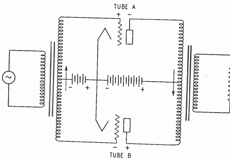
Fig. 1—Typical push-pull audio amplifier.
