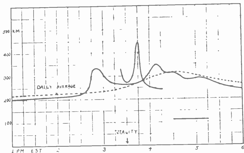
Fig. 10—Layer heights during the eclipse period.
