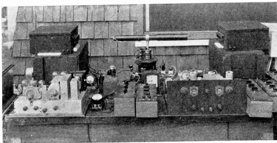
Fig. 2—Assembly of recorder for 3492.5- and 4550-kilocycle channels showing receivers, rotating lamp, and cameras.
