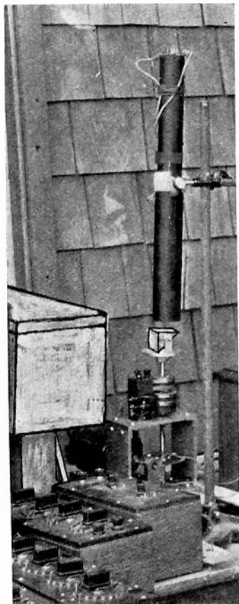
Fig. 3—Modified recorder assembly with stationary lamp.
