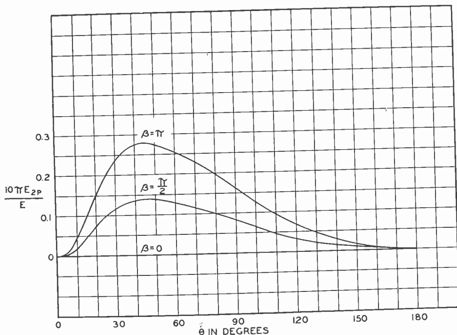
Fig. 7—Second harmonic of output voltage for conditions of Fig. 5.
