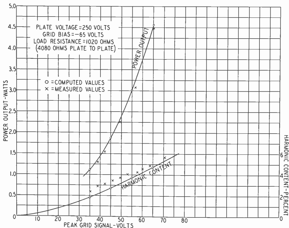
Fig. 6—Comparison between values of power output and harmonic content as computed from Fig. 5 and measured values.
