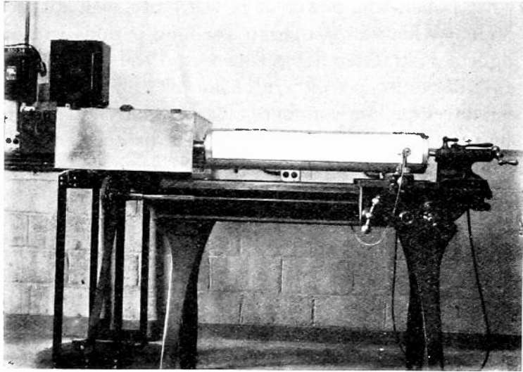
Fig. 1—Rotating drum type of recorder.
