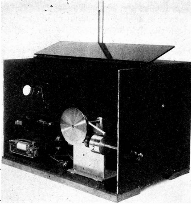
Fig. 2—View of audio-frequency generator with front panel removed.
