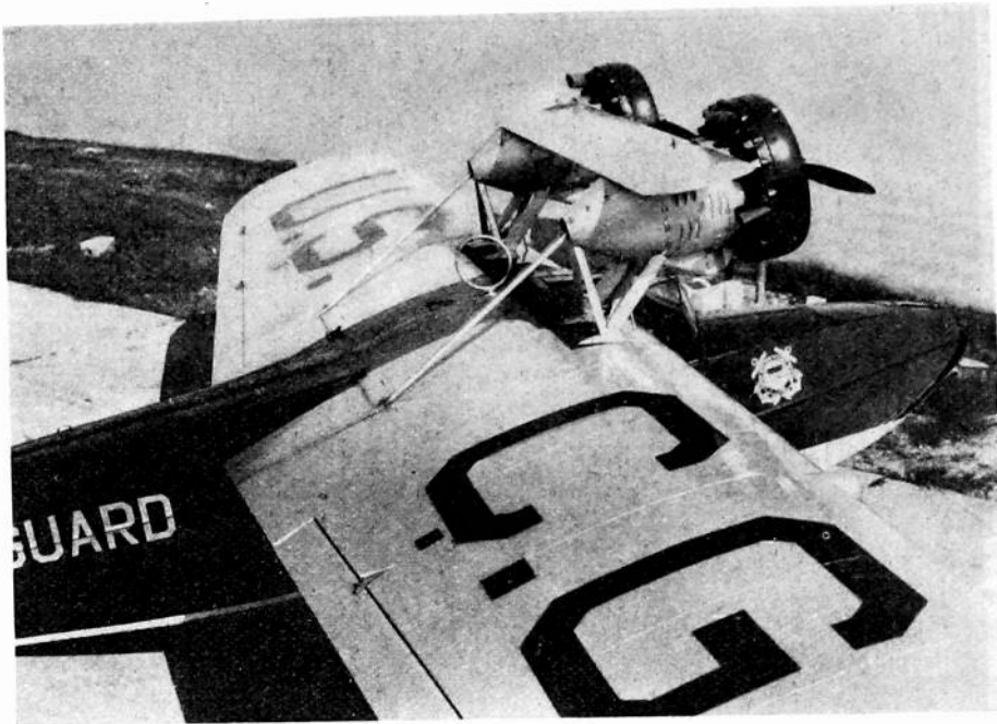
Fig. 31—Model CGR-19-B direction finder loop mounted on U. S. Coast Guard plane.
