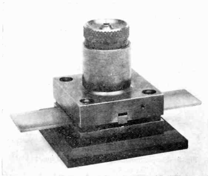
Fig. 4—Mounting for bar-shaped quartz plates.
