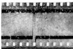
Fig. 1a—Type of pulse received in the absence of sky waves. (Interval between adjacent timing marks in all oscillograms shown is 1/120 second.)
