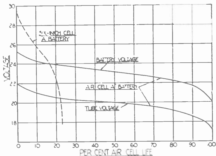
Fig. 1.—Comparative discharge curves of the air cell battery and a series-parallel group of eight six-inch dry cells, assuming an air cell receiver usage of three hours per day. Rated filament current = 0.56 amperes.
