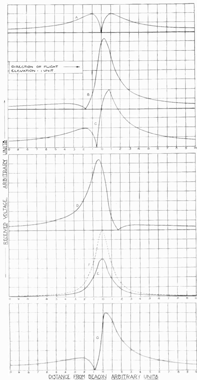
Fig. 3—Graphs of localizing effects for antennas studied. A —vertical antenna or symmetrical T antenna of either longitudinal or transverse type; B —inclined antenna ( \beta_2 = 30^\circ ); C —inclined antenna ( \beta_2 = 60^\circ ); D —trailing wire antenna ( \beta_2 = -30^\circ ); E —horizontal L antenna; F —horizontal V antenna (angle between each wire and fuselage center line = 30^\circ ); G —inclined V antenna, angle between each wire and fuselage center line = 30^\circ , angle of inclination = 45^\circ .
