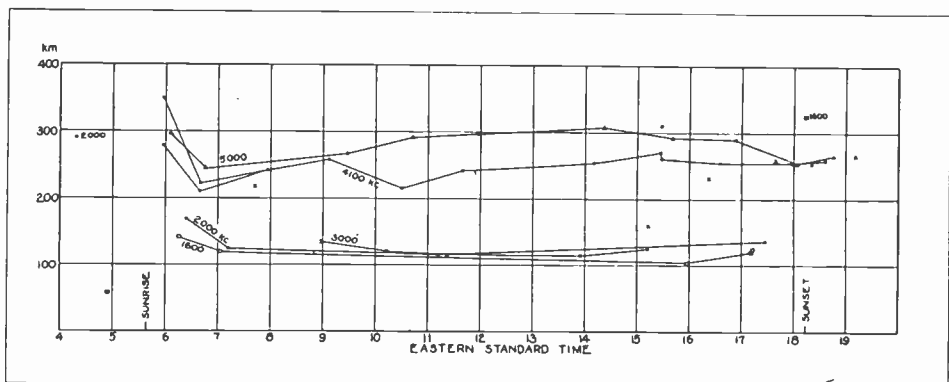
Fig. 9—Diurnal changes on 1600, 2000, 3000, 4100, and 5000 kc September 12, 1930. The lowest distinct height from each oscillogram record is indicated by a cross, and distinct greater heights (not in simple multiple relation) are denoted by dots.
