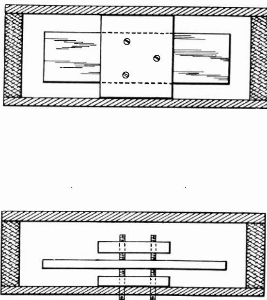
Fig. 3—Mounting for long rectangular quartz plates.
