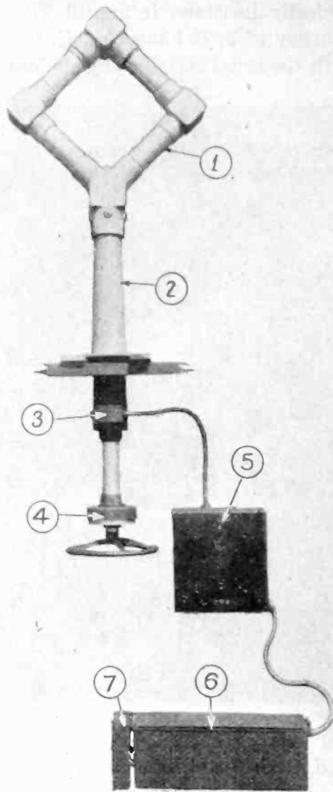
Fig. 21—U. S. Coast Guard radio direction finder, Type-B, Model CGR-18, complete assembly.
