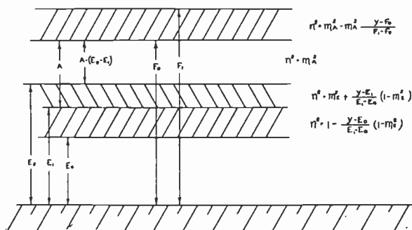
Fig. 14—Layer distribution corresponding to more general variation of n indicated in Fig. 13.
