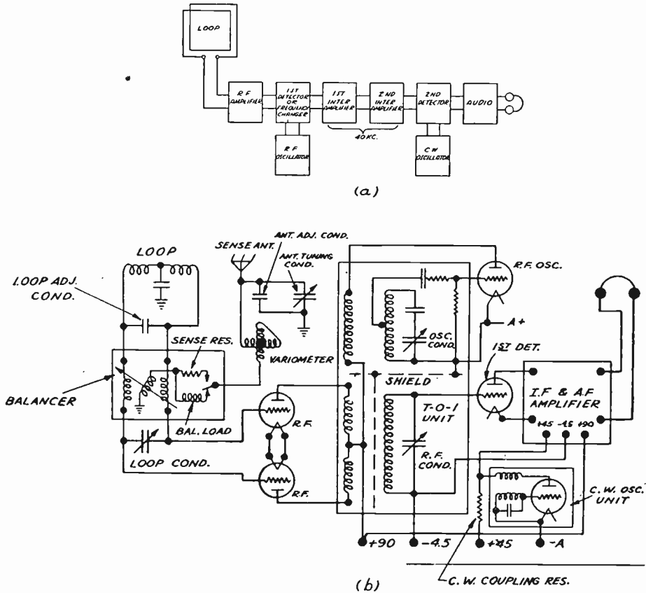
Fig. 24—U. S. Coast Guard radio direction finder schematic circuit arrangement.
