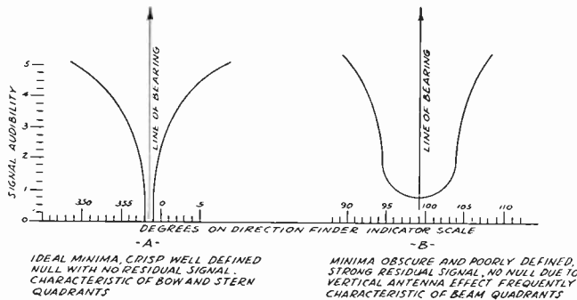
Fig. 2—Residual signal.
