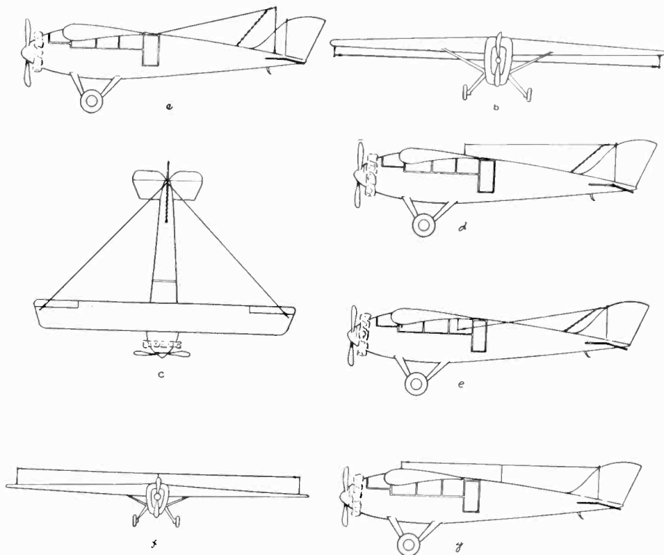
Fig. 1—Experimental installations of antennas studied. a —inclined antenna; b —horizontal dipole antenna (half of this was used for a horizontal L antenna); c —top view, V antenna; d —side view, horizontal V antenna; e —side view, inclined V antenna; f —symmetrical transverse T antenna; g —symmetrical longitudinal T antenna.
