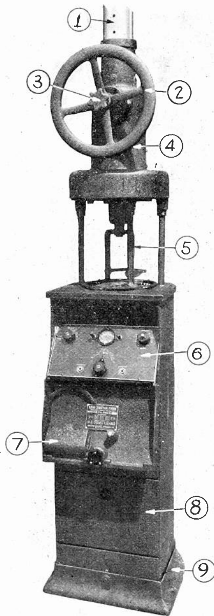
Fig. 18—U. S. Coast Guard radio direction finder, Type-A, Model CGR-17-C, lower assembly.
