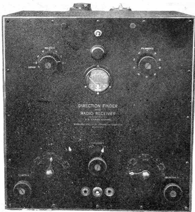
Fig. 22—U. S. Coast Guard radio direction finder, Type-B, Model CGR-18, receiver.
