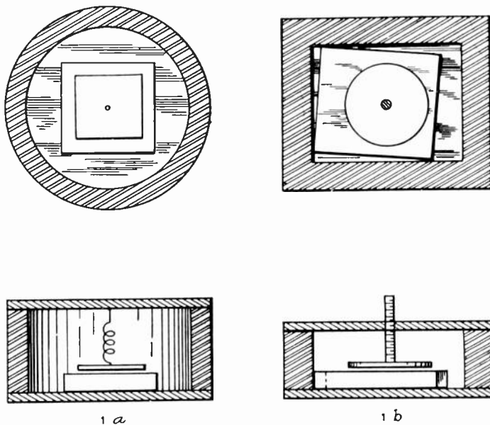
Fig. 1—Types of simple quartz plate holder.
