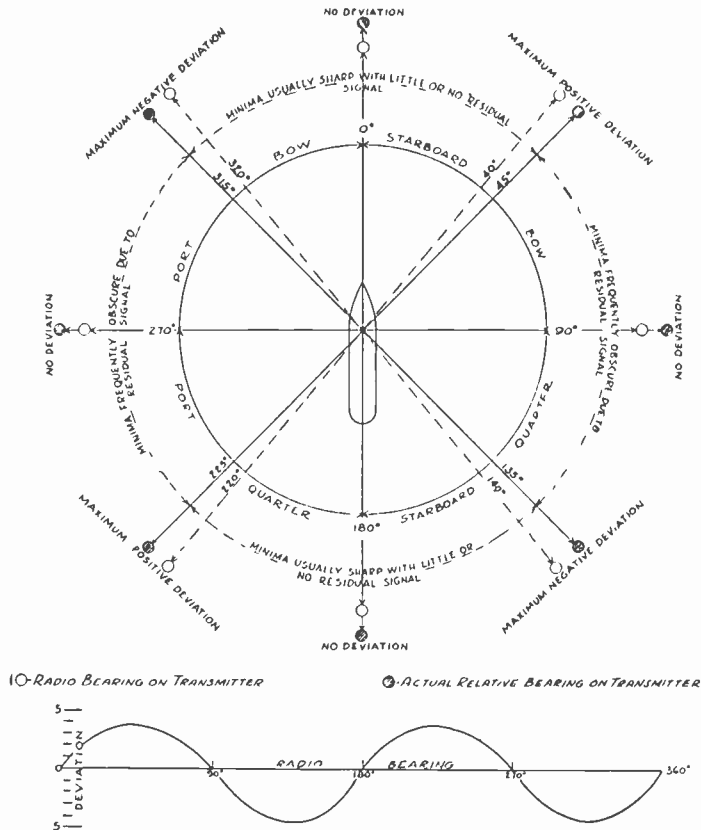
Fig. 3—Normal quadrantal error and minima characteristic.
