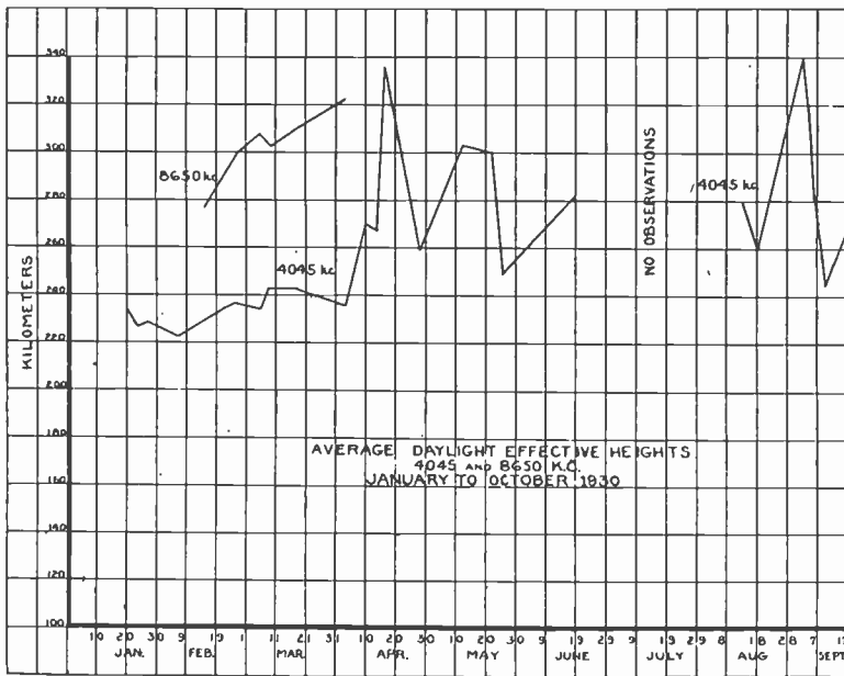
Fig. 2—Average daylight (virtual) heights of the Kennelly-Heaviside layer from January to October, 1930. (4045 and 8650 kc). Note sky waves returned from 8650 kc only between February and April of the period of observations.
