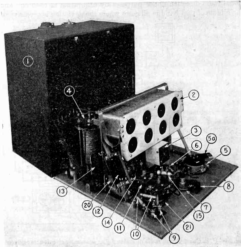
Fig. 23—U. S. Coast Guard radio direction finder, Type-B, Model CGR-18, receiver assembly.
