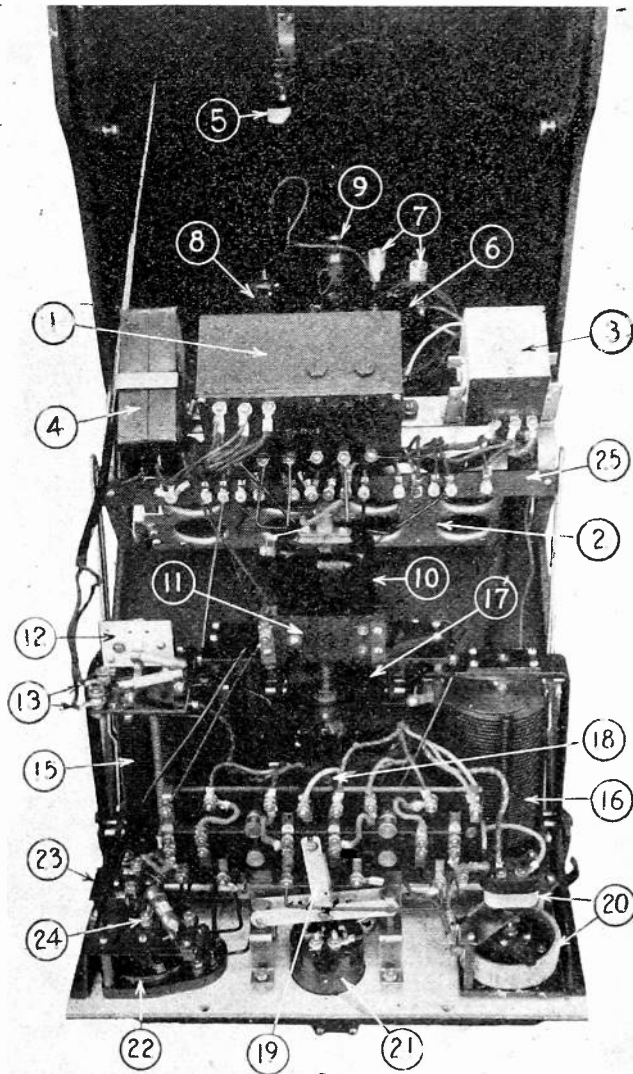
Fig. 20—U. S. Coast Guard radio direction finder, Type-A, Model CGR-17 C, receiver assembly.
