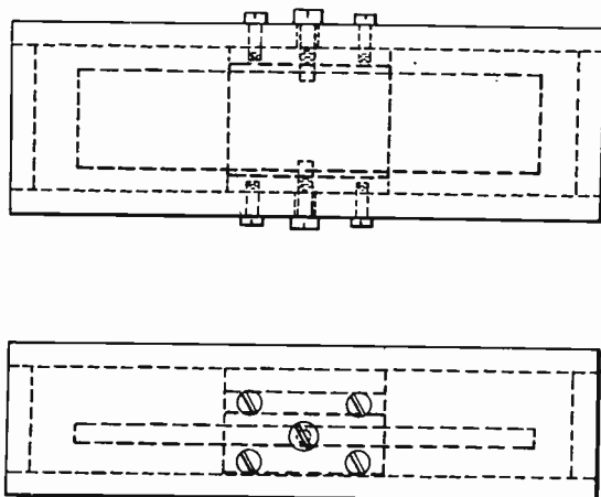
Fig. 2—Mounting for long rectangular quartz plates.
