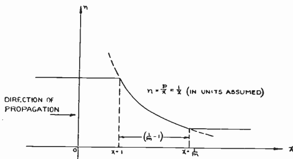
Fig. 17—Form of transition assumed in investigation of reflection (Case III).
