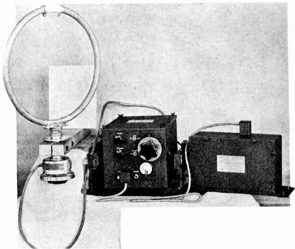
Fig. 26—U. S. Coast Guard aircraft radio direction finder, Model CGR-19-B.
