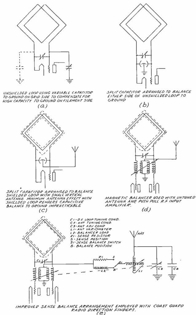
Fig. 1—Evolution of sense-balancer circuit arrangements
