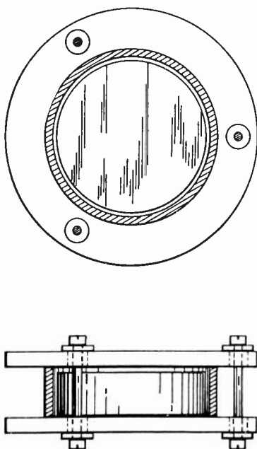
Fig. 5—Simple mounting for cylindrical quartz plates.
