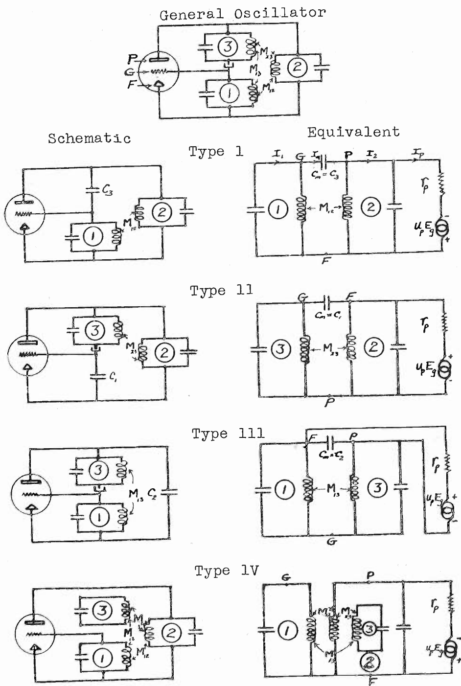
Fig. 2—Schematic and equivalent diagrams of four derived types from the general oscillator.
