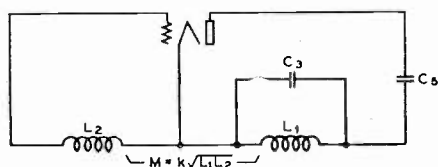
Fig. 11—Reversed feed-back oscillator, plate stabilization.
