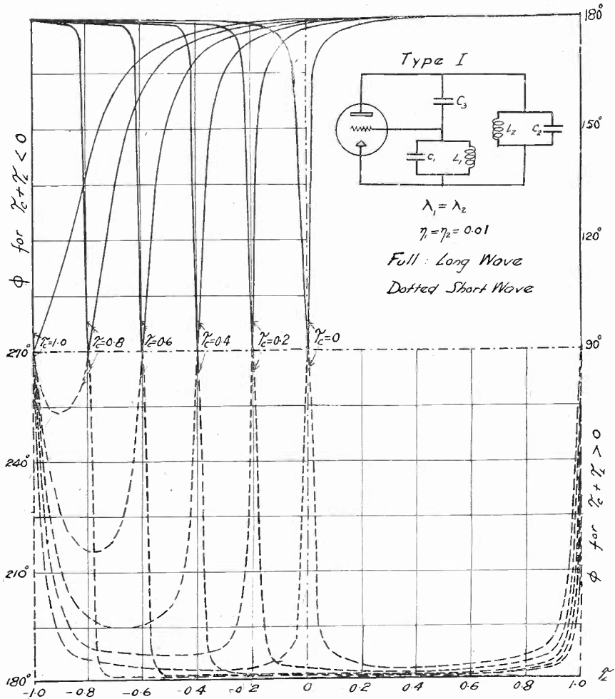
Fig. 14-a— \Phi vs. \tau_L at constant \tau_C for Type I oscillator. Note that the phase relations are completely shown for the long and short waves.
