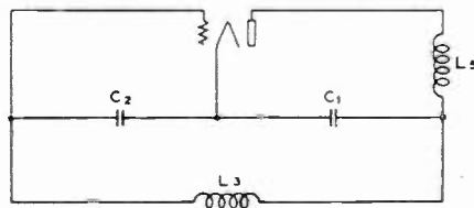
Fig. 5—Colpitts oscillator, plate stabilization.
