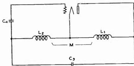
Fig. 3—Hartley oscillator, Grid stabilization.
