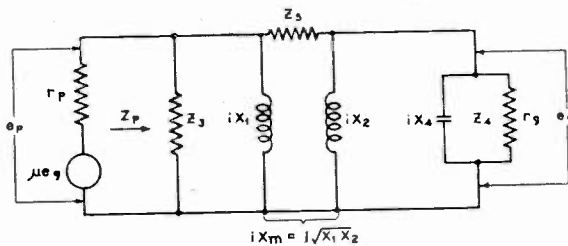
Fig. 15—Equivalent circuit of oscillator with unity coupling.
