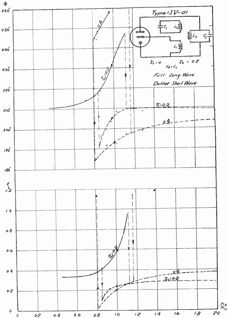
Fig. 29—Experimentally determined \Phi and \epsilon vs. \lambda_2/\lambda_3 for Type IV-a oscillator for two different values of \tau_{23} .
