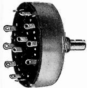
No. 7150A 5 positions, 2 circuits
