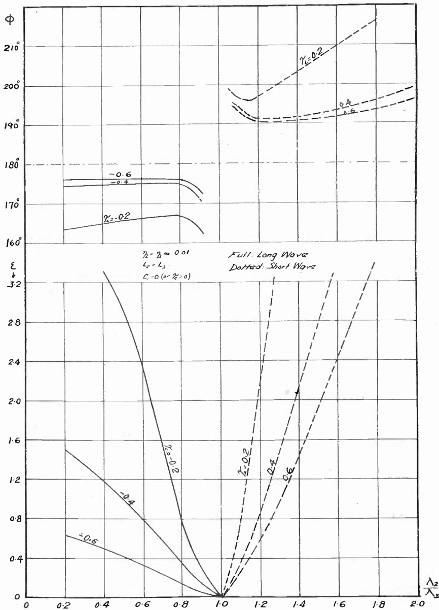
Fig. 20-b— \Phi and \epsilon vs. \lambda_2/\lambda_3 for Type II oscillator ( \tau_C = 0 ) for different values of \tau_L .
