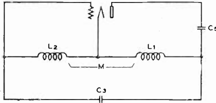
Fig. 2—Hartley oscillator, plate stabilization.
