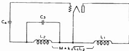
Fig. 9—Feed-back oscillator, grid stabilization.
