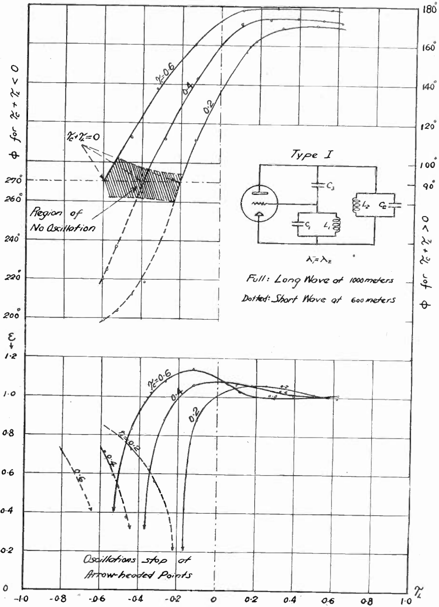
Fig. 26—Experimentally determined \phi and \epsilon vs. \tau_L for Type I oscillator for different values of \tau_C .
