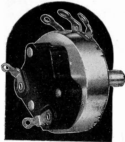
Above: No. 70 Series, with Underwriters' Laboratories Inspected Switch. Rated 1.5 amps., 250 volts; 3 amps., 125 volts. Illustration is actual size.
