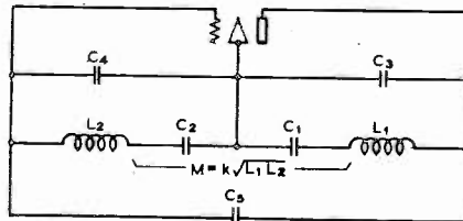
Fig. 18—General circuit of oscillator with unity coupling, plate and grid stabilization.
