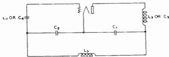
Fig. 7—Colpitts oscillator, plate and grid stabilization.
