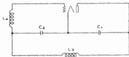
Fig. 6—Colpitts oscillator, grid stabilization.
