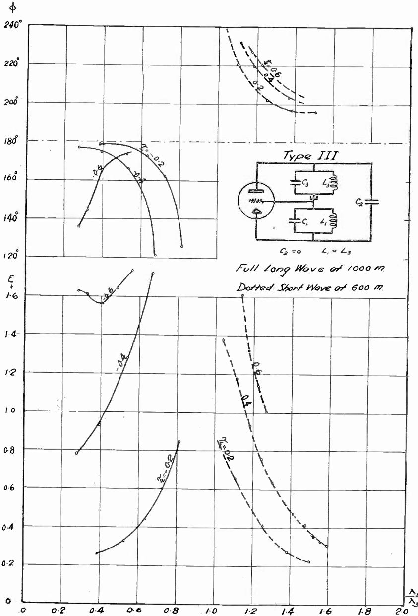
Fig. 28—Experimentally determined \Phi and \epsilon vs. \lambda_1/\lambda_3 for Type III oscillator for different values of \tau_L .
