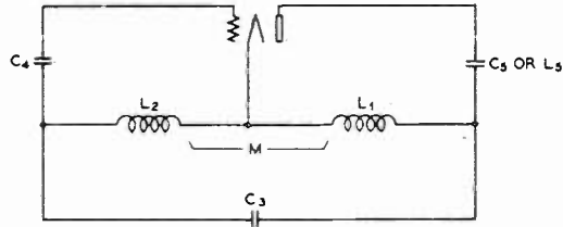
Fig. 4—Hartley oscillator, plate and grid stabilization.
