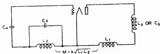
Fig. 10—Feed-back oscillator, plate and grid stabilization.
