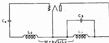
Fig. 12—Reversed feed-back oscillator, grid stabilization.
