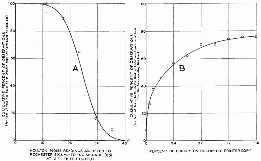
Fig. 6—Cumulative curves of signal-to-noise ratio derived from Houlton noise observations and of per cent of errors on the printer copy observed at Rochester.
