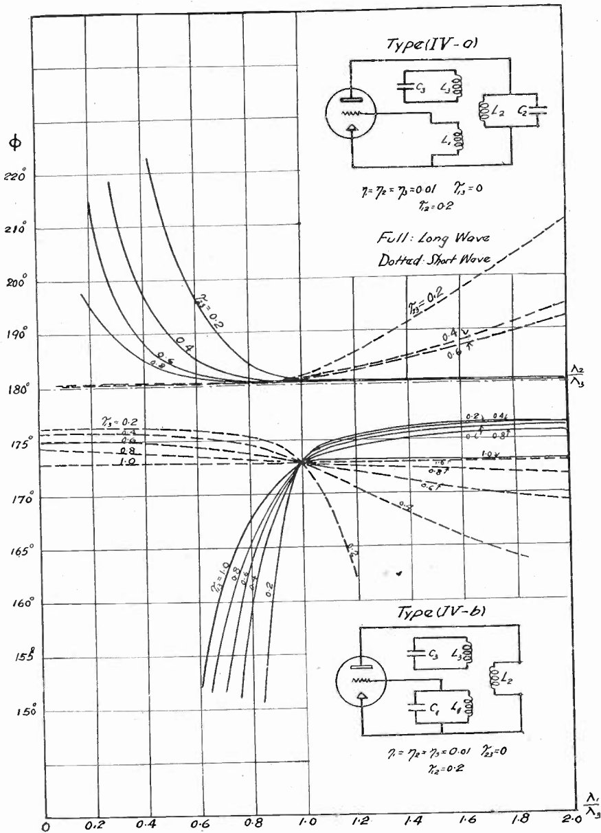
Fig. 23-a—(Above)— \Phi vs. \lambda_2/\lambda_3 for Type IV-a oscillator. Fig. 23-b—(Below)— \Phi vs. \lambda_1/\lambda_3 for Type IV-b oscillator. Note the difference in the angular scale.
