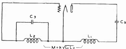
Fig. 8—Feed-back oscillator, plate stabilization.
