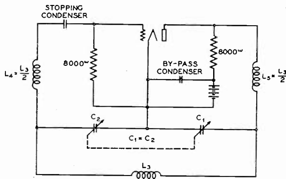
Fig. 19—Practical arrangement of oscillator with three series tuned coupled circuits.
