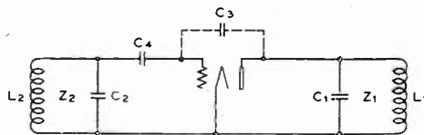
Fig. 14—Tuned-plate, tuned-grid oscillator with no magnetic coupling.
