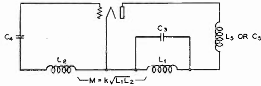
Fig. 13—Reversed feed-back oscillator, plate and grid stabilization.
