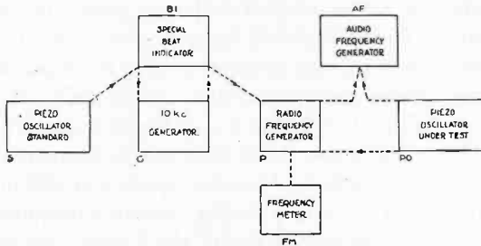
Fig. 2—Diagram of apparatus used in testing piezo oscillators for broadcast stations. The dotted arrows indicate how the various pieces of apparatus work with the remainder of the equipment.
