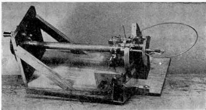
Fig. 1—Tube receiver, wavelength 3 m, first form designed by O. Cords.
