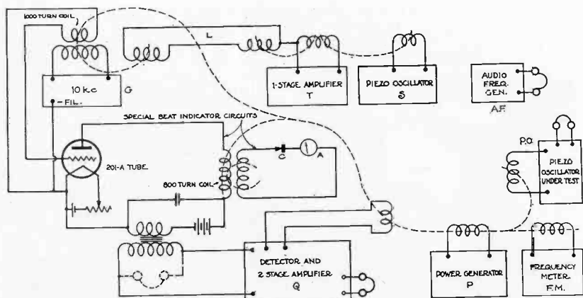
Fig. 3—Schematic diagram of apparatus used in testing piezo oscillators, showing electromagnetic coupling between different units by dotted lines.
