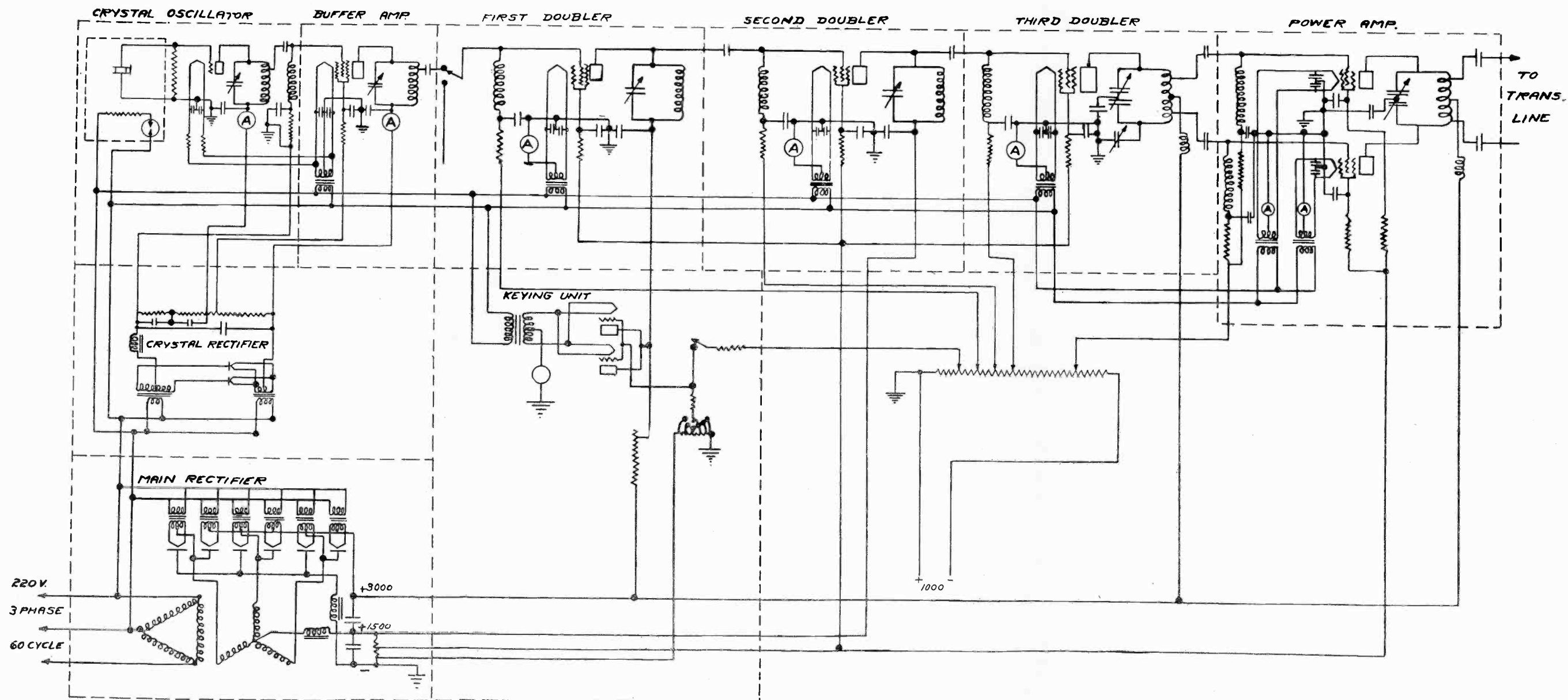
Fig. 1—Exciter unit for 20-40-kilowatt transmitter.
