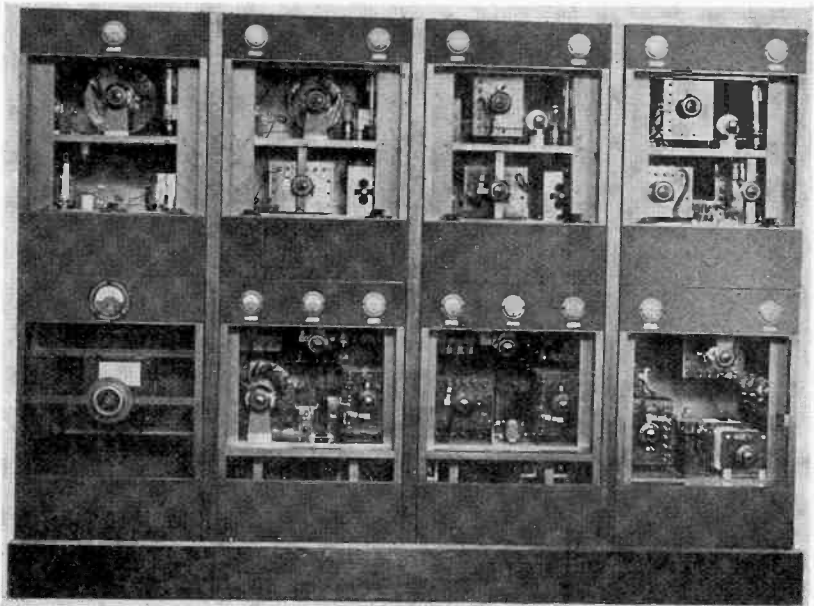
Fig. 3—Amplification equipment, front view. Cover plates removed.
