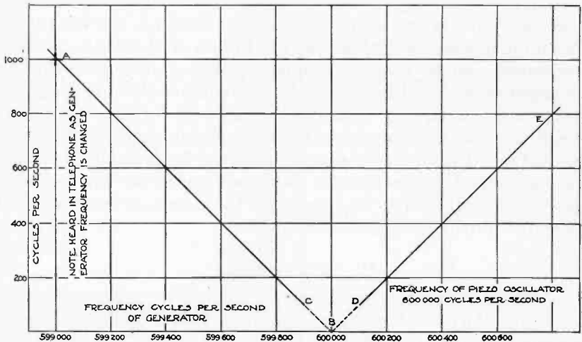
Fig. 1—Diagram illustrating beat note produced between piezo oscillator and a radio-frequency generator whose frequency may be changed.
