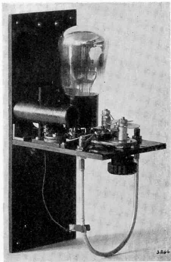
Fig. 6—High-frequency part of transmitter by C. Lorenz, 3 m, 1 to 2 watts.
