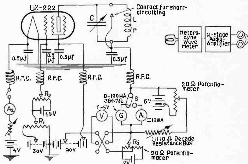
Fig. 3—Circuit arrangement of measurement.
