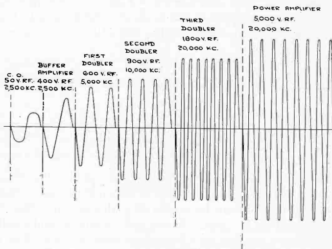
Fig. 4—Frequency multiplication in exciter unit.
