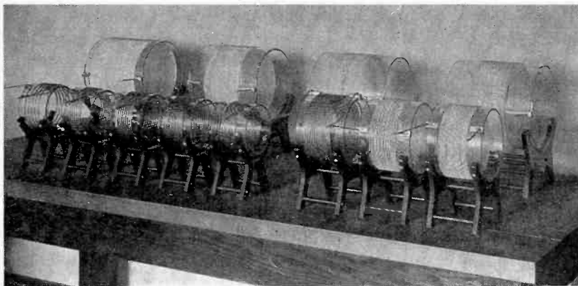
Fig. 5—Series of inductors used on frequency meter shown in Fig. 4. Frequency range covered, 170 to 5350 kc.
