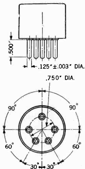
Fig. 9—Essential dimensions of five-pin receiving tube base.
