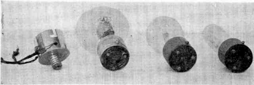
Fig. 1—From left to right: Adaptor, W. E. Co. tube, G. E. Co. tube, and de Forest tube.
