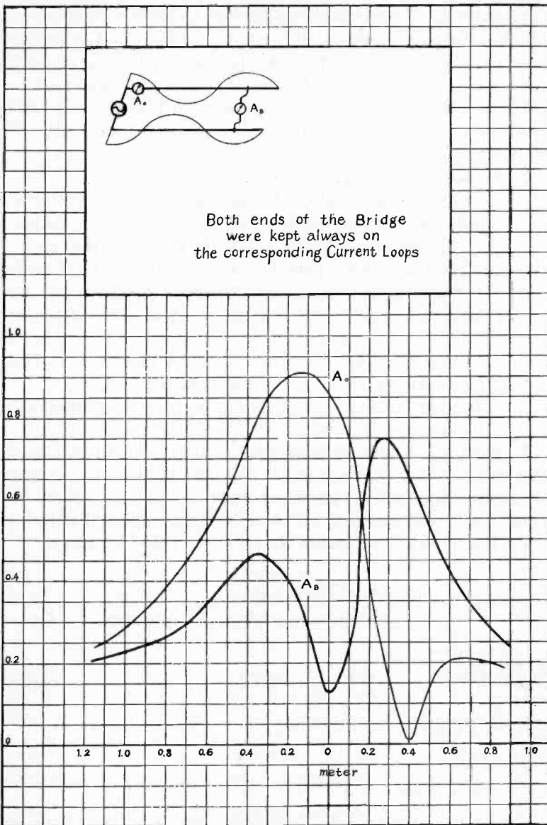
Displacement of Bridge from a Current Loop
