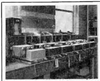
The break-down test. The Operadio Power Units illustrated ran under full load July 28, 1928 to July 28, 1929.
