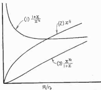
Fig. 3—General form of the functions of x = (R/r_p) occurring in terms (1), (2), and (3) of equation (13).
