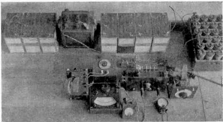
Fig. 1—Laboratory setup of the four-electrode vacuum-tube beat-frequency oscillator.
