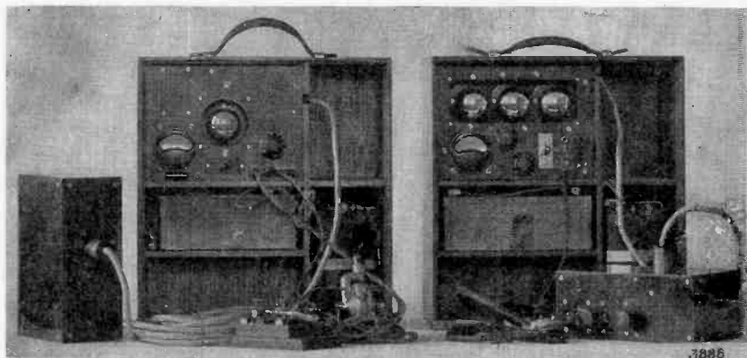
Fig. 5—Transmitter and receiver by C. Lorenz, 3-m wavelength.
