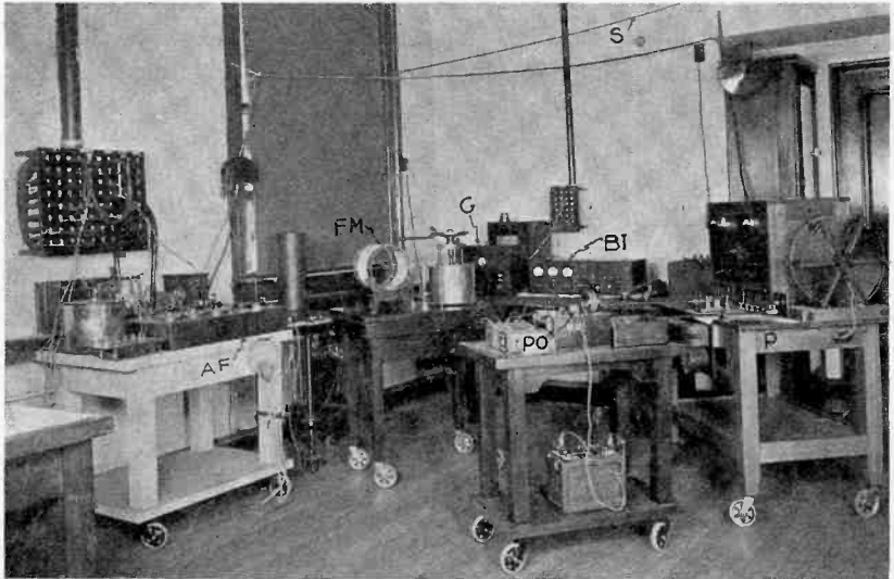
Fig. 7—Photograph of apparatus used in testing piezo oscillators:— S —wires leading from 200-kc standard G —10-kc generator BI —special beat indicator P —radio-frequency generator PO —piezo oscillator under test FM —frequency meter AF —audio-frequency generator
