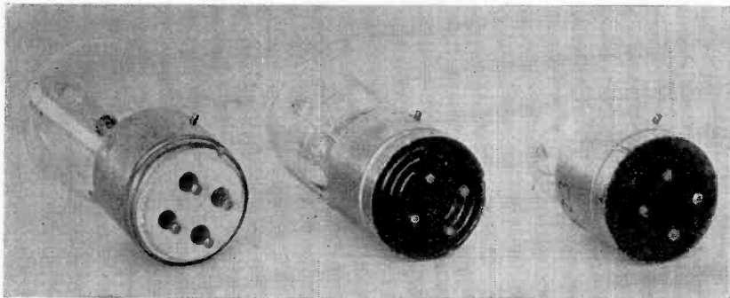
Fig. 3—Signal Corps tubes of war period. From left to right: General Electric, Western Electric, and de Forest.
