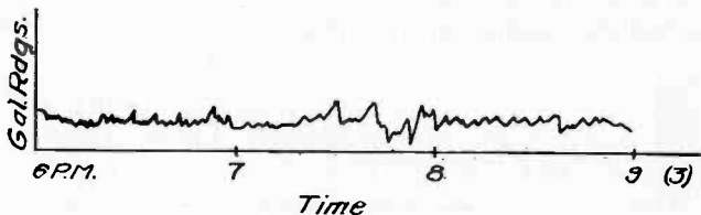
Fig. 3—Tuesday, October 9, 1928. Intensity constant after darkness sets in. No change in weather conditions.
