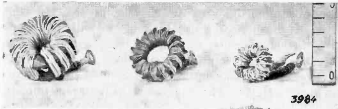
Fig. 2—Frequency transformer of the first, second, and third amplification stage (from left to right).
