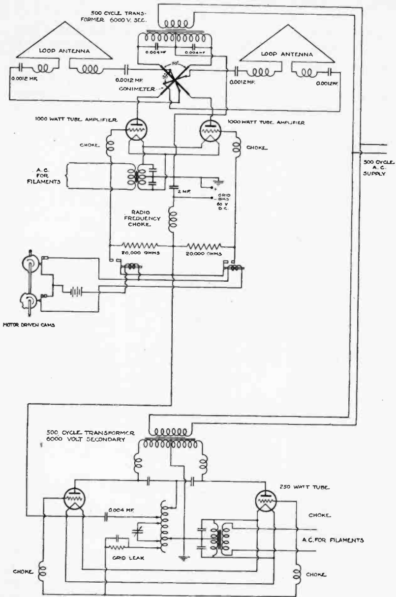
Fig. 4.—Improved Directive Beacon Circuit Diagram Showing Connections of Interlocking Mechanism.
