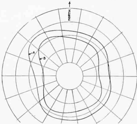
FIELD PATTERN COMPARISON VERTICAL & FLAT TOP ANTENNAS PATTERN A- VERTICAL ANTENNA 240 FT. LG. PATTERN B- "T" ANTENNA. HORIZONTAL LENGTH 240 FT. VERTICAL LENGTH 80 FT.
