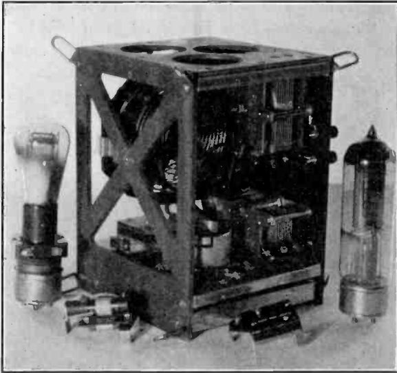
Fig. 29—Rear View of Byrd's High-Frequency Transmitter.
