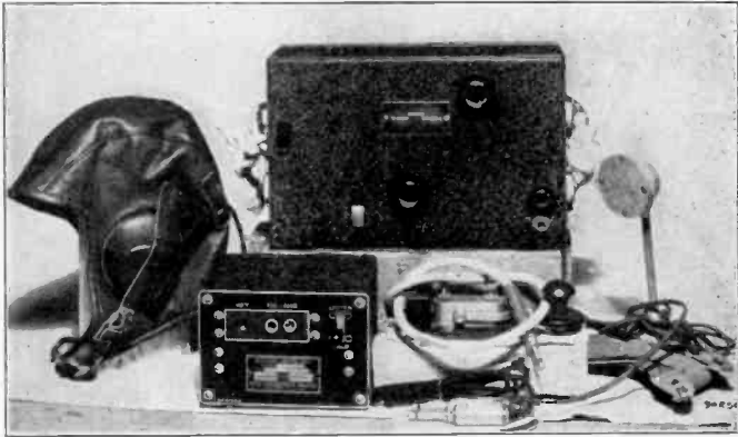
Fig. 46—300-Watt R.C.A. Equipment, Model ET-3654, Showing Receiver and Auxiliaries.
