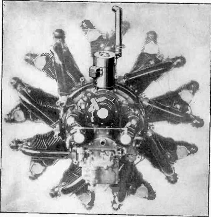
Fig. 11—Leece-Neville Generator Geared to Pratt and Whitney "Wasp" Engine.
