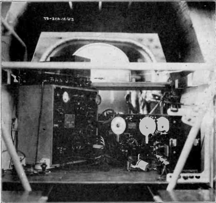
Fig. 40—Radio Installation in DT-2 Torpedo Plane.
