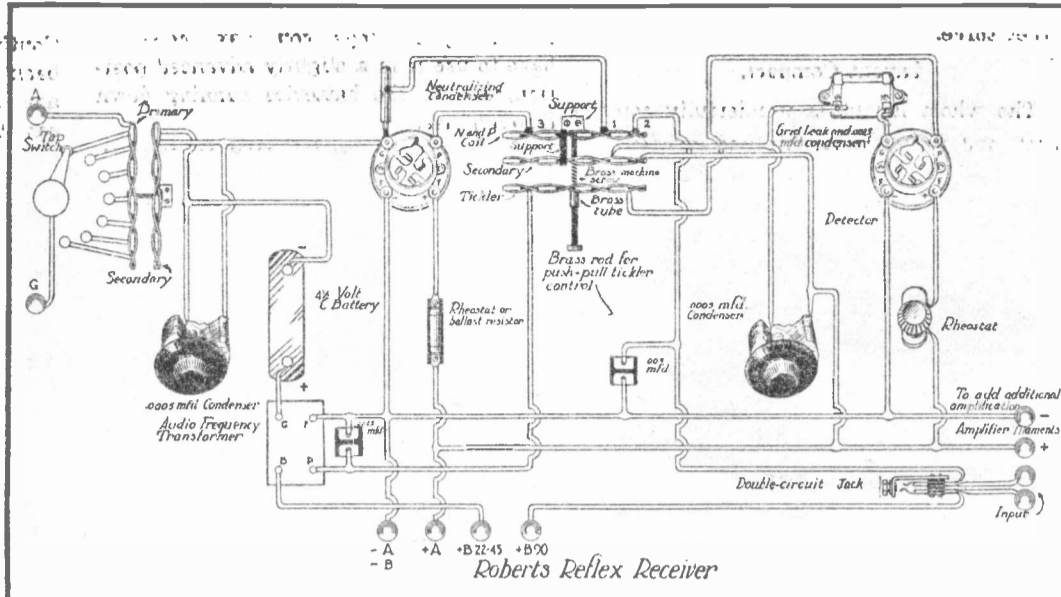
A SIMPLY CONSTRUCTED SET TO WHICH AMPLIFICATION MAY BE ADDED
