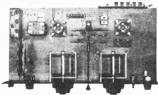
LOCATION OF INSTRUMENTS IN ROBERTS REFLEX RECEIVER
