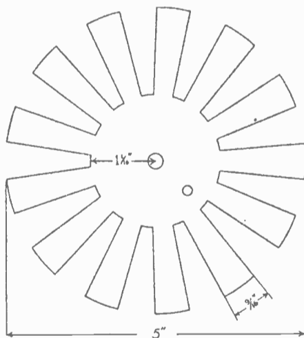
A MODEL FORM FOR ROBERTS COILS
