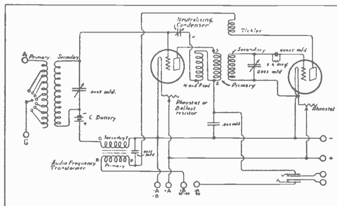
HOOK-UP OF THE ROBERTS REFLEX RECEIVER
