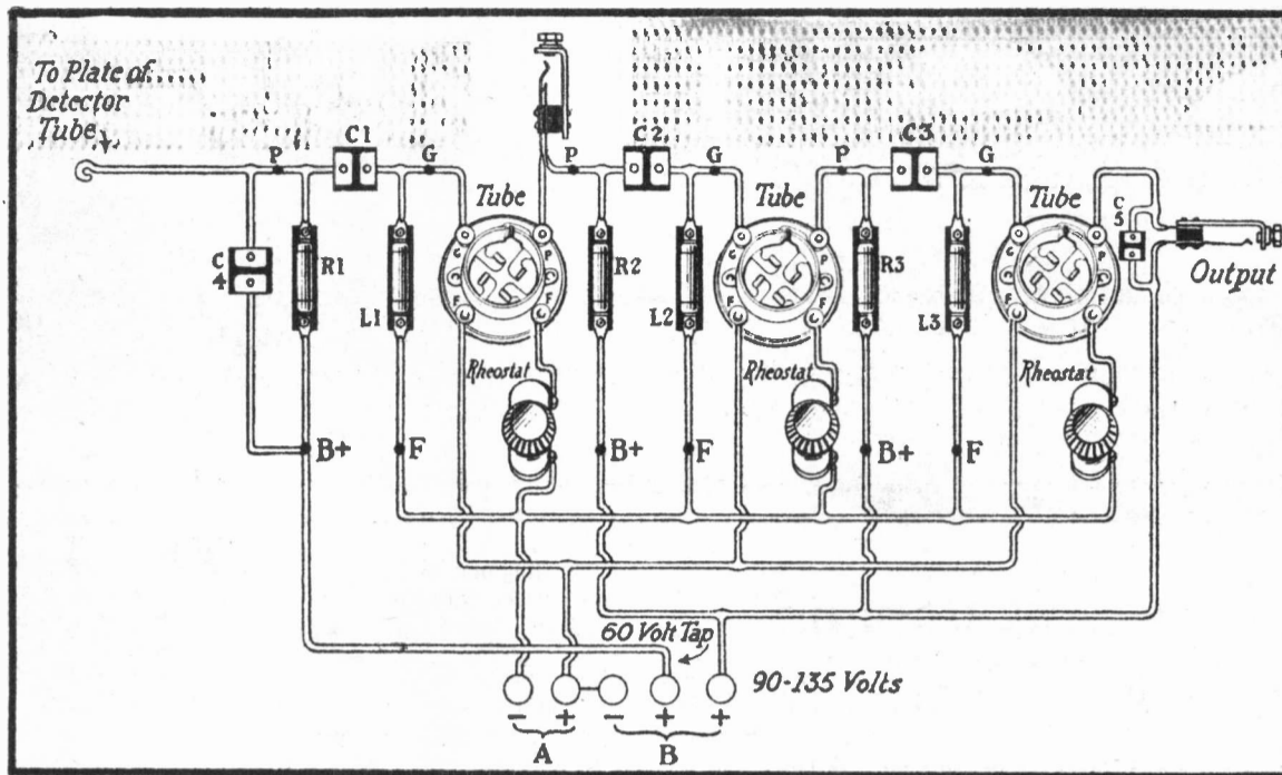
A PICTURE DIAGRAM SHOWING THE CONNECTIONS FOR A RESISTANCE-COUPLED AMPLIFIER
