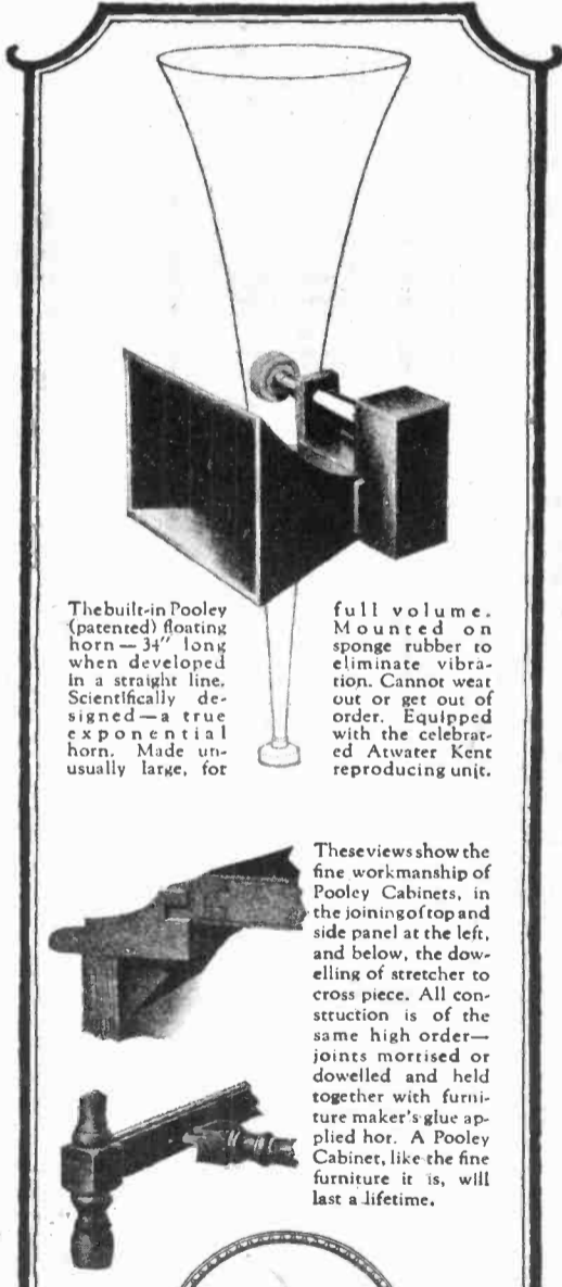
Model 1700-R-2 Finished in American Walnut or English Brown Mahogany, with built-in Pooley (patented) Floating Horn and Atwater Kent Receiving Set. Prices complete, without tubes and batteries. $240 to $320
