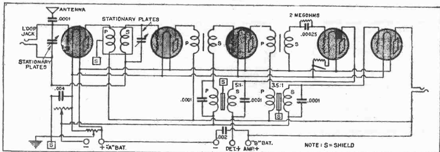
Complete circuit diagram of the five-tube De Forest reflex receiver with three stages of tuned radio frequency, detector, one stage of reflexed A. F. and one stage of straight A. F.
