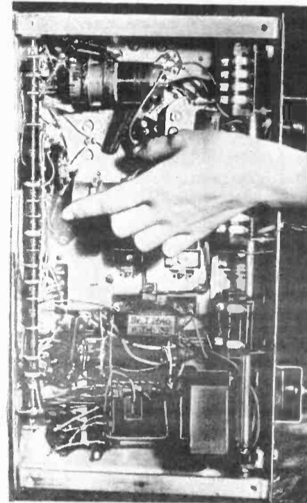
Under-chassis view of the receiver.
