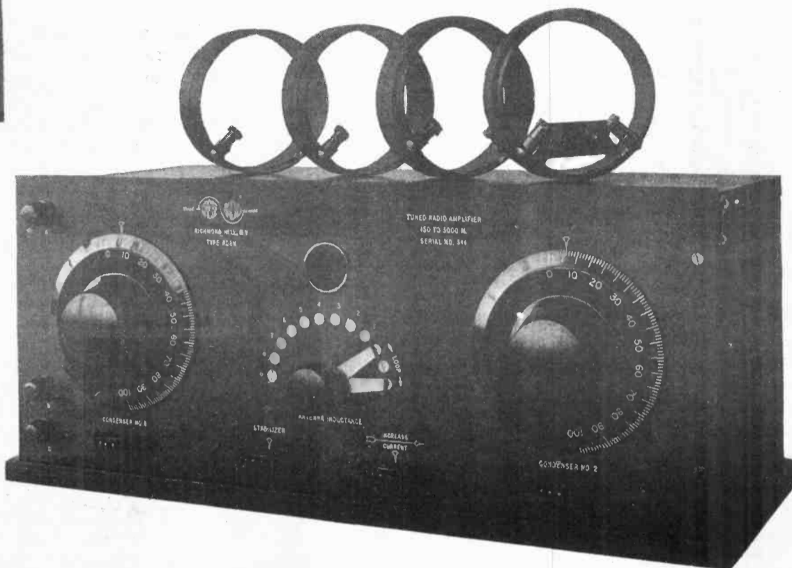
A SINGLE STAGE OF TUNED RADIO-FREQUENCY AMPLIFICATION Is provided in this amplifier, which may be applied to any form of receiver without making special connections. Four output coils, giving a wavelength range of from 150-3000 meters, form the coupling between the radio-frequency amplifier and the receiver proper. The price of this unit and the coils is $60.
