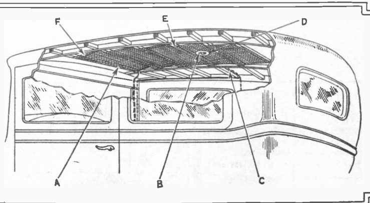
At the left is shown a typical car installation and at the right is shown a typical car antenna. At A are shown stagger tacks to permit listings on head lining, to be tacked over screen; at B, dome-light; at C, dome-light wiring; at D, a hole which is cut to clear the dome-light—the edges of the screen are soldered; at E, the antenna screen—use bright copper or bronze wire only; at F, edges of screen—they must be soldered.
