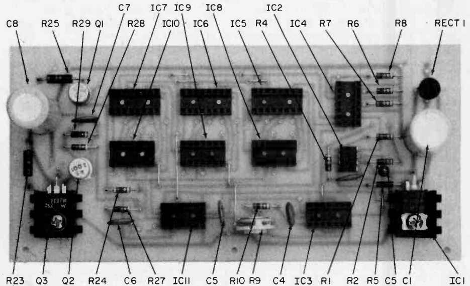
A neat, clean, professional printed circuit board can be made using the free template available from e/e. To obtain one, send a stamped, self-addressed envelope to: Rhythm & Blues Box, ELEMENTARY ELECTRONICS, 380 Lexington Ave., N.Y., NY 10017.
