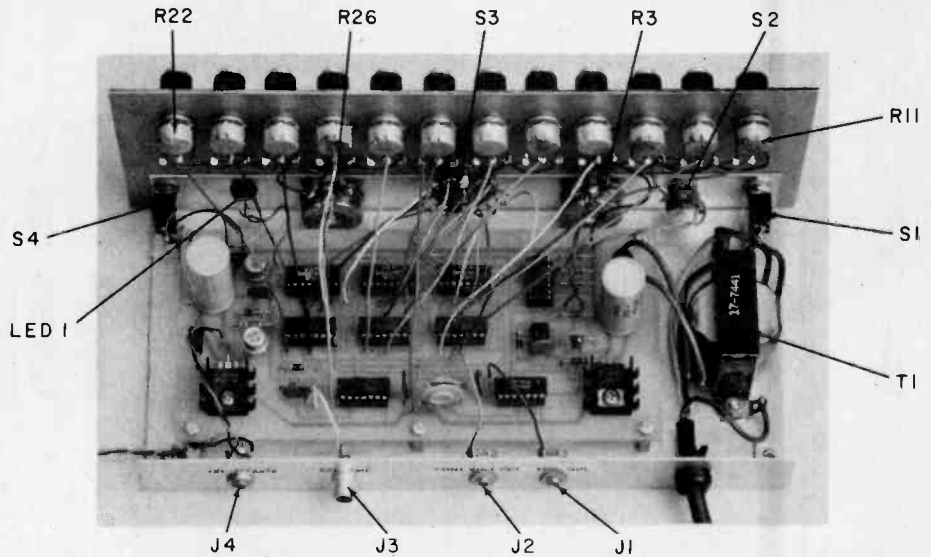
With the cover removed, the placement of all components can be observed. When wiring the front panel pots, it's a good idea to tag the wires from the PC board for identification. For more work room, install only every other pot at first, wire, then install the rest.
