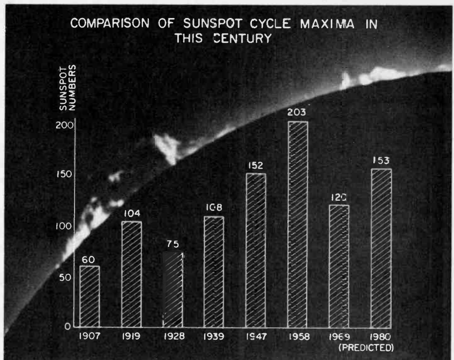
The amount of sunspot activity appears to be increasing according to this chart. The peaks occur at about 11-year intervals but this varies enough to be statistically significant.
