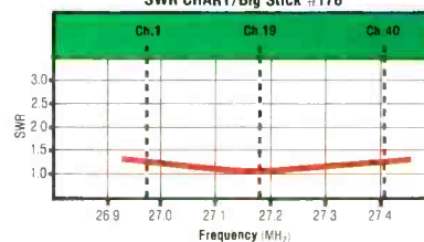
SWR CHART/Big Stick #176
