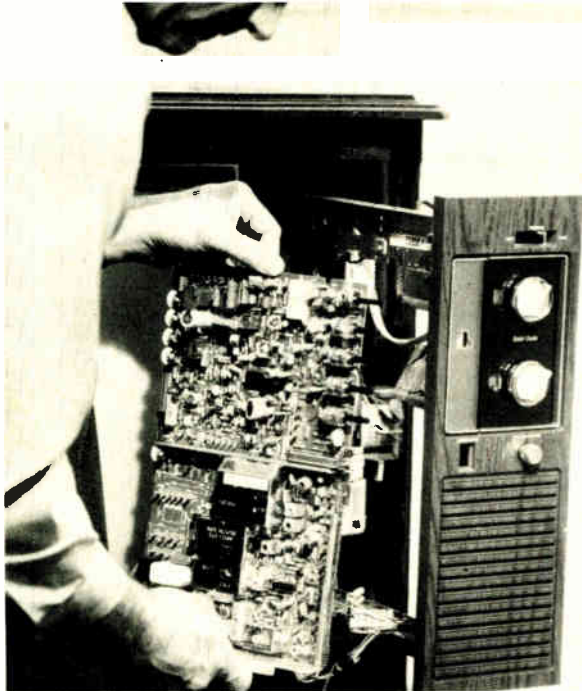
10. The works, the drawer. Quasar's new Super Module contains about 75% of the circuitry for the receiver on one board and can be replaced completely by the serviceman in the field or repaired. The new "works in the drawer" also reduces component count.
