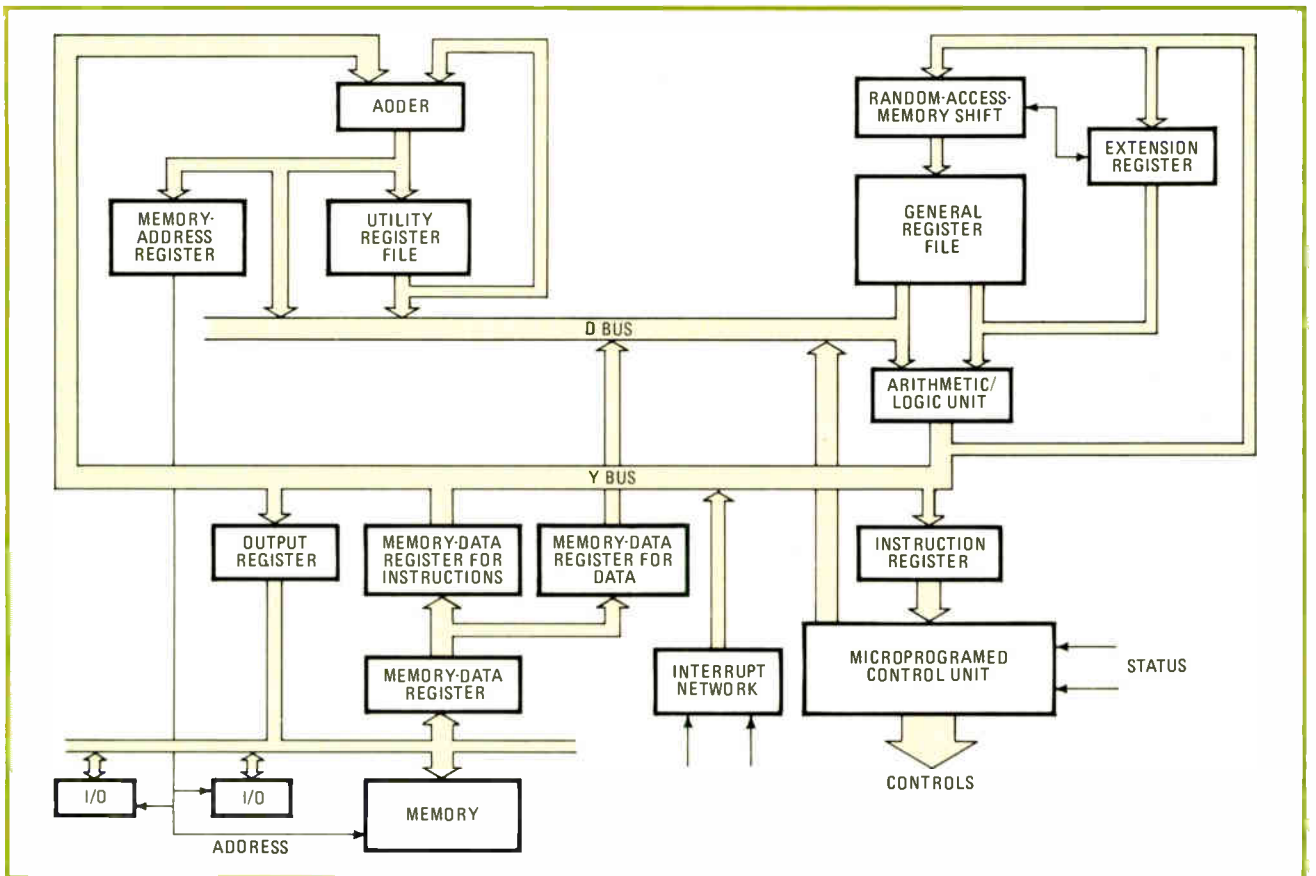
6. The computer. In the single-board ATAC-16M minicomputer, the memory and input/output devices communicate asynchronously with the CPU through a buffered port. Address formation logic, two working registers, and the program counter use Fairchild Macrologic parts.
