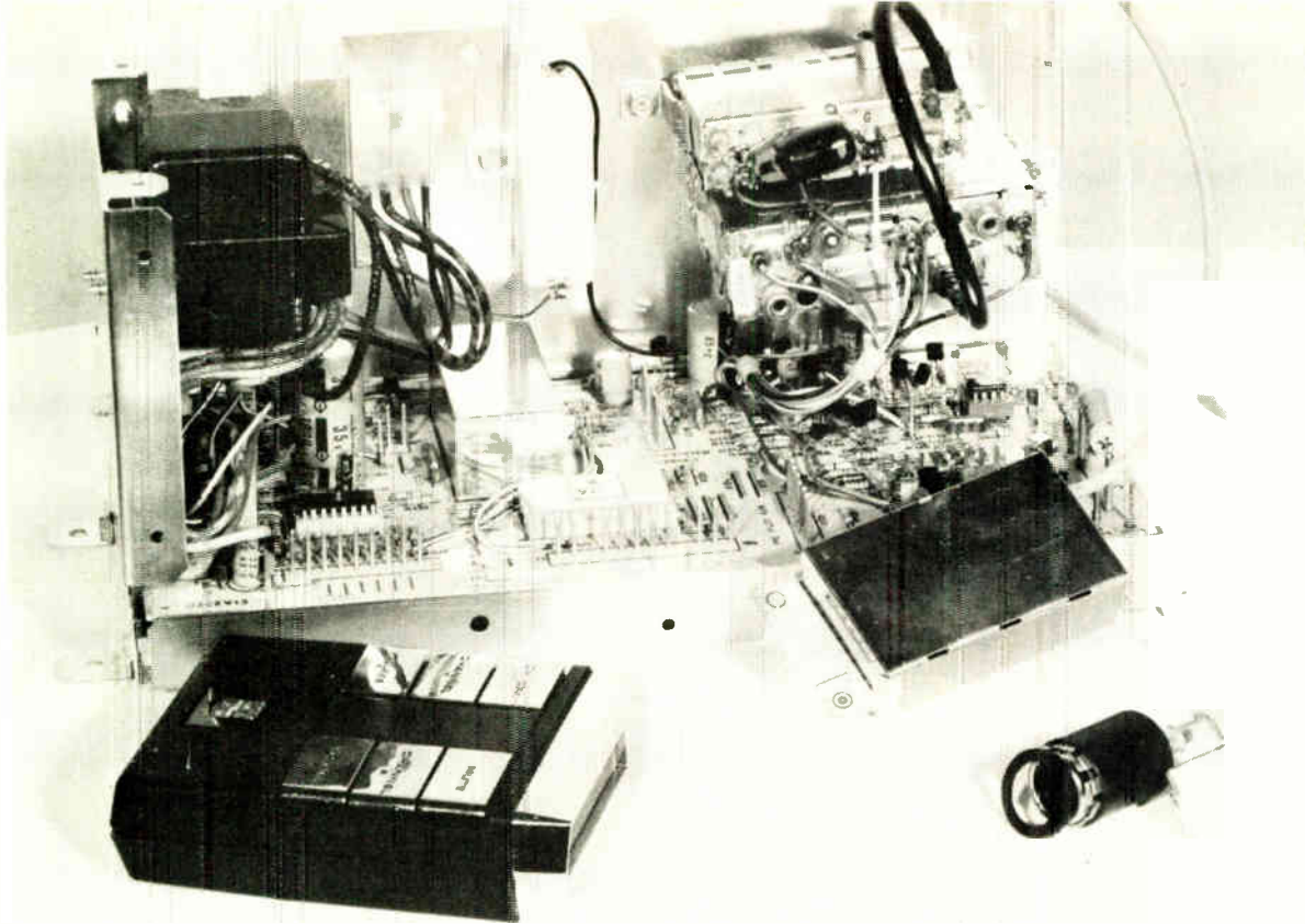
1. Remote afterthought. This new Magnavox tuner features a field-installable remote-control unit. An interface circuit and ultrasound mike (lower right) are put in through the back of the set to handle signals from the hand-held transmitter.
