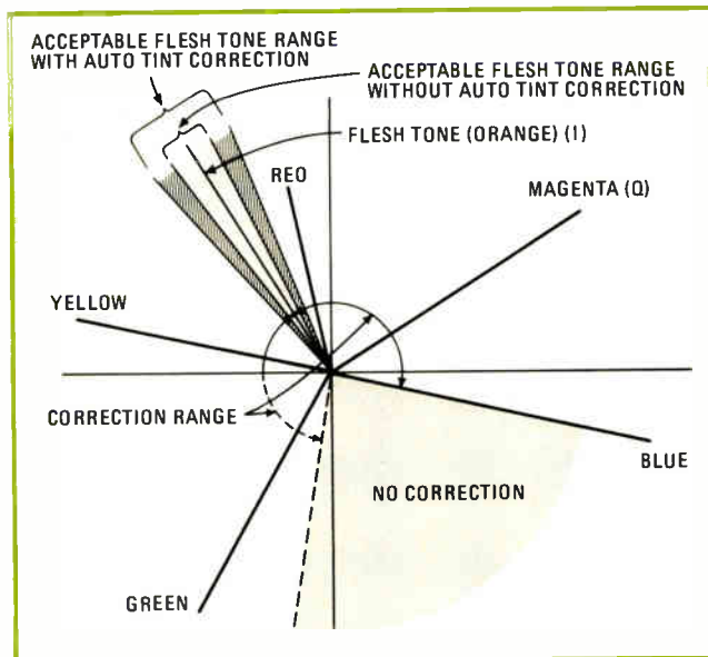
6. Tinting. The RCA automatic phase-correction tint control operates within a wider range of colors than usual flesh-tone correctors. However, the tradeoff in this approach is that the correction circuit alters almost all of the color spectrum except blue.
