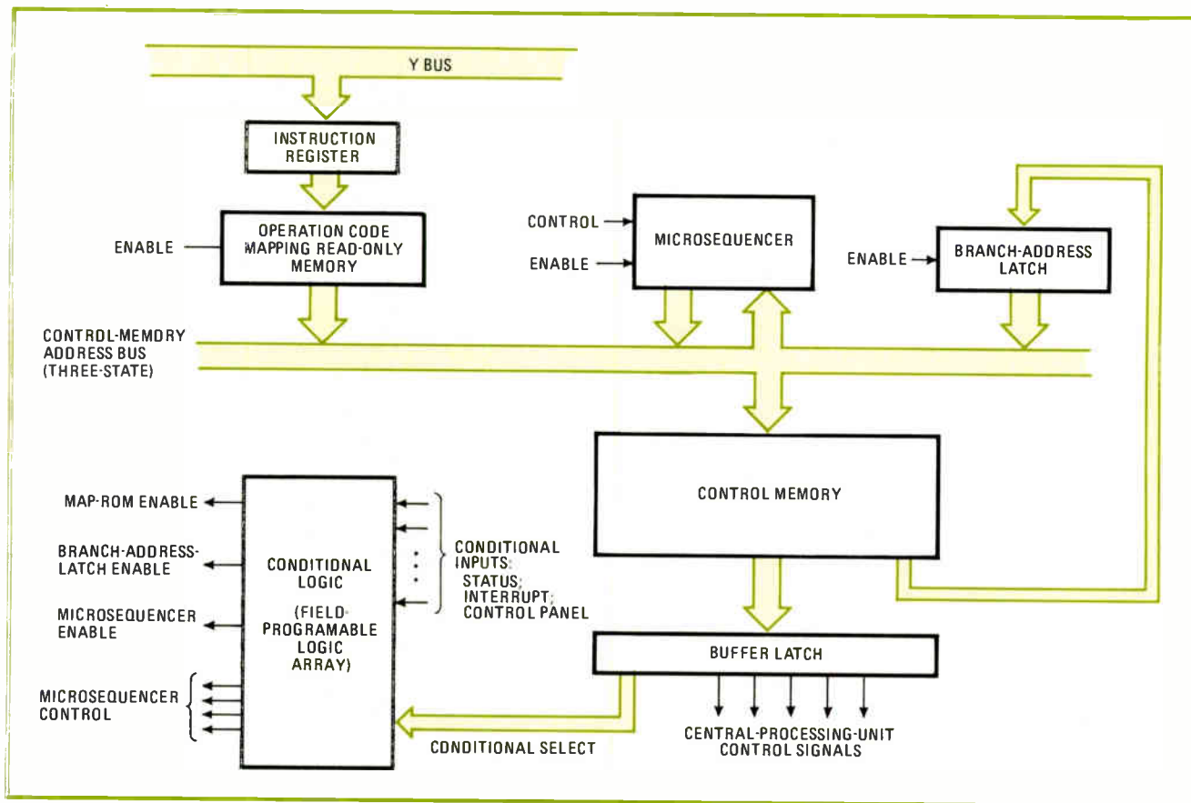
2. Control. Microprogram control was achieved with the AM2911 sequencer, a field-programmable logic array, and nine 4-k bipolar PROMs. During each microcycle, the PLA selects the sources of the next address, based on the condition-select field.
