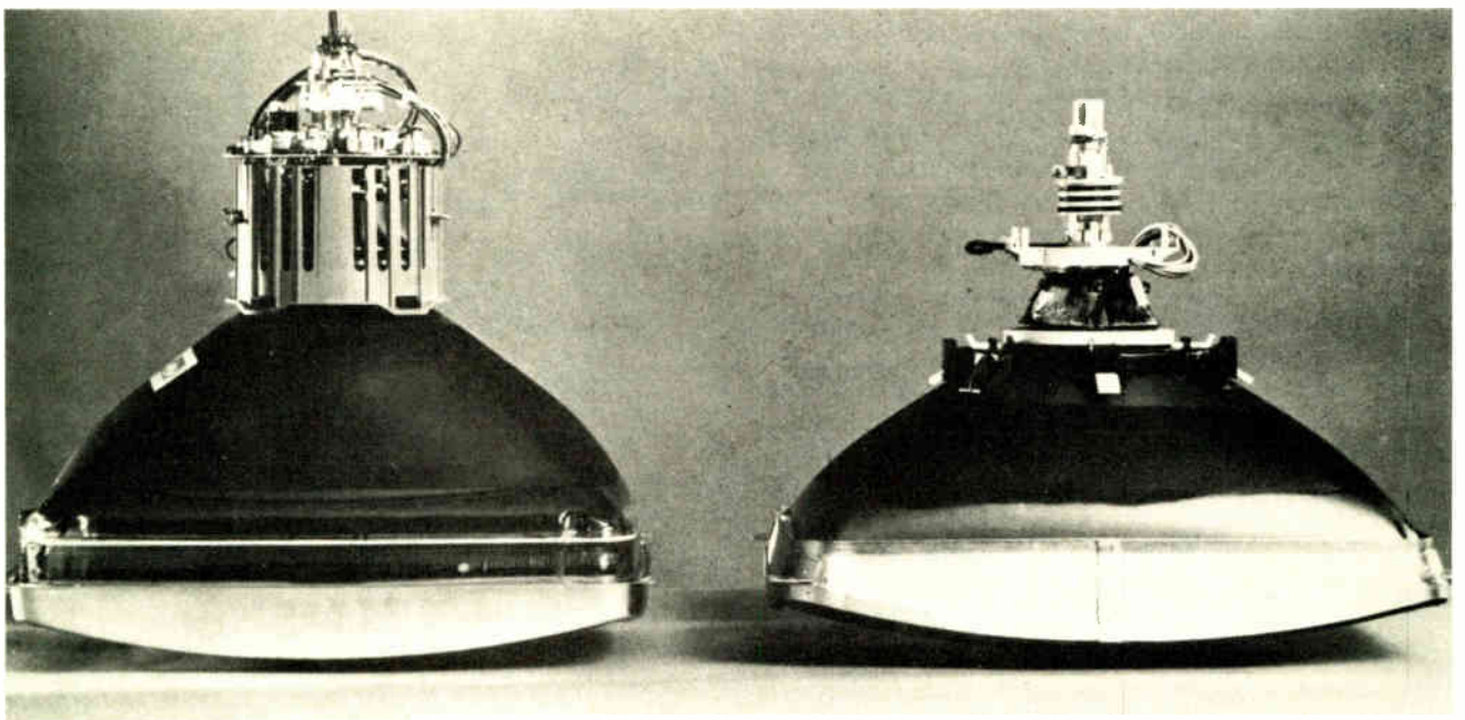
8. New tube. Zenith's Ellipse II 19-inch receiver (left) features the new Able picture tube. With its tripotential, extended-field-lens, in-line gun, the 100° deflection tube at the right below is 2½-in. shorter than present delta-gun, 90°-deflection, 19-in. models at the left.
