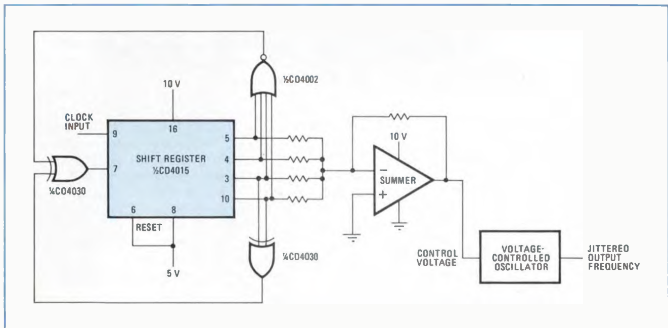
2. Random oscillator. Output voltages from individual stages of shift register are summed and used to determine output frequency from VCO. Feedback arrangement in shift register makes summed voltages vary among four levels in pseudorandom, repeating 15-step sequence. Four-input NOR gate suppresses all-zero condition in register after turn-on, so that exclusive-OR gates can generate sequence of voltage levels. Longer registers produce more levels, longer sequences, and a more nearly gaussian distribution.
