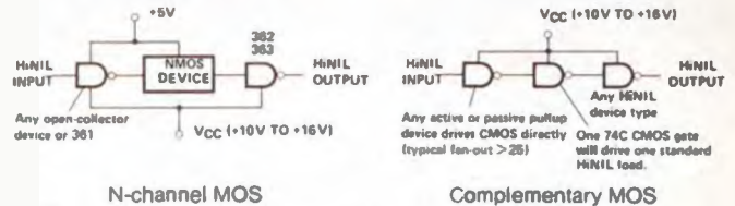
Figure 2. Typical HiNIL/MOS and HiNIL/CMOS interfaces
