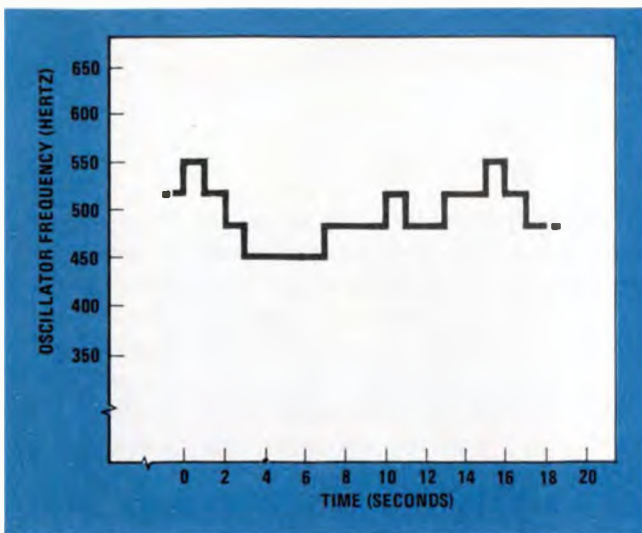
1. Frequency jitter. Pseudorandom jitter of frequency from voltage-controlled oscillator is generated by using the sum of the outputs from individual stages of a four-stage shift register to tune VCO. Oscillator's output frequency has more possible values, with more noise-like distribution, when more shift-register stages are used.
