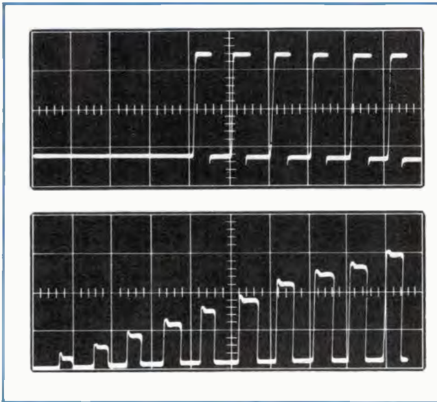
4(b). Linear. A 709 operational amplifier can act like a comparator. With sequential pulse inputs increasing in amplitude from -50 to +50 millivolts in 10\text{-mV} steps, the output level of this amplifier switches from 0 to 1 at an input of -10\text{ mV} .
