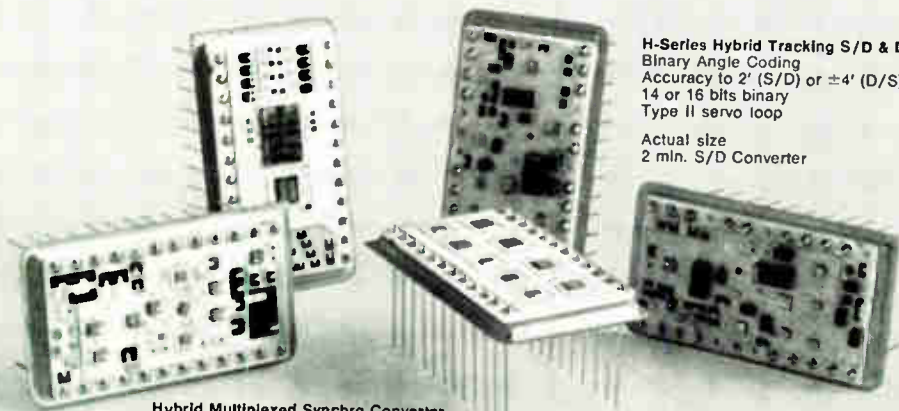
Hybrid Multiplexed Synchro Converter Binary Coding Accuracy to 5.3' Resolution 1.3' 150 \mu s conversion time (not shown)
