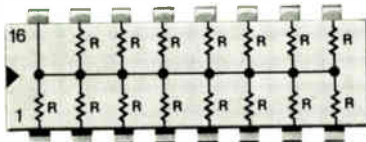
898-1 (15 resistors) Price (1,000-4,999) $1.85
