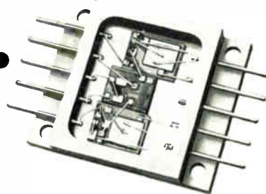
10 Lead Flat Pack (Just one of the many hybrid packages available from Solitron)
