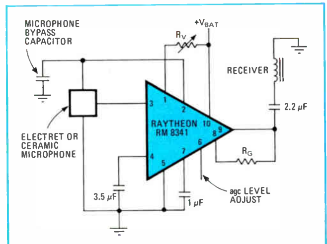
1. Complete amplifier. IC audio amplifier can operate from a single battery over a wide voltage range. Automatic gain control is implemented by the capacitor at pin 7; maximum gain is determined by resistor R_G . A standard volume control, R_V , can be used.
