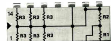
899-40 DIP network provides six line terminators and the threshold setting divider for the Intel 3208A sense amplifier. Price (1,000-4,999) $1.35
