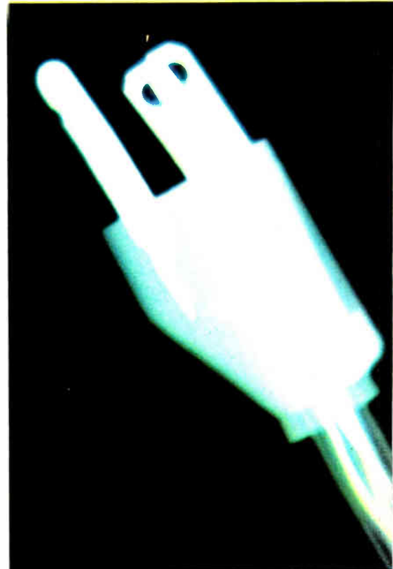
3. Poor ground. X-ray reveals broken ground wire in electrocardiograph's molded plug. Since this unsafe condition can't be detected visually, molded plugs shouldn't be used.
