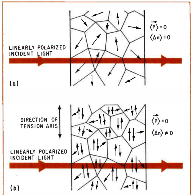
4. Straining. Strain-biased ceramic plate achieves 90° domain rotation without a transverse field. Randomly aligned domains (a) align in the direction of the tension axis (b).
