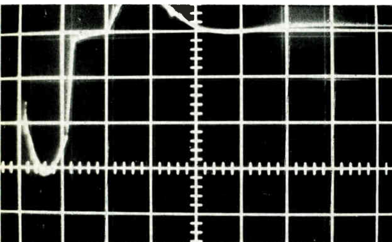
5. Changing output. Most defibrillators are designed to put out pulses like one in top photograph. However, as defibrillators age, waveshapes can change, and it's not uncommon to find older units delivering deformed pulses like two lower traces. Since such outputs can injure cardiac muscle, hospitals should periodically check defibrillators for output waveshape. But they can't. No manufacturer has developed an instrument that'll perform this test.
