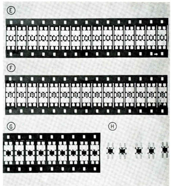
Step at a time. These are the steps involved in producing the Minimod package. Copper, A, and polyimide, B, are laminated, D, after punching the polyimide, C. Copper is photoetched and plated, E, chips are bonded, F, and then encapsulated, G, and sheared apart, H.
