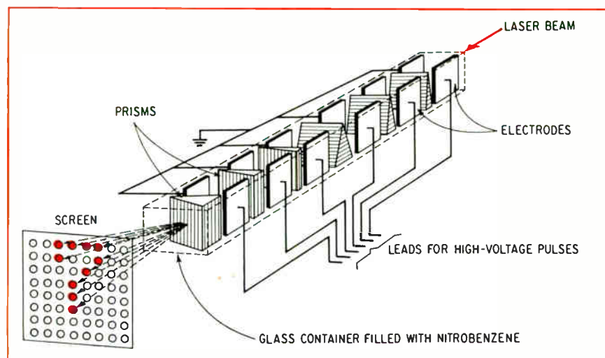
On the beam. Researchers at Philips Central Laboratory in West Germany set up a row of 20 Kerr cell/prism pairs to generate a 1,024-by-1,024 array.
