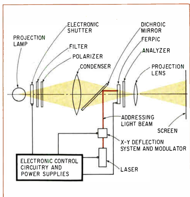
6. On display. System has reset, write, and view cycles. To write, laser scans the image, writing an element at a time. Projection lamp goes on for viewing.
