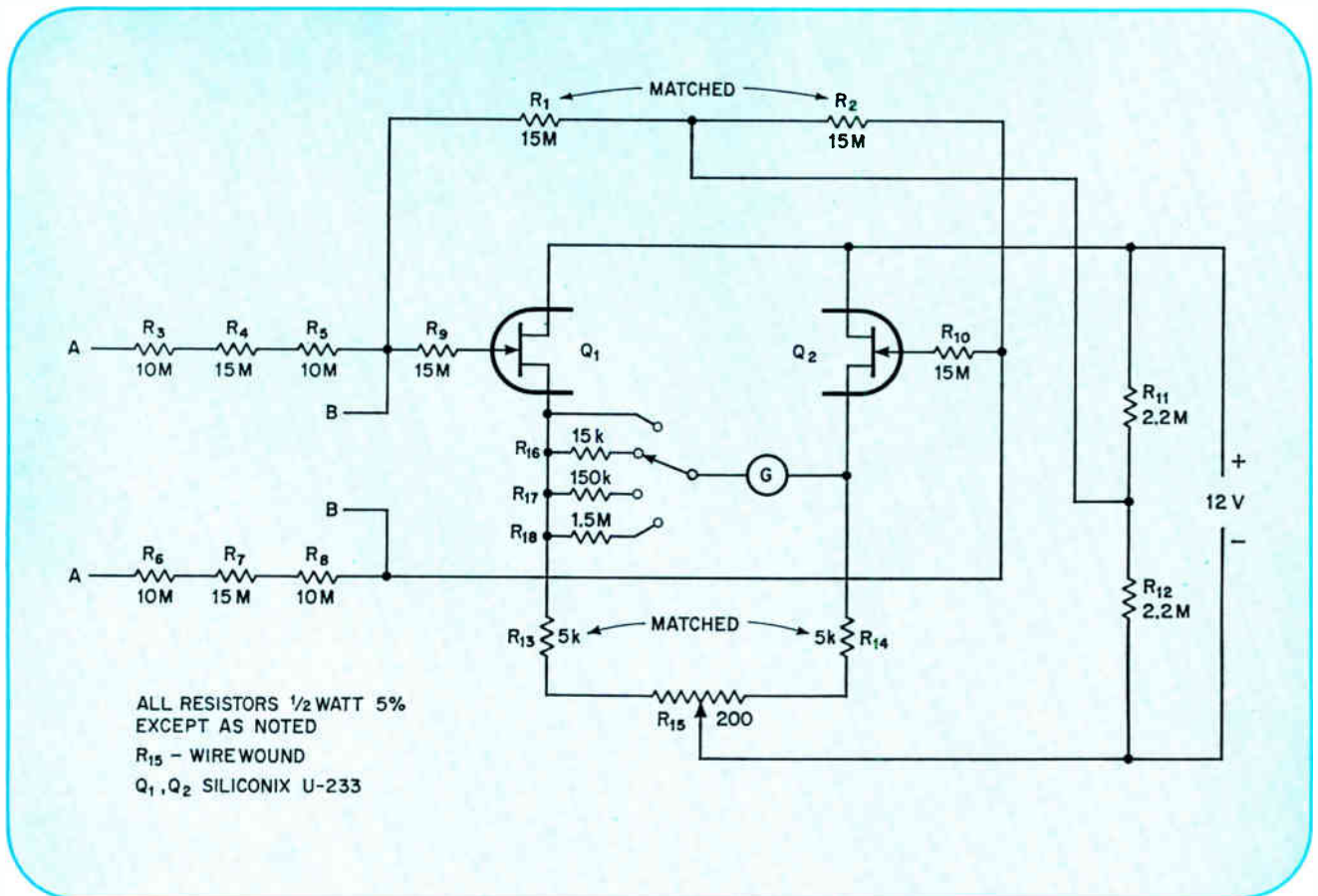
FET null detector. Transistors Q_1 and Q_2 improve the galvanometer's sensitivity when nulling a bridge with high-resistance values. Input resistance is raised to 100 megohms by resistors R_1 through R_8 . The transistors operate as a differential pair, biased with a dc supply. Switch ranges are 1 volt to 1 millivolt per meter division.
