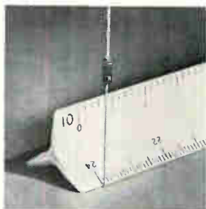
Temperature compensated zener reference units series 1N821-1N829 and 1N935-1N939 in DO-7 case provide stability and low noise. Applications include d-c voltage standards, d-c decade voltage reference sources, d-c voltmeters, X-Y strip recorders, and other applications requiring close temperature regulation. International Rectifier, 233 Kansas St., El Segundo, Calif. [437]
