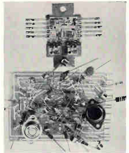
New and old. Hybrid module does job of discretes shown at bottom.
