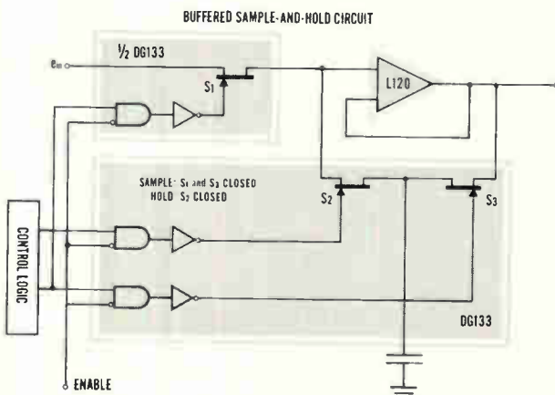
Low input leakage of the L120 OP AMP makes it ideally suited for sample-and-hold circuits. Two channels of this circuit require three DG133s and one L120. An alternative approach would require two DG129s and one L120 for two channels.
