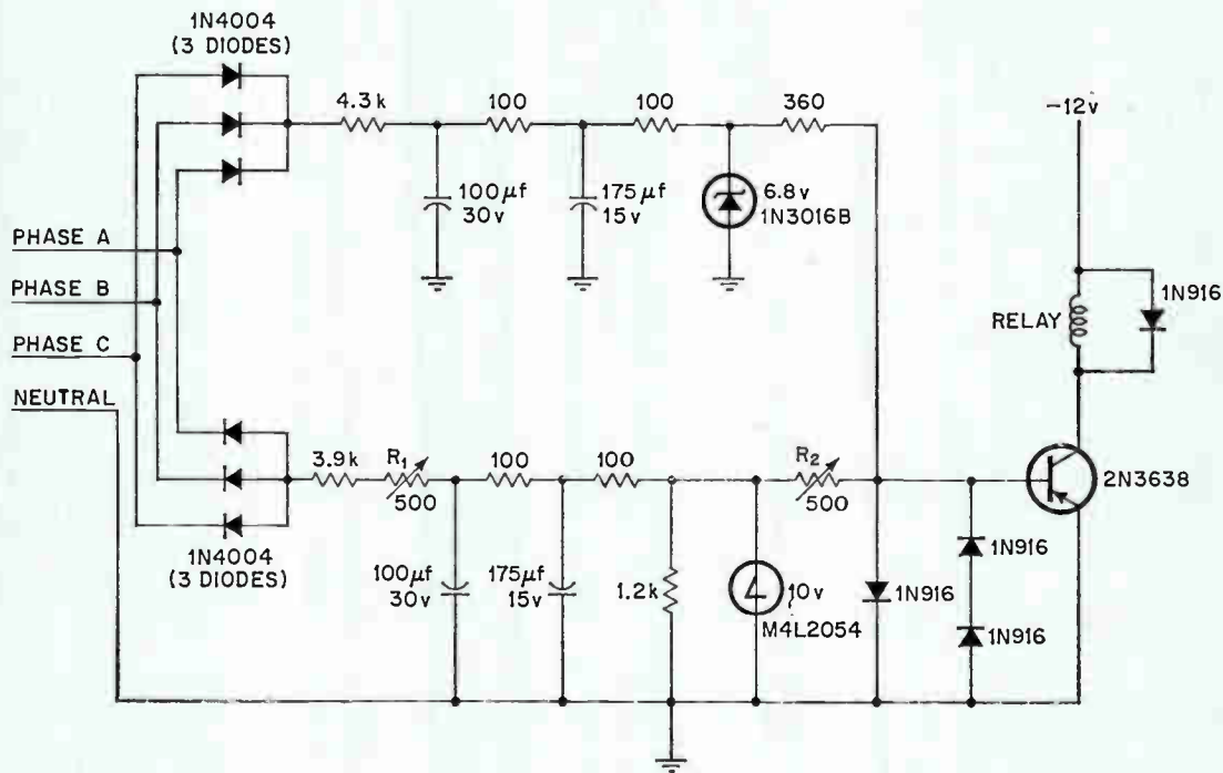
Protection. The positive output of the regulated supply (above) is summed with the negative voltage from the unregulated supply (below) at the transistor's base junction. Overvoltages or phase loss apply a net positive voltage to the transistor's base to open the control relay.
