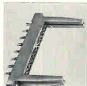
Card-edge connector 6030, available with 15 single-readout or 30 dual-readout contacts, offers a choice of terminations that includes solder (wire hole or p-c tab), taper tab, and low-cost wire wrap post. Current rating is 5 amps, with a contact resistance of 6 milliohms. Insulation resistance exceeds 25,000 megohms. Elco Corp., 155 Commerce Dr., Fort Washington, Pa. [344]
