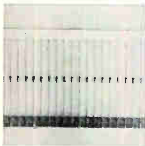
Silicon stabistors come in single (AP103), double (AP203) or triple (AP303) types. Chips are available in a 400 mw whiskerless package. Stabistors are used where controlled forward voltages are necessary such as voltage regulator circuits, sensing, and computer circuitry. Forward voltages are from 0.86 to 2.6 v at 100 ma. American Power Devices Inc., Andover, Mass. [440]
