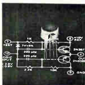
Hybrid IC ladder switches CDA4 are for direct-from-logic operation in digital-to-analog conversion. The CDA4 is meant for use with a +10-v reference. When used in conjunction with a 10K/20K ladder network, the switch provides 12-bit accuracy. Settling times under 1 μsec allow high speed operation. Price (1-99) is $38 each. Crystalonics, 147 Sherman St., Cambridge, Mass. [441]
