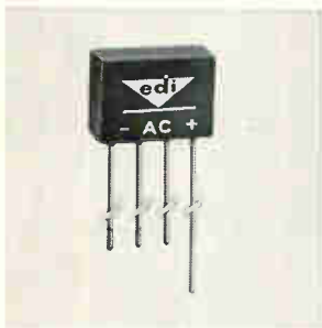
Miniature silicon rectifier bridges have piv ratings of 1,000, 1,500 and 2,000 v. Applications include voltage regulators, spark ignition systems, microwave tube and laser supplies, pocket scopes and electrostatic supplies. Dimensions are 0.625 x 0.468 x 0.25 in. A transfer molded case insures void free encapsulation. Electronic Devices Inc., 21 Gray Oaks Ave., Yonkers, N.Y. [436]
