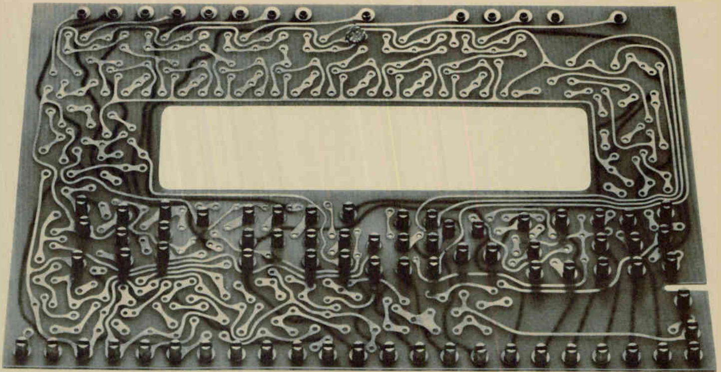
Circuit boards for lunar module required extremely tight specs in a small production run.
