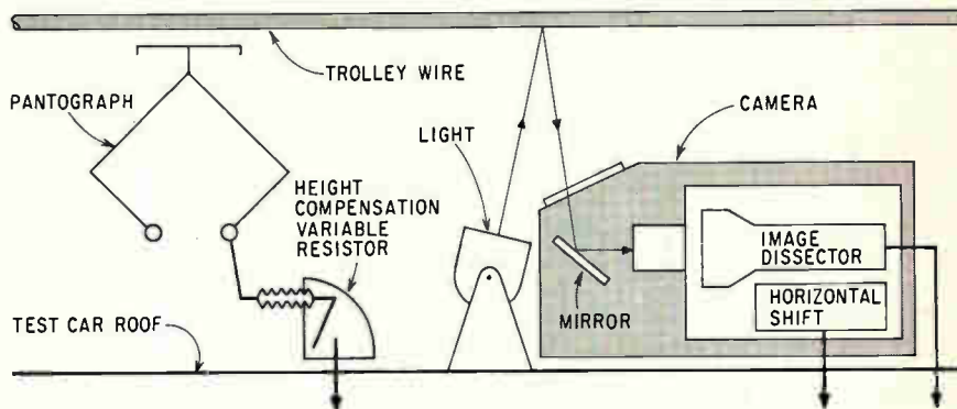
Midnight special. One night a week, test car zips down Tokaido line tracks at 125 mph while image-dissection tv camera checks overhead electrical wire wear.
