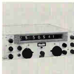
H-f receiver model RA6218 features an electronic counter with a 7-digit display, locked to a built-in high stability crystal frequency source, enabling the operator to read the receiver tuned frequency to within 10 hz. Frequency range is 1 to 30 Mhz. The unit measures 5\frac{1}{4} x 19 x 17\frac{1}{2} in. Racial Communications Inc., 8440 Second Ave., Silver Spring, Md. [387]
