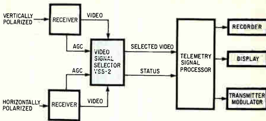
Pick 'em. Dynalex's VSS-2 compares AGC voltage from the receivers. The video signal with the higher voltage is switched to telemetry signal processor in 500 nanoseconds, averting loss of data frames. DEI 1074 receivers were used in Navy evaluation tests.
