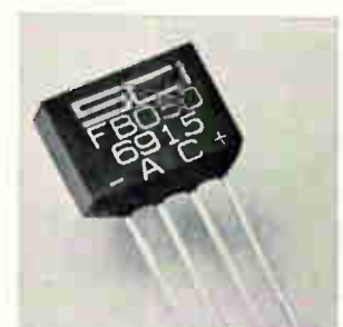
Full-wave bridge rectifiers FB are fabricated with double diffused silicon rectifier cells. Unit is encased in plastic with an in-line configuration easily adaptable to p-c board mounting. Units are rated for a maximum output current of 2 amps and peak in-verses voltages of up to 1,000 v per element. Scientific Components Inc., 350 Hurst St., Linden, N.J. [443]
