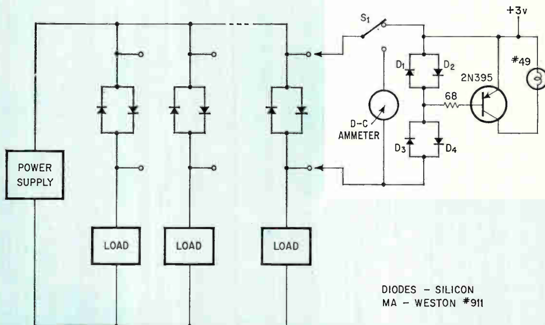
Fault finding. Parallel diodes connected in a front-to-back arrangement along with the current measuring circuit at the right, provide a means of reading load current without breaking the circuit. In addition, if the conducting diodes in series with the load circuit are faulty, a warning lamp lights.
