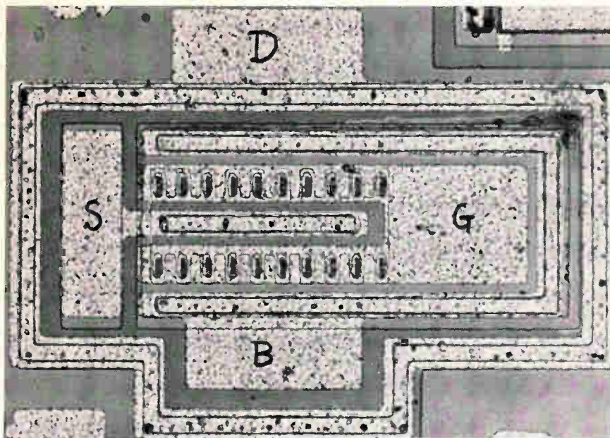
Diffused MOS. Non-planar geometry of microwave-frequency FET is one of two used by Japanese team to make transistor by bipolar-type diffusion. The rows of vertical slots are gate moats etched through the source, base and drain depletion layers, then covered with oxide and metal.
