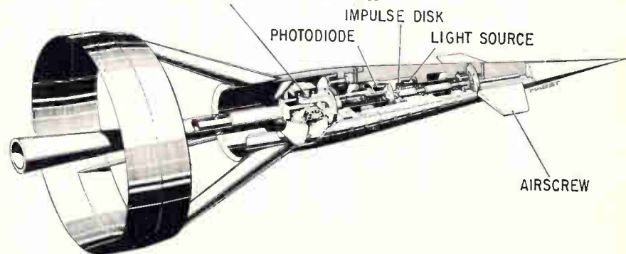
Out in front. Mounted on a boom extended ahead of an airplane, the Airlog is free to swivel. Potentiometers and airscrews deliver in-flight data.
