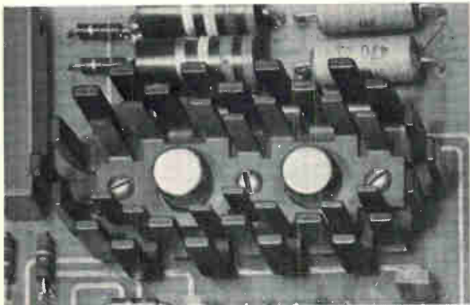
Thermal mating of matched transistors, such as these TO5's shown on a dual LP, maintains matched operating characteristics. The LP's unique multiple staggered-finger design (both single and dual models) maximizes radiation and convection cooling, results in a high efficiency-to-weight and -volume ratio.
