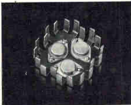
High power TO3's, TO66's, TO6's, TO15's, etc. can be operated with much more power when used with HP's. These compact, light-weight staggered finger devices accommodate from one to four TO3's. Provide the same heat dissipation as an extrusion that's three times heavier and one-third larger.
