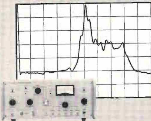
Power spectral density of bat cry transformed from autocorrelation function by Model 102 Fourier Analyzer (Price: $2,950.)
