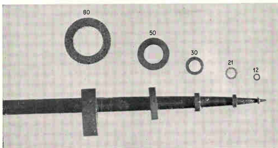
Sized for speed. Five common ferrite core sizes have been in use in computers. Each was smaller than the one before, and made it obsolete, because the new size could switch faster. Numbers show the outside diameter of the cores are in mils; the lower line-up shows them mounted on the tip of a sewing needle.
