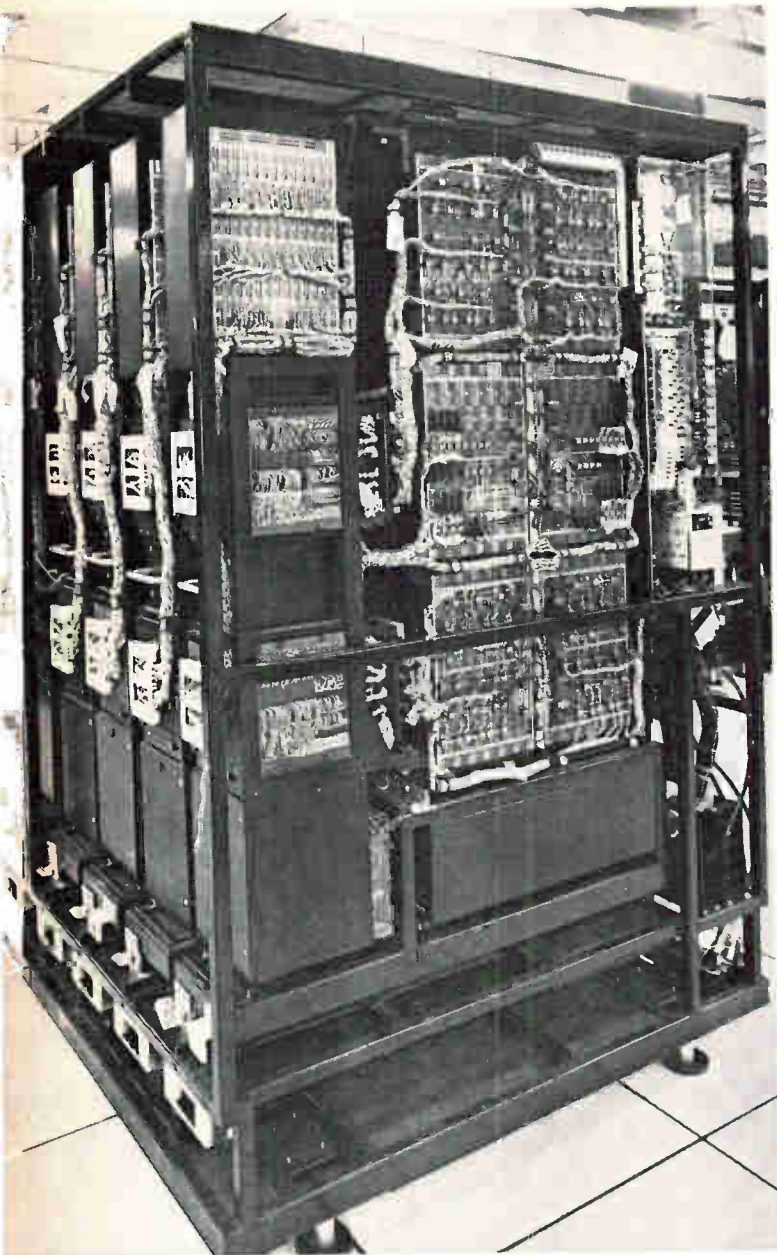
Mouthful. This frame stores one million bytes of data or instructions; any group of 16 bytes is accessible in 960 nanoseconds. It's part of the main memory for the IBM 360/85.
