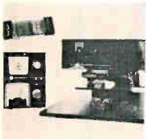
Flat flexible cable soldering systems series FS joins soldered connections rapidly and reliably using focused infrared heating techniques. Entire rows or groups of joints are soldered simultaneously and the heater never touches the workpiece. A complete row of terminations, as many as 200 joints, require less than 5 sec to complete. Argus Engineering Co., Hopewell, N.J. [425]
