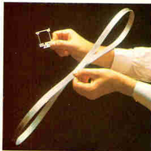
Small and light. Desktop-size printer swings open in front for loading convenience. Font belt, shown above with one of the print hammers, takes the place of chains and drums used in many printers.
