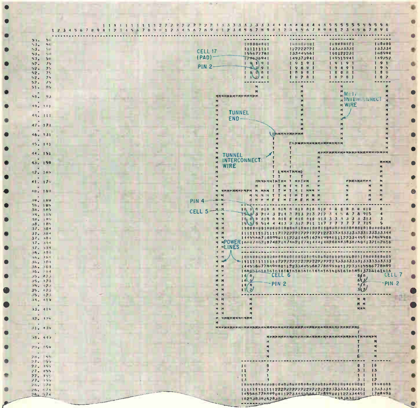
Coded layout. A line printer delivers a plot of the chip layout, with metalization coding paths, device cells, and bonding pads coded alphanumericly. This is one portion of the dual 32-bit serial accumulator developed by Collins.
