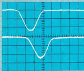
Fast pulse input and output signals: Hor: 10ns/div Vert: 5mv/cm
