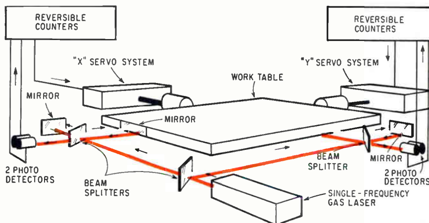
Light beams, shown in color, are the measuring elements in a laser interferometer that servopositions IC master plates with high accuracy.
