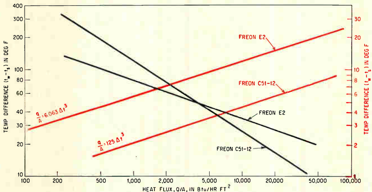
Heat transfer rates of IC's in two types of Freon. Curves and temperature scale in color represent solutions to equations for nucleate boiling and those in black for partial nucleate boiling.
