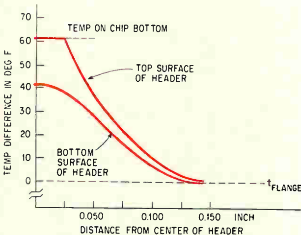
Thermal profiles at the top and bottom of a typical header. Heat flows from chip toward the flange.
