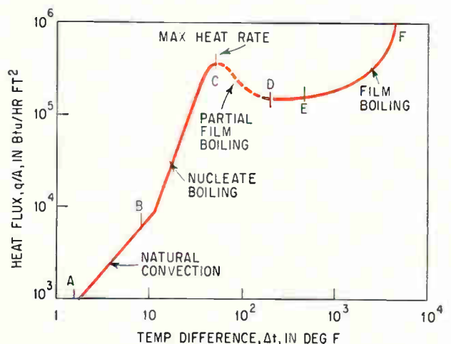
Boiling curve indicates relationship between heat flux and difference between temperatures of heat source and liquid. Heat is removed rapidly from heat source until at point C vapor film forms and impedes heat transfer.
