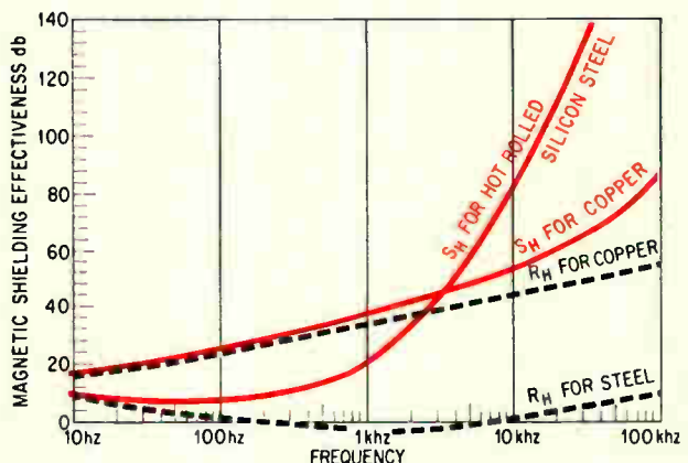
Magnetic shielding is plotted for copper and hot rolled silicon steel 15 inches from source of interference. Broken lines are reflection losses; solid lines in color plot sum of absorption and reflection losses.
