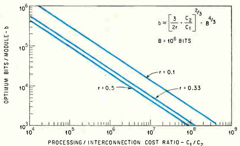
Optimum bit capacity varies with processing-interconnection cost ratio and a confidence parameter, r , related to memory plane production.
