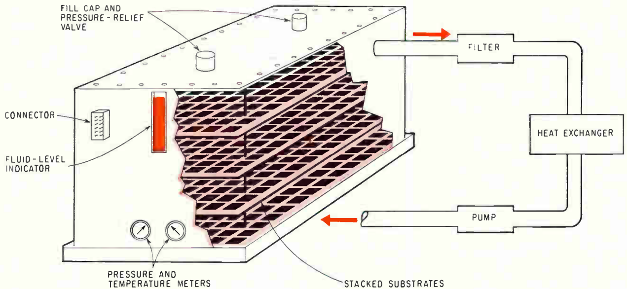
Integrated-circuit chips or packages could be put close together on substrates stacked in liquid-cooling housing. In some applications, external heat exchanger could be replaced by cooling fins on the housing.
