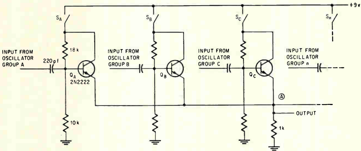
Conducting transistor associated with an oscillator group back-biases the other transistors, isolating group outputs.
