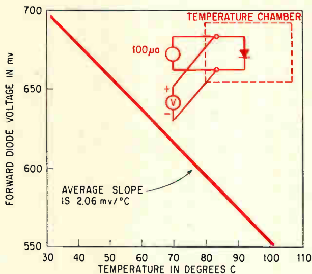
Temperature of IC's is monitored by measuring diode voltage. This calibration curve was obtained with the test setup shown in color.
