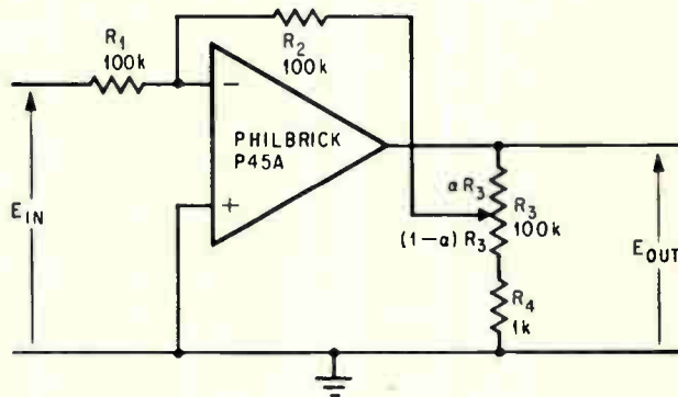
T-network that includes 10-turn potentiometer provides wide gain-adjustment range.
