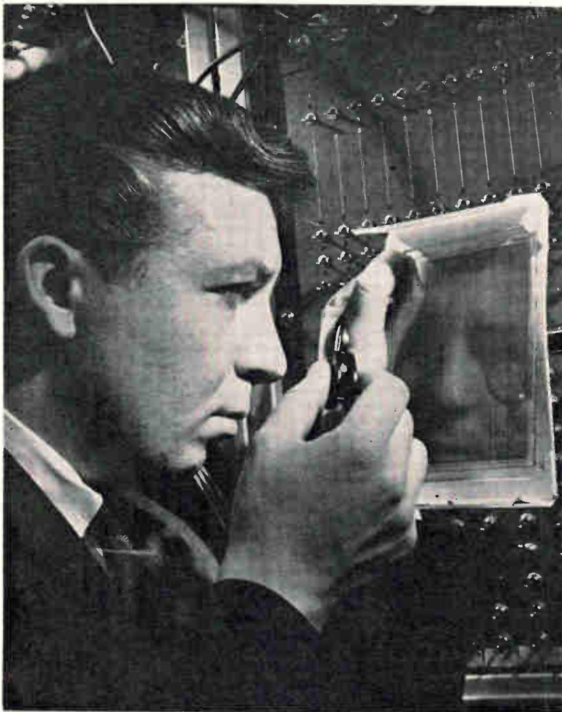
Author Gange examines a 250,000 bit cryoelectric memory plane arranged in 64 modules of 4,096 bits each. Studies indicate that it is feasible to build a 10^8 bit memory using 512 of these planes operating in a coincident-current, random-access mode and with microsecond cycle times. Successful operation has already been obtained with smaller, 6,000-bit planes operating in a 14,000-bit cryoelectric memory. The planes are arranged in stacks and operated at liquid helium temperature, 3.5^\circ\text{K} .
