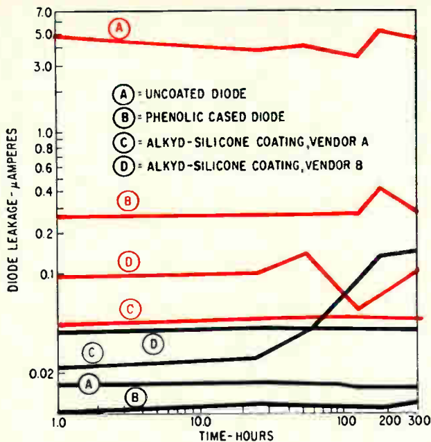
Leakage currents of microdiodes react under exposure to dry ammonia (curves in color). The curves in black represent the same devices in a dry nitrogen atmosphere.
