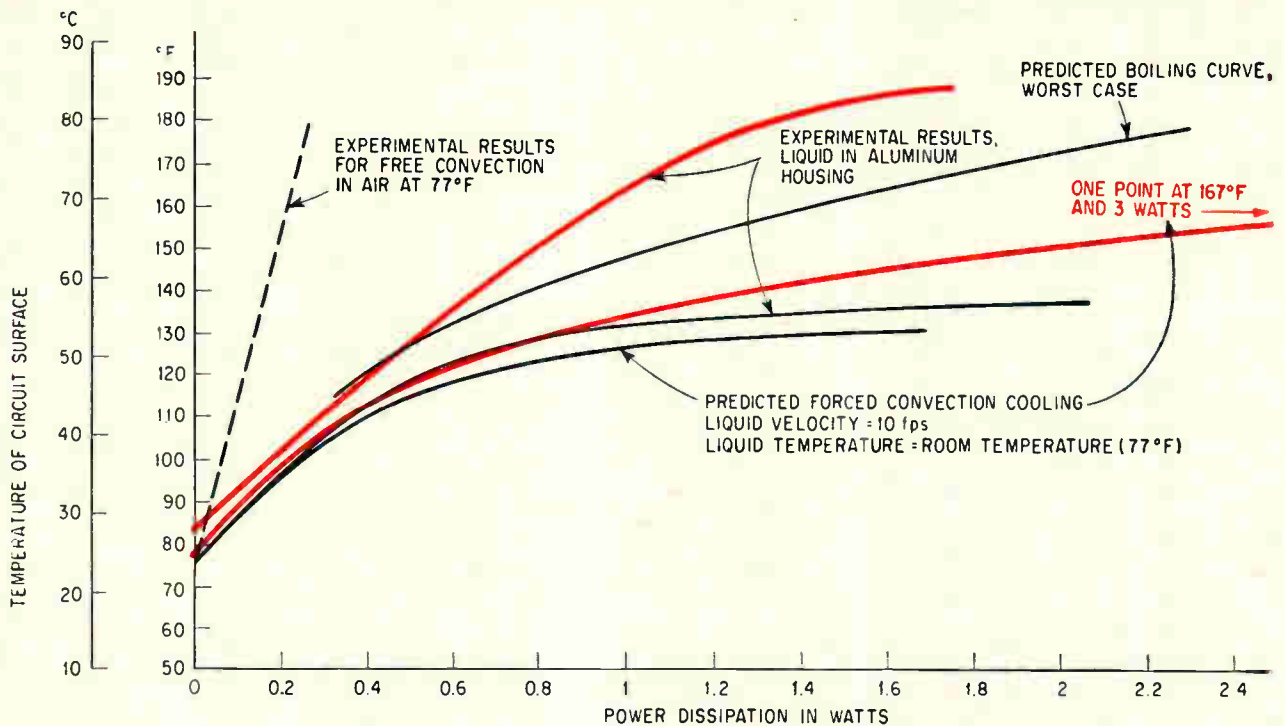
Experimental results are contrasted with calculated cooling rates for Freon C51-12 (black curves) and Freon E2 (color curves). Even without forced convection, a circuit in Freon E2 gets no hotter than a circuit in air despite a five-fold increase in applied power.
