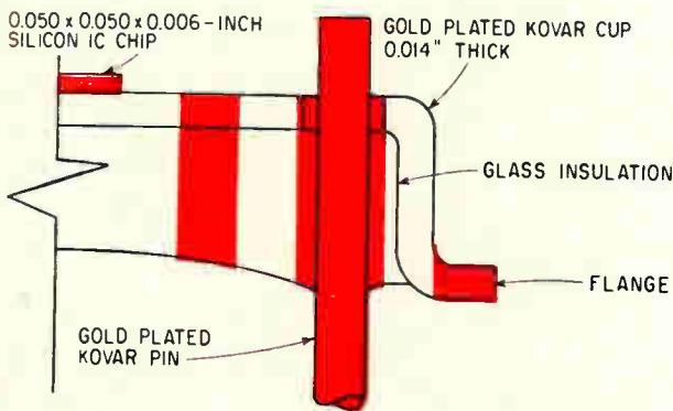
Header surfaces are divided into chip area and six concentric rings to aid heat transfer computation.
