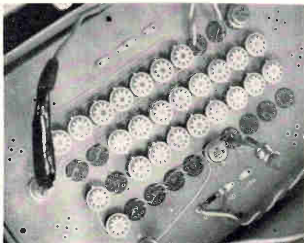
Experimental cooling chamber is simply a housing with a close-fitting plastic cover and tube sockets for connections through housing walls. Lamp at front of housing flickers when test circuitry is operating.
