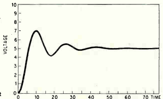
Output response for sample circuit
