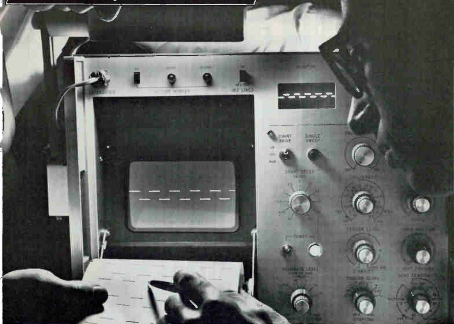
The 1806 records a 60KC square wave during a high-frequency pulse train check.
