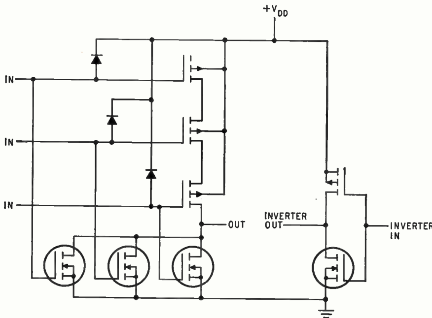
Complementary MOS device to be introduced by RCA is a dual 3-input NOR gate, and inverter on one silicon chip. Only one gate is shown, with the p-channel elements circled in color. Supply voltage may range from 6 to 12 v.
