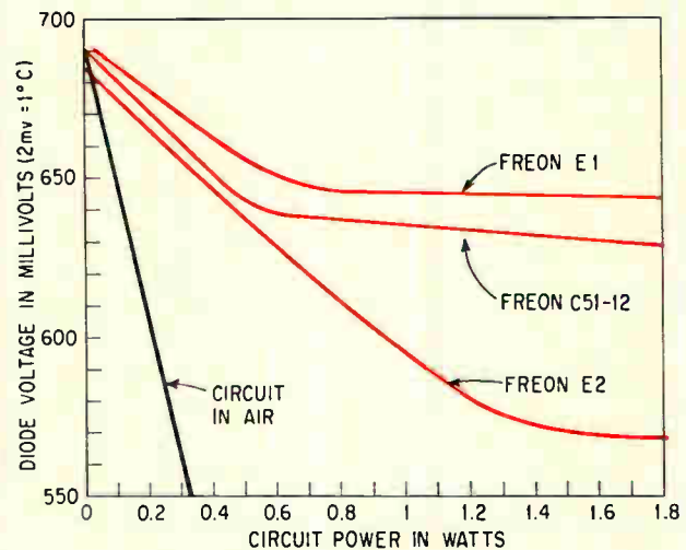
Integrated circuit operated in air quickly heats up, as indicated by sharp drop in diode voltage (black curve). In dielectric fluids, same circuit remains relatively cool at several times the applied power (color curves).
