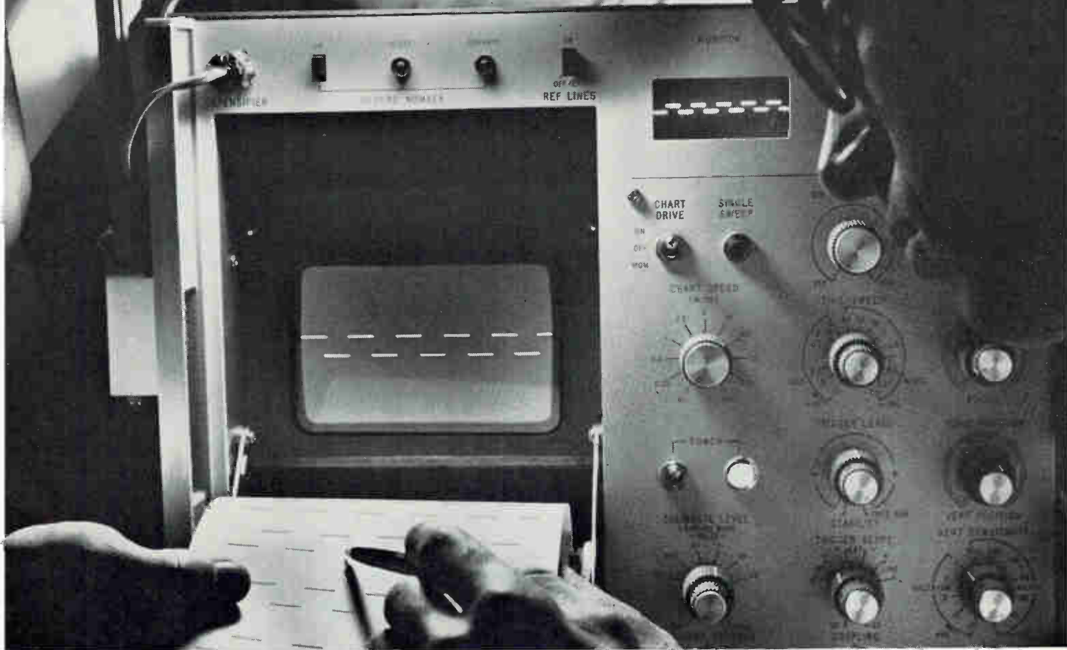
The 1806 records a 60KC square wave during a high-frequency pulse train check.
