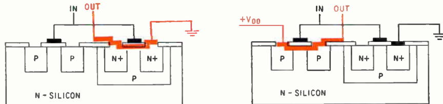
Diagram on left corresponds to high input, diagram on right, to low input. Output current paths are shown in color. N-channel device is at right of section drawings. Output current paths are shown in color.
