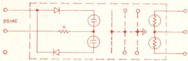
Internal schematic of AC Drive Type 5510, 60 to 400 cps. R = Limiting resistor.
