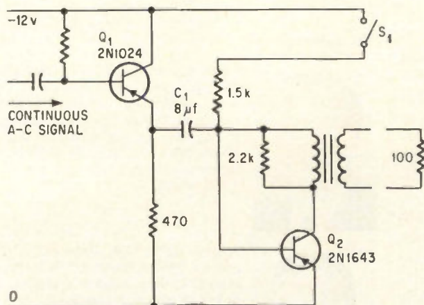
Two transistors and a 1:1 transformer accomplish audio switching without collector bias.
