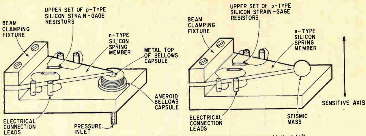
Two semiconductor transducers for converting force variations into changes in voltage. Unit at left monitors air pressure; device at right monitors acceleration. Four p-type silicon strain-gage resistors are diffused into the n-type silicon spring member and connected to function as a Wheatstone bridge. The spring member is deflected by the force exerted by the aneroid pressure capsule (device at left) or by acceleration. This creates a bending moment in the cantilever beam that is detected by the diffused strain-gage resistors and converted into a change in electrical output.
