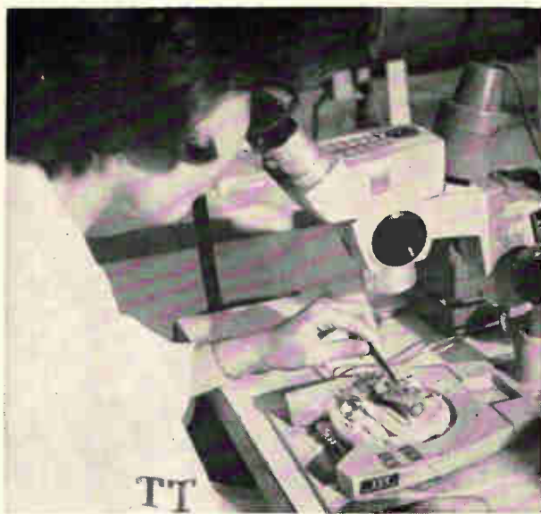
Bonding and sealing setups used in initial production. Bonds are made (left) one at a time, but automatic parts feeders and bonding tools that make all 14 bonds simultaneously will be used. Likewise, sealing will be converted from a hotplate operation (right) to a mechanized process.
