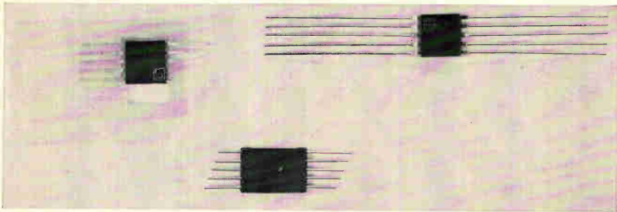
Steps in flatpack preparation: ribbon leads are cut short, flattened wire leads are welded to ribbon leads and flatpack is potted.
