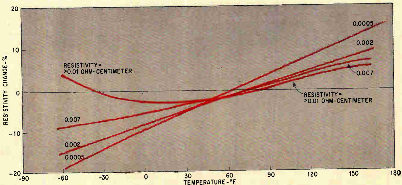
Plotting change in resistivity as a function of temperature for various values of resistivity shows that sensitivity to temperature is less with high resistivity values. The junction depth of the n-type silicon material is 2 microns.
