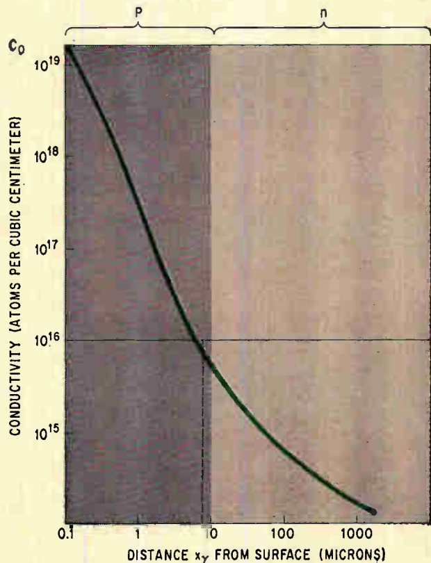
Conductivity profile for a typical semiconductor transducer with a distance of 10 microns from the surface to the p-n junction.
