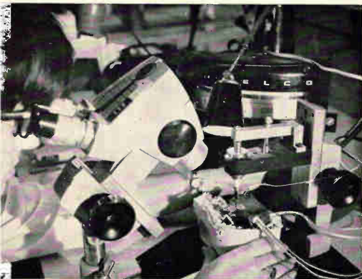
Bonding and sealing setups used in initial production. Bonds are made (left) one at a time, but automatic parts feeders and bonding tools that make all 14 bonds simultaneously will be used. Likewise, sealing will be converted from a hotplate operation (right) to a mechanized process.
