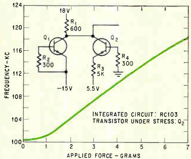
Curve shows how application of force increases the operating frequency of the avalanche oscillator circuit (inset) with the RC103 transistor under stress. Relationship of frequency and force is nearly linear.
