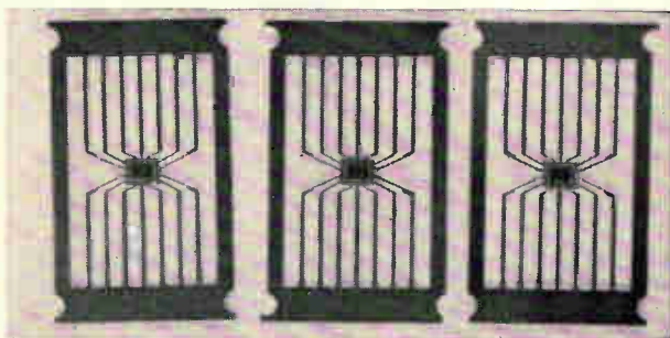
Lead frames are now handled individually during bonding. Under ITT's plans for production automation, the frames will be made in strips of 15. At left are chips with bonded leads, at right are sealed circuits.
