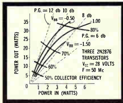
Figure 3. Performance curves for 50 mc amplifier shown in Figure 4
