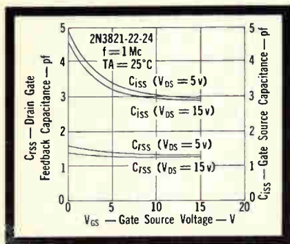
Figure 2. Important capacitance curves for 2N3821, 22, 24 transistors
