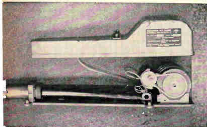
High-frequency voice antenna forms into a tube as it unwinds from chain-driven drum.
