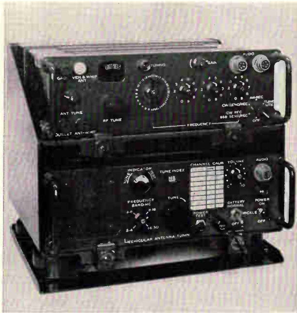
The Army's AN/PRC-62 will be of two types—vehicle (shown above) and man-pack. It will be all transistorized except for the transmitter output stages.
