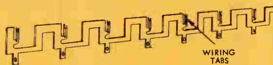
Encoding Strips allow code to be set up within the switch and eliminate diode matrices, and costly cables and connectors.
