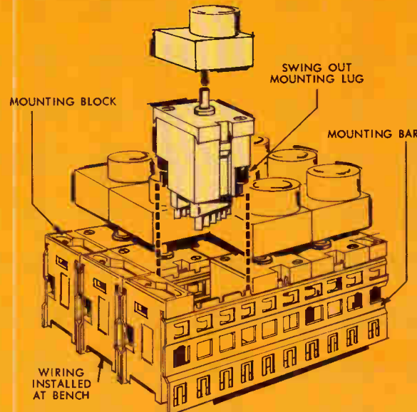
Matrix is assembled at the bench —mounting bars and mounting blocks are assembled in single rows with only a screwdriver. Rows simply snap together into a multiple-row matrix. And at the bench the matrix is completely assembled. All assembly, encoding and wiring is done conveniently before the keyboard is installed.
