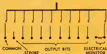
Contact Arrangement. For reliability, moving contacts are trifurcated. As the switch is operated, the common and electrical monitor circuits are made first, followed by the output bits, and the strobe circuit which tells other equipment, "All circuits made and ready". ("Repeat" function optional.)
