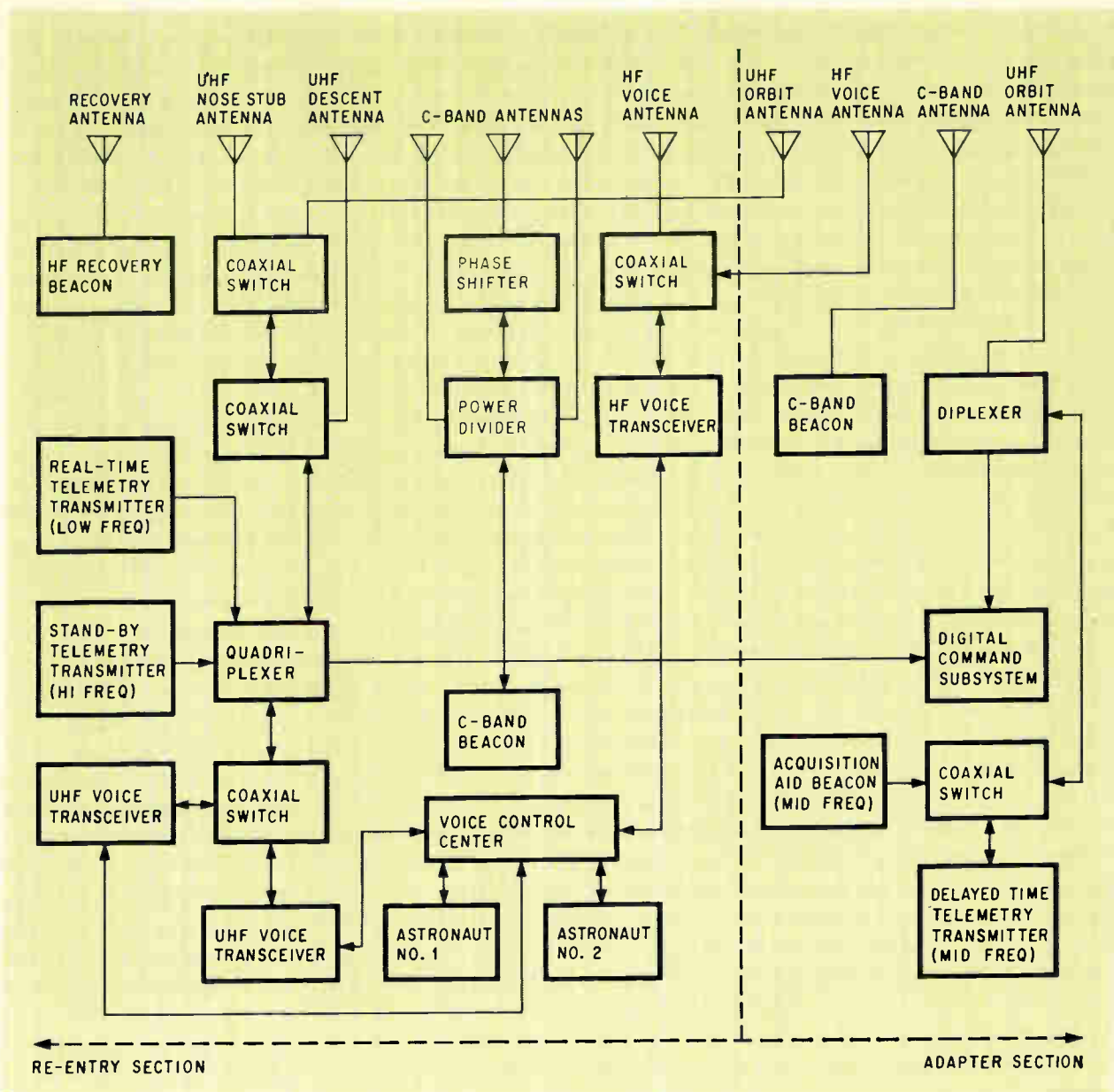
Block diagram of entire communications system. Coaxial switches allow each astronaut to select antennas as well as transmission mode. All controls are in the voice control center.
