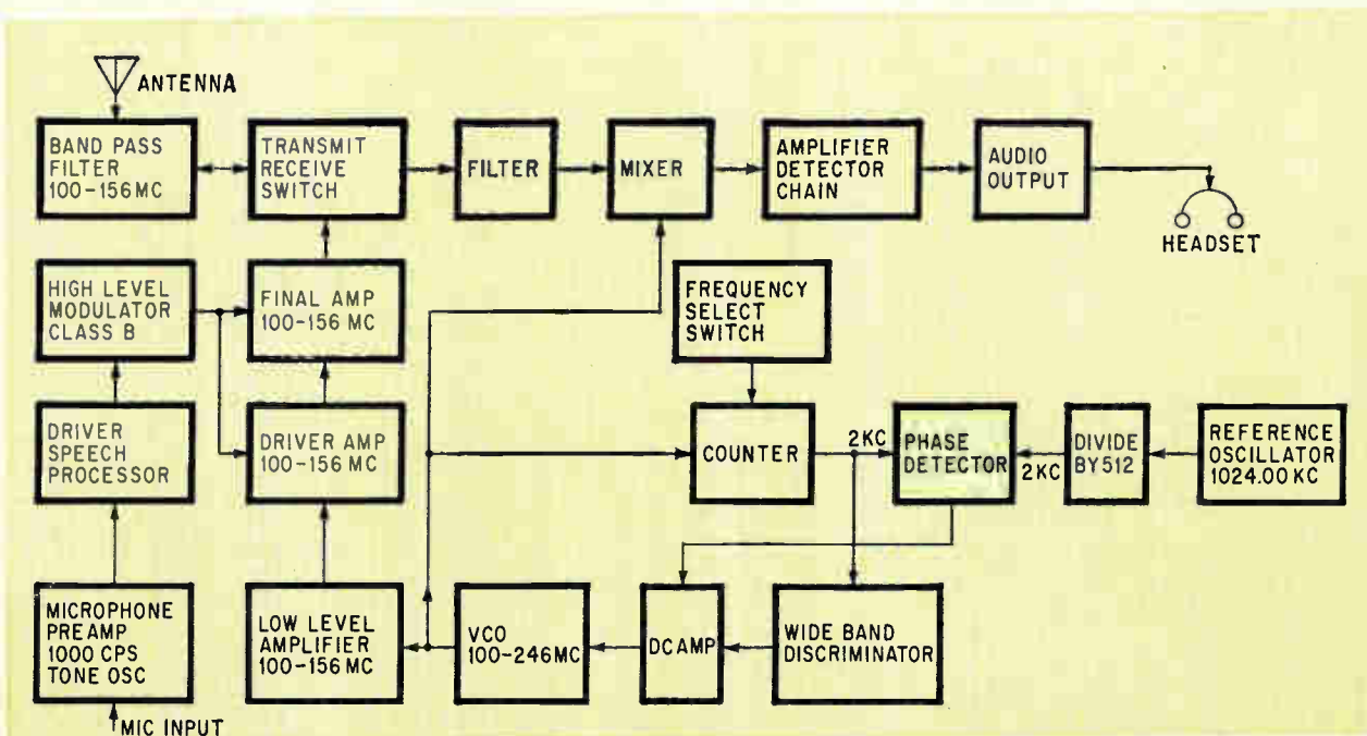
AN/PRC-65 transceiver block diagram. Broadband r-f amplifiers require no tuning adjustments.
