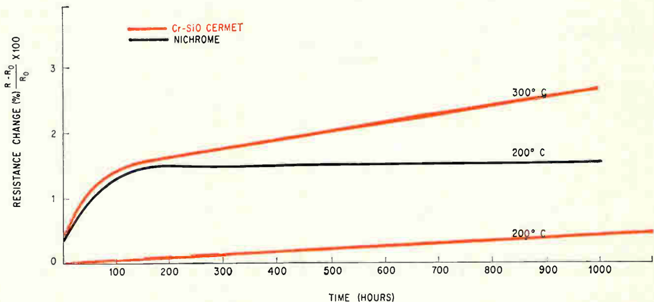
Stability of cermet-film resistors compares favorably with that of Nichrome film resistors.
