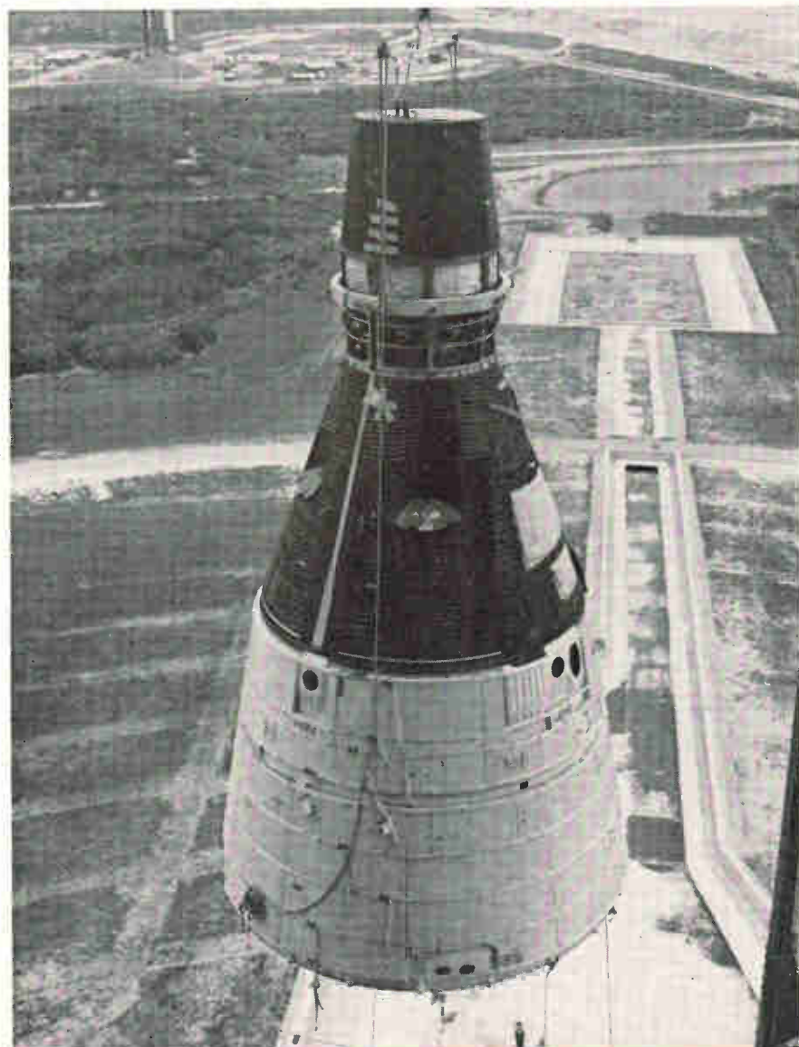
Gemini spacecraft raised to top of gantry for mating to Titan II. Similar craft will be launched next year and guided from space command center near Houston.
