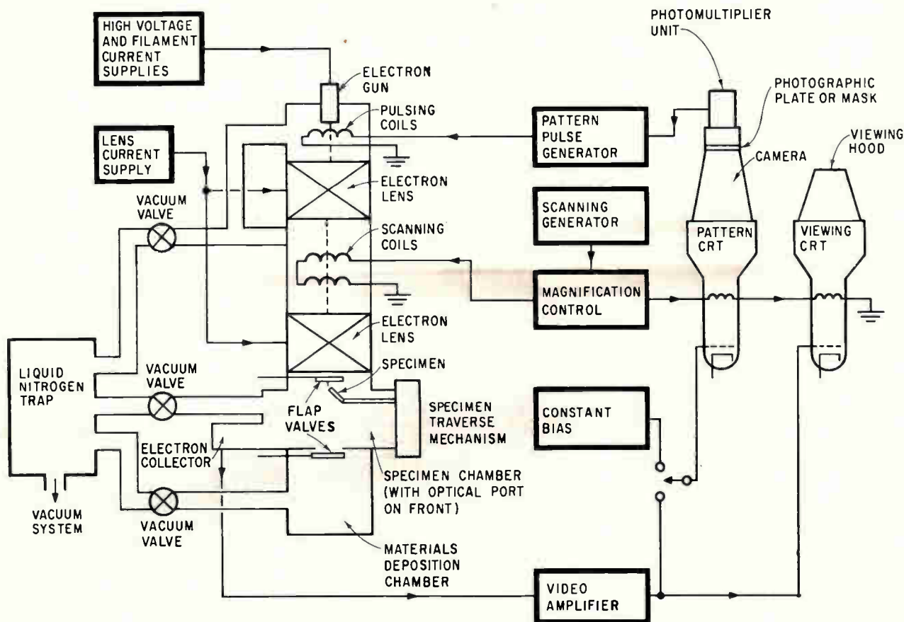
Resist-masking setup for the Micro-Scan. The scanning electron beam is gated as the pattern crt (flying-spot scanner) scans a film or black-and-white pattern of the resist pattern.
