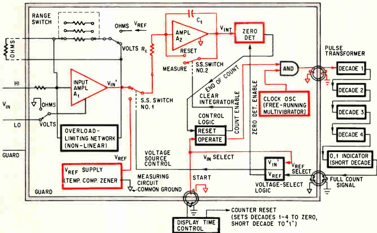
Integrating digital voltmeter designed to eliminate errors caused by noise. Many of the components are standard equipment. Amplifier A_2 (below) integrates the signal voltage being measured for 9,999 counts, which brings the decade counter to its maximum count. The next pulse overflows the counter and causes solid-state switch 1 to feed the reference voltage to A_2 . As indicated by the waveforms above, the return of the output of A_2 to zero ends the measurement.
