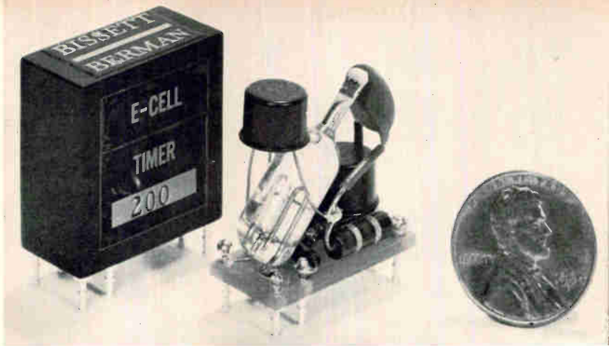
Timer is compatible with solid-state components.
