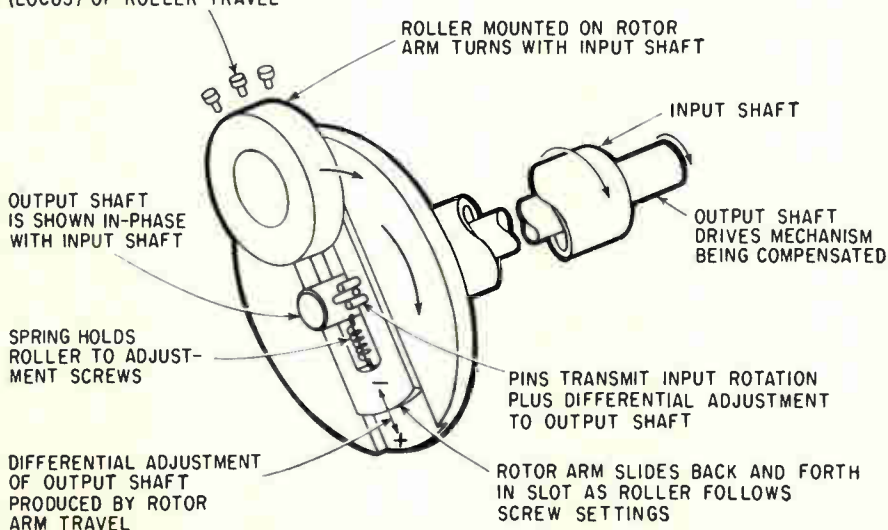
36 INDIVIDUALLY ADJUSTABLE SCREWS DEFINE PATH (LOCUS) OF ROLLER TRAVEL
