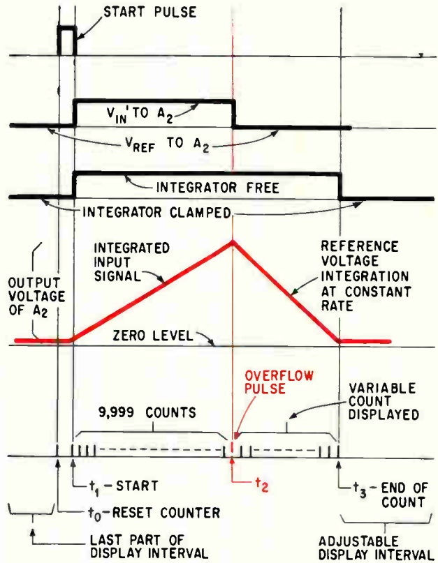
Integrating digital voltmeter designed to eliminate errors caused by noise. Many of the components are standard equipment. Amplifier A_2 (below) integrates the signal voltage being measured for 9,999 counts, which brings the decade counter to its maximum count. The next pulse overflows the counter and causes solid-state switch 1 to feed the reference voltage to A_2 . As indicated by the waveforms above, the return of the output of A_2 to zero ends the measurement.
