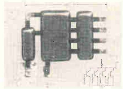
Isolith circuit bonded face down: Gaps between parts isolate the load resistor (left) from the four transistors (center) and the four input resistors (right).
