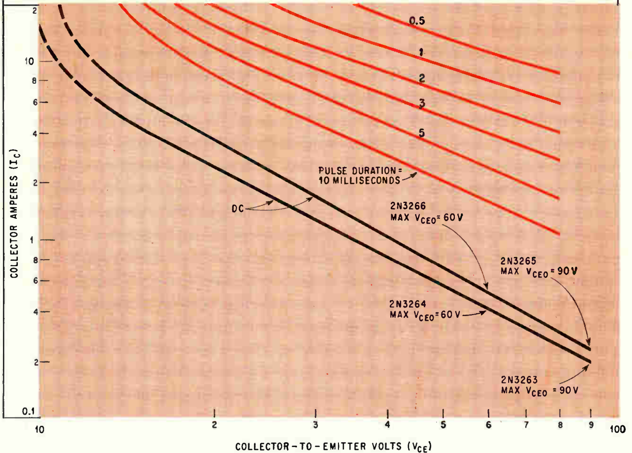
Graph taken from 2N3265 data sheet shows the safe region of operation for various pulse durations. The circuit operates safely at 50 kilocycles (10 microseconds pulse duration).
