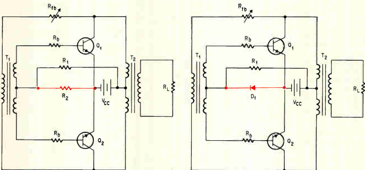
Two practical starting circuits. Inverter on the left uses a resistive voltage-divider network to supply the necessary bias. Inverter on the right uses a diode-type starting circuit.
