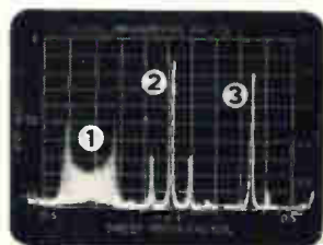
Dynamic analysis shows SB-15a versatility: (1) FM (shows dynamic deviation), (2) AM, (3) SSB with sine wave modulation.
