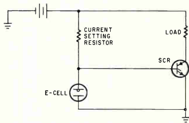
Simple timing circuit
