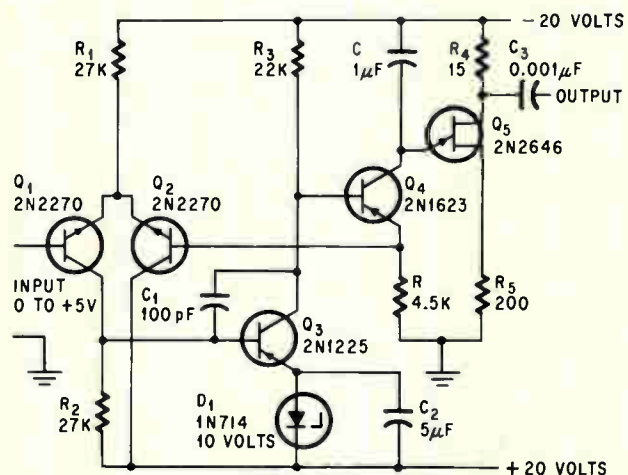
Transistor Q_4 controls the charging current for capacitor C , which regulates the output frequency of the unijunction relaxation oscillator.
