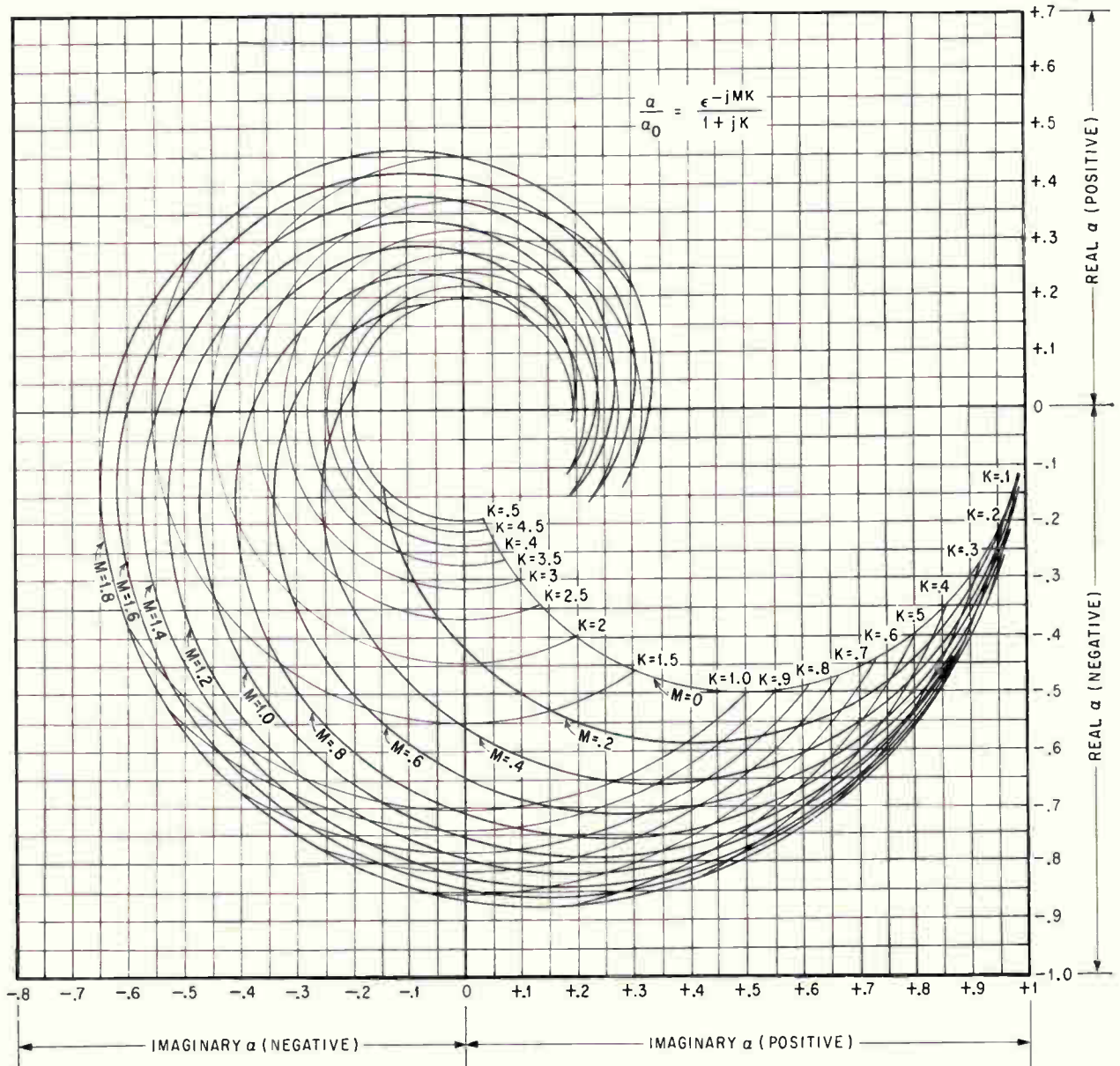
Intersection of the loci of M and K yields the normalized real and imaginary components of \alpha (High-frequency phase shift).
