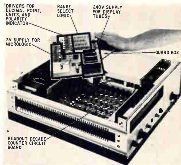
All circuits are contained on 11 plug-in cards. Common mode rejection is 140 db at d-c, 120 db for a-c. Teeth on side of cabinet are ventilation ports.
