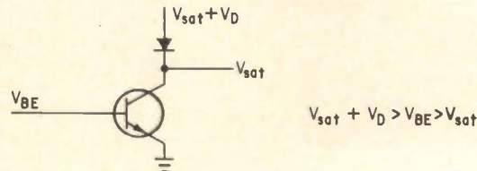
C PNPN CONDUCTING Relationship of blocking and reverse biases of a pnpn device
