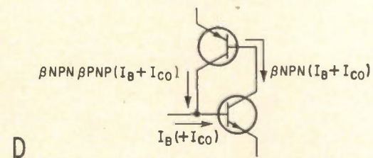
D Diagrams help explain how the two-transistor circuit of a pnpn device is derived.
