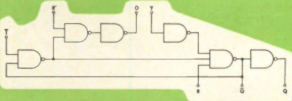
One-shot multivibrator
