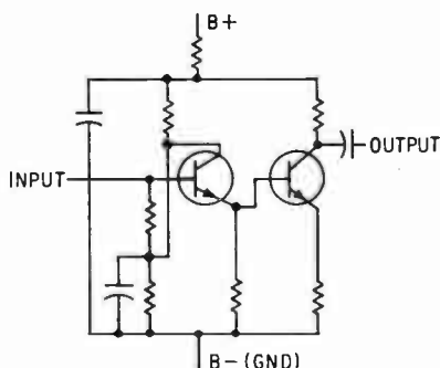
12-MC I-F AMPLIFIER on single chip is used in Motorola 120 Mc a-m receiver
