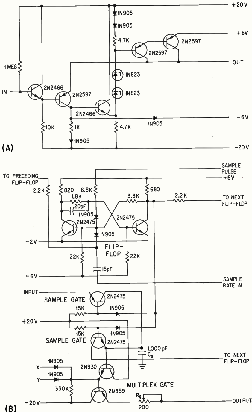
(B) VIDEO AMPLIFIER with unity gain (A); sample-and-hold circuit (B)—Fig. 2
