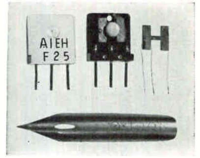
PORTION of filter assembly (opposite), showing H-shaped ceramic element and mounting
