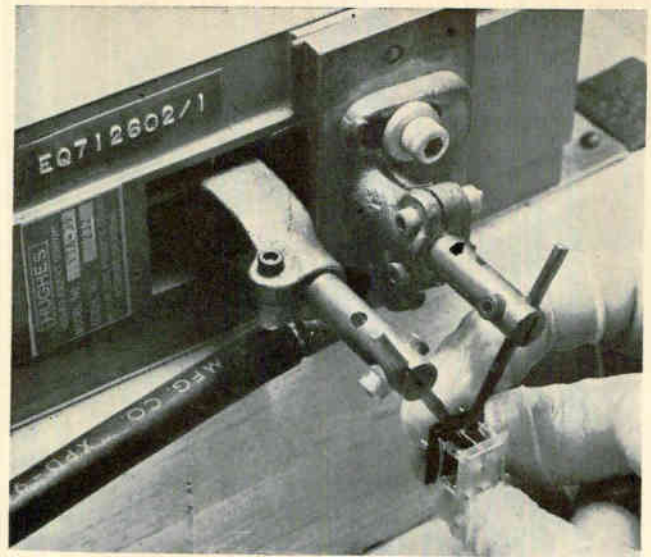
OPERATING one of twelve Hughes welders used by Martin-Orlando in fabrication of welded modules. Most welds are made at right angles, allowing the welding electrodes to close properly on the leads. Two variables, electrode pressure and power, in watt-seconds, must be proper to obtain a good weld. Before undertaking a welding program, several hundred welds are made under varying conditions. They are examined with a Hunter pull tester and the best combination chosen
