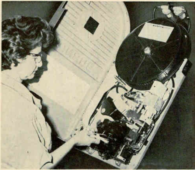
CRIMPING TOOL runs at high speed beneath protective cover, opened here to show inner workings. Machine can be adapted to a wide variety of Burndy contacts, including those used in modules. It was developed to insure quality of crimped terminal connections and turns them out at an average of 3,000 an hour. The machine can be flat mounted or set at intermediate angles up to 45 deg. There are no external moving parts and the small wire entry port gives positive protection to the operator
