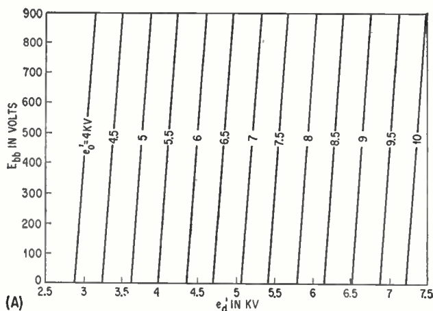
(A) DAMPER-cathode pulse voltage E_a (A), the ratio of output-tube plate dissipation to average plate current P_{bo}/I_{o(avg)} (B), and the ratio of output-tube plate dissipation values at maximum brightness and at zero beam (C) may also be determined from previous curves—Fig. 3
