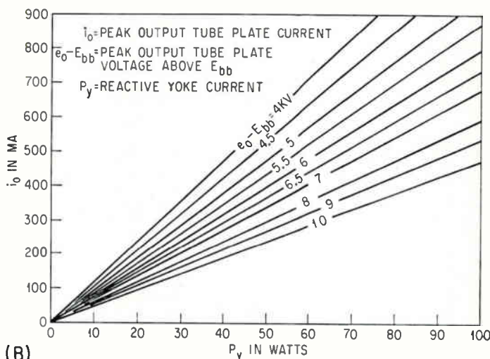
YOKE reactive power P_y , as a function of peak-to-peak yoke current \bar{i}_y and yoke inductance L_y (A) and required peak output-tube current i_o for a given yoke power and output-tube plate pulse voltage e_o (B)—Fig. 1
