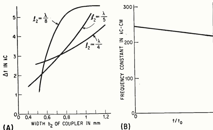
RELATION between coupler width and length (A), with 455-Kc center frequency; and relation between frequency constant and ceramic thickness (B), where ceramic area equals resonator area—Fig. 2
