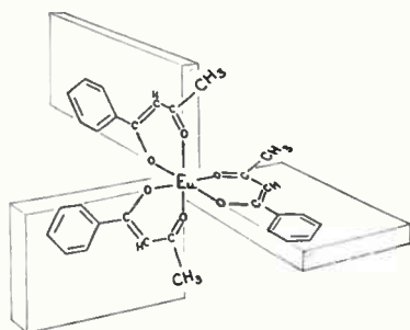
STRUCTURE of europium trisbenzoylacetonate, a typical rare earth chelate—Figure 1
