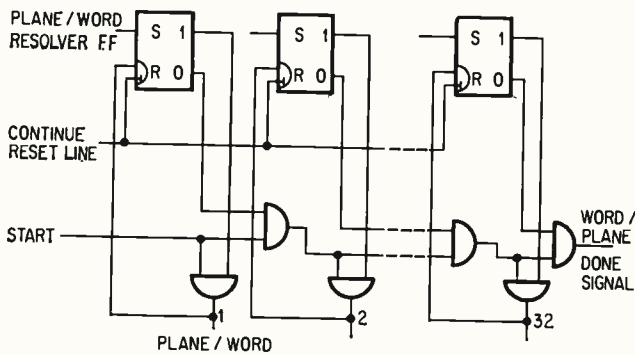
PLANE and word-resolver circuit—Fig. 5
