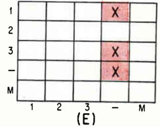
LINEAR ARRAY (A). Failure patterns, with signal channel number in the first column of each, for input (B), channel component (C), beam combiner (D) and for probable beam combiner (E)—Fig. 1
