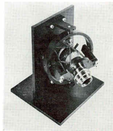
ROTATING fiber optics assembly is mounted in gimbals, with springs moving the ball (center) through half the deflection angle
