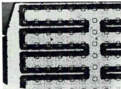
OVERLAY transistor has 156 emitter elements, 1/2-mil square and fabricated to 1-micron tolerance (RCA)
