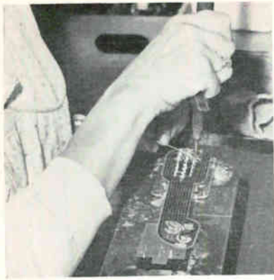
TYPICAL production setup for soldering Flexprint cable to assembly's fixed terminals
