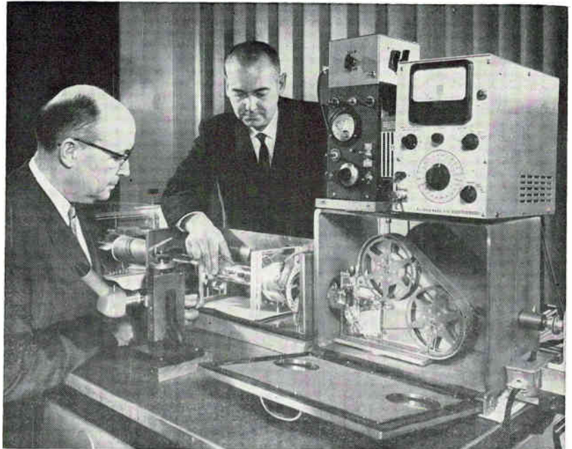
EXPERIMENTAL UNIT has camera chamber, lower right, attached to tube containing electron gun, left, with external deflection system; entire system is evacuated to 2 \times 10^{-6} Torr
