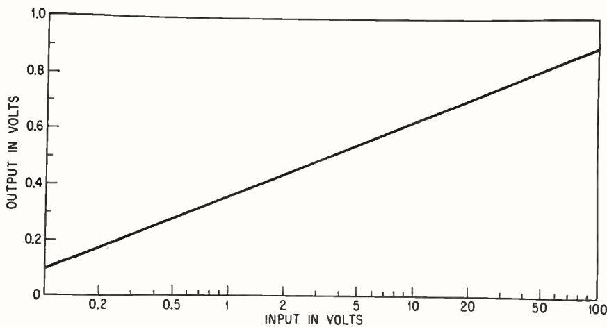
CALIBRATION of three-decade logarithmic attenuator—Fig. 2
