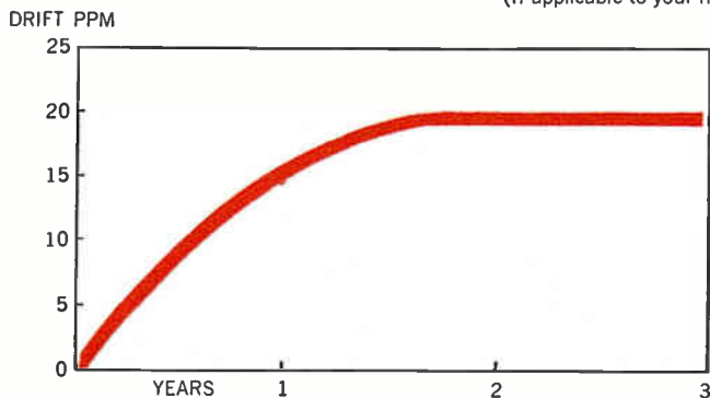
Drift in PPM. Resistors stored and measured at room temperature without the use of controlled atmosphere.
