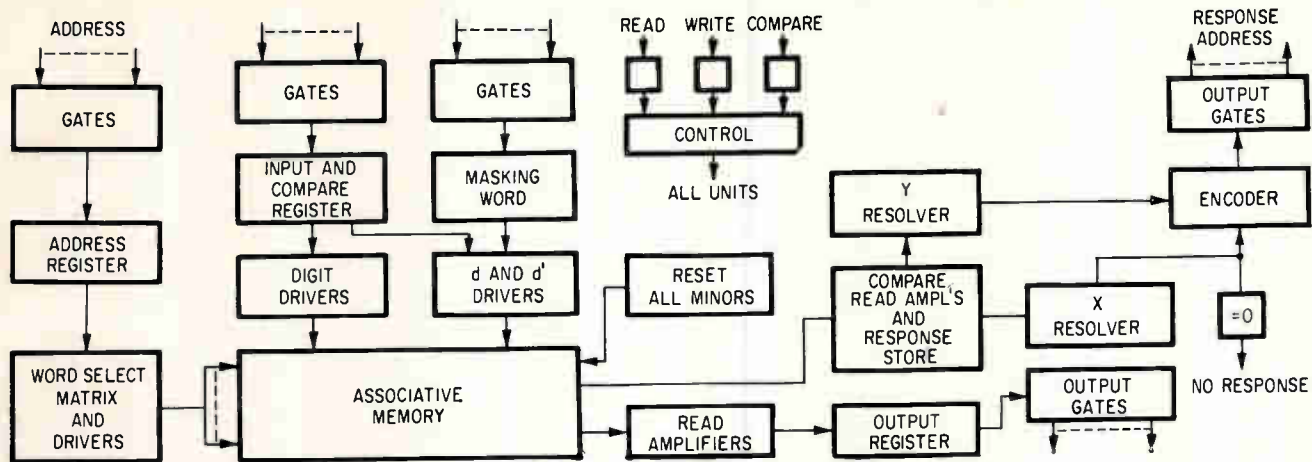
ASSOCIATIVE MEMORY—Fig. 3
