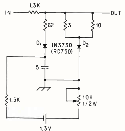
LOG ATTENUATOR for positive polarity only—Fig. 3
