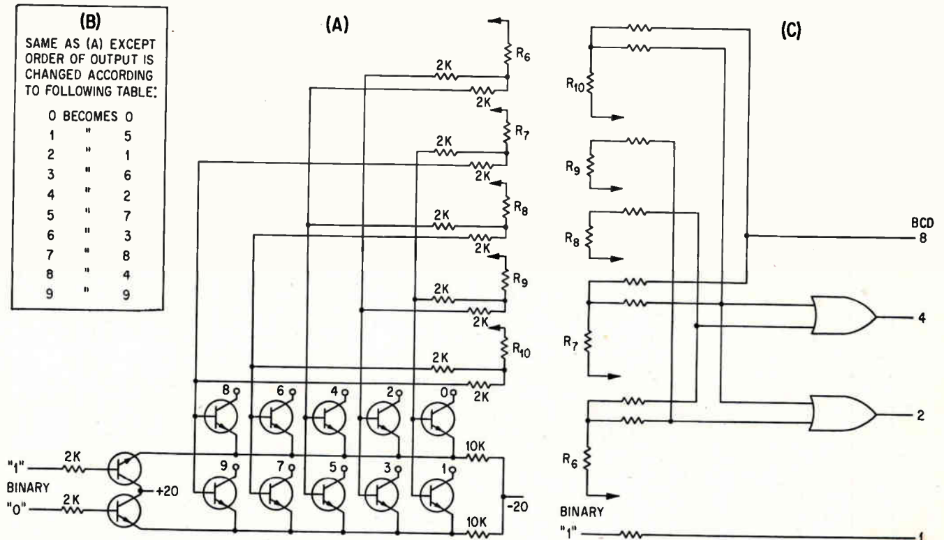
COUNT of bi-quinary decade is displayed by Nixie indicators (small numbered circles) which require no buffers (A). Outputs are reversed for qui-binary decade (B); conversion of qui-binary to BCD (C)—Fig. 3
