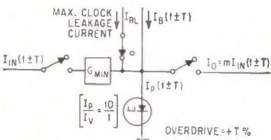
(B) TRANSISTOR COUPLED LOGIC
