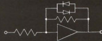
NON-LINEAR AMPLIFIER
