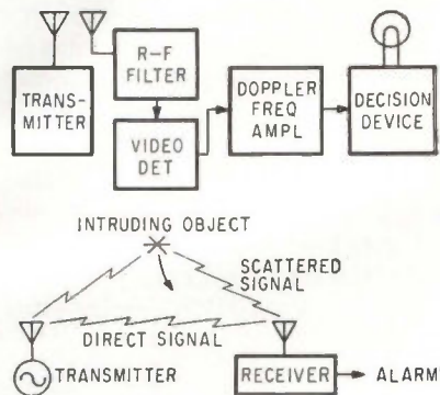
BISTATIC radar radiates intruder detection "fence"
