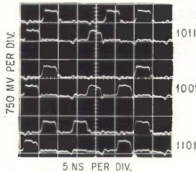
WAVEFORMS recirculating in a 10-bit memory loop at 250-Mc phase rate
