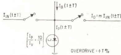
(A) SINGLE STAGE TUNNEL DIODE LOGIC
