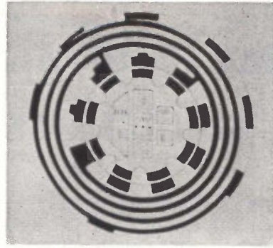
QUARTER-INCH circles are integrated circuits used to telemeter physiological data from animals. Schematics (A)
