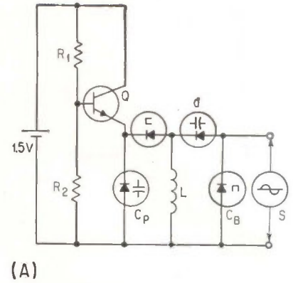
QUARTER-INCH circles are integrated circuits used to telemeter physiological data from animals. Schematics (A)
