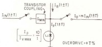
(A) SINGLE STAGE TUNNEL DIODE LOGIC
