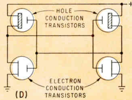
INSULATED-GATE field-effect transistor (A) has output characteristics of (B) and transfer characteristics of (C) when gate bias is varied in 2-v steps from 0 to 20 v. Load is 10,000 ohms and supply is 20 v. Complementary pairs of transistors could be used in the memory cell designed by P. K. Weimer of RCA Labs (D) whose two stable states would have essentially no dissipation—Fig. 4
