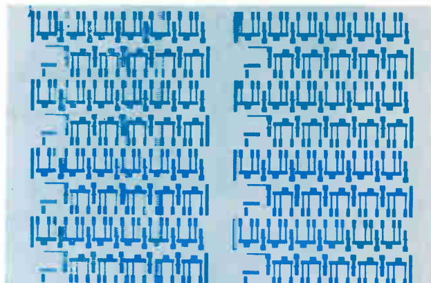
(2) Resistor Lands, Some Cu Interconnections
