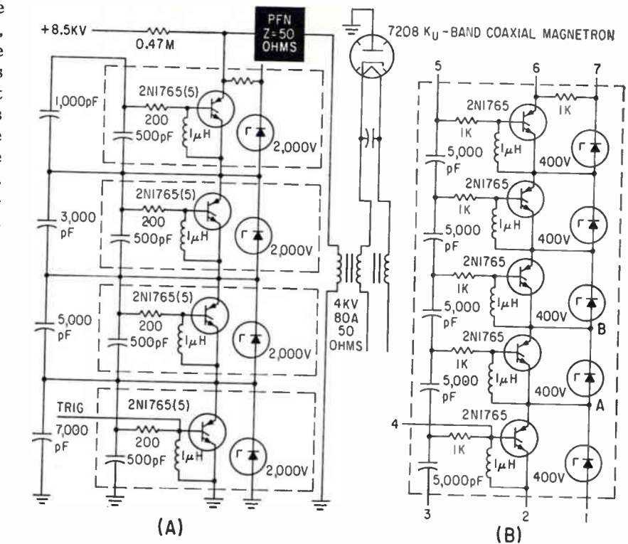
DEVELOPMENTAL 300-Kw modulator (A) uses four 2-Kv switching modules (B) in series—Fig. 4
