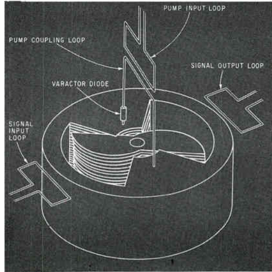
EXTREME SIMPLICITY of parametric amplifier is evident in these pictures—Fig. 1
