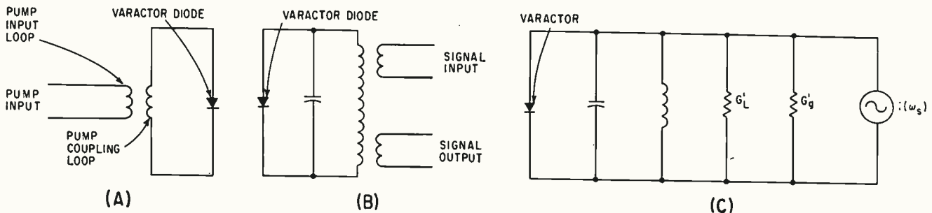
EQUIVALENT CIRCUITS at pump frequency (A), at signal-idler frequency (B) and for mathematical analysis (C) where G_g' and G_L' are the equivalent, transformed, generator and load conductances—Fig. 3
