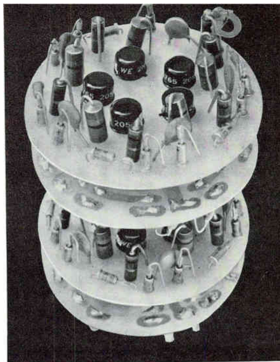
MODULES in 8-Kv experimental switch assembly are mounted back to back to limit inductance
