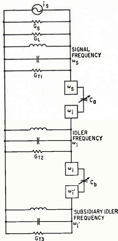
NARROW-BAND ideal bandpass filters for signal, idler and subsidiary idler frequencies are represented by boxes in equivalent circuit—Fig. 1
