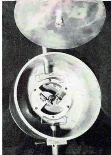
EXTREME SIMPLICITY of parametric amplifier is evident in these pictures—Fig. 1
