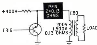
LINE-TYPE modulator uses single pnpn transistor—Fig. 1
