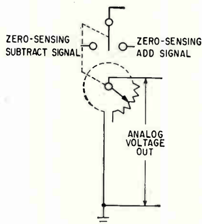
POTENTIOMETER encoder with analog output—Fig. 6
