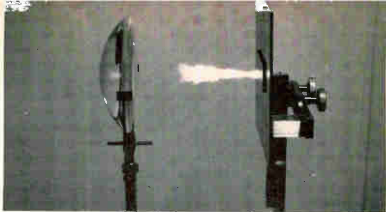
CARBON STEEL gives off metal vapor plume when hit by focused beam of American Optical Co.'s Nd glass laser
