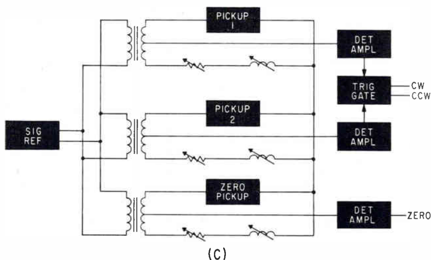
HIGH RESOLUTION can be obtained using phase-relationship encoding systems (A) and (B) with a sensing readout circuit (C)—Fig. 5
