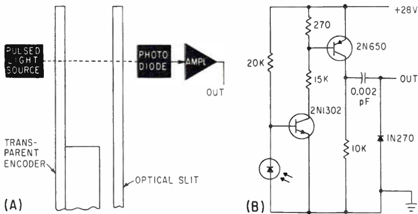
TYPICAL PHOTODIODE shaft-position encoder (A) can be used with amplifier (B) to produce pulses for logic circuit—Fig. 3
