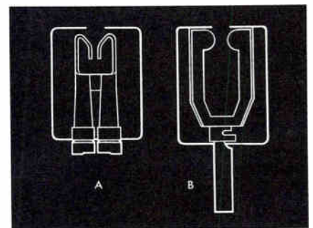
Wedging action of Amphenol ribbon-type (A) and long spring base of Amphenol Prin-Cir connectors (B) assure firm printed circuit board retention, whether board happens to fall at low (.055") or high (.073") end of thickness tolerance.
