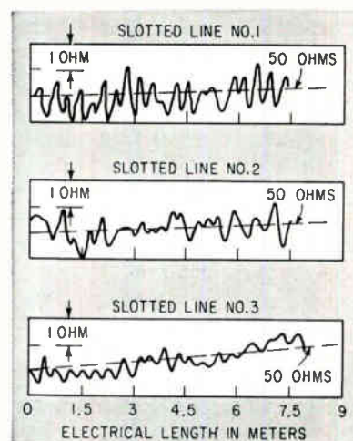
MEASURED characteristic impedance for three lines—Fig. 2
