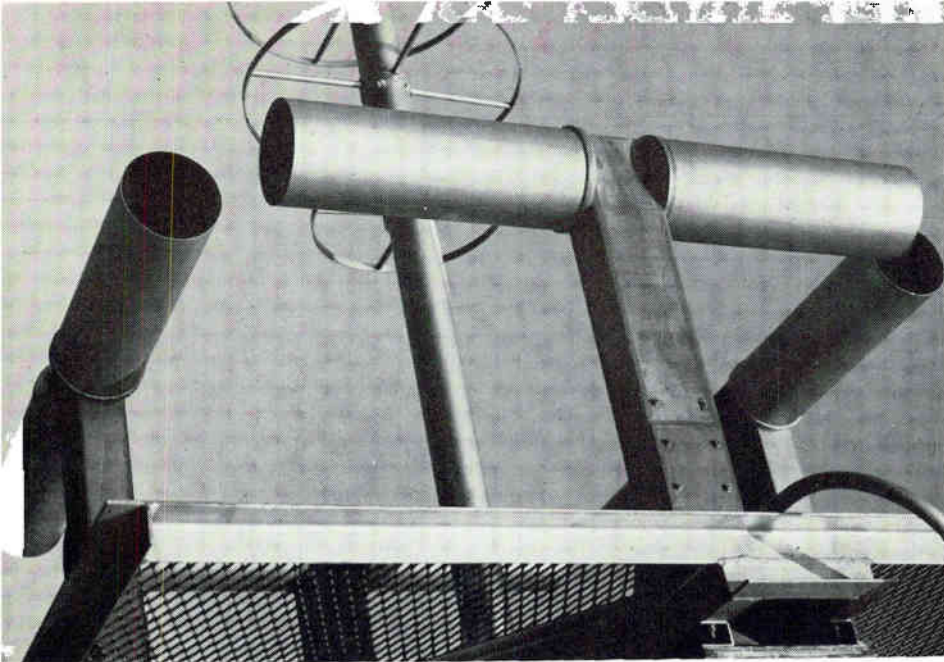
THIS DIPOLE, designed by the procedure given in text, yielded impedance data shown in Fig. 2C
