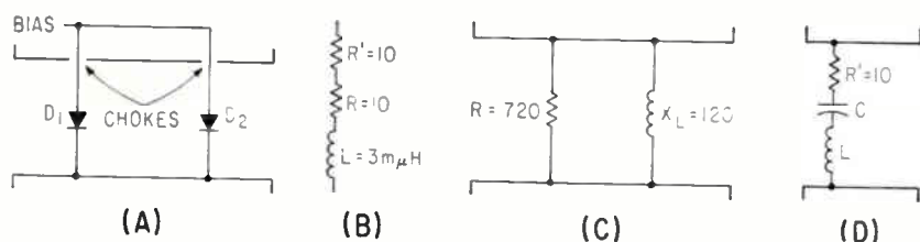
WAVEGUIDE SWITCH contains two germanium diodes one-quarter wavelength apart (A). Equivalent circuit of one diode with forward bias (B) and the waveguide equivalent circuit at 6 Gc. Waveguide equivalent circuit with reverse bias (D)—Fig. 4
