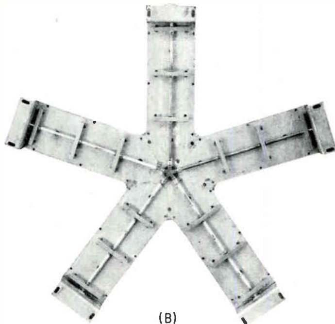
FIVE WAY switch at S-band is a slab line structure using germanium diodes (A). Center conductors (B) contain four diodes in series—Fig. 3
