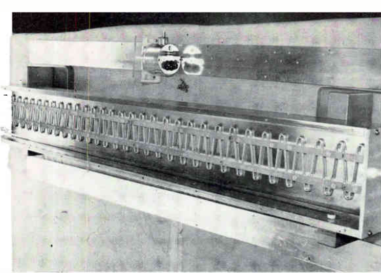
SLOTTED LINE No. 1 has a wave retardation factor of 5, a range from 25 to 200 Mc, and is 62½ inches long
