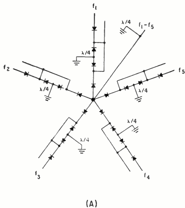
FIVE WAY switch at S-band is a slab line structure using germanium diodes (A). Center conductors (B) contain four diodes in series—Fig. 3
