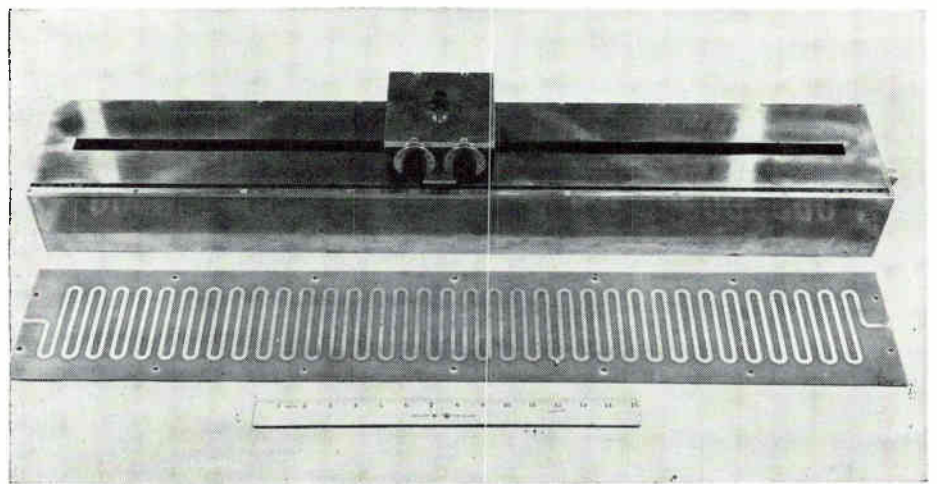
SLOTTED LINE No. 3, with traveling probe, is only three feet long but can be used from 25 to 250 Mc
