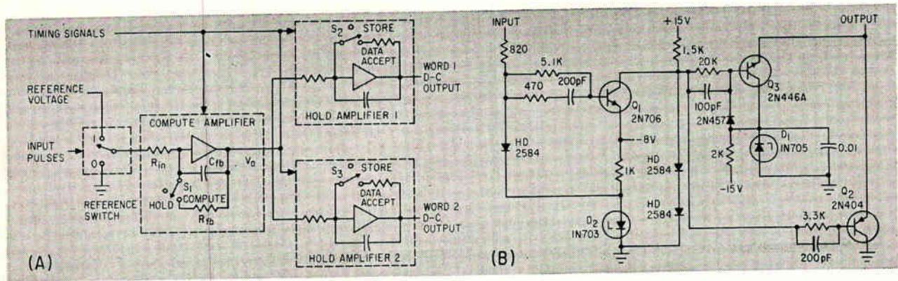
SERIAL DECODER (A) and reference switch (B)—Fig. 1
