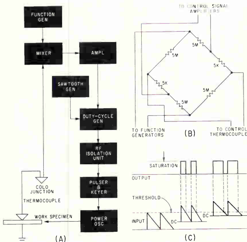
CONTROL SYSTEM block diagram, (A); low-level mixer circuit, (B); method of voltage-to-pulse conversion, (C)—Fig. 1
