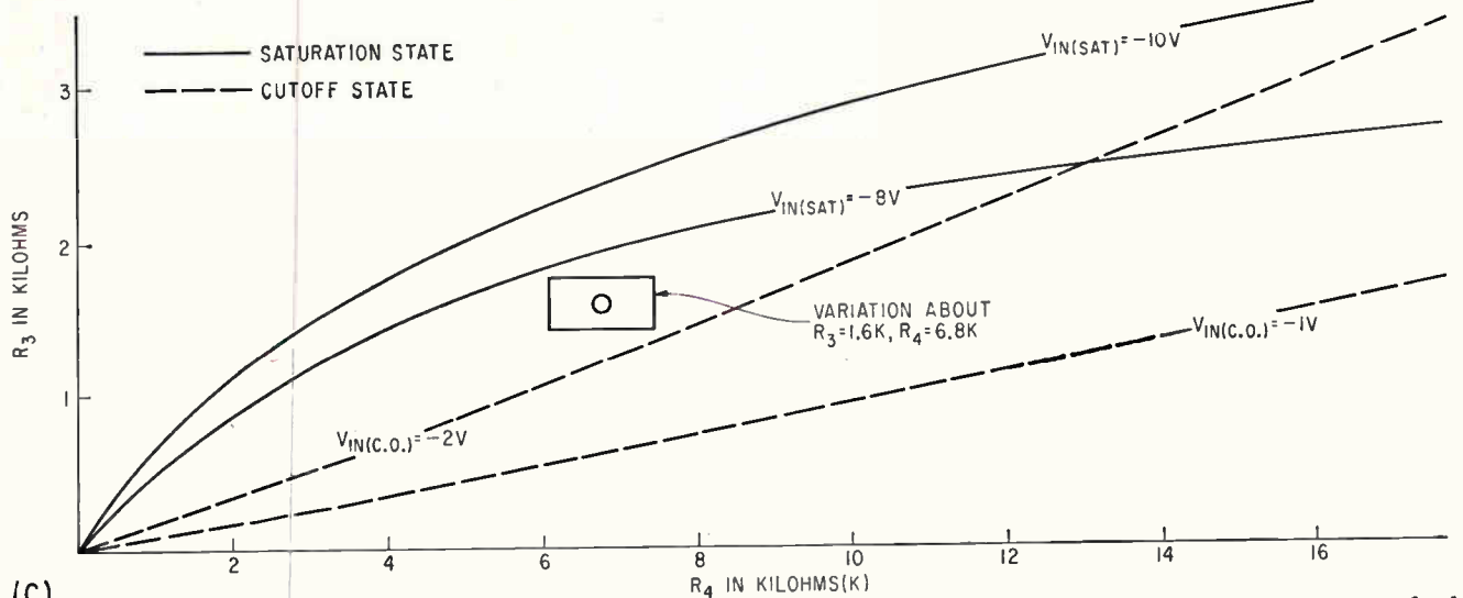
(C) EXAMPLE uses basic OR gate shown in (A) in the noninverting amplifier (B). Graph (C) provides insight on final choice of resistance values—Fig. 5
