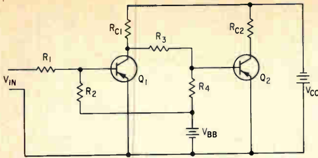
NONINVERTING transistor amplifier—Fig. 3
