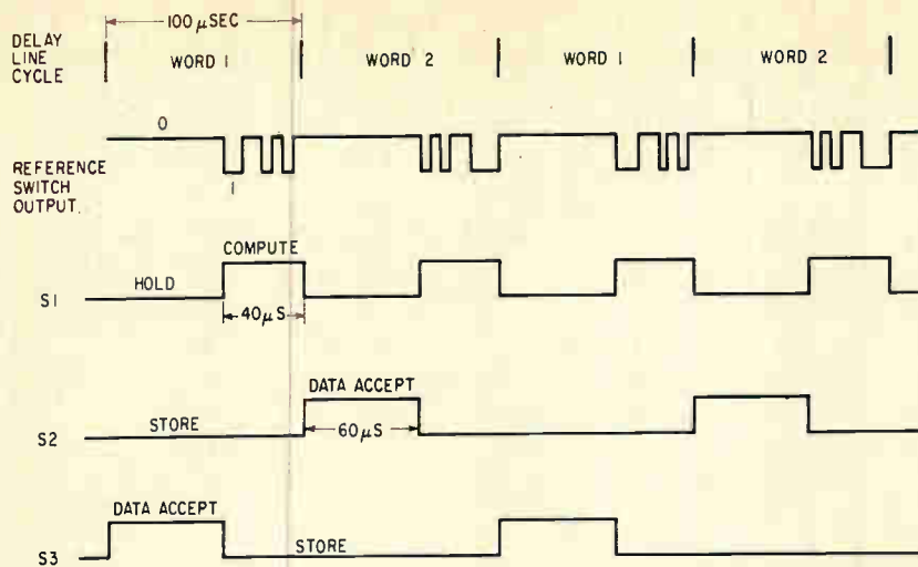
SWITCHING CYCLE for a two word system. Input data was obtained from a magnetostrictive delay line containing two serial words—Fig. 2
