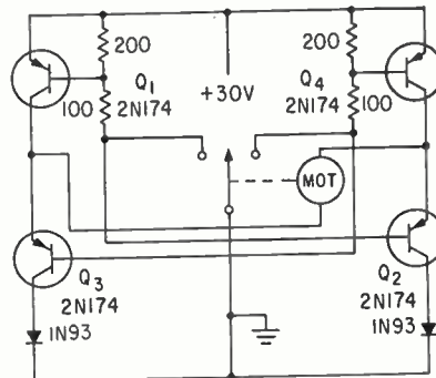
INERTIAL governor with transistor circuit regulates tendency toward motor overshoot—Fig. 2
