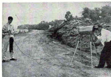
TERRA-SCOUT, made by Soiltest, Inc., Chicago, indicates on crt time for shock wave to travel from hammer (left) to crt indicator
