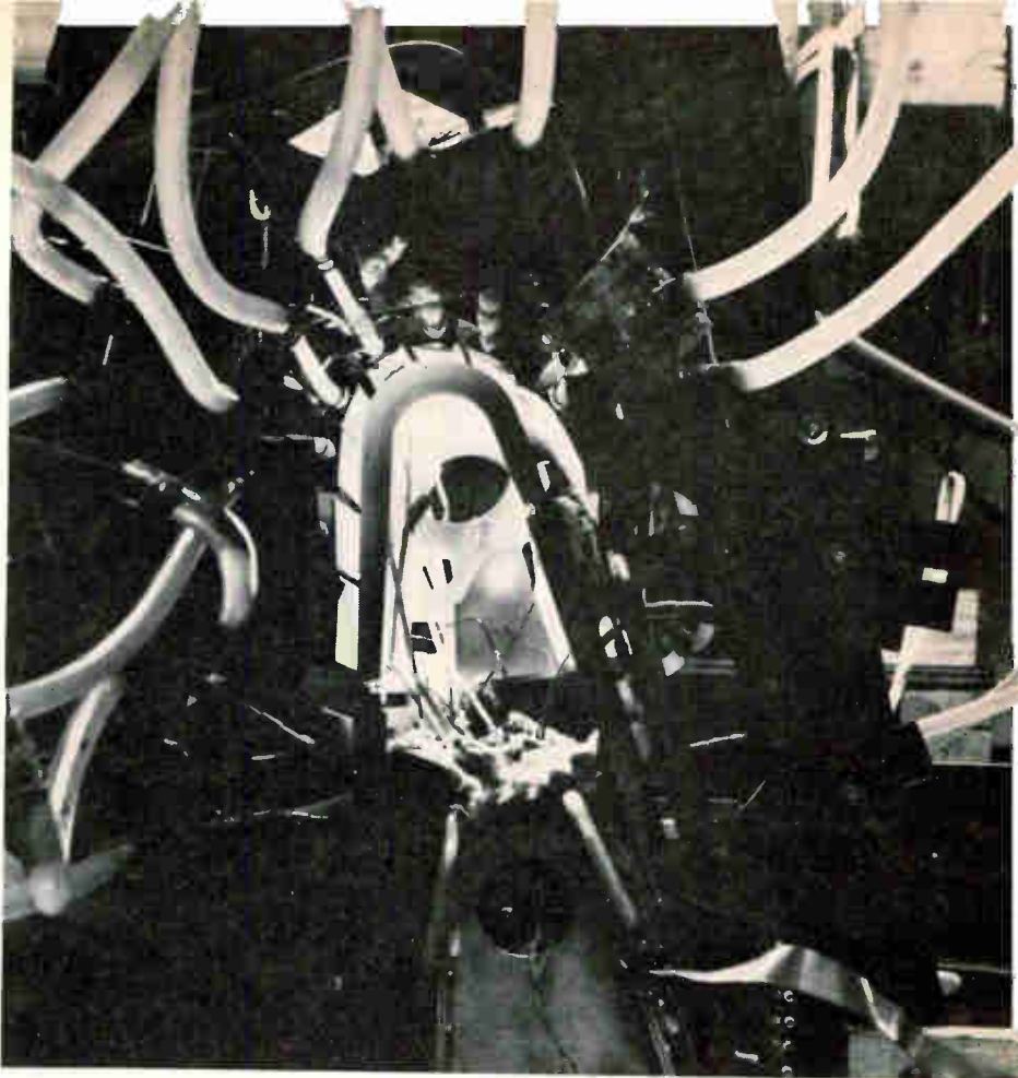
SECTION molybdenum alloy wing leading edge is heated to 3,000 deg F during testing to simulate reentry heat flow
