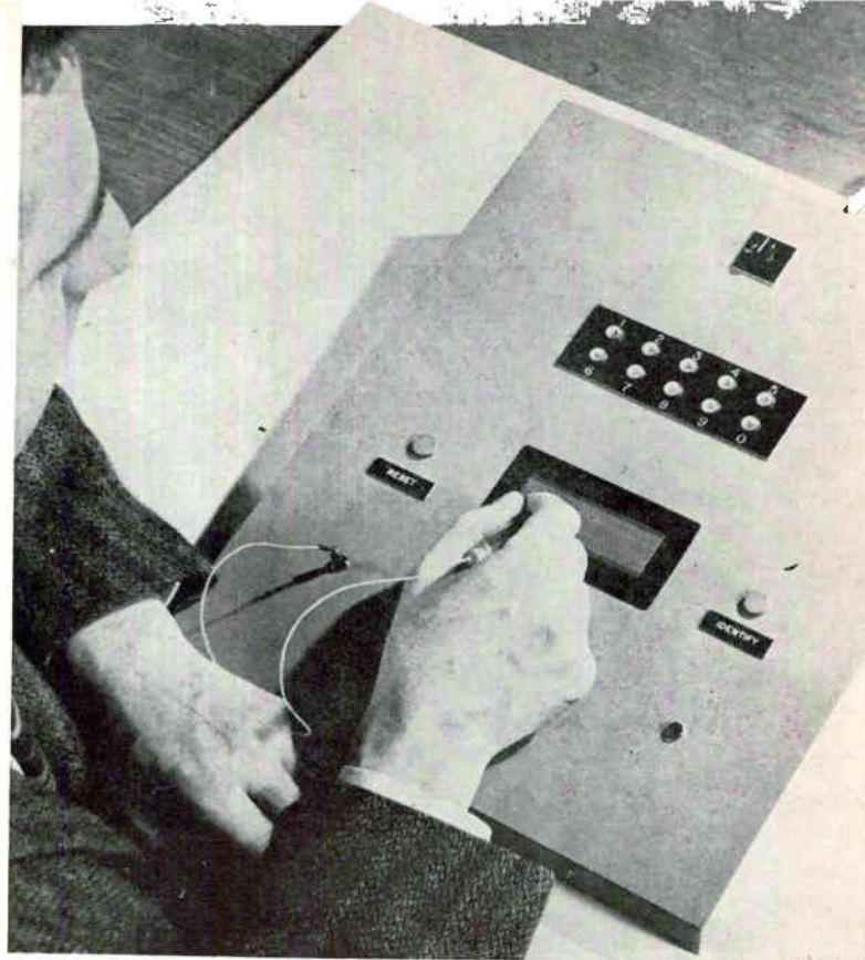
WORKING MODEL of the cursive-script reader contains 12 relays and 8 diodes. Here the author prepares to demonstrate its capabilities
