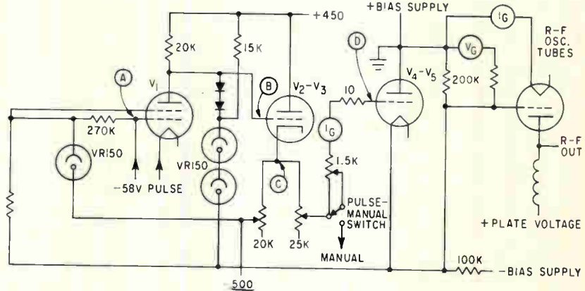
PULSER AND KEYER simplified circuits—Fig. 4
