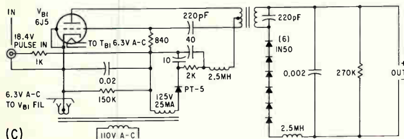
PULSE GENERATOR circuit, (A); sawtooth and sync generator, (B); isolation oscillator, (C)—Fig. 2
