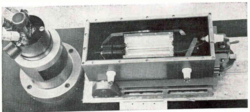
RUBY LASER is pumped by rotating mirror at Stanford Research Institute, enabling it to generate very short pulses of increased intensity. Mirror can rotate up to 10,000 rps, has rotated at 7,000 rps so far
