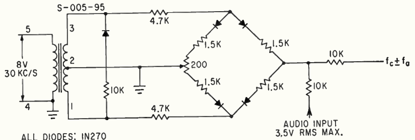
BOYNTON-SCHOLT modulator gives a 60 db suppression of 30 Kc carrier without adjustment over a wide range of ambient temperature and frequency—Fig. 1
