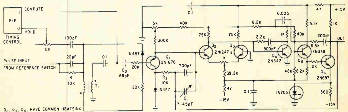
COMPUTE AMPLIFIER converts digital output of reference switch to equivalent analog voltage—Fig. 3
