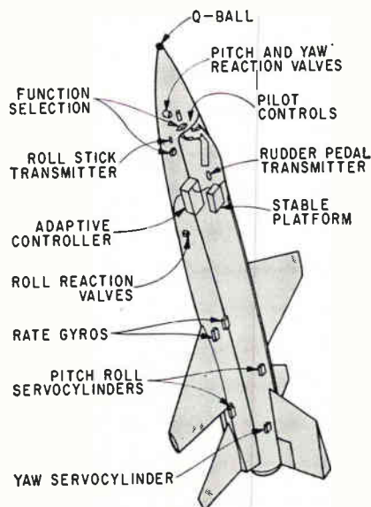
CONTROL SYSTEM components location in the X-15
