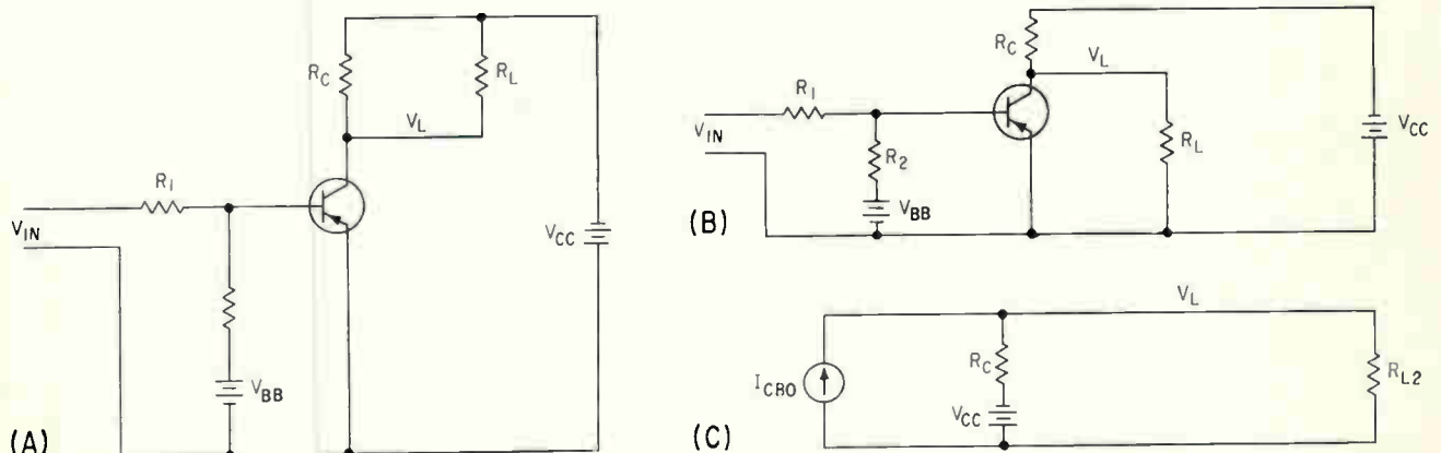
TRANSISTOR CIRCUIT with load tied to supply (A). Transistor circuit with load tied to common (B); equivalent circuit of (B) is shown in (C)—Fig. 1
