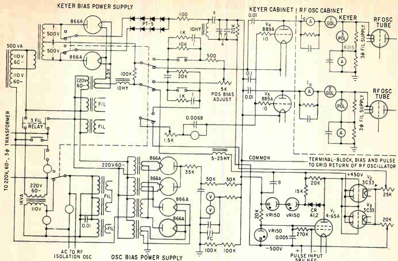
OSCILLATOR, KEYER and pulse driver circuit—Fig. 3
