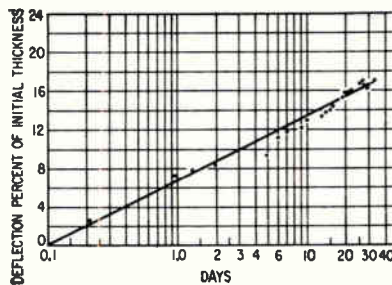
FIG. 2—Drift characteristics of sample with a 31-lb load in a 482 F chamber
