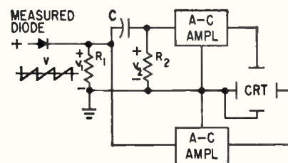
FIG. 1—Logarithmic behavior of 1N302 germanium diodes can be determined using a sawtooth input of 0.1 volt peak and a frequency of 30 kc
