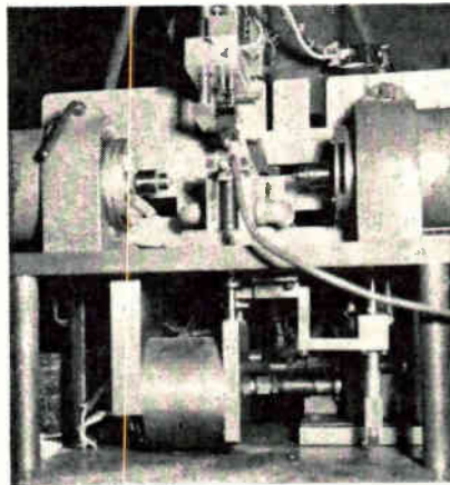
Closeup of mechanism. Drum of lower left is magnetic brake
