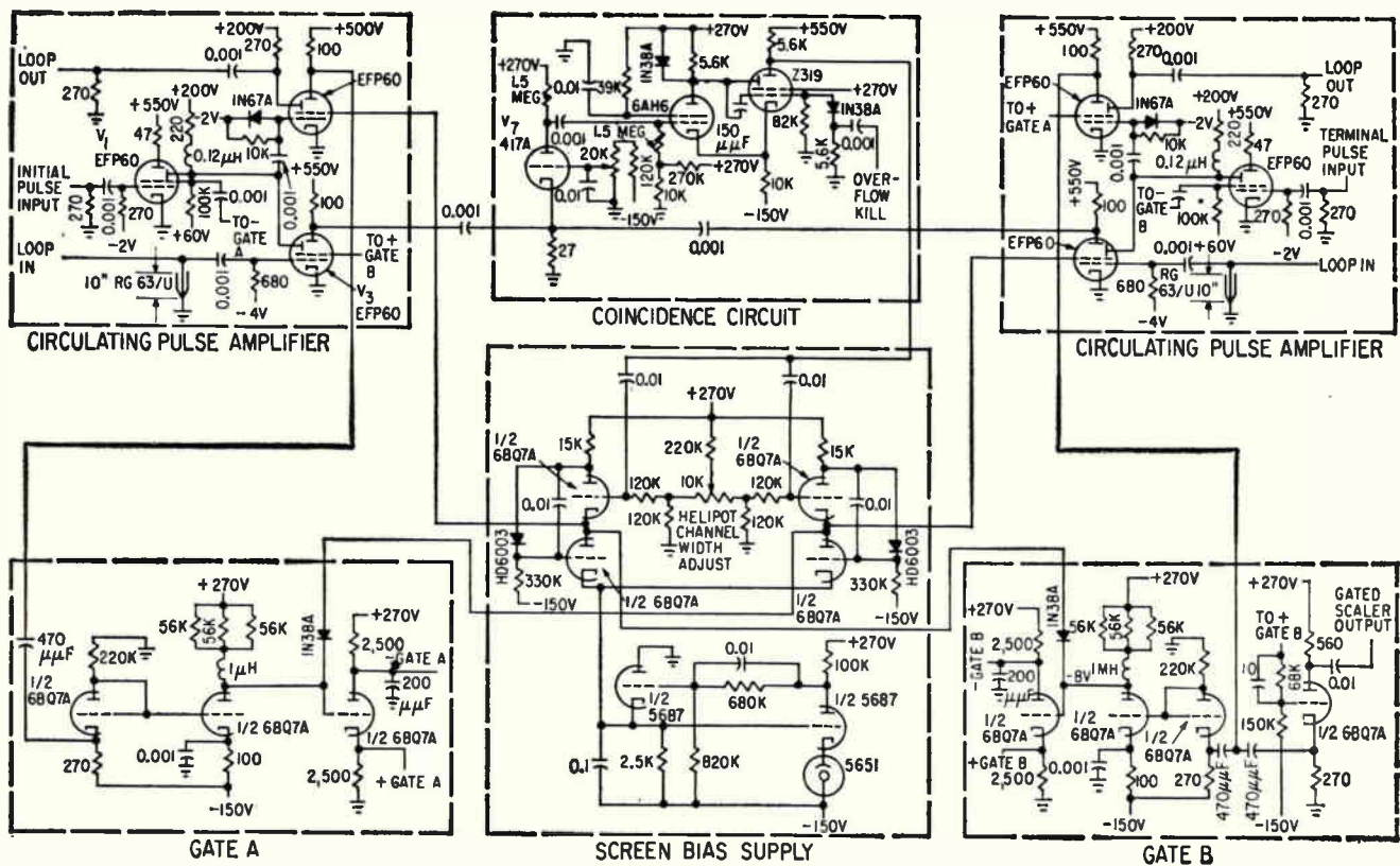
FIG. 3—Complete schematic diagram of the vernier chronotron. The circulating cable loops are not shown
