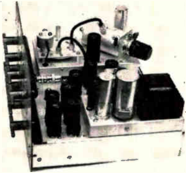
Complete transmitter and receiver assembly. Lighthouse oscillator tube is mounted horizontally at top-right
