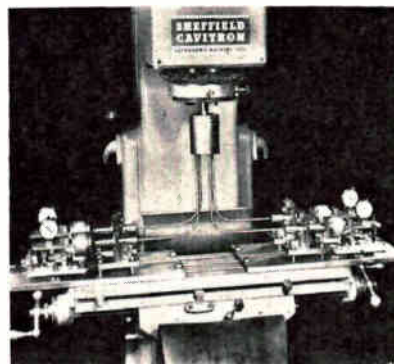
Setup with 4 cutting heads. Eight heads have been operated from a transducer
