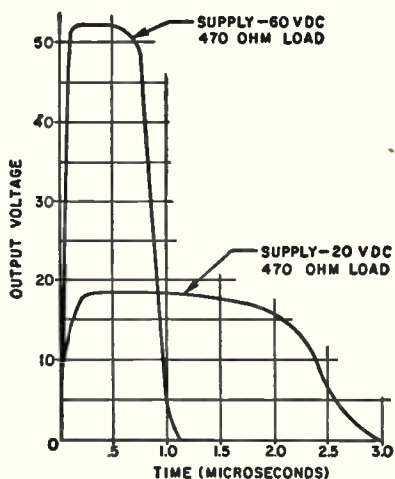
These are typical output curves for the "1PB600" Series "One-Shot" switch, illustrated above.
