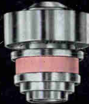
Typical RCA Ceramic-Metal Power Tubes utilize beam power design, and feature high-efficiency forced-air cooling.
