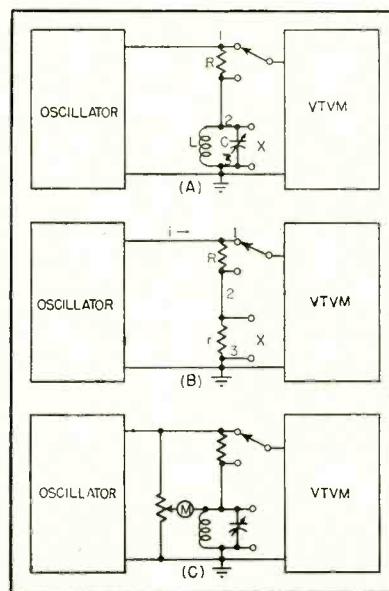
FIG. 1—Development of the admittance-measuring equipment on the basis of a d-c ohmmeter
