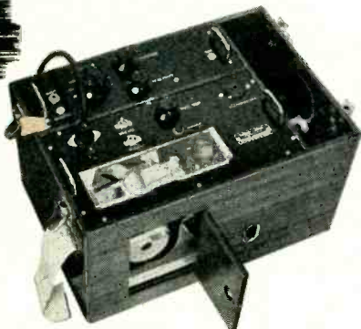
FIG. 3—Panel of the indicator contains balancing potentiometer at lower left and checking switch at lower right
