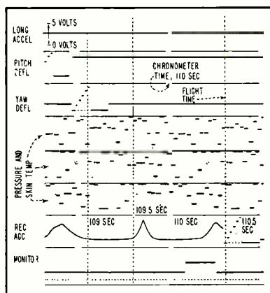
FIG. 7—Typical record of matrix telemetering system
