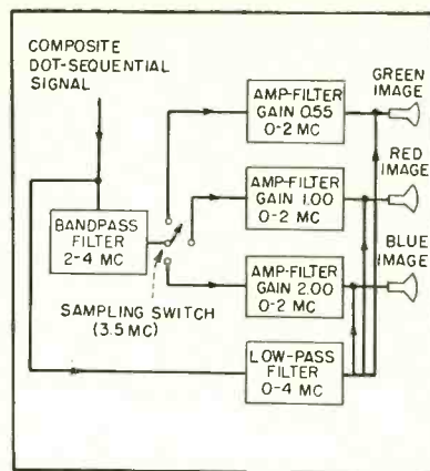
FIG. 2—Circuit arrangement for handling the three color signals
