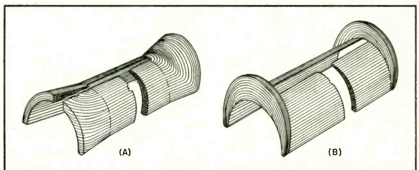
FIG. 2—Cross-section of initial experimental model of cosine deflection coil A and coil actually used in television receivers B
