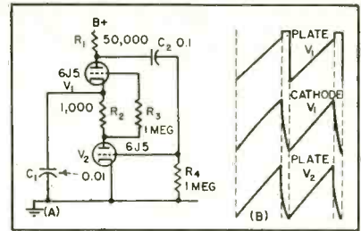
FIG. 1—Basic diagram and voltage waveforms for series sawtooth oscillator
