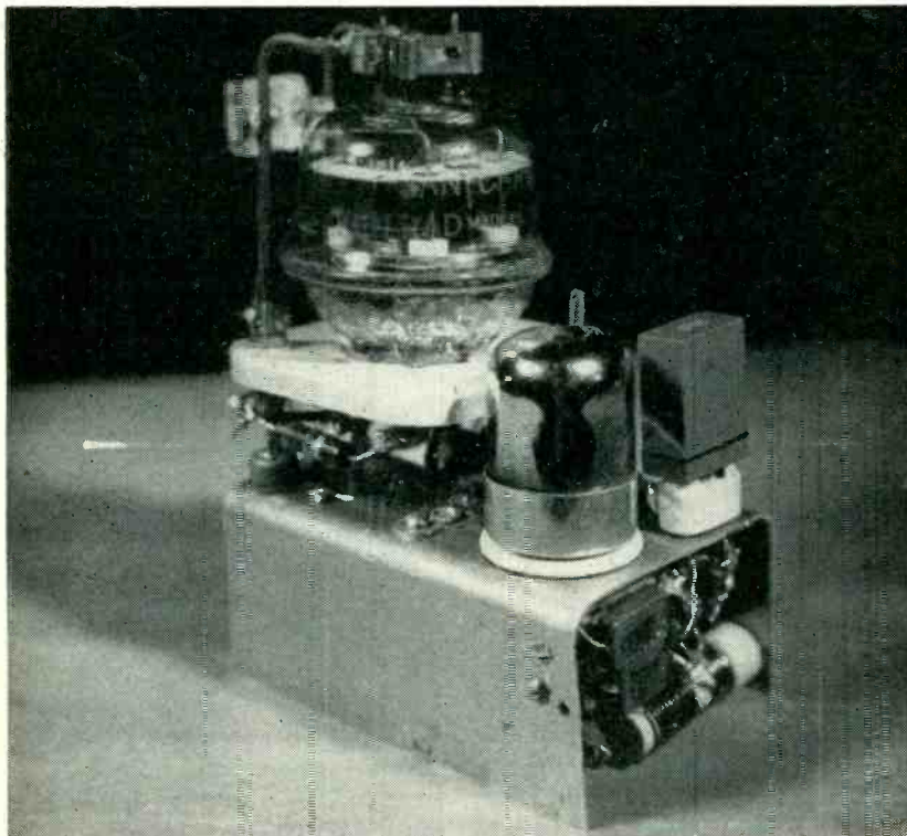
All components of the circuit shown in Fig. 1 are mounted on this small chassis that fits inside the case of the BC-645
