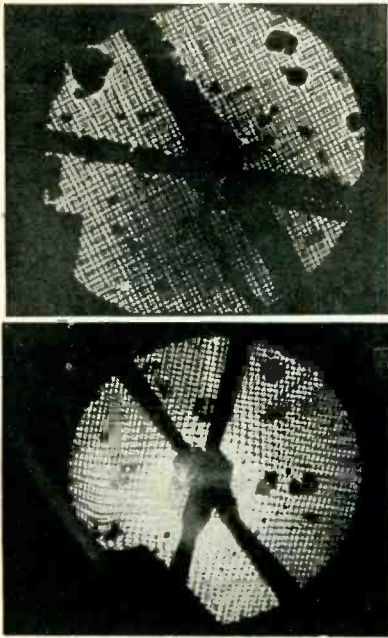
FIG. 3—Photograph at top shows no magnetic field within magnetron. Bottom view shows distortion of shadow network due to magnetic field, and a space-charge ring in central region
