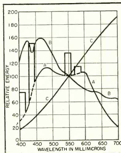
FIG. 2—Spectral energy distribution curves. A 6,500-K daylight fluorescent lamp is represented by curve A. Curve B applies to north skylight and curve C a 500-watt tungsten lamp
