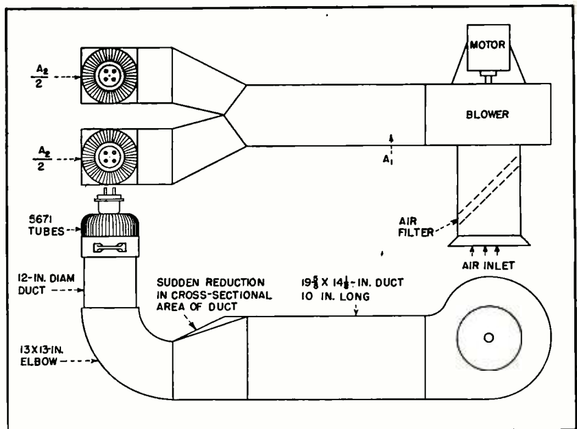
FIG. 7—Typical duct arrangement for cooling two power triodes
