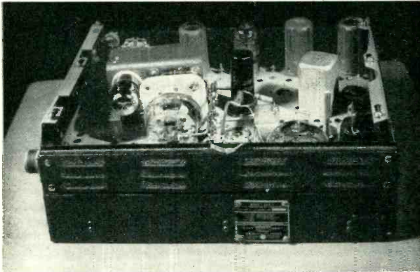
Complete transmitter-receiver for citizens band after crystal exciter has been added. Cover plates cause slight detuning of doorknob grid circuit
