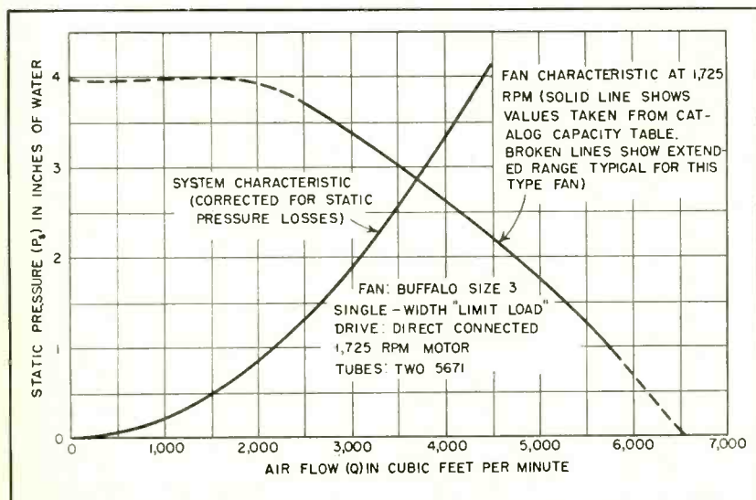
FIG. 1—Fan performance and system characteristic curves
