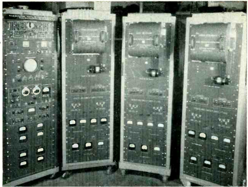
FIG. 2—Receiving station equipment employs direct video recording on continuous film strips
