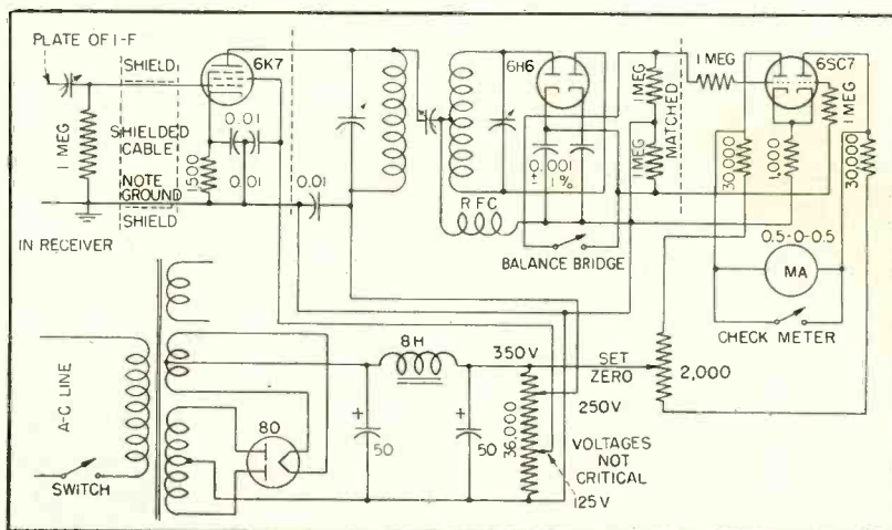
FIG. 1—Circuit of tuning indicator forms a complete unit that can be added to any standard superheterodyne receiver
