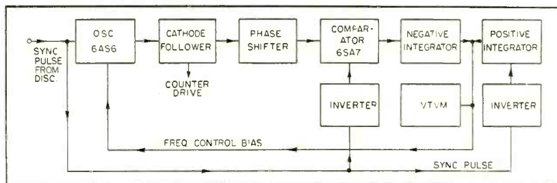
FIG. 6—Block diagram of receiving station matrix oscillator
