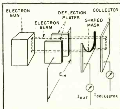
FIG. 1—Functional schematic of the beam-deflection tube
