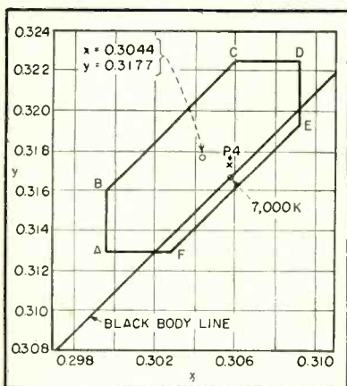
FIG. 4—JETEC specification for neutral filter face-plate glass
