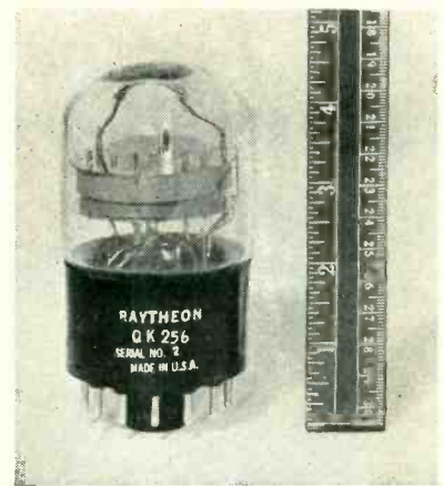
FIG. 2—Beam-deflection tube for squaring 40-mc pulses
