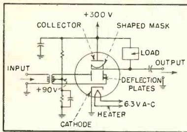
FIG. 4—Schematic of squaring amplifier circuit
