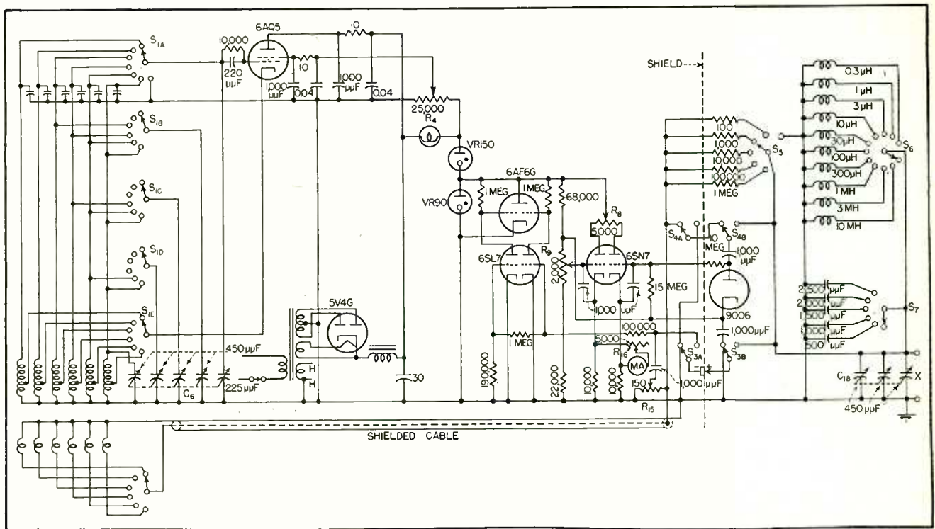
FIG. 2—Circuit diagram of the admittance meter. Oscillator portion at the left is connected to the measuring circuit by a shielded cable
