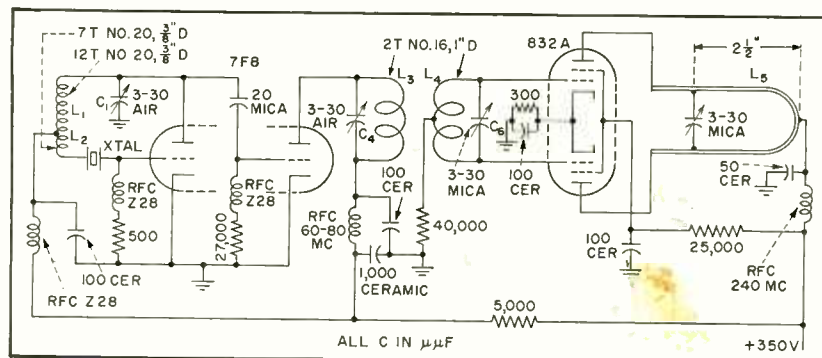
FIG. 1—Circuit of exciter unit added to BC-645. Coil L_1 is spaced the wire diameter and the others are closewound. A six-inch length of \frac{1}{8} -inch copper tubing is connected to each plate of the 832-A to form L_5 .
