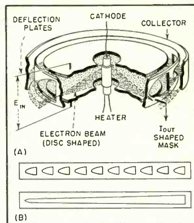
FIG. 3—Cutaway view of beam-deflection tube and equivalent mask shapes
