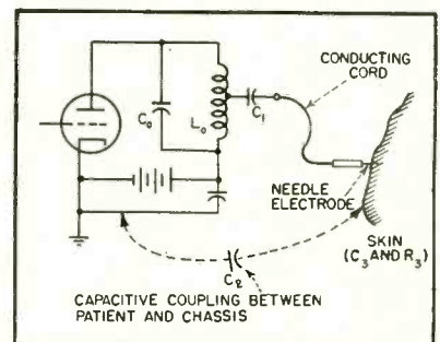
FIG. 1—The r-f pulse is conveyed by a single-conductor cord. Capacitive coupling provides the return path
