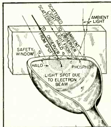
FIG. 1—Exaggerated view of picture tube and safety window shows effects of ambient light and halation
