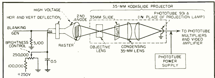
FIG. 5—Small transparencies can be accommodated by employing the optical system of a 35-mm projector backwards, with the phototube in place of the usual lamp
