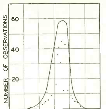
PER CENT ERROR, TYPE 105-A MICROMETER FREQUENCY METER
