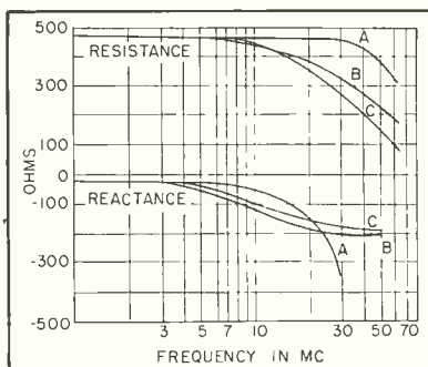
FIG.1—Resistance and reactance characteristics of MPO-17 resistor
