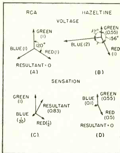
FIG. 1—Vector relations of voltage and visual sensation for the two systems. Angle blue-red is 105 degrees
