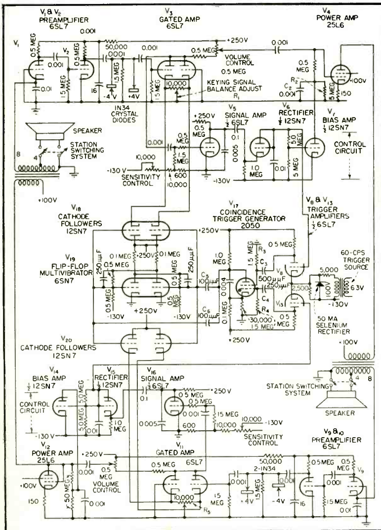
FIG. 2—Amplifiers and control circuits. Power supplies and station-switching arrangements are conventional hence not shown
