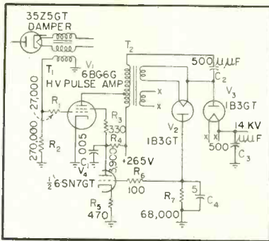
Regulated high-voltage power supply utilizes ringing current in primary of T_2 .
