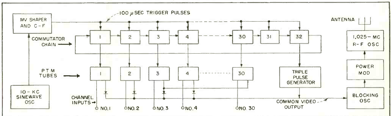
FIG. 3—At the transmitter, timing intervals are initiated by a 10-kc oscillator
