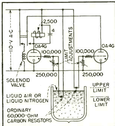
FIG. 1—Circuit diagram of low-temperature liquid level control
