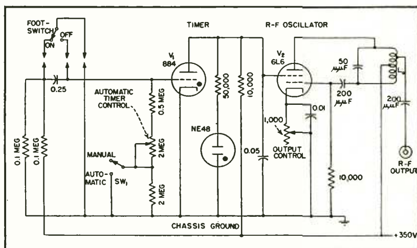
FIG. 3—Schematic of oscillator and automatic pulse timer which resembles those used in electronic exposure controls for photography
