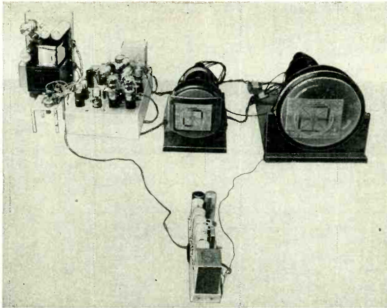
The phototube and video amplifier chassis faces test transparency on the face of the transmitting crt. For demonstration purposes the monitor picture tube at right is fed deflection currents and high voltage from the sweep chassis
