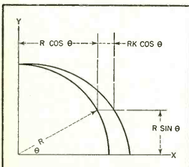
FIG. 1—Geometry of potential theory on which the yoke design is based
