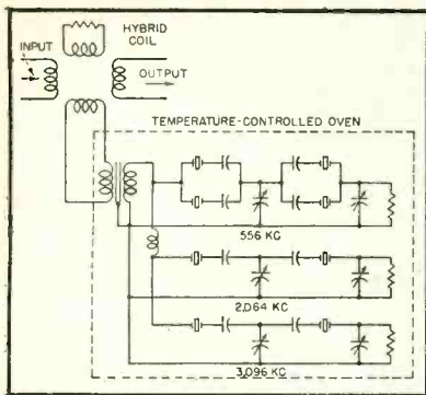
FIG. 3—Filter for elimination of pilot tones at three frequencies
