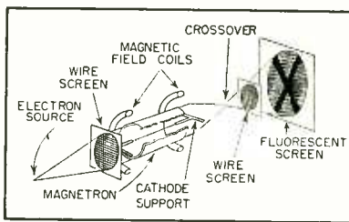
FIG. 1—Perspective drawing illustrates principle of new electron-optical technique for mapping electric-field distribution within a magnetron
