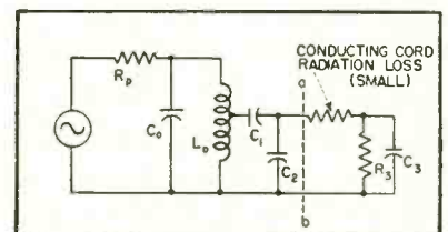
FIG. 2—Portion of equivalent circuit to right of line a-b represents the load on the r-f oscillator
