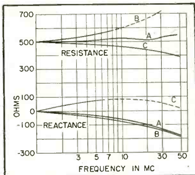
FIG. 3—Resistance and reactance characteristics
