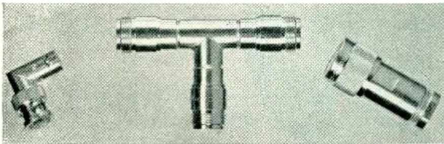
Three types of coaxial connectors for use on frequencies up to 10,000 megacycles using Teflon as the dielectric—Courtesy Industrial Products Company, Danbury, Conn.
