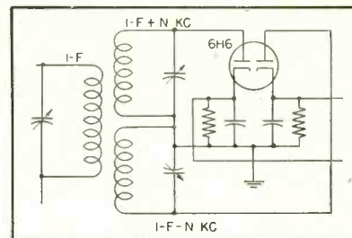
FIG. 2—For special applications, such as telemetering and telecontrol, the Doppelganger discriminator may be more useful
