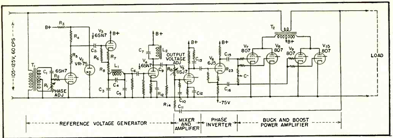
FIG. 2—Simplified schematic showing arrangement of reference generator, amplifier, inverter and buck-boost amplifier
