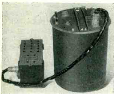
FIG. 1—Transmitting equipment weighs 130 pounds, with batteries, and produces 4 kw peak power at 1,025 mc
