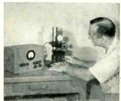
FIG. 1—Ceramic thickness gage gives direct, nondestructive measurements of thickness of nonconducting coatings on nonmagnetic metals
