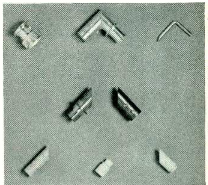
Right-angle connector showing component parts and mitered sections before silver soldering and plating. Teflon dielectric is shown at bottom—Courtesy Industrial Products Company, Danbury, Conn.
