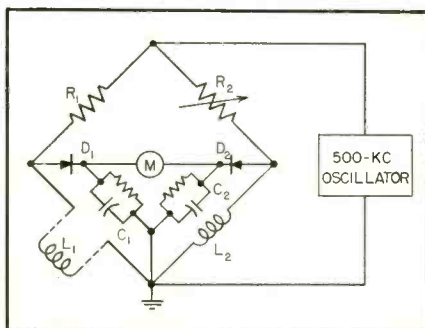
FIG. 2—Simplified schematic of inductance bridge used in ceramic thickness gage
