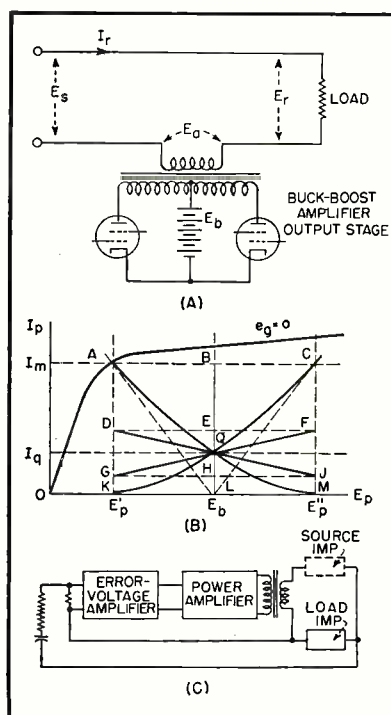
FIG. 3—(A) Load circuit of the regulator. (B) Load lines corresponding to types of operation outlined in text. (C) The feedback loop comprises error-voltage amplifier, p-a, and the circuit network, which has three elements
