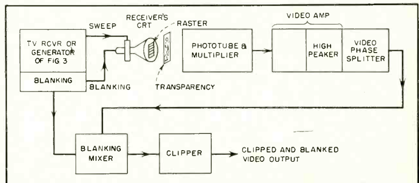
FIG. 1—Stages of the picture-generating system. The video output can feed the video stage of a conventional receiver or modulate an r-f signal generator
