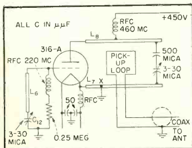
FIG. 2—Final stage of the transmitter after modification. Inductor L_6 couples to L_5 of Fig. 1
