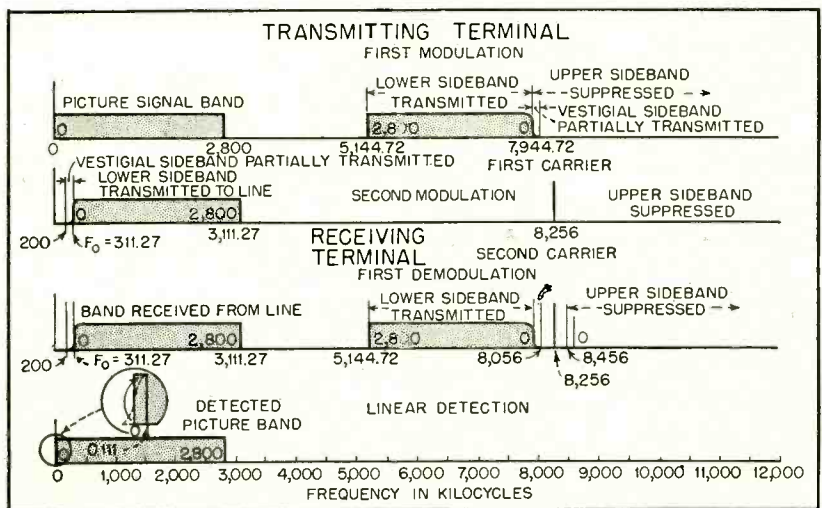
FIG. 2—Modulation diagram for television carrier terminals
