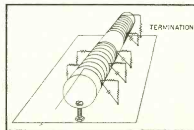
FIG. 2—Distributed-constant resistor approximate a lossy distortionless line
