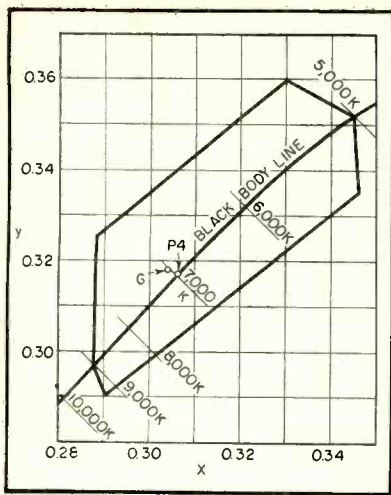
FIG. 3—JETEC color limits for P4 white phosphor
