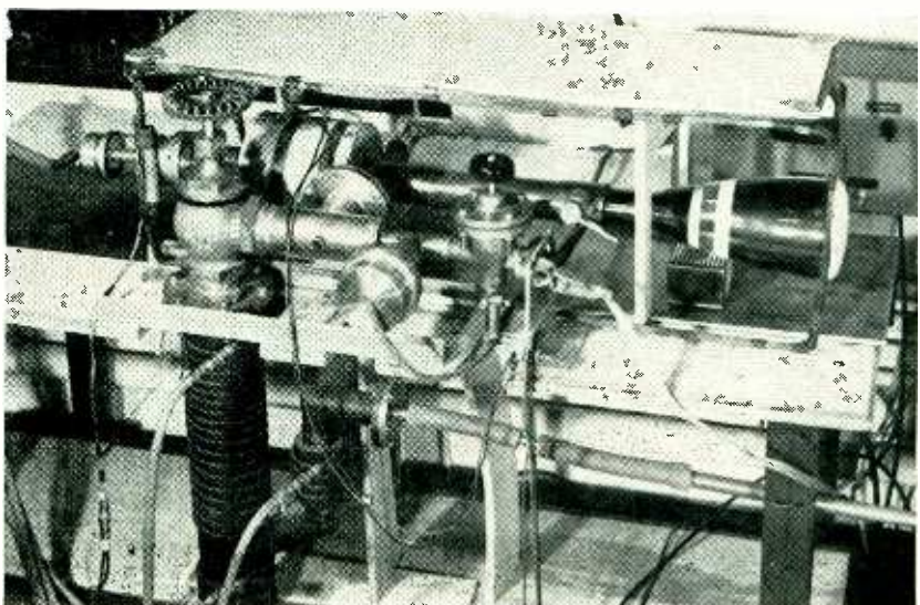
FIG. 2—Special cathode-ray tube setup for field-mapping equipment
