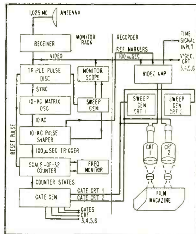
FIG. 5—Matrix receiving equipment must be kept in both frequency and phase synchronism with transmitter timing oscillator
