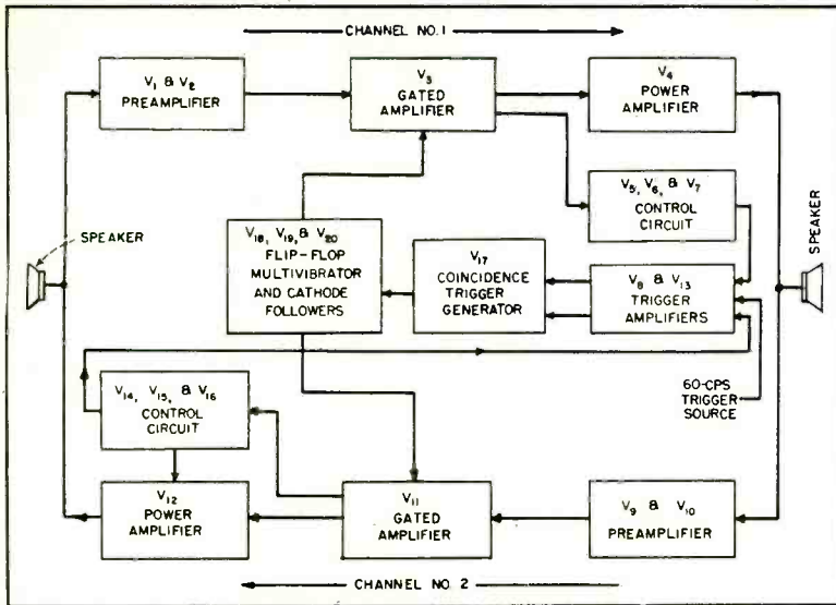
FIG. 1—Twenty stages, some using halves of dual-function tubes, keep either channel open as long as voice signals are present and permit other channel to take over quickly at end of message
