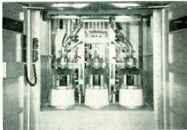
Tube end of system using ducts to radiators and to filament connections
