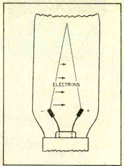
FIG. 1—Edison effect in an incandescent lamp with V-shaped filament
