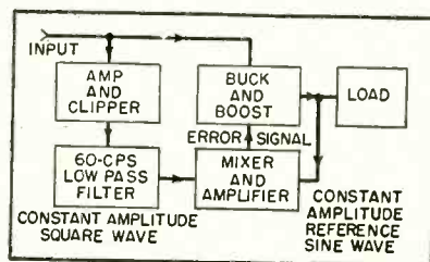
FIG. 1—Elements of the 60-cycle voltage regulator
