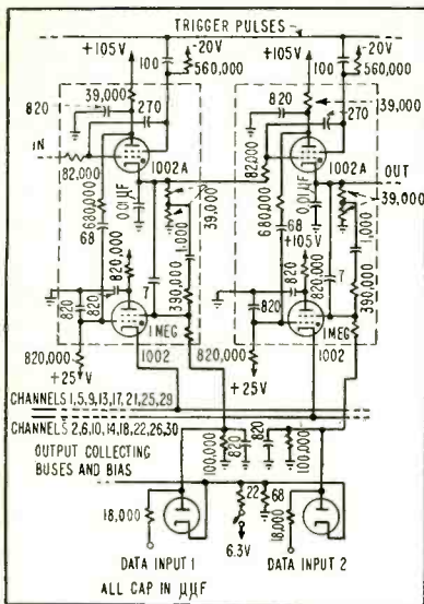
FIG. 4—Two typical stages of the 30-channel chain and pickoff circuits
