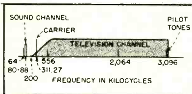
FIG. 1—Television allocation for L-1 coaxial system
