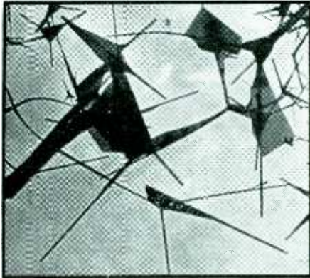
Zinc smoke particles consist of four fine spikes joined together. \times 10,500
