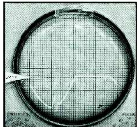
Fig. 5—Firing tube grid voltage when not firing
