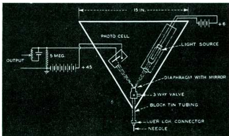
Fig. 7—Circuit of a device for making an accurate record of the pressure changes in the cardiovascular systems of animals such as the dog and turtle
