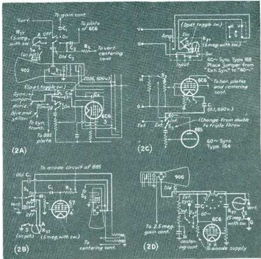
Fig. 2—Oscilloscope circuit modifications suggested for electronic welding control maintenance work. Heavy lines show new connections, light lines show original connections. (2A) RCA types 151, 151A and 151-2. (2B) RCA types TMV-122B and D. (2C) DuMont types 164 and 168. (2D) G.E. type OFM-3
