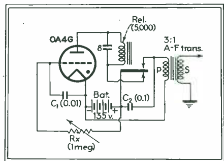
Fig. 2—Arrangement for higher output
