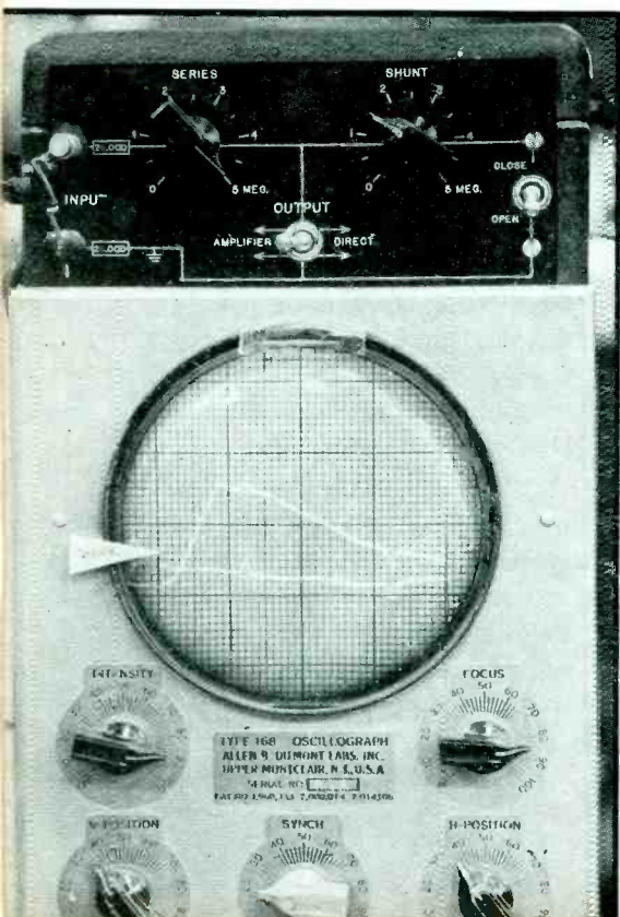
Fig. 1B—The trace on the screen of the cathode-ray tube in this instance is useful only for determining variation of the "off" time a-c bias. D-c bias component is inaccurately illustrated because, for purposes of illustration, the input voltage was incorrectly applied through the instrument's a-c amplifier
