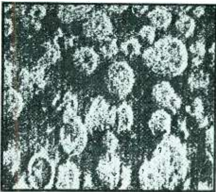
Micrograph of slightly annealed brass made with the scanning microscope. \times 3500
