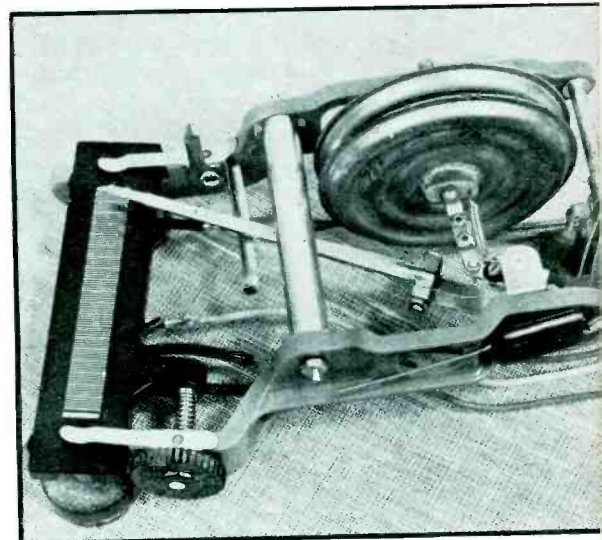
The pressure switch. This connects the transmitter to the temperature tube when the contact rests on an insulator between silver segments; to the humidity potentiometer when the contact is on one of the thin silver segments, or to fixed reference resistors when contact is made with a thick segment
