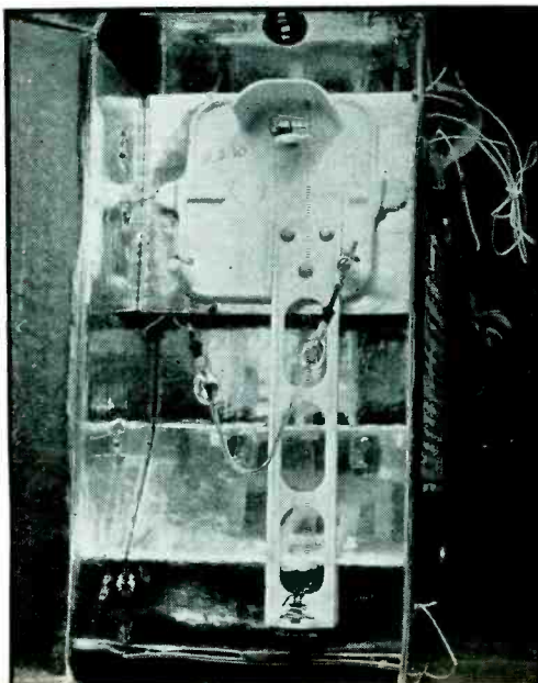
Temperature tube and hair hygrometer. The radiation shield has been removed. The outer box is covered with metal foil to reduce solar heating
