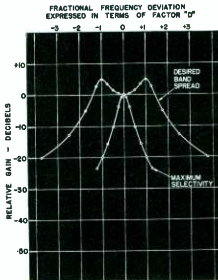
Fig. 6—Calculated universal resonance curve of matched two resonant circuit transformer network
