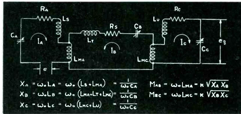
Fig. 3—Three resonant circuit network with common resistance coupling
