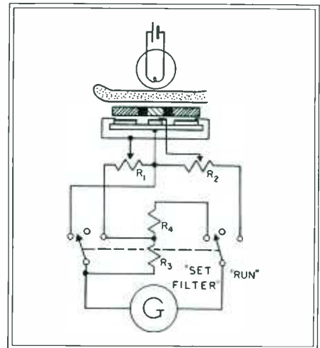
Fig. 3—Circuit diagram of single scale oximeter, with automatic adjustment for ear thickness
