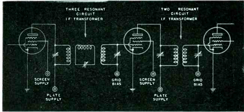
Fig. 1—Schematic wiring diagram of two stage amplifier containing a three resonant circuit network and complementary two circuit network for providing uniform response in the pass band
