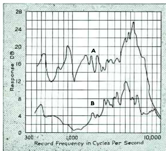
Fig. 7—Characteristic labeled A is record noise from a conventional pickup of the replaceable needle type. Characteristic labeled B represents the new design
