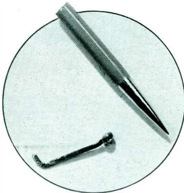
Fig. 4—A comparison of the physical size of the coupling-stylus assembly used in the new pickup with that of a standard needle. The scale is provided by the standard needle which measures 0.068 inches in diameter by 0.625 inches long
