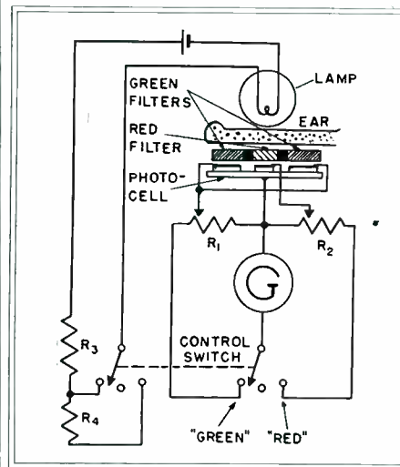
Fig. 1—Schematic wiring diagram for multiple scale oximeter, which, when used multiple scale, permits direct readings to be made of oxygen saturation of the blood
