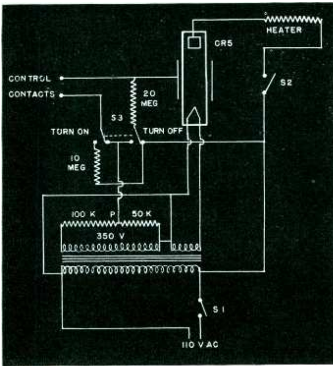
Fig. 1—Electronic relay used for temperature control. Employs a tube with an external control element
