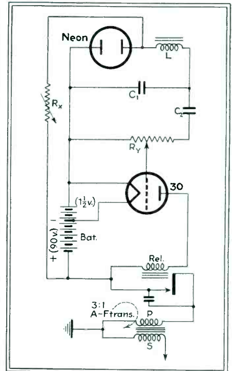
Fig. 6—Battery operated relaxation type timer using high vacuum tube
