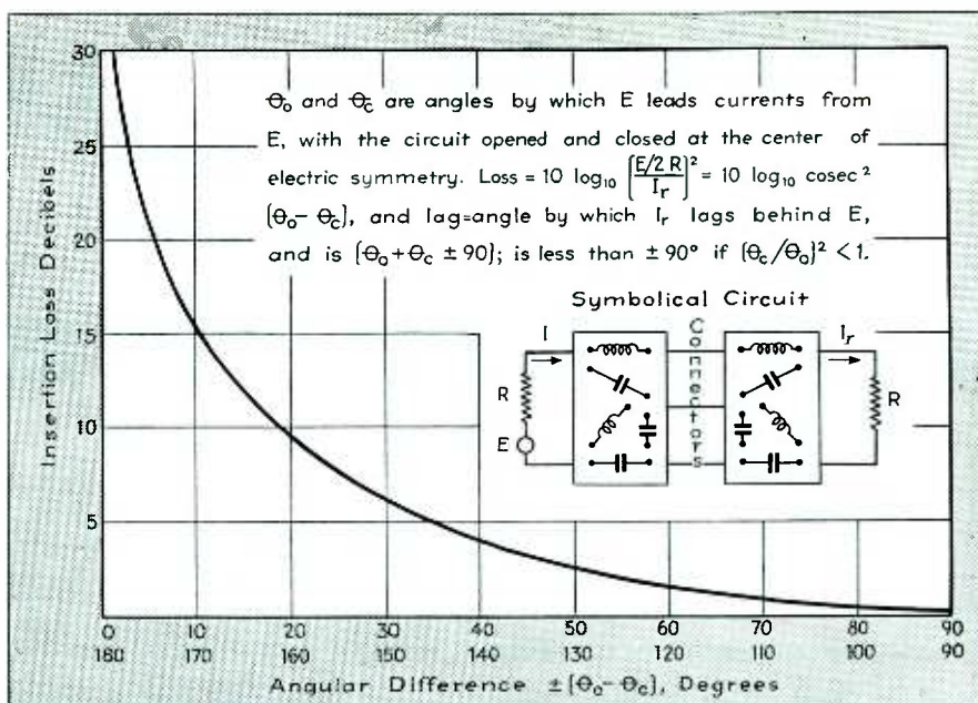
Fig. 2—Loss and lag characteristics for bisectable R - X circuits
