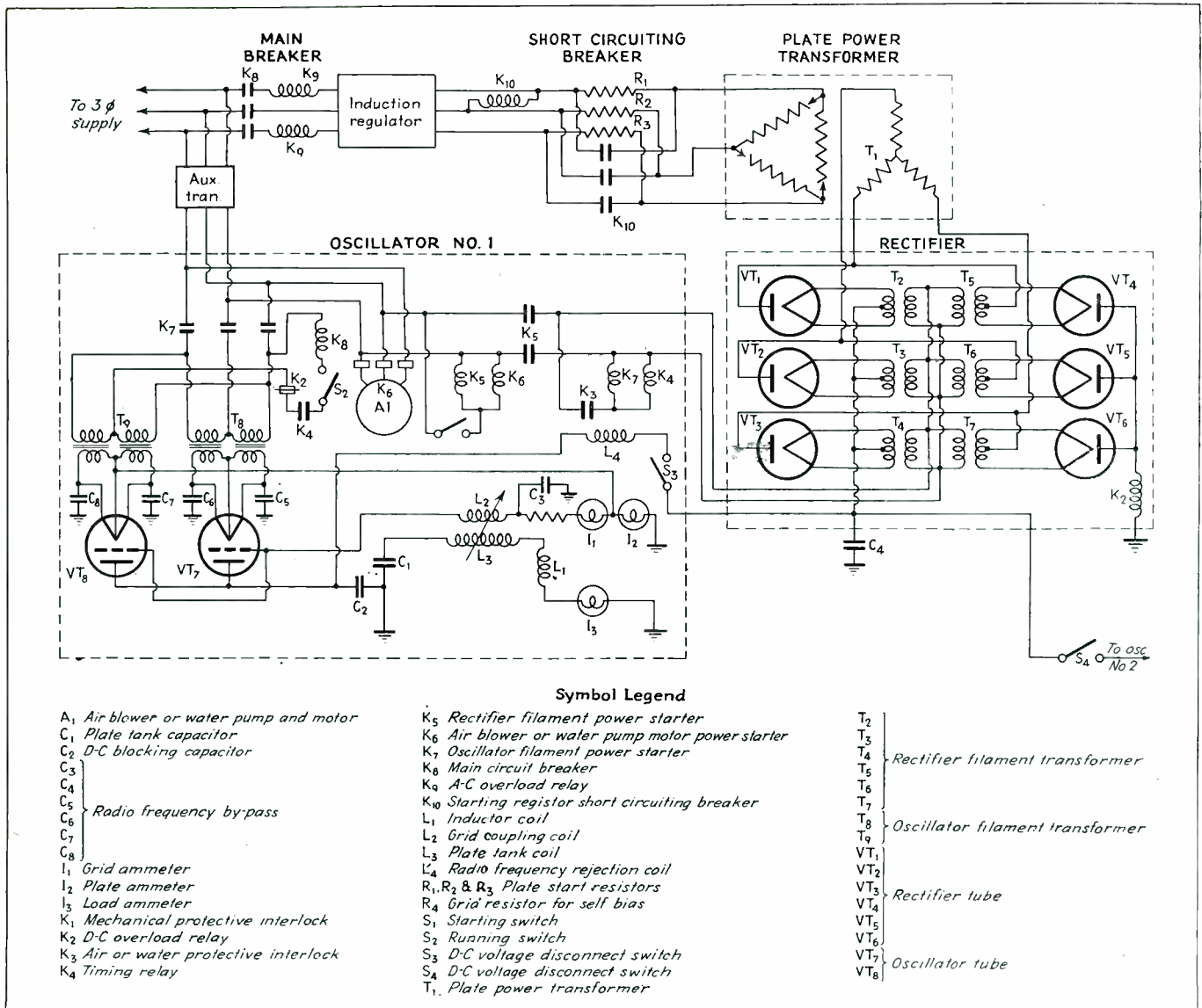
Fig. 1—Schematic diagram of electronic high frequency heating oscillator
