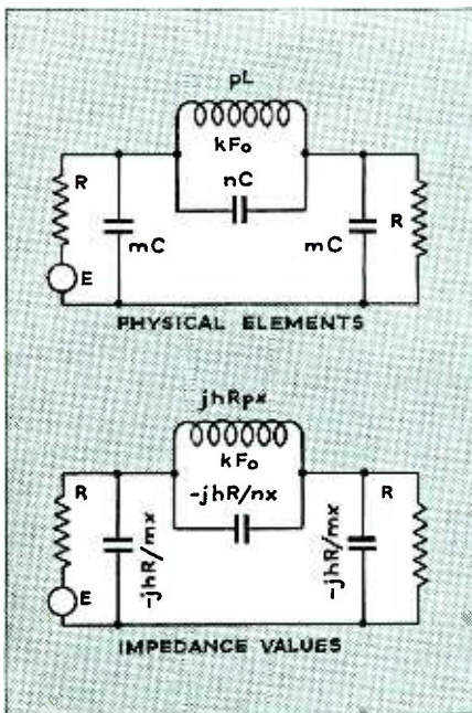
Fig. 3—Circuit designations showing relation between physical elements and impedance values
