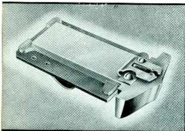
Fig. 5—The bottom view of the complete pickup assembly. A guard will be observed which serves to protect the stylus and coupling against damage
