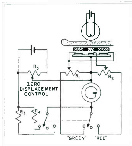
Fig. 2—Schematic wiring diagram of single scale oximeter with manual adjustment
