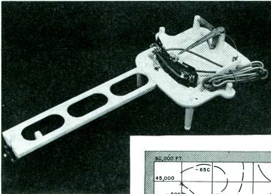
The hair hygrometer before assembly, showing potentiometer. A clear plastic cover that protects the potentiometer from moisture and dirt is not shown
