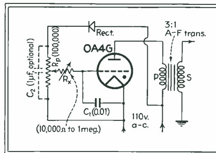
Fig. 3—Pulse generator operated from a-c line
