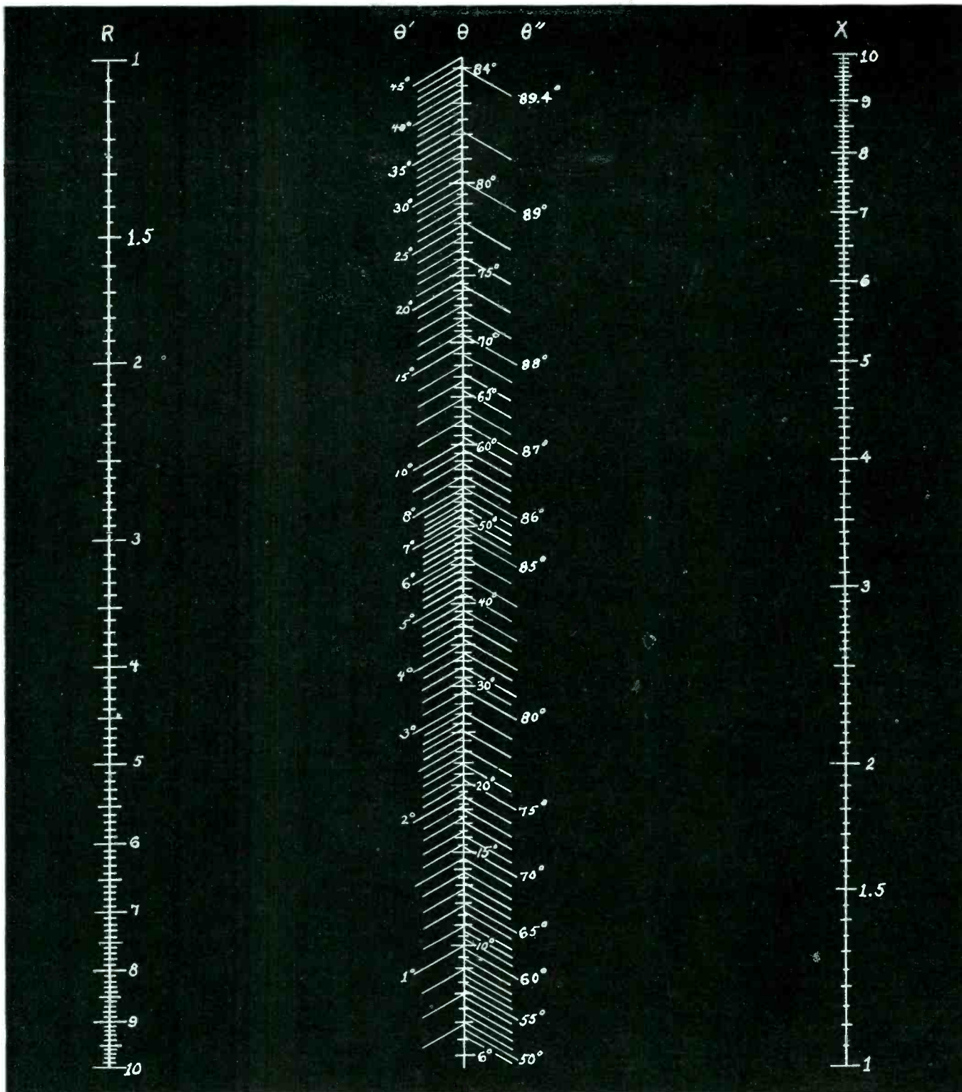
IMPEDANCE MAGNITUDE ALIGNMENT CHART
