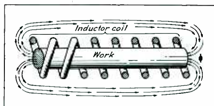
Fig. 2—Diagram of inductor heater coils with lines of magnetic flux
