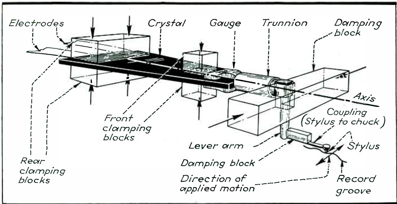
Fig. 1—Schematic illustration of the pickup described in this paper. For clarity, the case and tone arm are omitted
