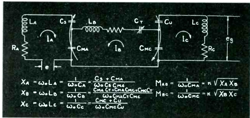
Fig. 4—Three resonant circuit network with common capacitance coupling
