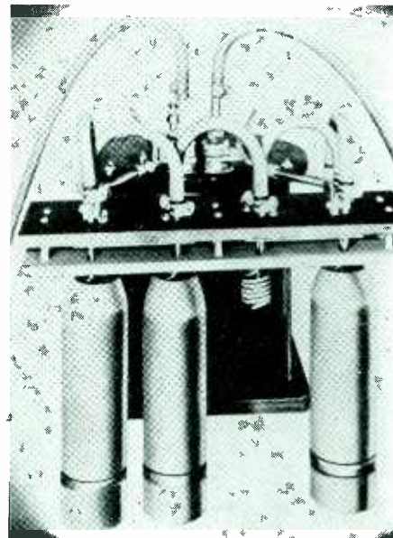
"Business end" of r.f. induction heating unit designed to anneal shell noses. Three shells are shown in place on the four-unit jig. An applicator coil may be seen in the open position
