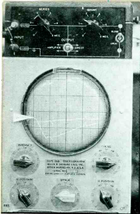
Fig. 1A—Trace showing normal "off" time bias on a typical electronic welding control inverter tube. In this instance, input voltage was correctly applied directly to the vertical deflecting plates of the oscilloscope's cathode-ray tube to accurately picture both a-c and d-c bias components
