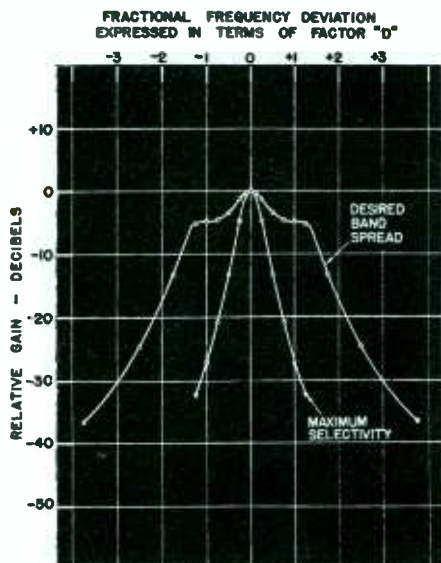
Fig. 5—Calculated universal resonance curve of critically coupled three resonant circuit network
