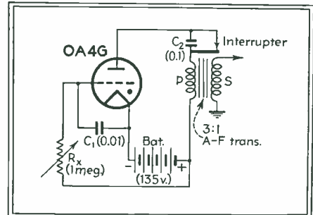
Fig. 1—Simple pulse-generating circuit
