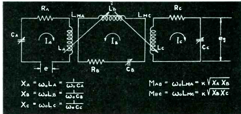
Fig. 2—Three resonant circuit transformer with mutual inductance coupling
