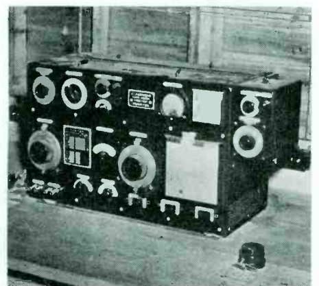
This Japanese short-wave transmitter was found by the U. S. Marines on Guadalcanal in the Solomon Islands after it had been abandoned by the retreating enemy during the early stages of the fighting
