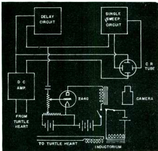
Fig. 3—A phototube myograph, a device for recording muscular contraction
