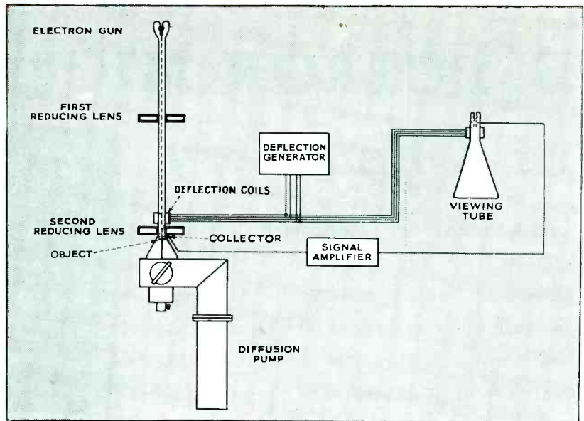
Simple scanning microscope for continuous observation
