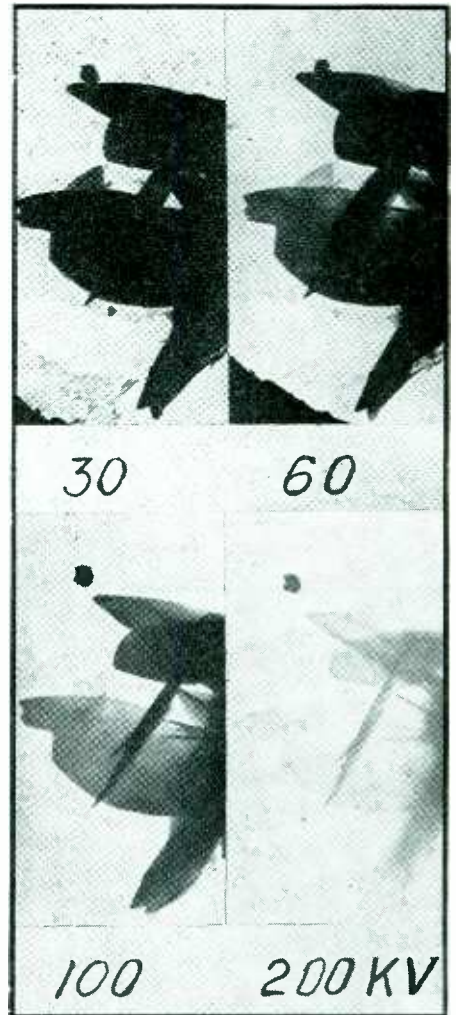
Effect of varying voltage on the electron microscope. Aluminum oxide monohydrate (diaspore) scales taken at 30 to 200 kv. \times 5500
