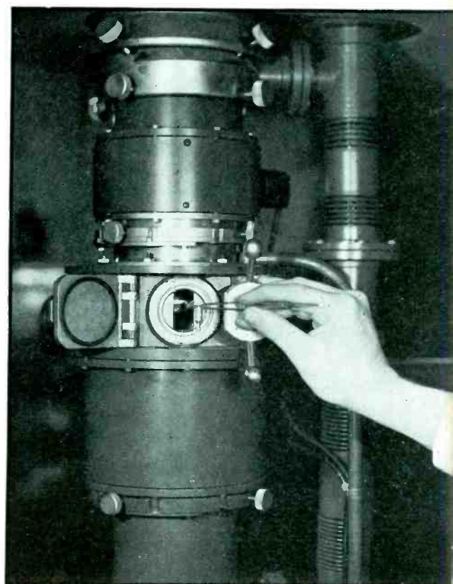
Method of introducing the object cartridge into the electron microscope (below)
