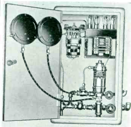
Fig. 2—In this particular control a pressure-sensitive device (lower right), operating a single make-break contact and four thyatron tubes (upper right) operate two a-c motors on a common shaft (upper left) in such a manner that steam pressure is kept at a selected critical value
