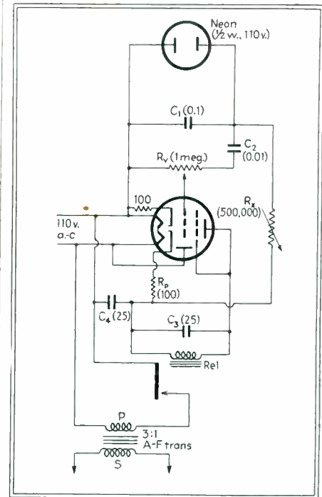
Fig. 5—"Relaxation" type timer using high vacuum tube
