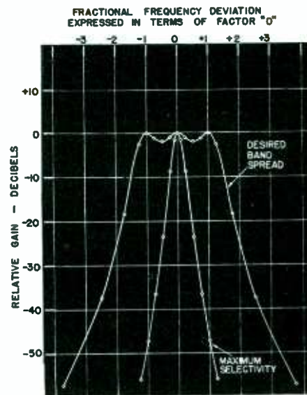
Fig. 7—Calculated resultant universal resonance curve for two and three resonant matched transformer networks
