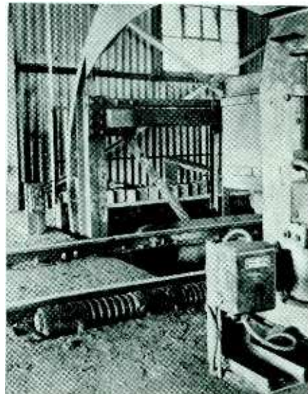
Exit end of rotary dump for coal cars, controlled by a phototube
