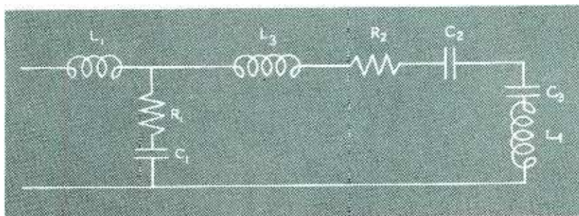
Fig. 3—Equivalent circuit of pickup for high-frequencies. This simplification is justified as the value of L_2 is many times the value of associated elements
