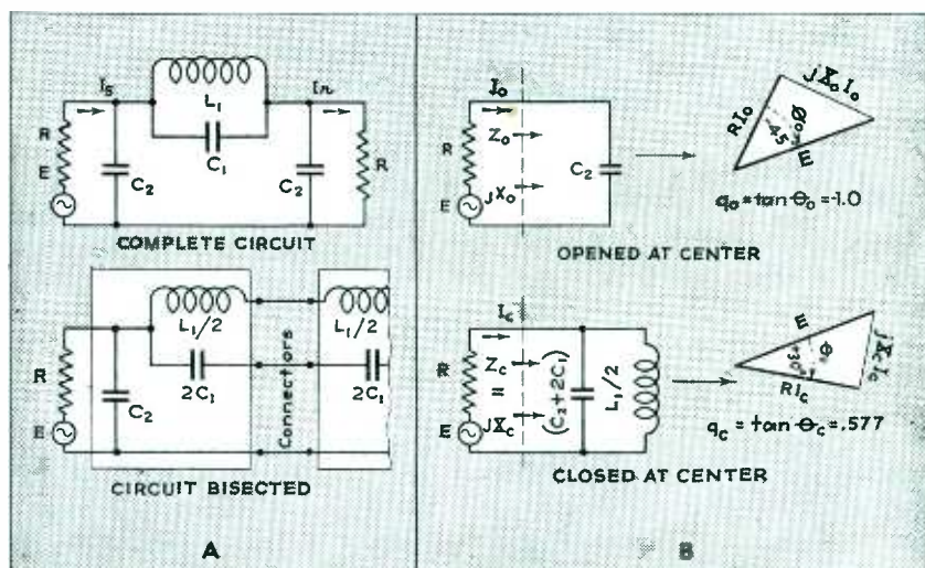
Fig. 1—Bisectable reactance networks with equal resistance terminations
