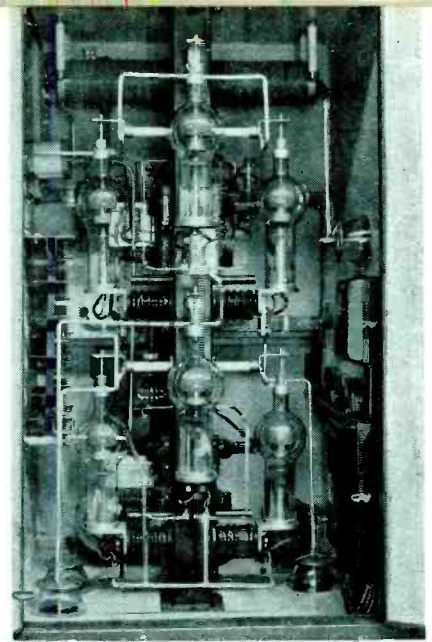
Electronic rectifier in which the alternating current is converted into direct current
