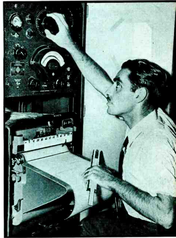
Equipment for receiving and recording the signals from Diamond-Hinman radiosonde. At top is a super-regenerative receiver; below it an electronic audio frequency meter and at the bottom a recorder which makes a record of the frequency meter readings
