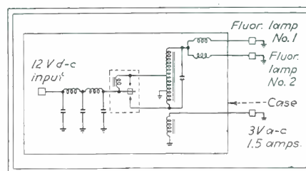
Circuit showing method of using vibrator type d.c. to a.c. inverter for operating aircraft fluorescent instrument lamps
