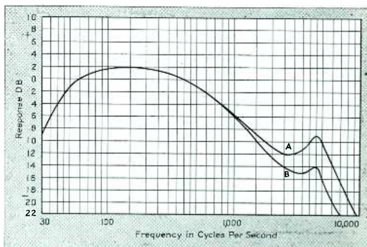
Fig. 8—The voltage-frequency response of the new design. The characteristic labeled A is normal and that labeled B is with the coupling (stylus-to-chuck) damping block removed
