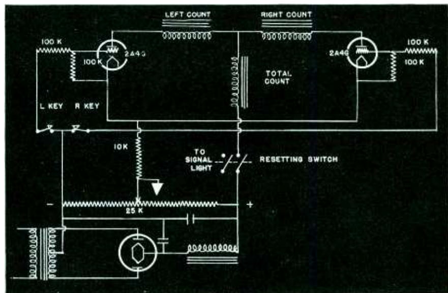
Fig. 2—A precedence indicator tells the investigator which of two contacts opened first
