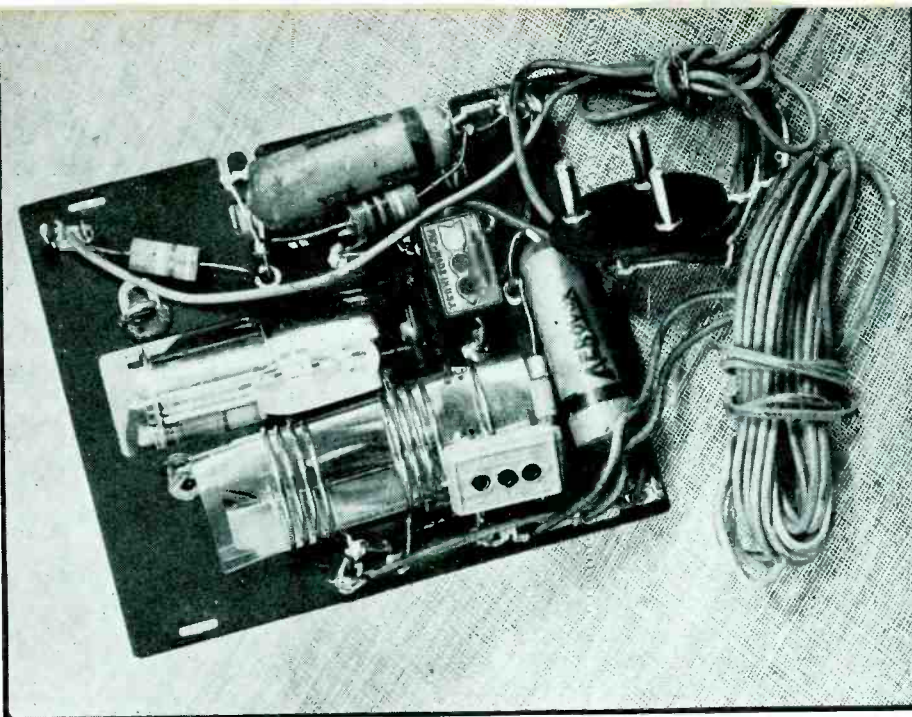
The transmitter. The carrier frequency is 72.2Mc, and the power output about 150 milliwatts
