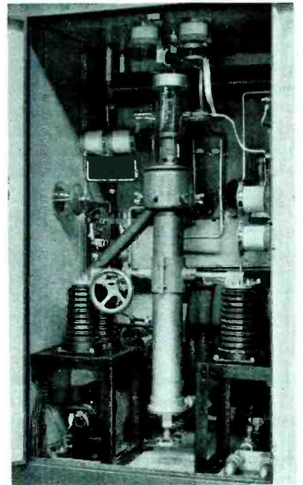
Water cooled oscillator tube (above and tank circuit (below) for generating power at 200 k.c.
