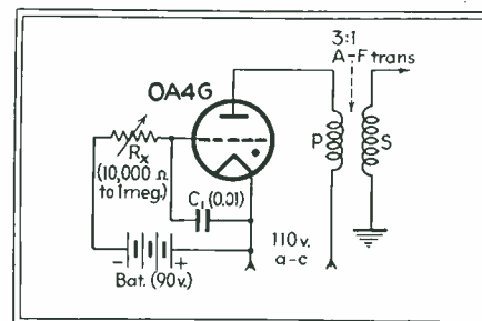
Fig. 4—Modification using battery to avoid timing changes with line voltage variations
