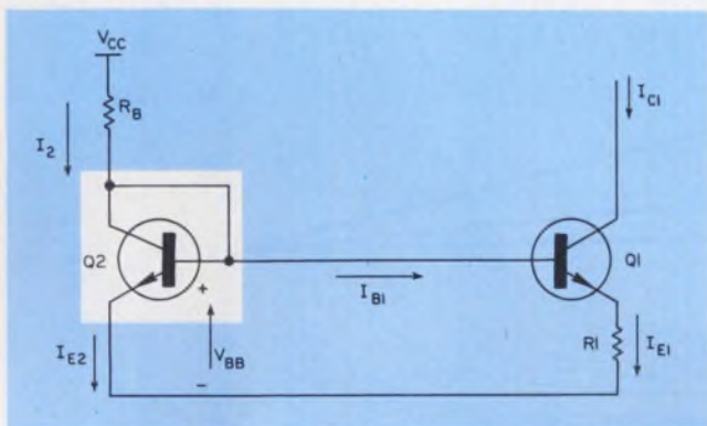
4. Transistor Q 2 , configured as a diode, provides bias for Q 1 . As a result, I E2 depends little on I E1 , especially when I E2 >> I E1 and Q 1 and Q 2 have identical characteristics.
