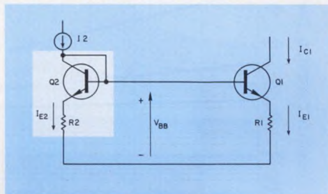
5. The so-called current mirror is the most popular current-source (or sink) configuration. It is designed around a resistor-diode-biased transistor pair.
