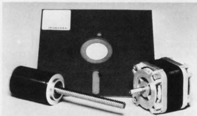
A lead screw attached to the motor shaft in these steppers from Eastern Air Devices is used to convert rotary motion to linear motion for floppy-disc applications.
