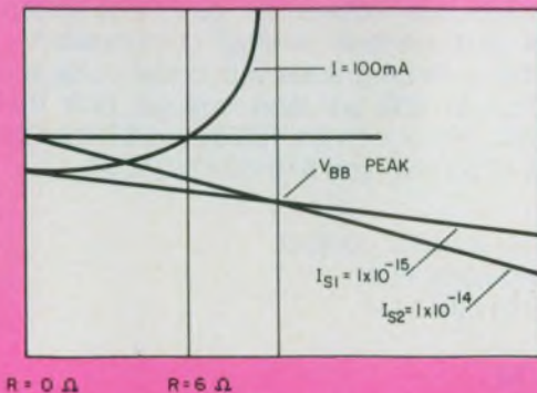
8. Emitter resistances of 6 \Omega equalize emitter currents at 100 mA for unequal transistors in parallel.
