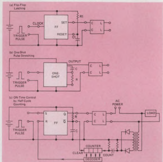
1. Many approaches can be used to hold or "stretch" narrow pulses for properly operating SSRs from logic-system inputs. A set-reset latch flip-flop (a), a one-shot multivibrator (b) or a binary counter (c) are some of the more common methods.
