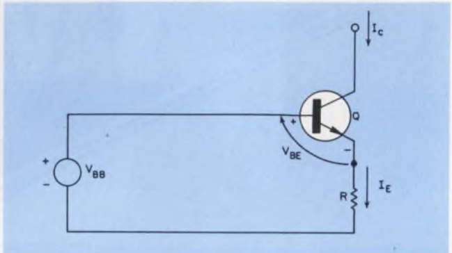
1. A resistor-diode circuit, the building block of current mirrors, consists of the resistor, R , and the diode of the transistor's base-emitter junction. Important variables are V_{BB} , V_{BE} , and I_E .
