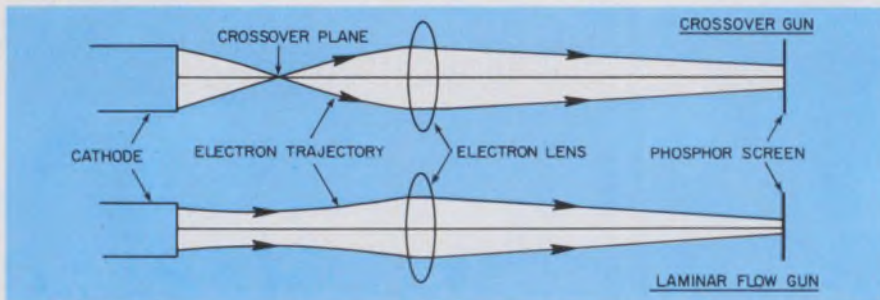
1. The differences between the Watkins-Johnson laminar-flow electron gun and the traditional crossover gun is apparent in the diagram.
