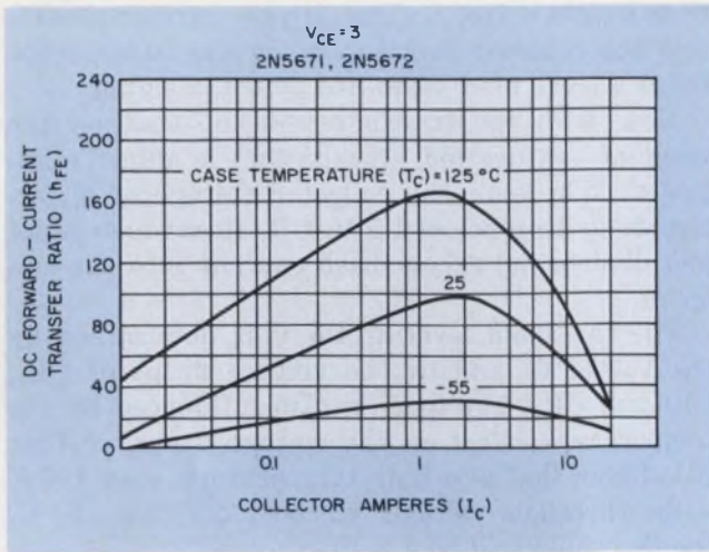
1. As temperature goes up, so does transistor gain. The resulting higher beta produces excess base-drive current, and so significantly boosts storage time. At low temperatures, a reverse effect occurs.
