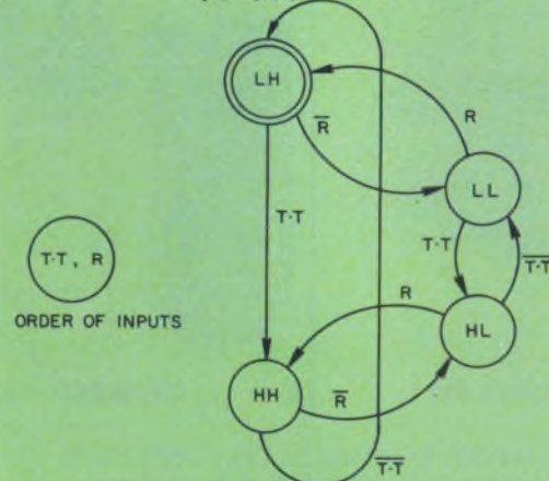
3. When the TR and TH inputs are connected, they form the combined input labeled T·T, and a simplified state diagram results.
