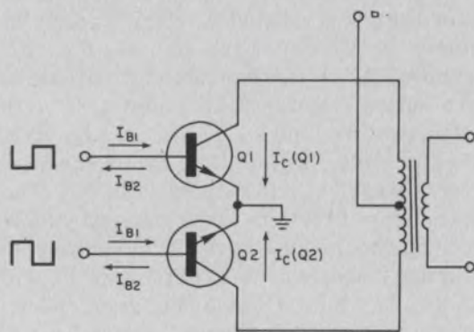
PUSH-PULL CONVERTER
