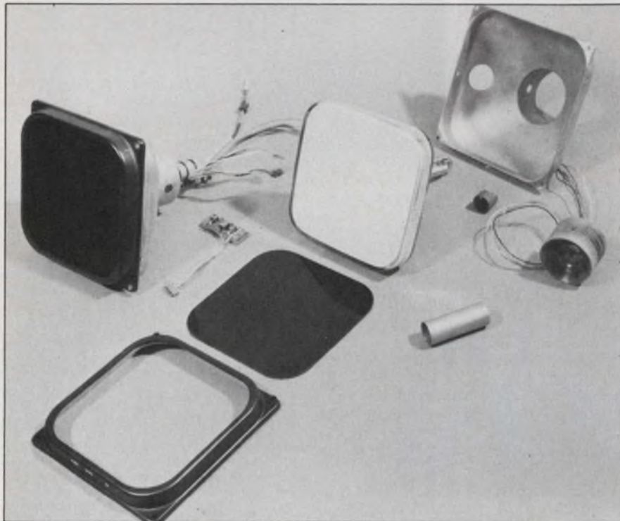
For displays subject to severe environmental conditions, the trend is toward integrated CRT assemblies in which the deflection yoke is prelocated on an electrostatic-focus CRT. Shown are the components and CRT for a ruggedized airborne display made by Raytheon's Industrial Components Operation, Quincy, MA.
