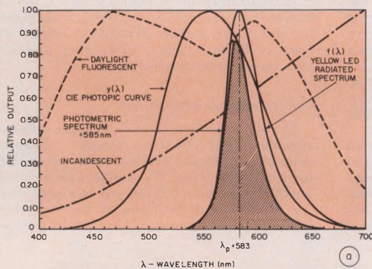
9. Yellow LEDs emit a spectrum that is fairly close to the eye's relative response (a). The peak of the LED is
