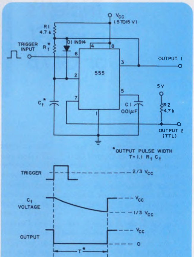
A mirror-image one-shot configuration for the 555 timer provides a negative output pulse for positive input triggering—the reverse polarities of the standard arrangement.
