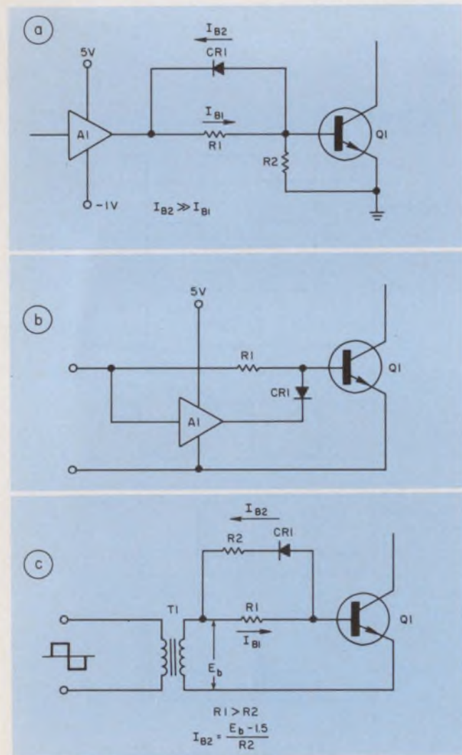
4. Another way to minimize storage time is to get rid of base charges fast. In one variation, a buffer A_1 sinks current to the -1V source (a). In (b) A_1 handles just I_{B2} . Another quick-discharge method uses a transformer to apply a negative pulse during the off period (c).
