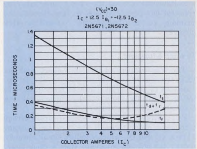
2. Note the drop in storage time as collector current increases, and how large the variations in t_s are compared with other switching parameters. The variations must be accounted for in design.
