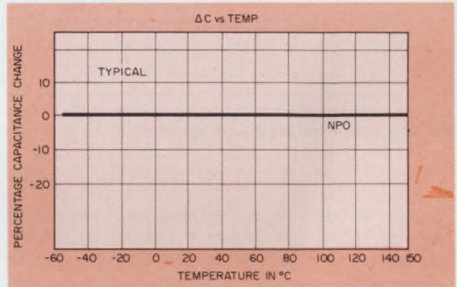
3. Class I NPO dielectric capacitors are available with a guaranteed \pm 30 ppm/°C drift from -55 C to +125 C.
