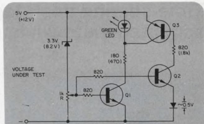
1. A voltage-limit sensing circuit lights a LED when the voltage is within 0.5 V above the limit set by potentiometer R. Values shown in brackets are for 12-V operation.
