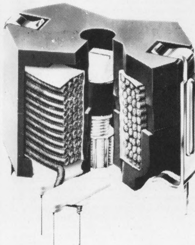
1. A ferrite pot core is completely self-shielding. Thus it eliminates worries about interference with nearby circuit components.
