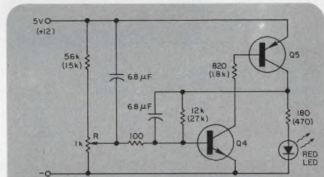
2. Ripple and noise voltages in power supplies can be detected over the range of 10 to 600 mV, peak-to-peak. Sensitivity is adjusted with potentiometer R.
