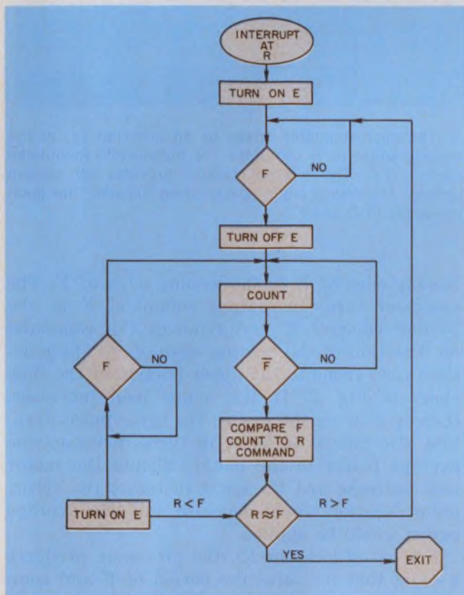
3. A variable-duty-cycle control signal is generated (upper section of program) when R = F to control phase. The lower portion of the program checks for gross frequency error by counting for the duration of clock pulse F and comparing the count with the command value.
