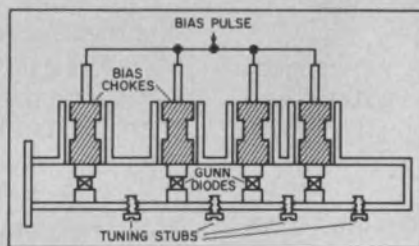
2. Four-diode oscillator produces about 45 W and is tunable over 1 GHz.
