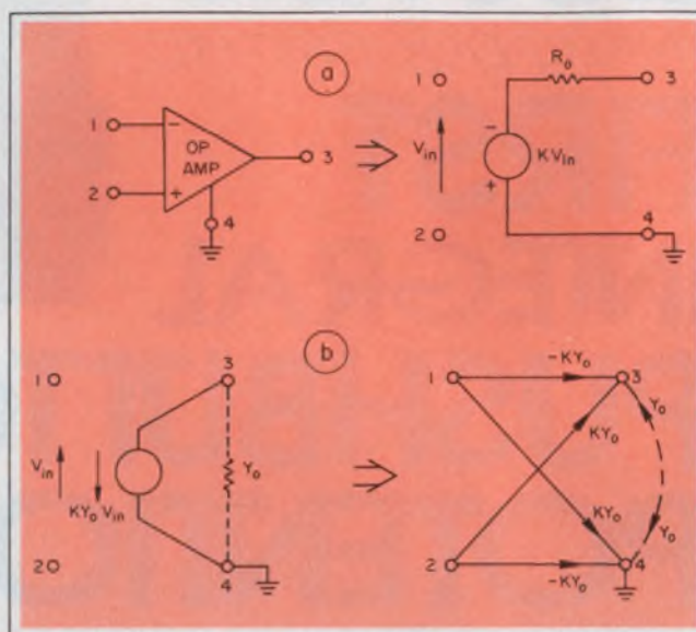
1. The topological graph of an op amp starts with the equivalent circuit (a), which is transformed to a current-source equivalent (b). This model is valid for infinite input impedance and finite output impedance.
