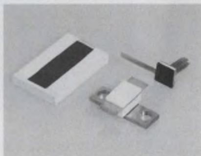
Conduction-cooled microwave resistors and terminations handle up to 100 W. These devices are from Pyrofilm on beryllia substrates.
