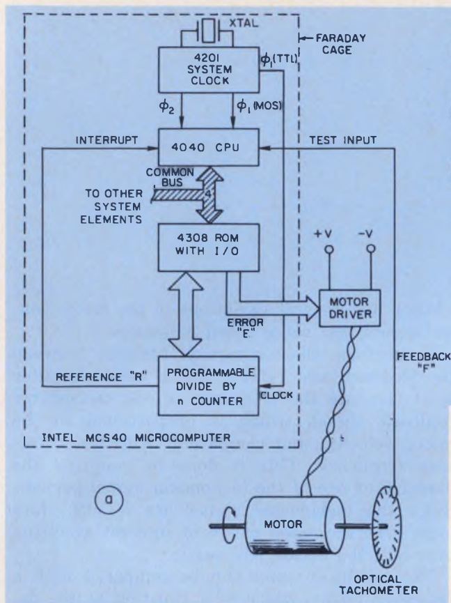
4. The microcomputer driven by an interrupt (a) at the leading edges of R computes the pulse-width-modulated control (b). The internal crystal provides all system timing. The phase angle is measured between the leading edges of R and F.
