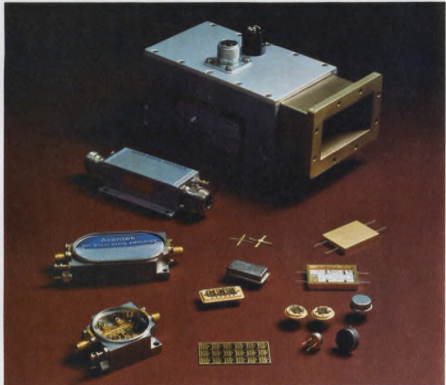
Microwave Integrated circuits come in a wide range of package types. Avantek offers both connector and connectorless packages at frequencies to about 4 GHz. Standard packages are made of welded steel.
