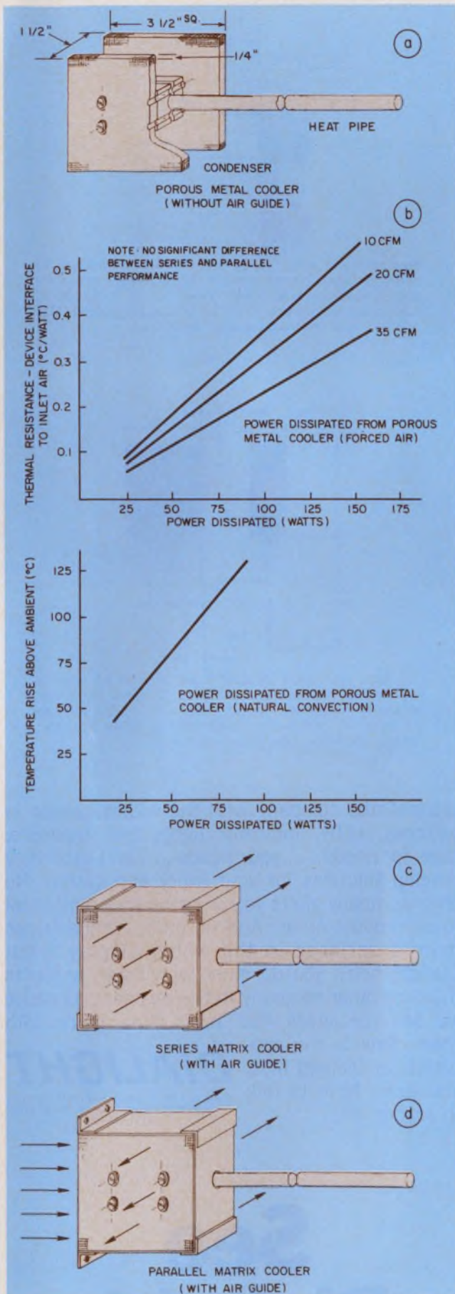
7. A high-performance condenser configuration for a heat pipe (a). There is no performance difference (b) between series (c) and parallel (d) air-flow patterns.
