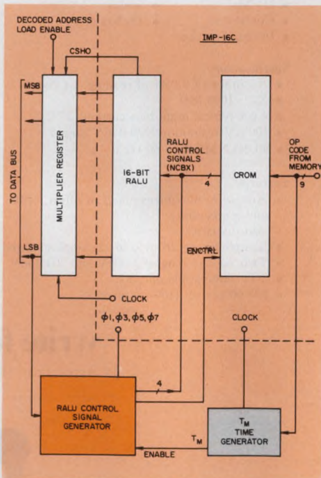
1. In this CPU complementary multiplication circuit, CROM outputs are replaced with special control signals that permit hardware multiplication operations. The additional circuit blocks consist of a time generator, signal generator and multiplier register.
