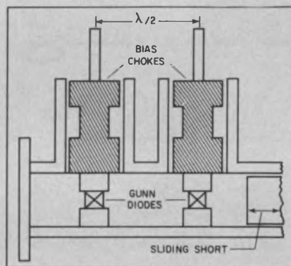
1. Two Gunn diodes in a waveguide structure provide 22-W pulsed output.
