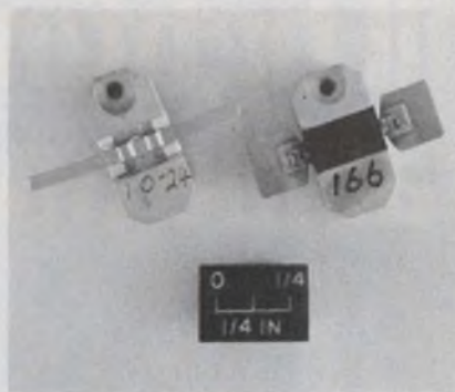
Over 500 W at 4.6 GHz in a p-i-n diode is tough to achieve. Motorola's wide gold lead is the key.
