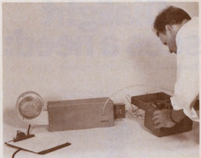
8. Test duct for transpiration coolers provides controlled, filtered air flow to allow measurement of component temperatures with a thermocouple. The blower housing contains a washable air filter.
