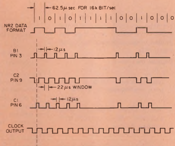
Phase-locked-loop circuit generates a synchronous clock signal from raw NRZ data and maintains a clock output even with temporary interruptions of the data.
