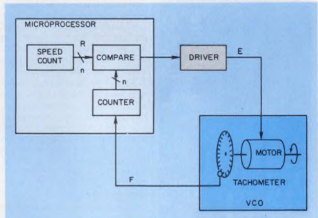
2. A microcomputer furnishes the speed reference and also performs phase and frequency comparisons under program control. Motor inertia provides the necessary loop filter.
