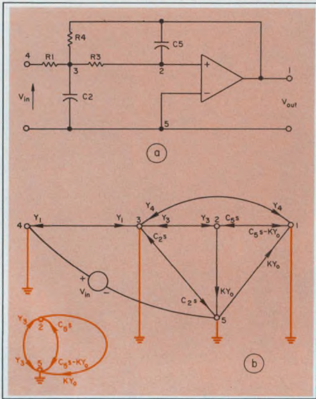
4. Ground the nodes that form paths between input and output to obtain numerator subgraphs. The circuit (a) is a multiple-feedback active filter and (b) its topological equivalent. A path subgraph is shown at bottom left.
