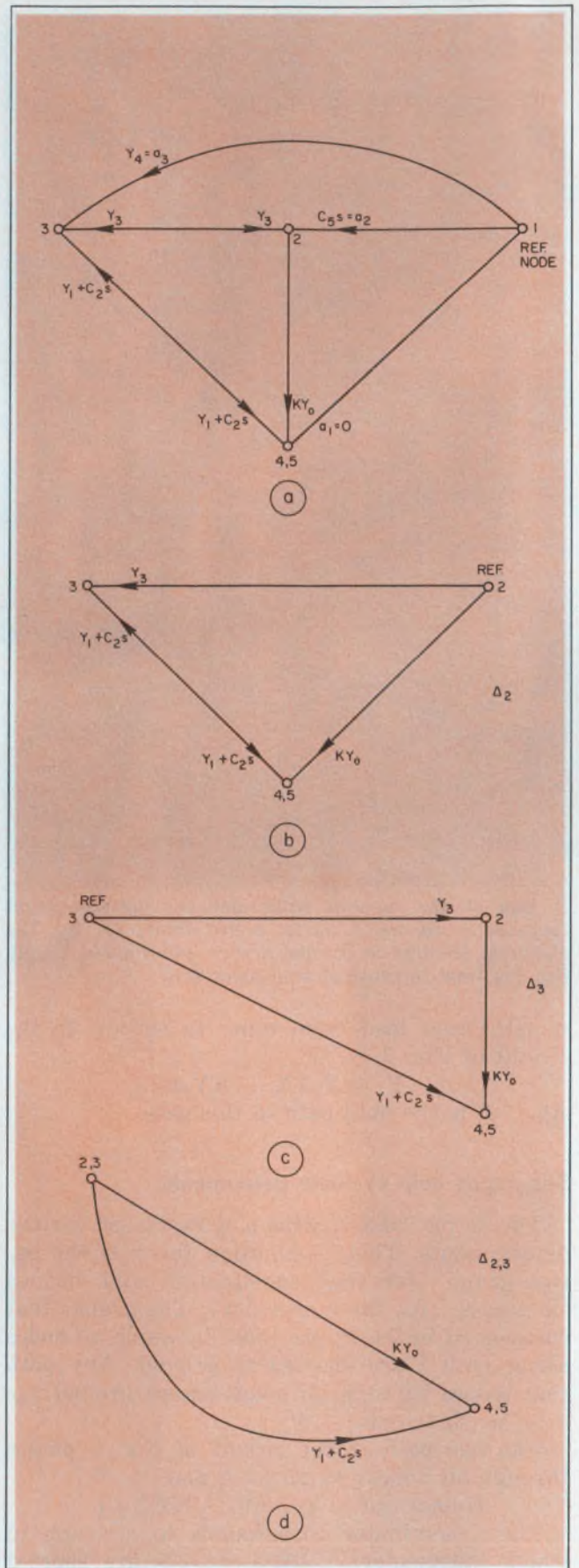
5. All voltage sources are grounded to obtain the overall subgraph for the denominator (a). The evaluation is accomplished from separate subgraphs (b, c and d) each of which may have a separate reference code.
