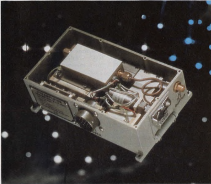
Temperature stabilization of this Micromega paramp system would normally require a 30-lb heat chamber. With thermal pads, \pm 1.8 F stabilization is achieved in a 42 oz. package.
