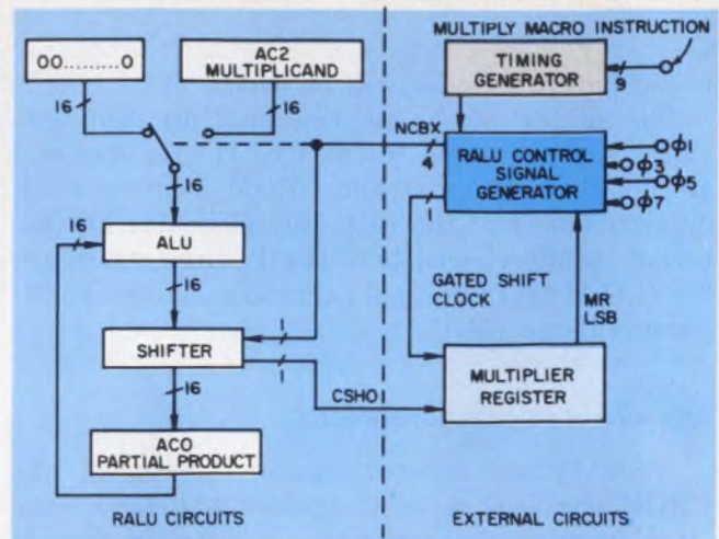
2. The complementary circuit provides alternative control signals, labeled NCBX, for the RALU. The technique can be used with the IMP-16C because it is a microprogrammable processor.
