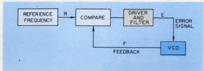
1. A conventional phase-lock loop makes the VCO frequency track that of a reference. For use with motor control, the VCO block is replaced by a motor-tachometer; comparator operation is not changed.
