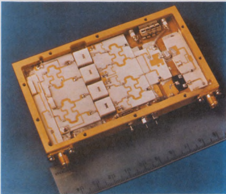
The 91024 S-band MIC power amplifier is offered in a small package by Microwave Semiconductor. The microwave transistors are mounted directly to the base to give 24 W at 55 C.
