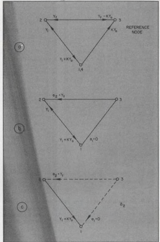
3. These transformations provide the graphic solutions. Node 3 is selected as the reference, and arrowheads directed to node 3 are removed. The single remaining branch and coefficients provide the circuit determinants.
