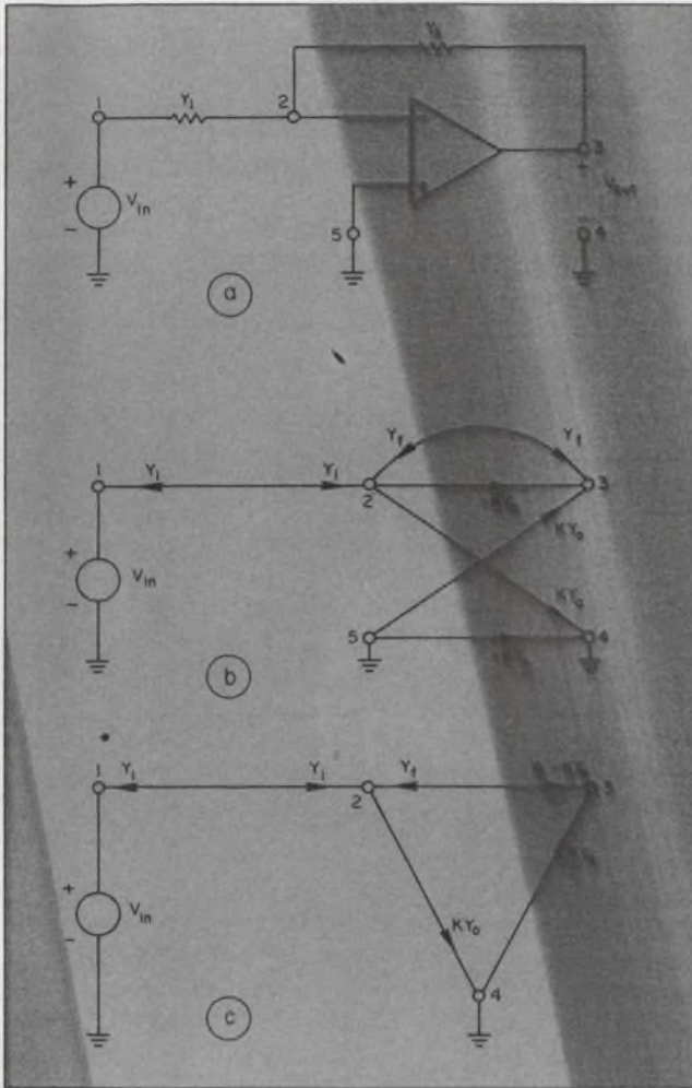
2. Use of the op-amp equivalent and passive-circuit representations helps model active filters (a, b). The algebraic addition of parallel branch admittances simplifies the final topological equivalent (c).
