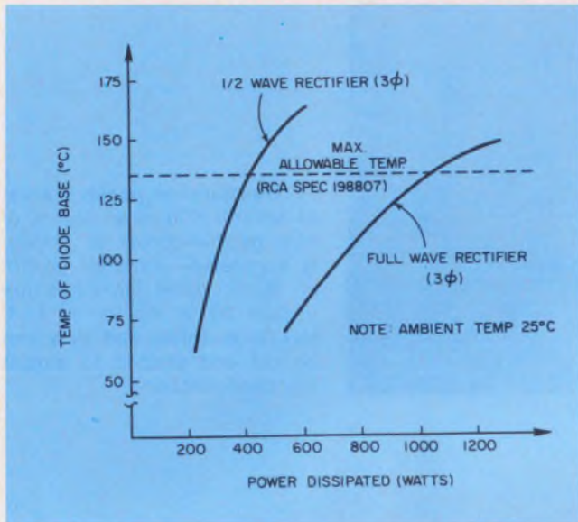
4. The cooling performance of the power-rectifier assembly shown in Fig. 3.
