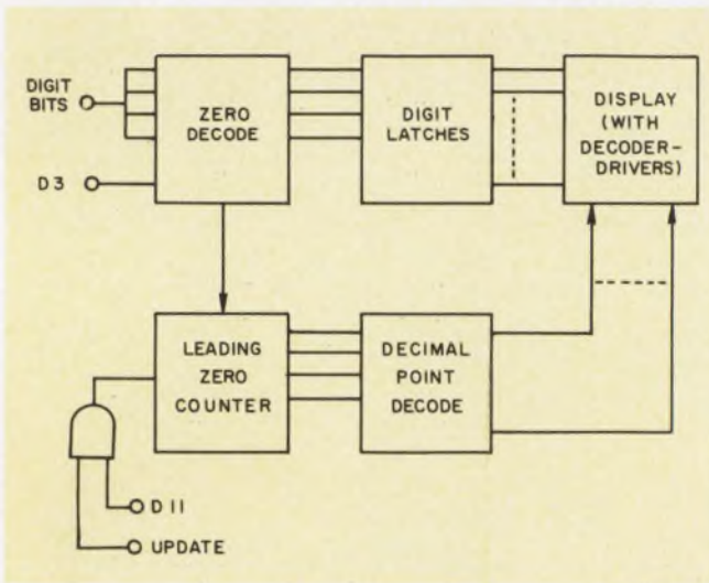
3. Output logic receives the calculator data, counts leading zeros and loads the DPM display with the 3-1/2 most-significant digits.
