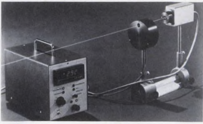
5. Electrical power is computed and displayed in a pyroelectric laser power meter. The instrument makes use of a null balance between the electrical calibration power and the laser's optical power.
