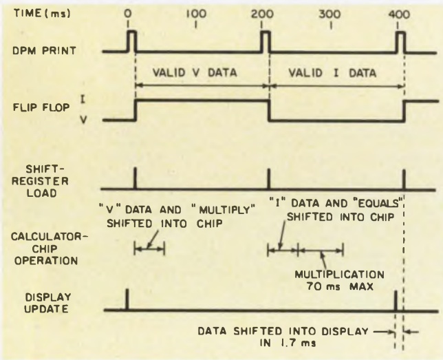
4. Timing of the power calculation is controlled by the DPM's conversion clock. The display is updated after two conversions, or about twice a second.
