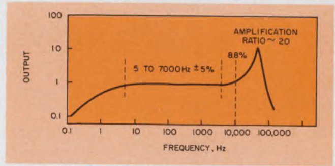
5. Typical output response of a piezoelectric accelerometer is very poor near dc, at input frequencies it is flat and at resonance it increases sharply.
