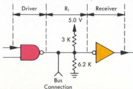
FIGURE 2 — transceiver implementation
