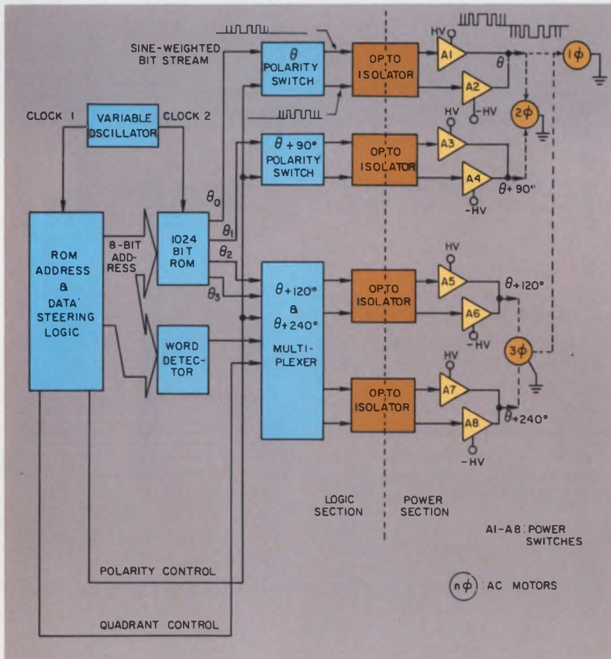
A versatile circuit capable of controlling the speed of four single-phase motors, one two-phase unit, or one three-phase device uses a 1024-bit ROM to generate sine-weighted, pulse-width-modulated trains of pulses having a variable repetition rate. The circuit, by Motorola, uses opto-isolators to decouple the low-level switching stages from the high-power driving stages.
