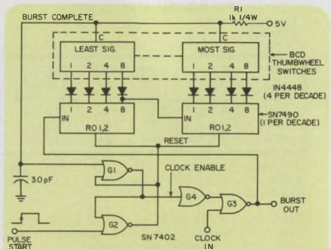
One 7402 NOR gate can control the switching for a large number of thumbwheel-programmed pulses.
