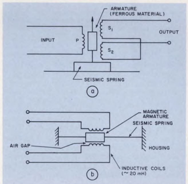
10. Differential transformer accelerometers (a) use a three-winding transformer that provides an output proportional to the displacement of a metal core within the coils. The variable reluctance accelerometer (b) uses a moving magnet to produce an electrical output due to mechanical shock.
