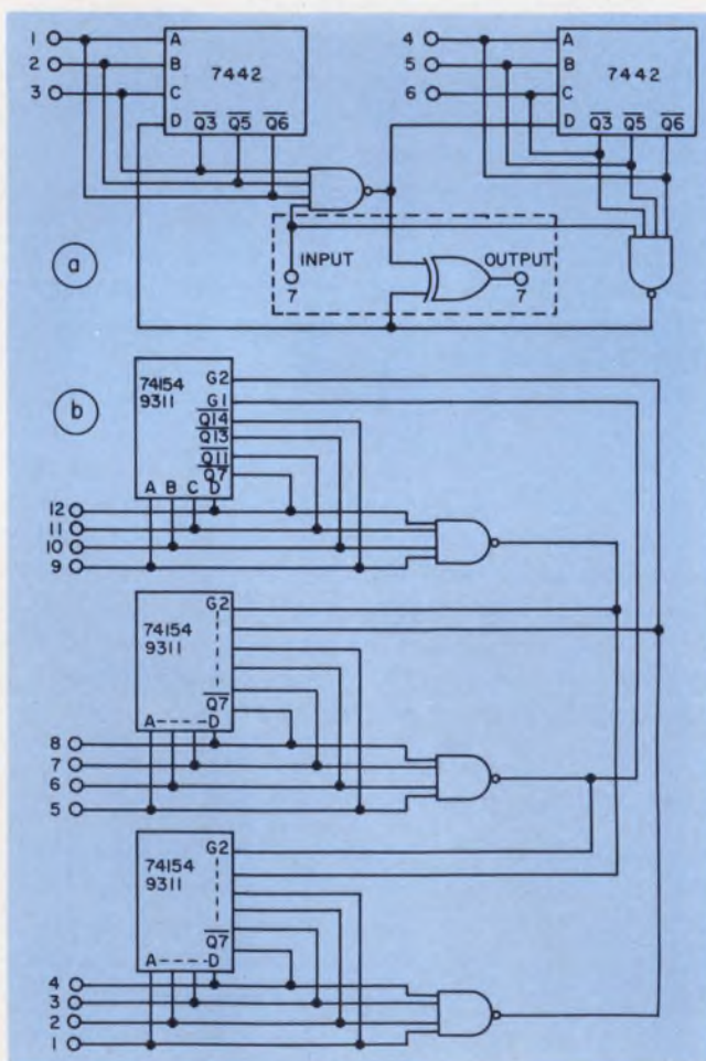
5. Larger n-flops can be built simply for special values of n. Two 7442 tri-flops gated together form a 6-flop (a). The decoder (dotted area) gives a seventh state. Three quad-flops form a 12-flop (b). The enable inputs release any latched condition if one of the other decoders receives an input.
