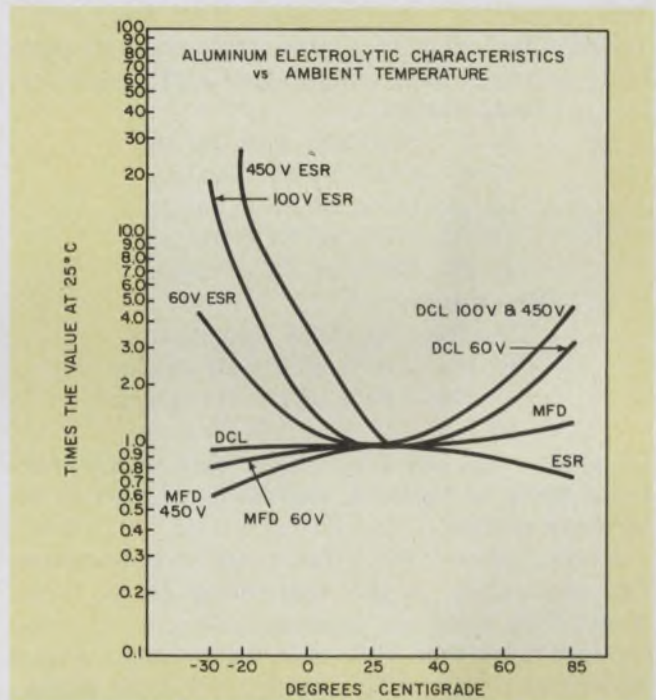
3. The important properties of an electrolytic depend strongly on the unit's temperature. DCL rises steeply but ESR drops with increasing temperature.
