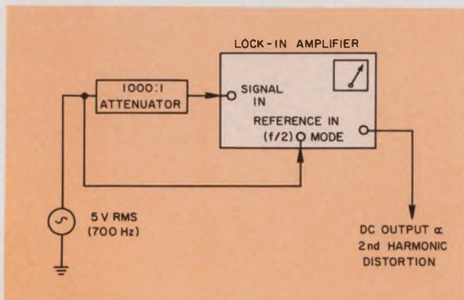
4. To measure the second-harmonic distortion generated in an amplifier (in this case, the lock-in itself), this test setup is used.
