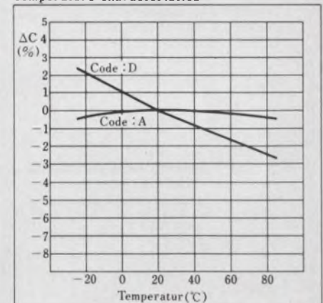
Temperature characteristics
