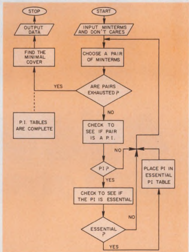
1. Flow chart of CAD program shows how logic functions are simplified. Minterm pairs are checked to find prime implicants in the final minimized function. A minimal cover process selects the fewest prime implicants to contain all minterms in the function. Essential prime implicants are always included.
