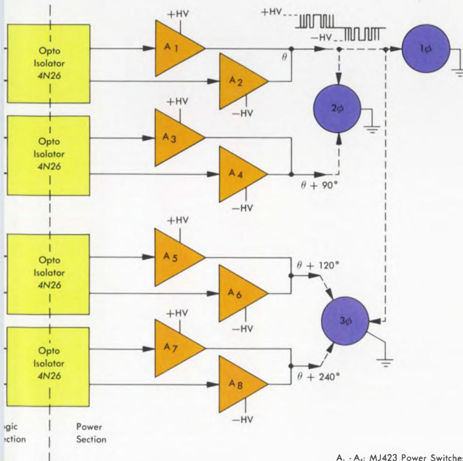
A 1 - A 8 : MJ423 Power Switches
