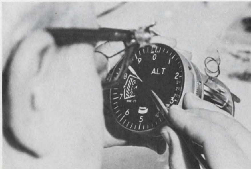
A 35,000-foot range encoding altimeter is assembled by a technician at Bendix Corp., Davenport, Iowa. It will measure and report the altitude of the da Vinci balloon in 100-foot increments. Used in conjunction with a transponder, the unit automatically transmits altitude signals to an air controller's ground control radar screen.
