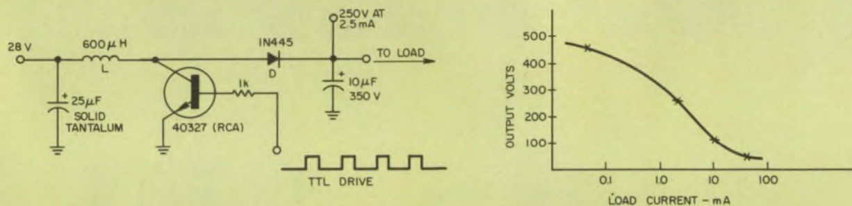
Small amounts of high-voltage power can be obtained with a simple inductor and high-voltage transistor.
