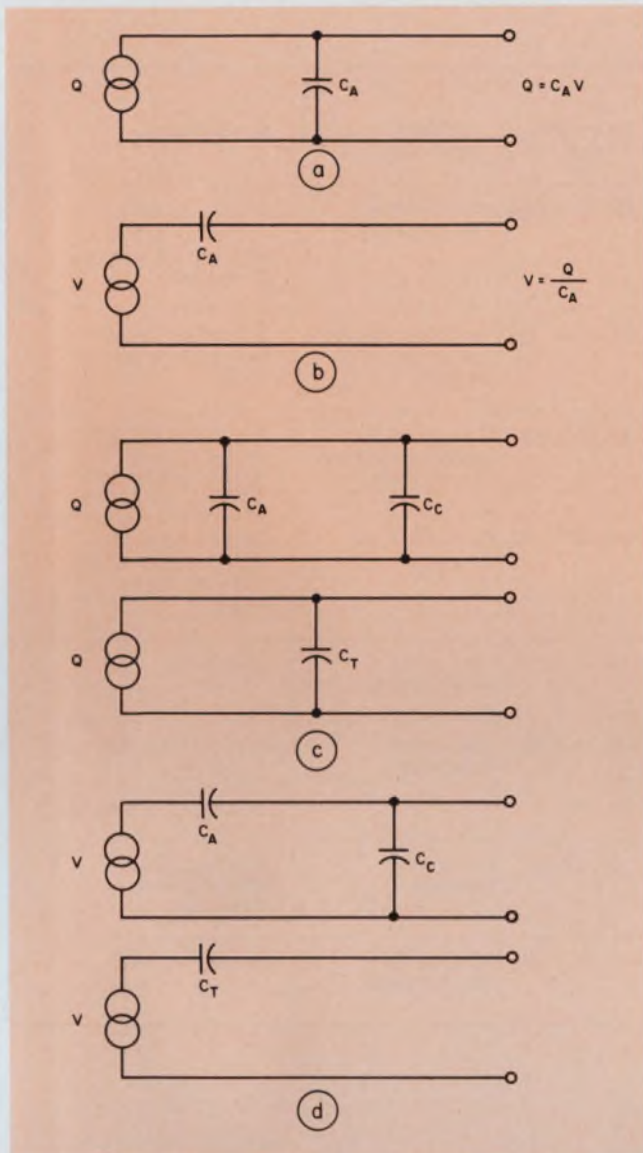
2. The piezoelectric accelerometer can be represented by a charge generator and a shunt capacitance (a) or by a voltage generator and a series capacitance (b). The effect of the cable capacitance can be added into the accelerometer models (c and d).
