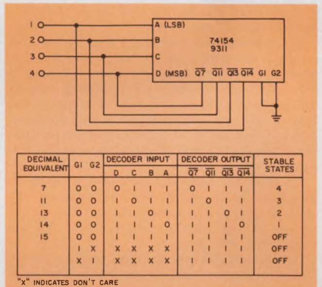
3. This quad-flop is built with a 1-of-16 decoder, as shown by the input-output table. A fifth state (1111) could be extracted with an external decoder, if needed.
