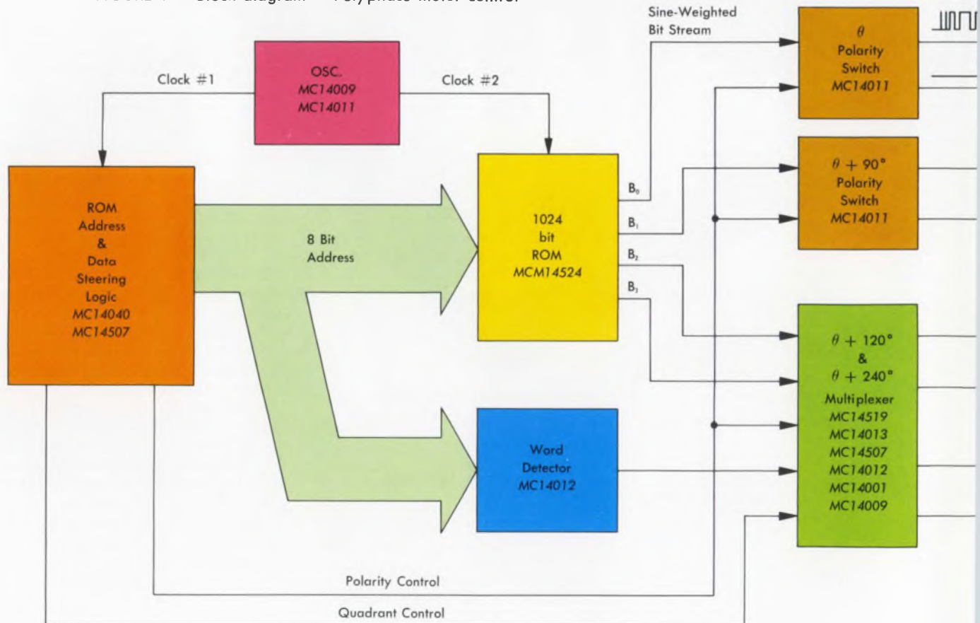
FIGURE 1 — Block diagram — Polyphase motor control
