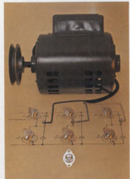
Power Darlingtons, such as these from TRW Semiconductor, are replacing SCRs in ac motor-control applications. They require less external circuitry than SCRs and are less prone to false triggering.
