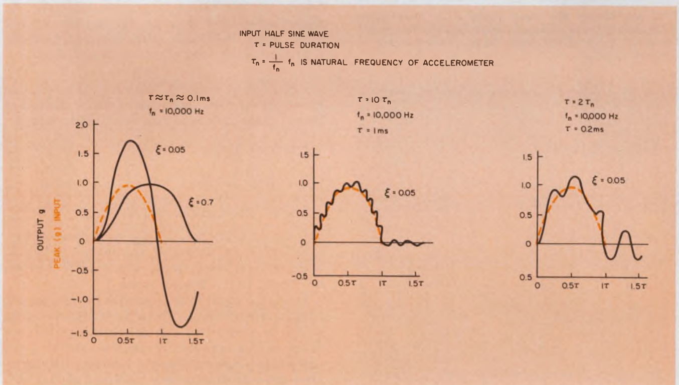
6. With an input of a half-sine-wave shock pulse, a typical transducer output doesn't necessarily follow
