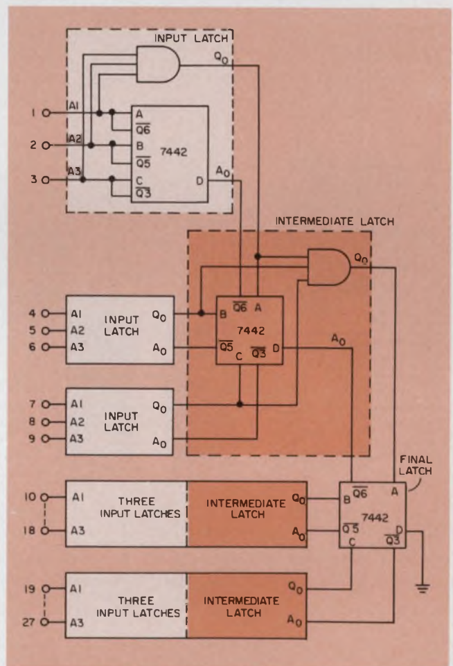
6. The tree structure allows construction of an n-flop of any desired size. Each stage of this 27-flop is essentially a 7442 tri-flop. The addition of more input and intermediate latches allows further expansion.
