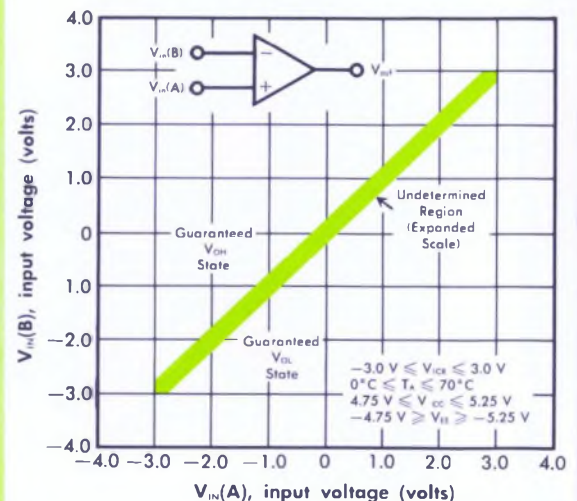
Guaranteed output state versus input voltage
