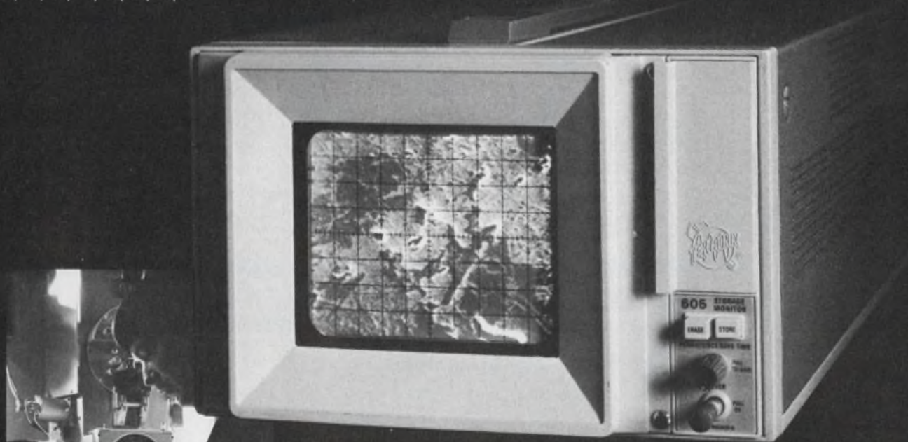
Gray scale capability and variable persistence storage of the 605 are used with a scanning electron microscope to study metal samples in a dental research laboratory.
