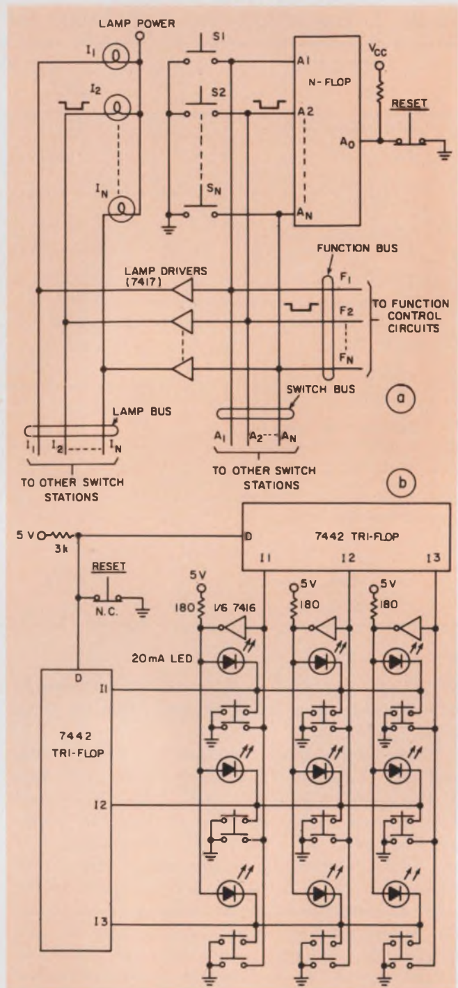
8. These n-flops latch for the most recent button pushed. The first circuit (a) uses single-contact switches. The m \times m arrangement (b) uses smaller n-flops.
