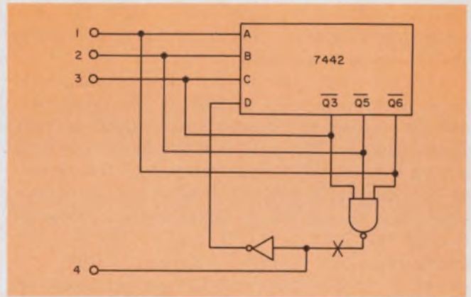
2. An auxiliary NAND gate adds a fourth stable state to the 7442 decoder. The connection can be broken at the point marked X if separate input and output terminals are desired.
