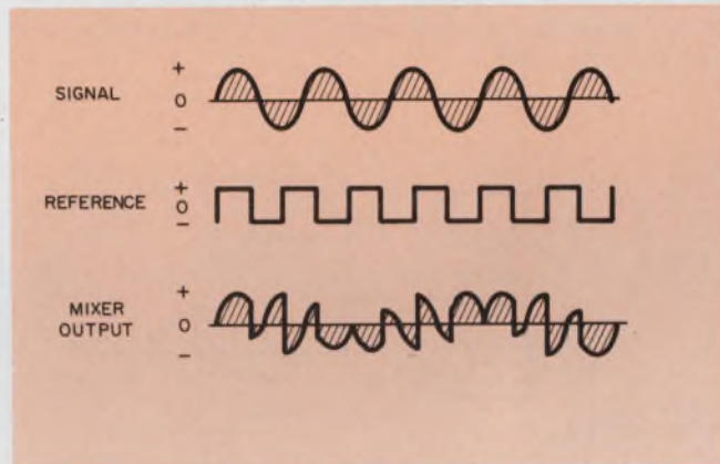
3. When the signal isn't synchronized with the reference, as in the case of noise, the average (dc) level of the mixer output is zero.
