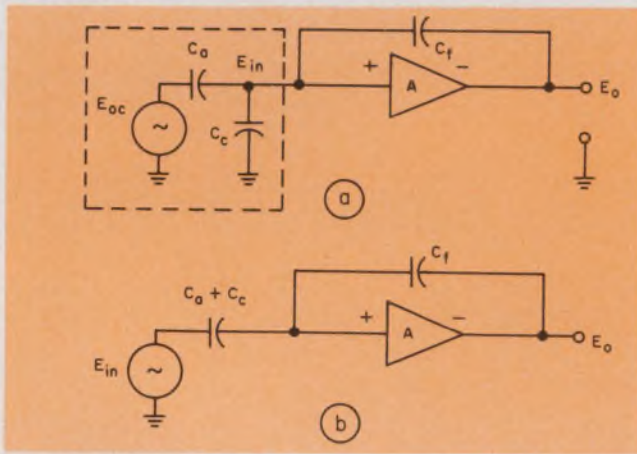
11. The basic charge amplifier allows different cable lengths, from 1 to 200 ft., to be used without affecting the charge sensitivity of the transducer system.
