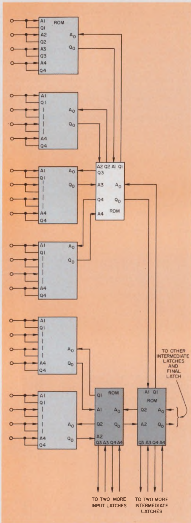
7. ROMs or programmable logic arrays (PLAs) can be the building blocks for large n-flops. Each ROM is a quad-flop. The circuit structure is a tree, and the over-all circuit has a lower package count than one built with decoders.
