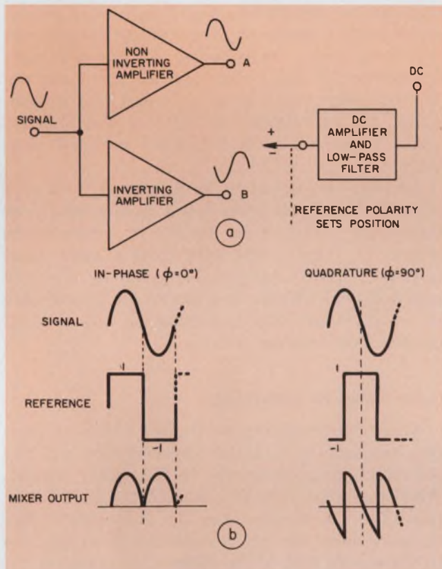
2. Key element of the lock-in is the mixer, which operates as a phase-sensitive switch (a). The switch position depends on the polarity of the reference square-wave drive, so that the input signal is commutated at the reference frequency (b).
