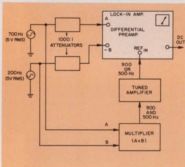
5. Intermodulation products can be measured with a differential preamp in the lock-in's front end. Harmonic distortion can then be calculated from the measured products. In this way the spectral purity (impurity, actually) of the excitation source can be neglected.
