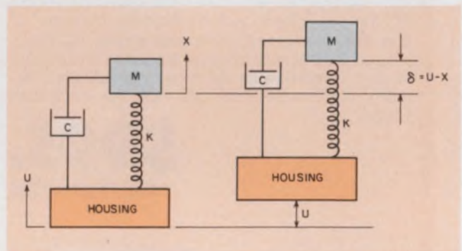
1. Ideal seismic systems can be modeled to simulate the transducer and the way it is affected by forces.
