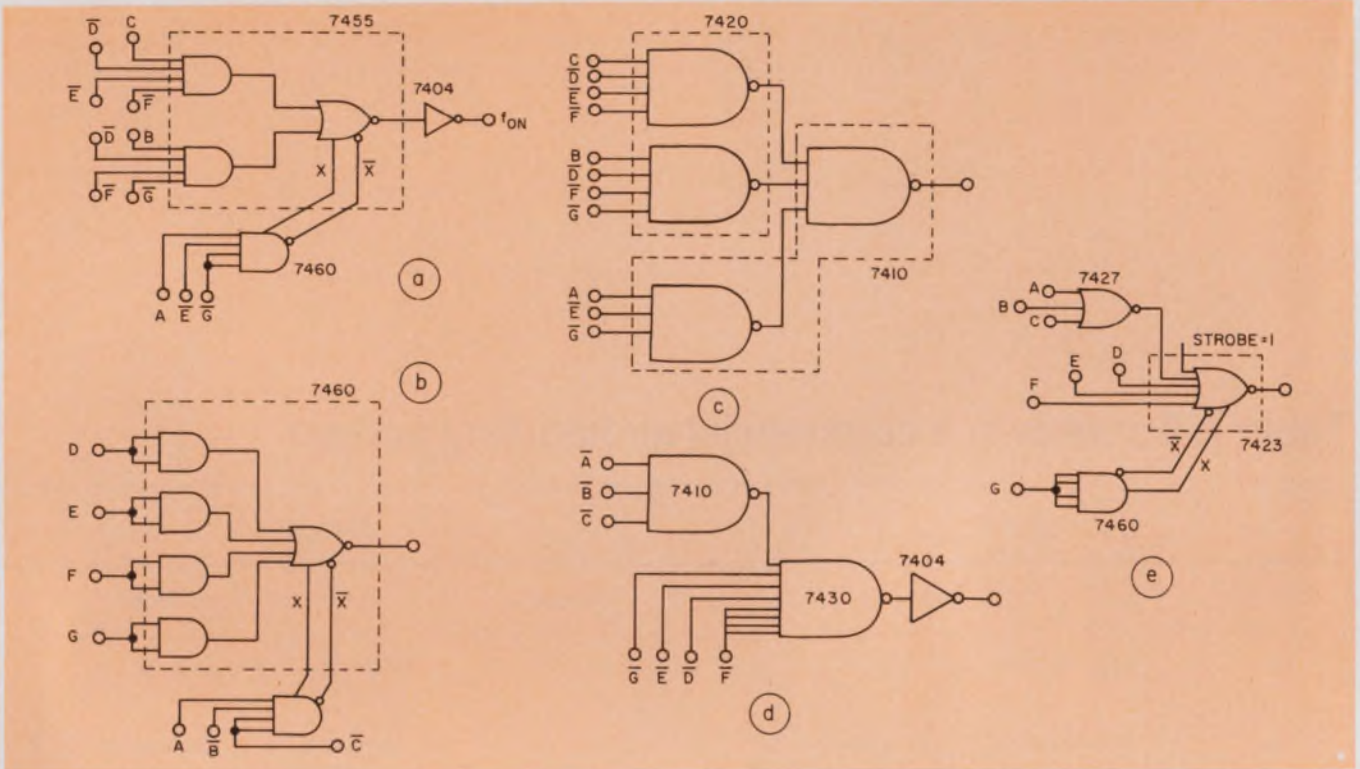
2. IC implementations of a CAD logic function problem (a) and (b) produce the function and complement, respectively, from the computer printout. A third circuit
