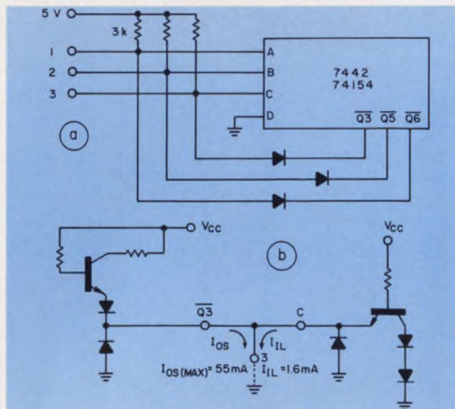
4. Isolation diodes reduce initial loading when the n-flop is switched to a new state (a). With the diodes, the input driver does not sink the output current of the decoder, which is generated by the active pull-up transistors inside the decoder (b).
