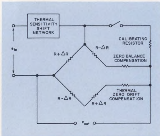
8. The strain-gauge accelerometer uses a balanced bridge network with thermal compensation added to maintain the zero drift and temperature sensitivity with specifications.
