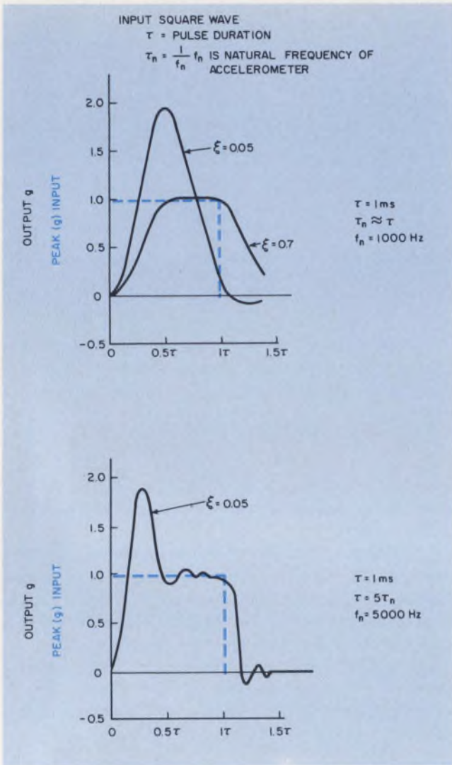
7. If you change the input signal to a square-wave shock pulse, the transducer output will usually exceed the actual value of the shock pulse unless the unit is critically damped.
