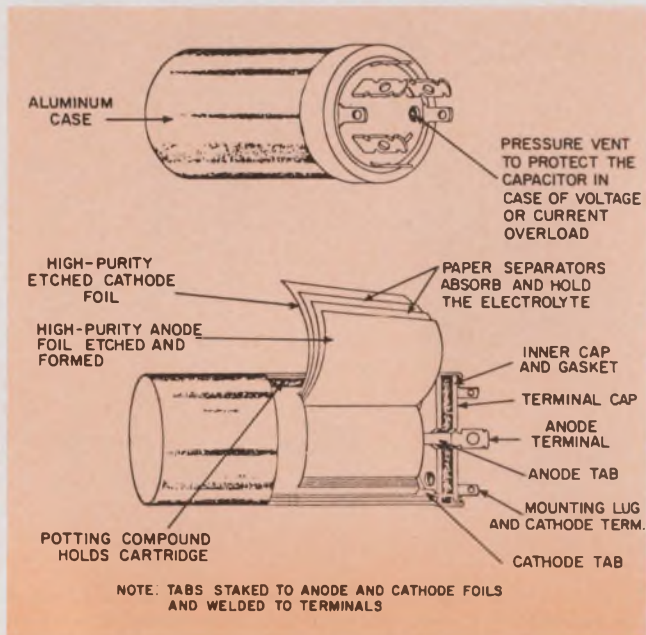
6. Large electrolytic capacitors have a vent to allow escape of any internal build-up of gas or vapor.
