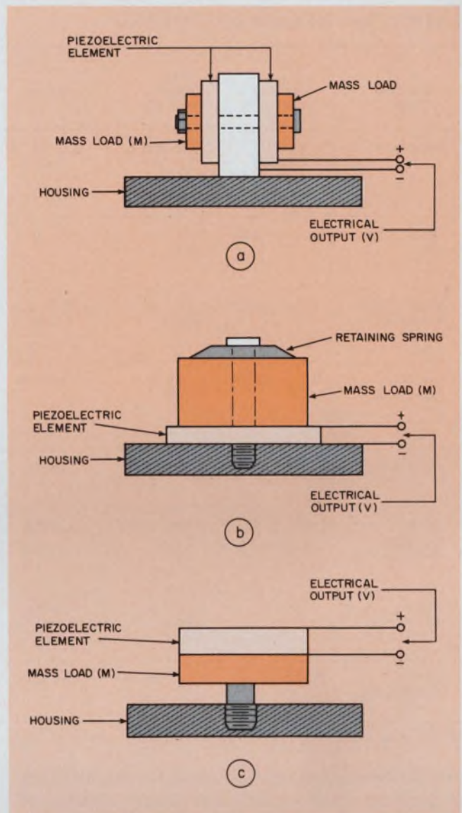
3. The piezoelectric accelerometer can be mounted to produce an output in either the shear (a), compression (b) or bender (c) mode of operation. In any of these operating modes, the accelerometer usually moves less than a thousandth of an inch.
