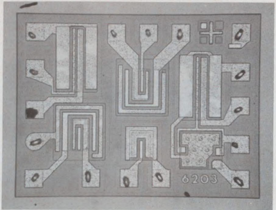
SCRs as part of monolithic ICs are bringing down the cost of controlling very small motors. The RCA CA3097E thyristor/transistor array contains an SCR with 150 mA max forward current, as well as an array of transistors and a zener diode.
