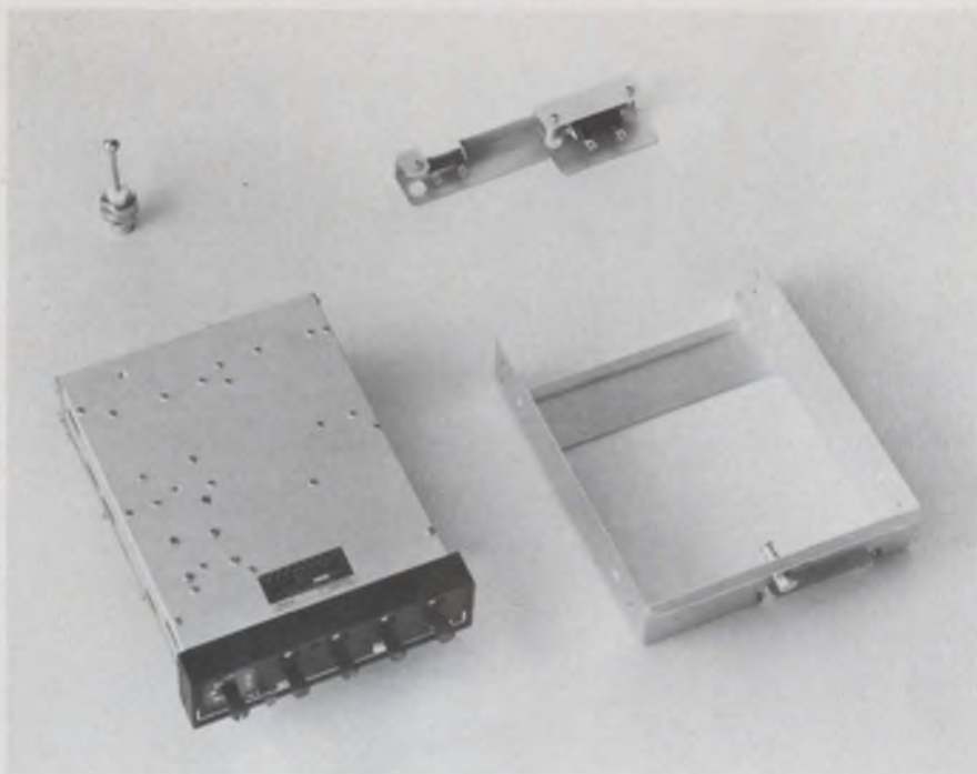
Transponder used on board the da Vinci balloon is an example of the latest technology used in avionics instrumentation. Developed by Bendix, the one chip replaces up to 200 discrete components required for previous designs.
