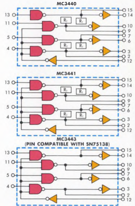
The MC3440 family of Quad Interface Bus Transceivers
