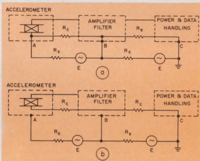
12. Ground-loop problems within a multicircuit measuring system can create many problems (a). If all the circuits use a common ground (b) the various pieces of equipment can work together.
