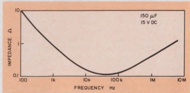
7. An electrolytic capacitor's impedance is equivalent to a series RLC circuit. Minimum impedance, which occurs at resonance, is resistive.
