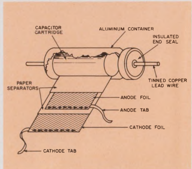
4. In axial-lead aluminum electrolytics, the container shell is usually connected to the cathode via a tab at one end. The anode lead passes through an insulating seal at the other end of the container.
