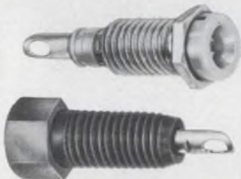
TEST JACKS for .080 diameter probe
