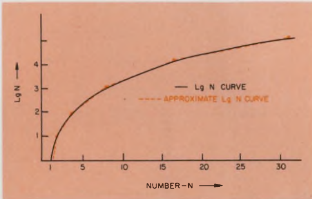
1. A plot of logarithms is closely approximated by straight-line segments between whole powers of 2, which are the logs 2 of the binary-number sequence.
