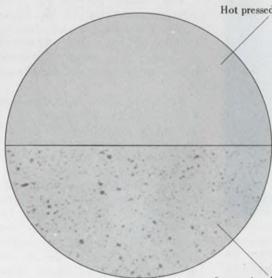
Conventional ferrite (Micrograph: x100)
