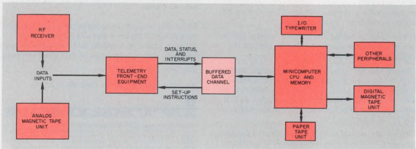
1. Raw telemetry data are buffered and converted to block form for processing by the computer. External
