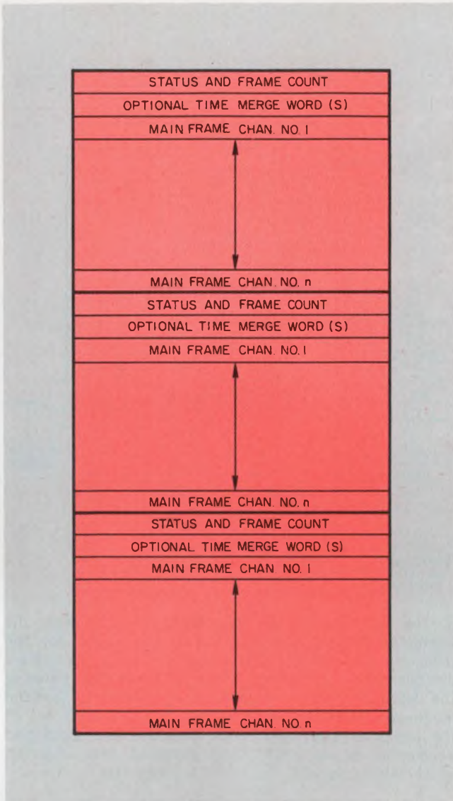
5. A typical data block in memory starts at location x and consists of y words. The status block permits the computation of the subframe or channel at which sampling began. The buffer signals the computer via an interrupt when a block is completed and begins a new block in an alternate buffer area.
