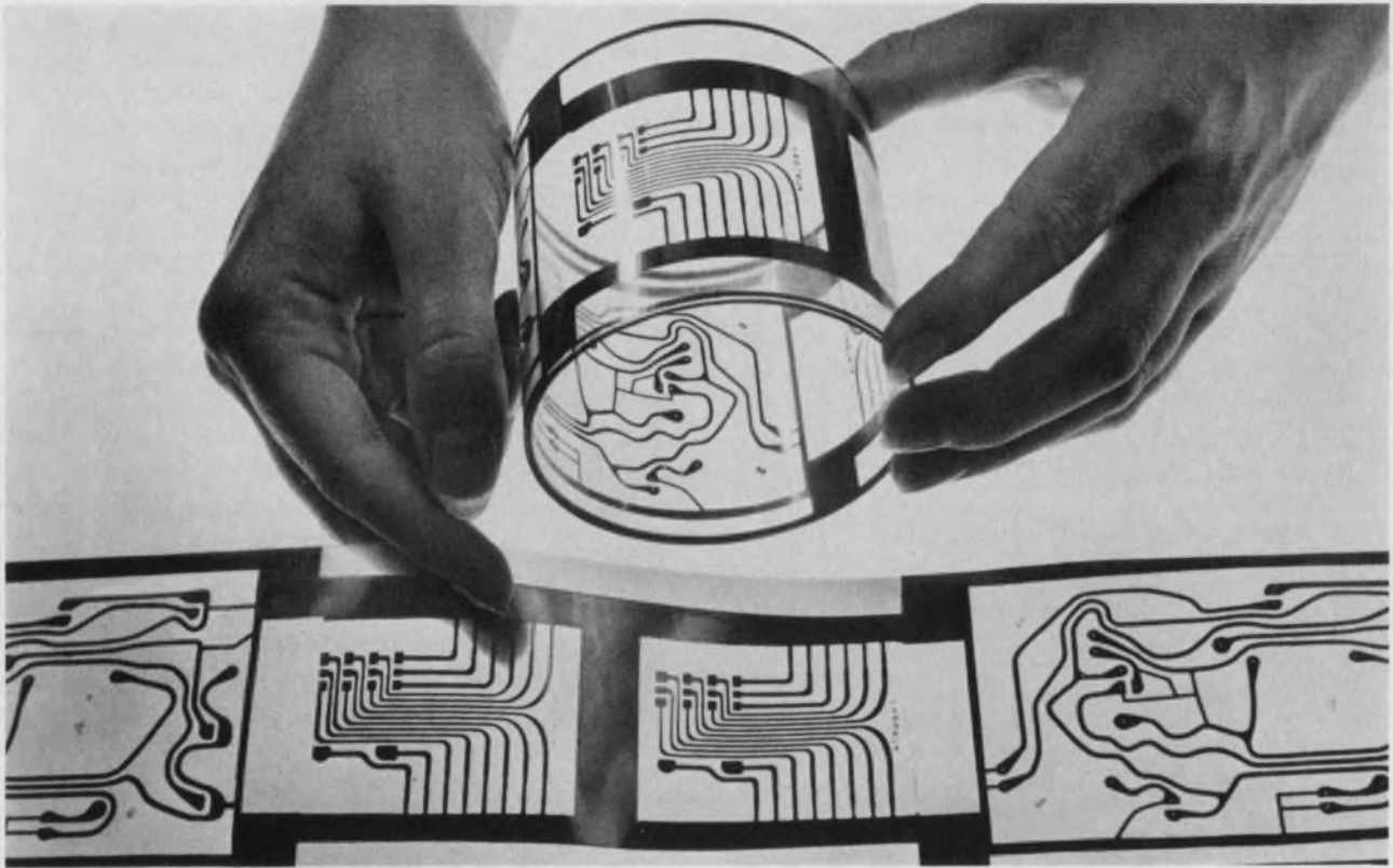
Copper conservation is an objective of this printed-circuit process introduced a number of years ago by Western Electric Co. In the process, copper cir-
