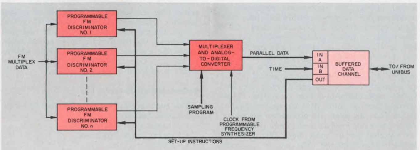
6. FM analog data must be digitized before being inputted to the buffer. The multiplexer controlled by the
