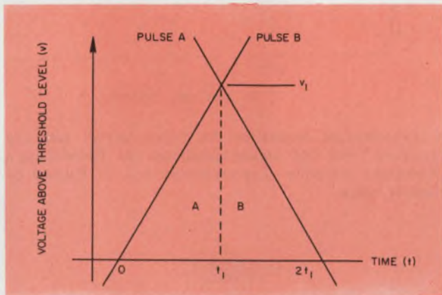
2. The amount of energy "injected" into a gate by two overlapping pulses can be determined by calculation of the area under the intersection. The amount injected decreases rapidly as the overlap narrows.
