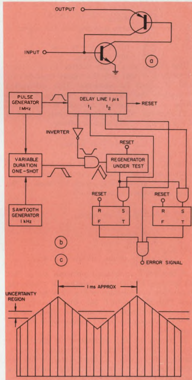
3. Typically, a regenerative circuit (a) follows a gate in a computing chain. When an arbitrarily small spike enters the regenerator, the circuit may delay in resolving the spike into a ONE or ZERO. The "uncertainty" can be measured (b) if an asynchronously modulated spike stream (c) is fed into the gate-regenerator and the error signals are monitored.
