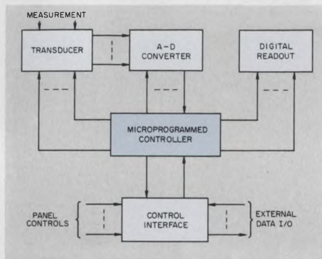
1. A microprocessor, functioning as a microprogrammed controller, allows the economical use of digital techniques for the required operations.
