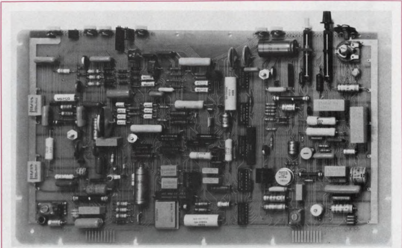
Vital to any computer system are components like these. This circuit board illustrates the Mepeco/Electra, Inc., line of resistors, capacitors, thermis-
