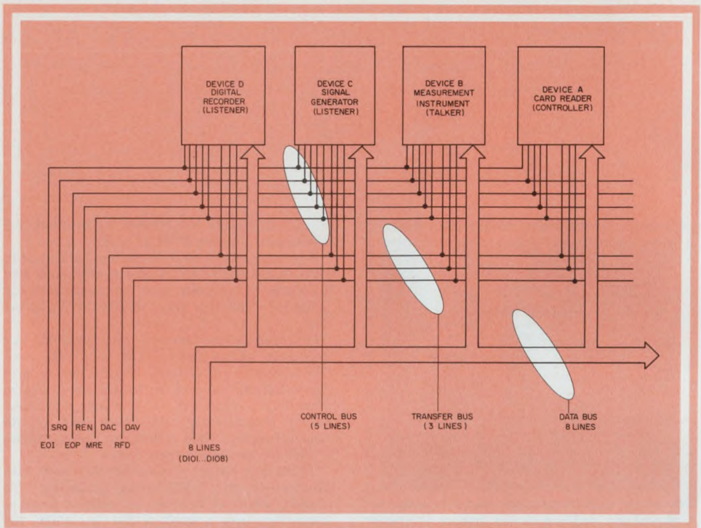
4. Systems communication network consists of three major busses: data, transfer and control.
