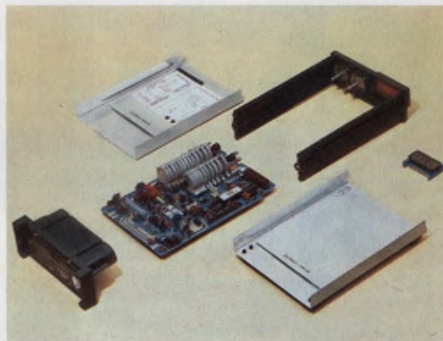
Slip the shafts out of the selector switches that are mounted to the PC board, and you avoid cable or socket wiring, as in Data Technology's Model 30 DMM.
