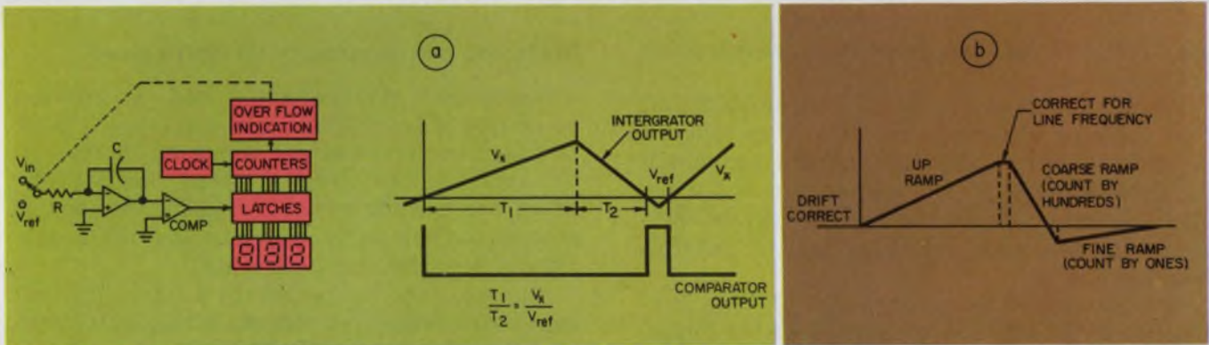
2. A variation of the basic dual-slope technique (a) is the triple-slope a/d conversion technique (b) used by
