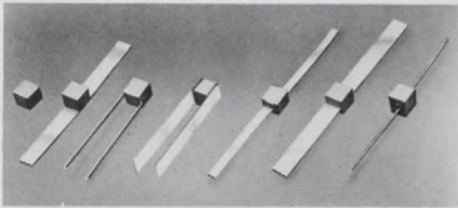
10. Terminations for chip components come in a variety of styles, as illustrated by American Technical Ceramics' rf capacitors.
