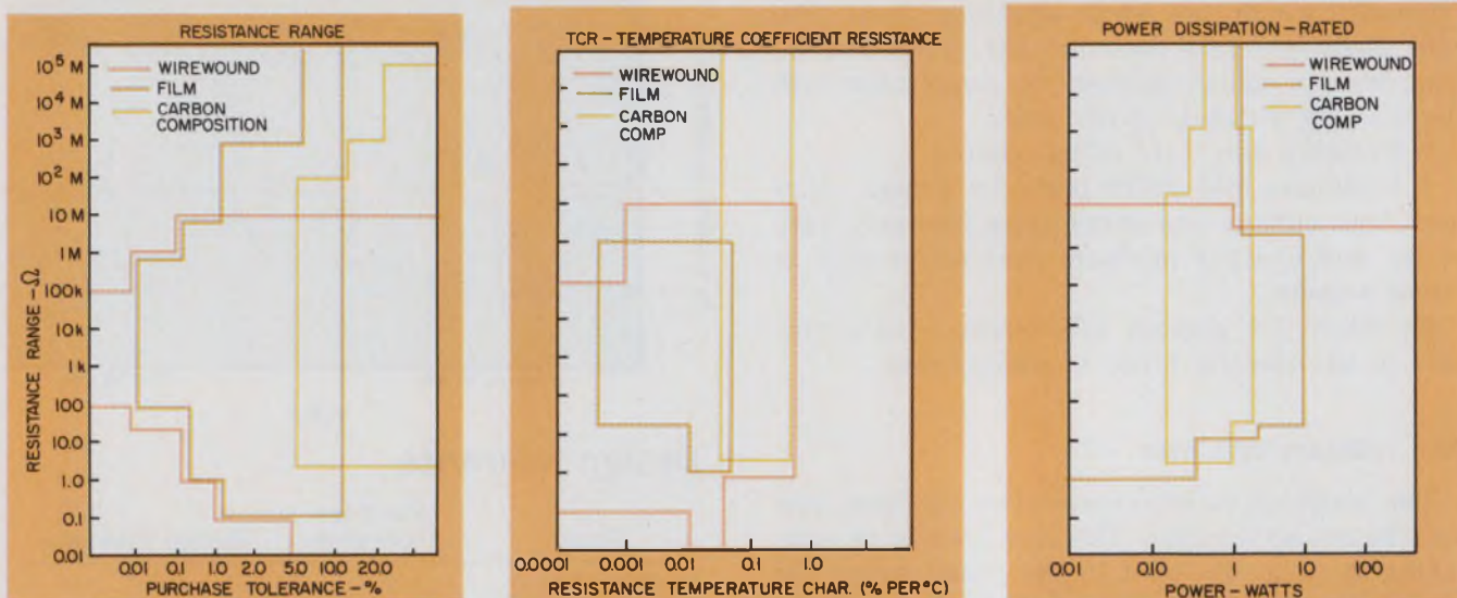
6. Some ranges of tolerance, temperature coefficient and power are dominated by a particular type of resistor, while other ranges can be handled by many different
