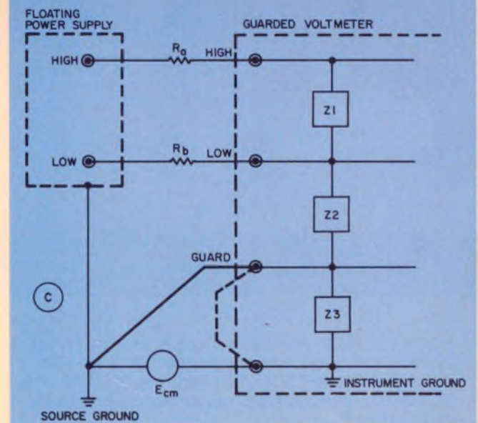
7. A source and guard can be connected in three ways. In the preferred connection (a), no common-mode current flows through R_a or R_b . In the other two connections (b, c), some current may flow in R_b .
