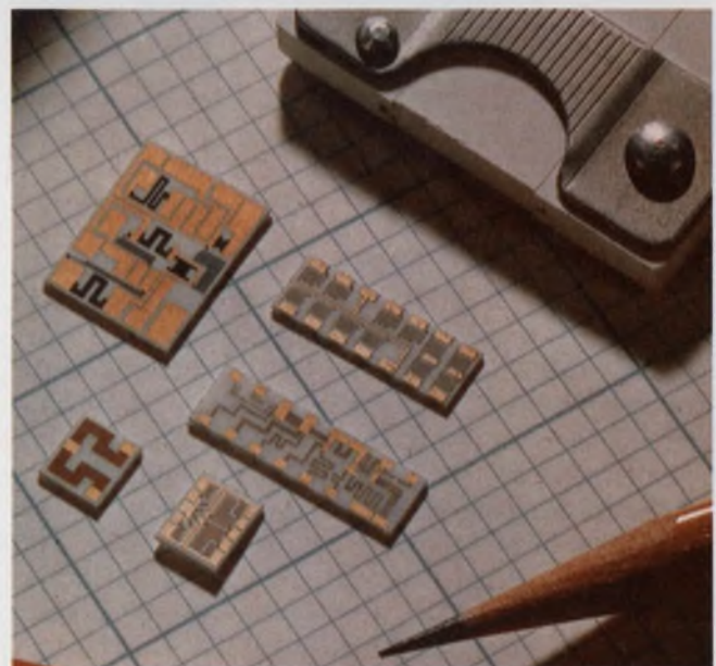
9. Resistor networks, such as these TRW TanFilm units, are filling industry needs for package-compatible components for hybrid and DIP configured circuits.
