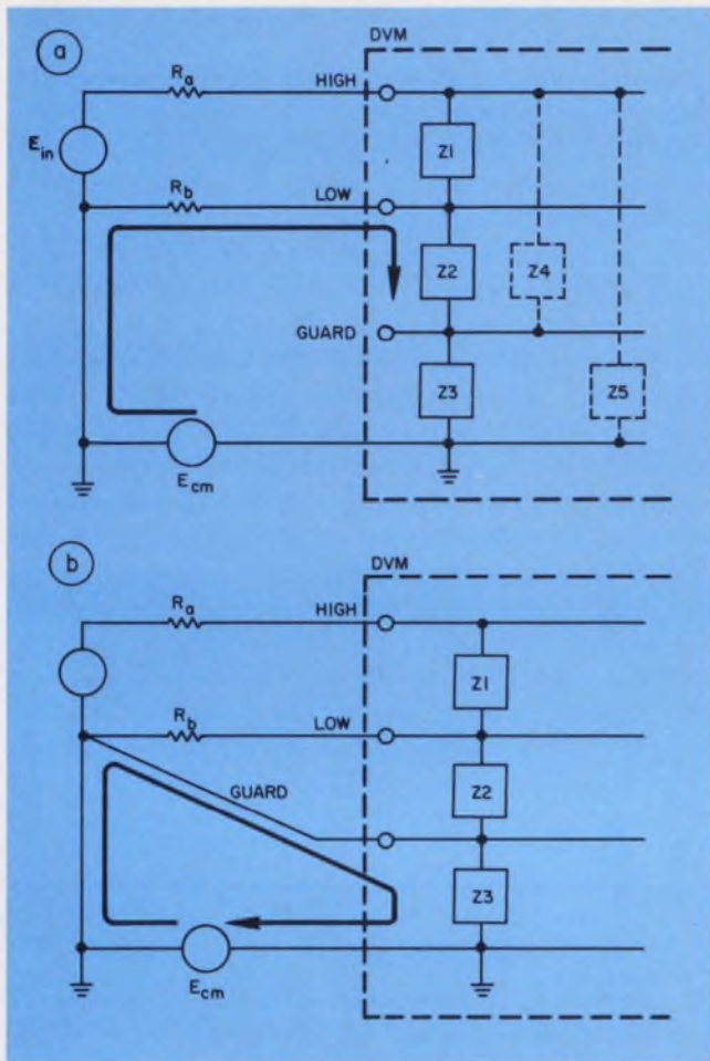
5. In DVMs with a guard, the impedance between low and ground is increased by Z_3 (a). Connecting the guard to the source low terminal shunts unwanted currents (b).
