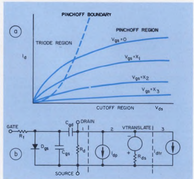
1. The three regions of FET operation, shown in a multi-curve plot of I_d vs V_{ds} (a), can be modeled with the circuit of b. The portions of the circuit labeled 1, 2, and 3 are used as the circuit model for, respectively, for cutoff, pinchoff and triode-region operation.
