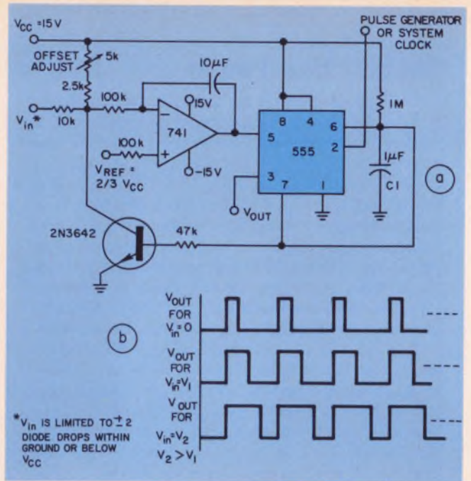
3. Voltage levels can be converted to pulse durations by combining an op amp and a timer IC. Accuracies to better than 1% can be obtained with this circuit (a) and the output signals (b) still retain the original frequency— independent of input voltage.
