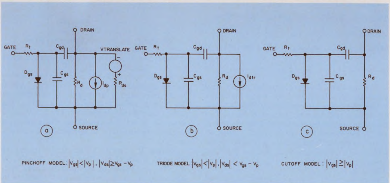
2. Depending on relative values for V_{gs} and V_{ds} , the circuit models for the pinchoff (a), triode (b) and cutoff (c) regions of FET operation can be applied. The models are valid for all values of drain current and
