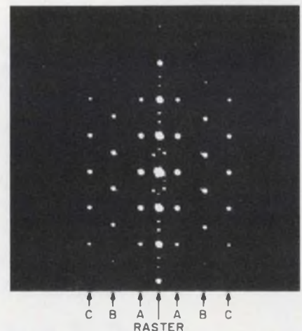
3. Synthetic gratings formed by modulating laser with three carriers have a unique white-light pattern.
