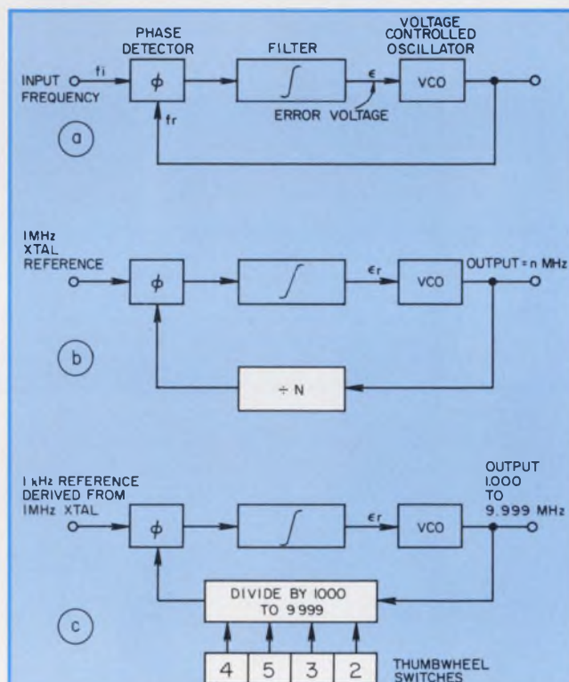
1. In a basic phase-locked loop (a), the VCO output is locked with the crystal oscillator. If a fixed divide-by-N circuit is inserted in the feedback loop (b), the output of the VCO can differ from the input reference. Any number of output frequencies within the range of the VCO can be obtained by setting the divide-by-N circuit with BCD thumbwheel switches (c).
