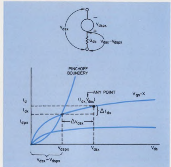
5. The origin of any V_{gs} curve is set at the pinchoff boundary to maintain the needed continuity along the boundary. Voltage source V_{dsp} is used to account for the difference between this origin and the actual one.
