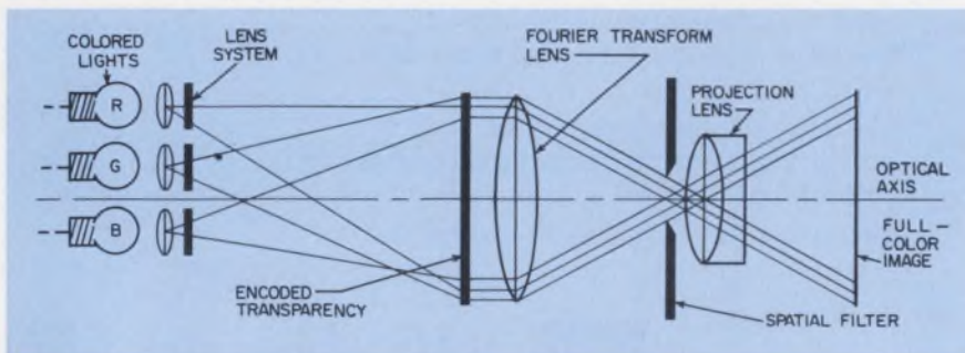
5. Simple optical system transforms the diffraction components of tricolor carrier gratings into a full-color reconstruction of original scene.
