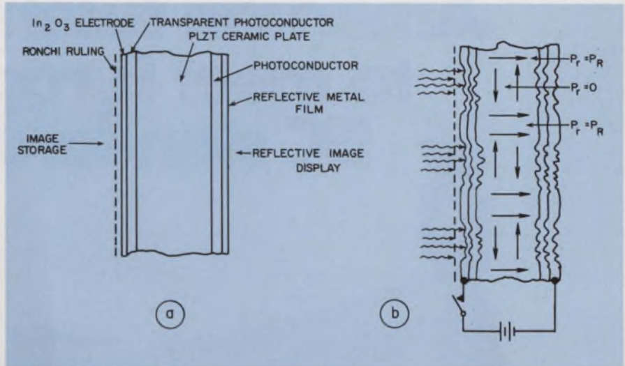
Fericon structure (a) stores images as strain-induced deformations (b) on the surfaces of lead lanthanum zirconate titanate (PLZT) plates.
