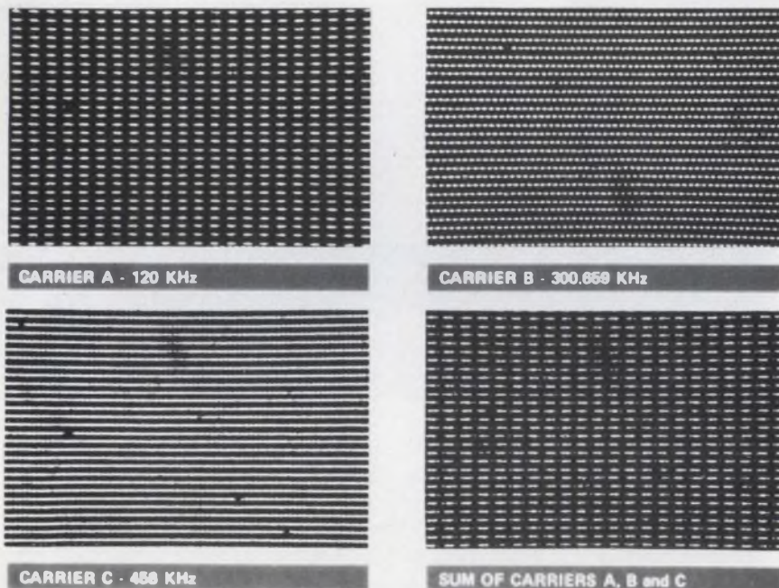
4. Microphotograph of a recorded film shows the synthetic diffraction gratings produced for red, green and blue colors. Their sum is white.
