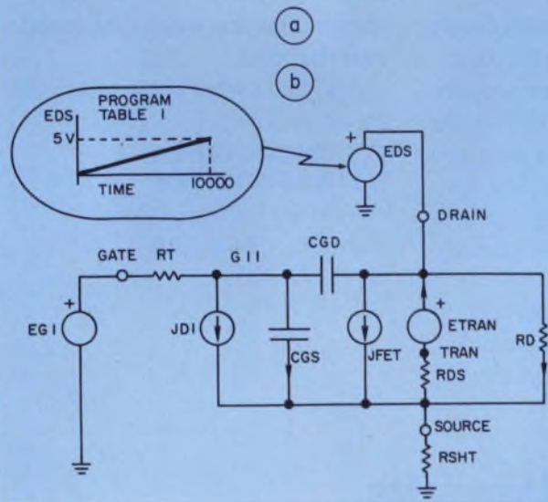
6. A program listing in SCEPTRE (a) permits the generation of FET I_d vs V_{ds} curves for constant V_{gs} . The accompanying schematic (b) relates the FET model derived to the program. A curve-tracer mode simulation is achieved by storing data points for various values of gate-to-source voltage (EG1) and formatting the output to display all V_{gs} curves on one I_d vs V_{ds} plane.
