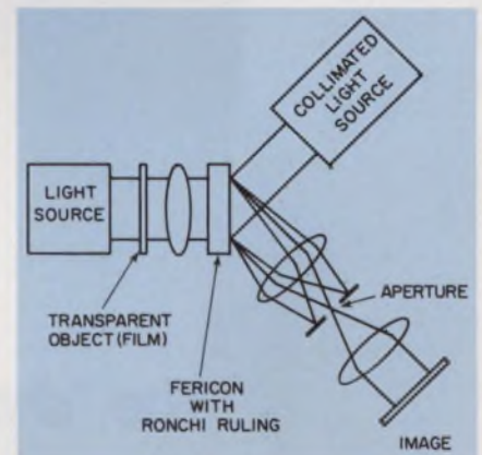
Phase-sensitive optical system is used for storing and projecting images stored in the Fericon.
