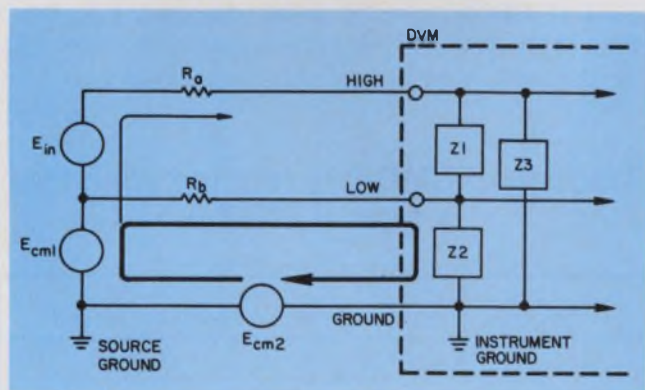
4. Two sources of noise— E_{cm1} and E_{cm2} —can appear in a floating measurement, in which neither source terminal is grounded.
