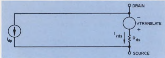
4. The model for the G_{ds} -slope at origin variation presumes that the G_{ds} curve begins at the pinchoff boundary. The difference between the actual origin and the boundary origin is accounted for by source V-translate.
