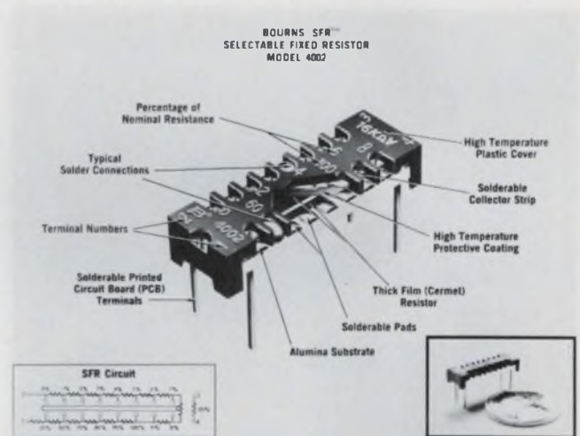
8. For those set-once-and-forget applications, Bourn's SFR selectable, fixed resistors provide a definition of 1% and a resistance range of 33 \Omega to 1.25 M \Omega with only 15 units.
