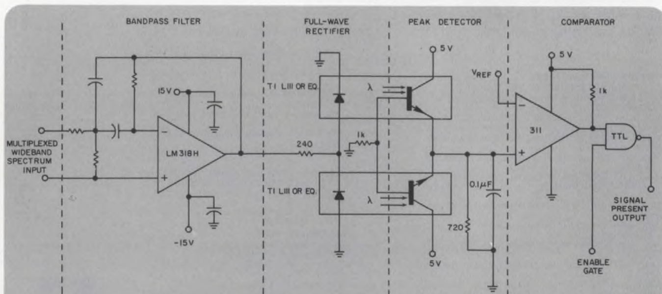
1. Ultrasonic detector with optical isolators avoids need for a transformer and bridge rectifier.
