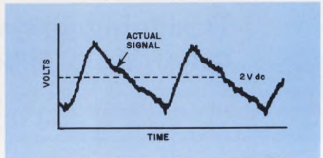
1. A "typical" noise signal consists of a periodic ripple and noise spikes—both superimposed on a dc level. This noise can cause 100% errors.
