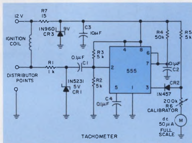
1. A car tachometer can be replaced by this low power circuit. The load current drawn by the 555 is negligible.
