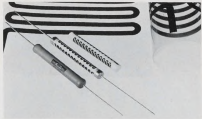
7. Caddock's serpentine film resistors have a minimum of inductance—little more than that of a wire the length of the resistor.
