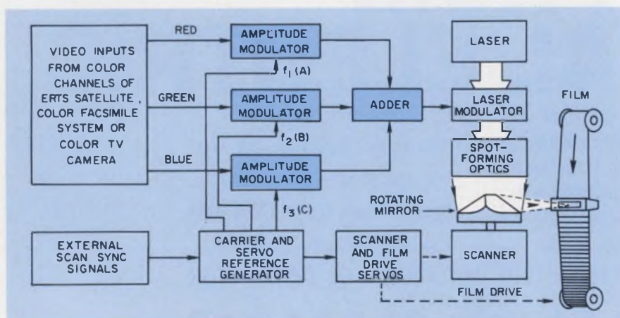
1. Modulated-laser scanner system records multicolor coded images on black-and-white film. Laser produces synthetic diffraction gratings on the film. They contain the image and color information.
