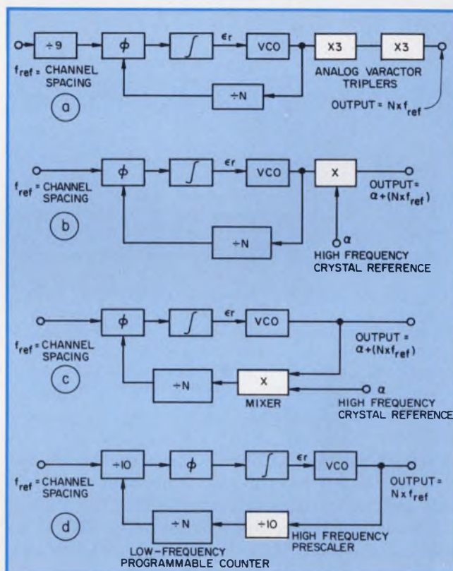
2. Higher frequencies can be obtained by multiplying the VCO output (a), by adding a serial mixer to produce a suitable offset frequency (b), by adding a mixer in the loop (c) or by inserting a high-frequency prescaler into the feedback loop (d).
