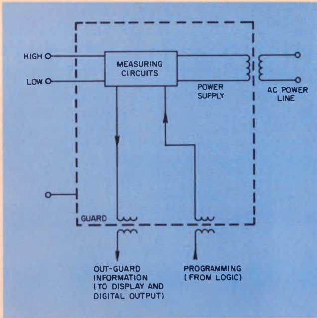
6. Guard-shield isolation must be maintained when information is passed from one side of the guard to the other. Pulse transformers are often used for this.
