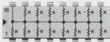
898-1 (15 resistors) Price (1,000-4,999) $3.85
