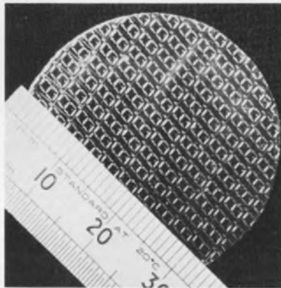
This slice of green-doped gallium-phosphide material has been processed to produce seven-segment numerics, each 2.5 mm high.
