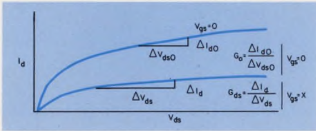
3. Conductance in the pinchoff region is normalized to the V_{gs} = 0 curve slope, G_0 . This conductance can be interpolated from manufacturers' curves.
