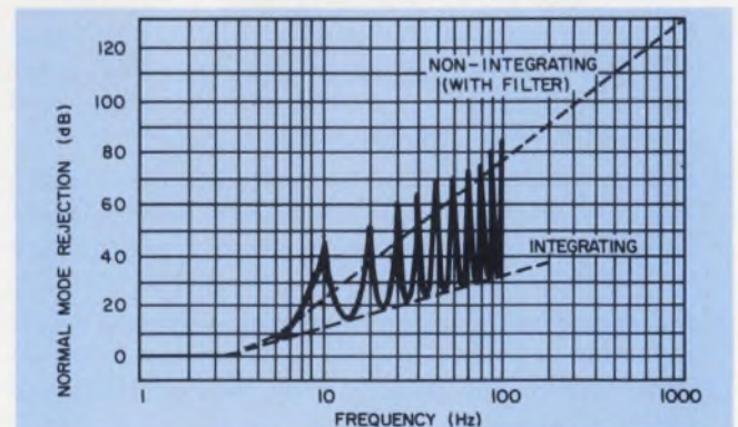
3. A comparison of an integrating and a filtered-input DVM shows that filtering is best for broadband noise. integration for line-related noise.
