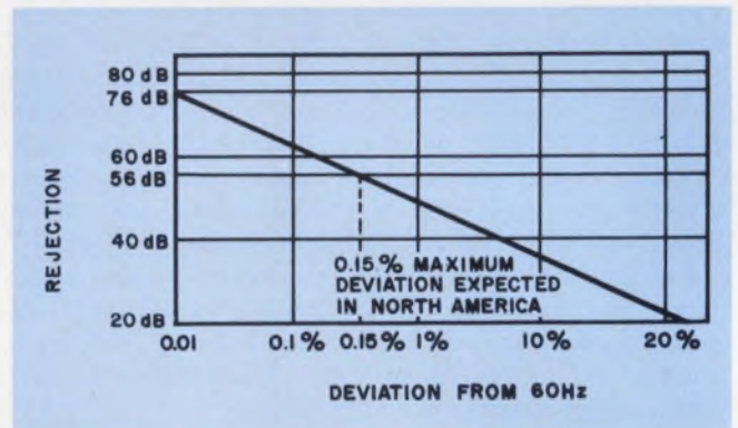
2. Integrating DVM with 1/60-s period of integration exhibits 56-dB of rejection for commonly-encountered line-frequency fluctuations of \pm 0.15\% .
