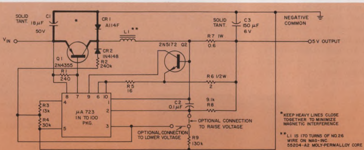
Switched regulator with current limiting can deliver half an amp using a low-cost plastic-packaged out-
