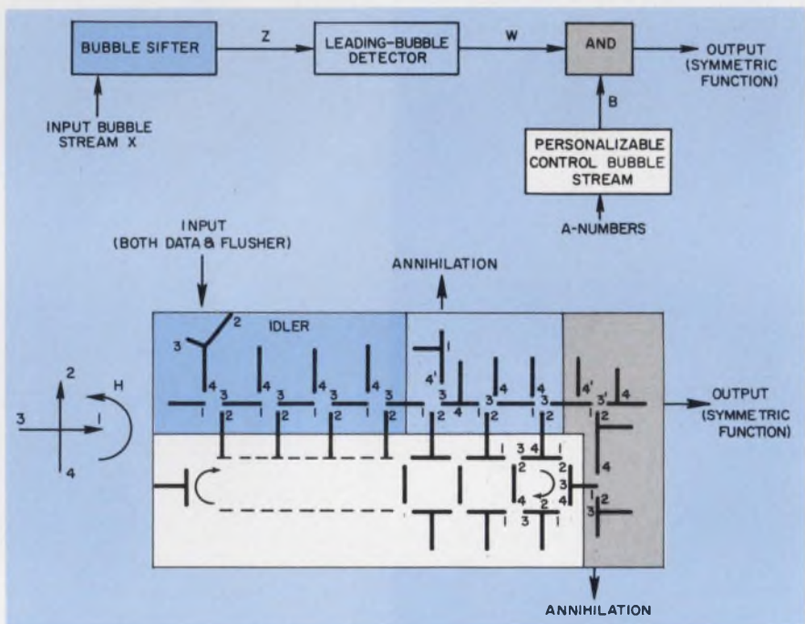
Required bubble mechanisms to realize symmetric switching functions are shown in the block diagram (above) and the permalloy pattern (below).
