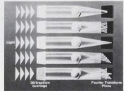
2. Diffraction patterns of gratings can be optically processed to recover impressed information.
