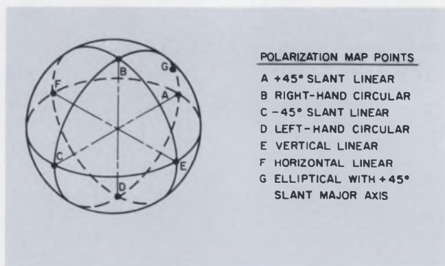
2. All possible polarizations are represented on the surface of this Poincare sphere. Points that are diametrically opposed represent polarizations that are orthogonal to each other. If these points correspond to the polarizations of a transmitter and a receiver, then the receiver will pick up none of the transmitter's power.
