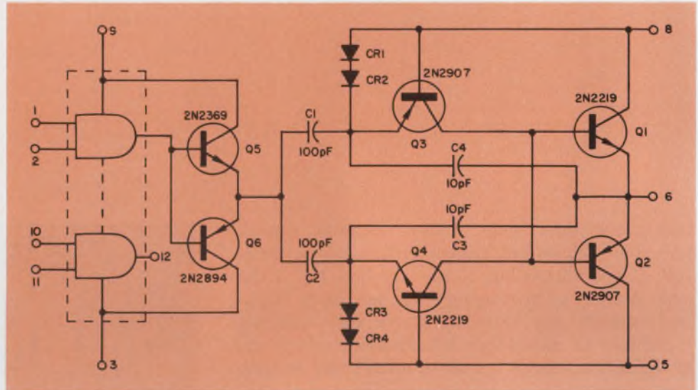
4. The output voltage swing of this hybrid clock driver circuit is above 28 V. Input logic functions are performed with a monolithic dual gate.
