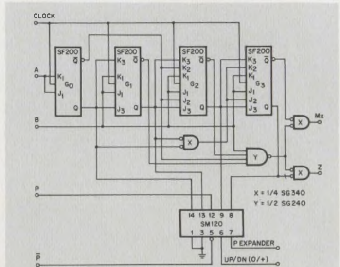
Fig. 1. Four-bit Gray-code up/down counter.
