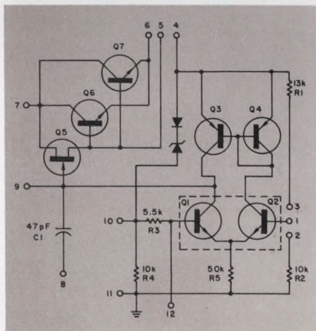
3. Resistor trimming techniques are used to set the output voltage of this 12-V regulator. The external compensation that monolithics require is not necessary.
