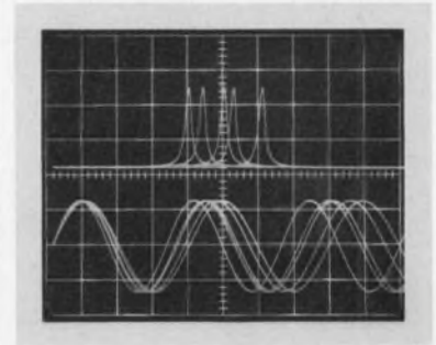
Stored time and frequency display showing oscillator drift using the 564B Storage Oscilloscope and 3L5 Analyzer.
