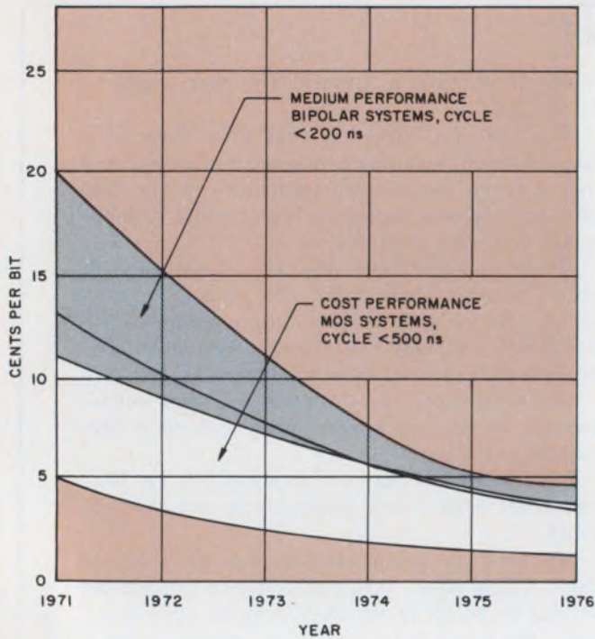
3. Cost projections for two of Cogar Corp.'s memory cards: a medium-performance bipolar card, 1 K x 18, with a cycle time of 150 ns at a cost per bit in 1971 of 12¢, and a "cost performance" n-channel MOS card, 8 K x 18, with a cycle time of 300 ns at a cost per bit in 1971 of 5¢. The low end of the band in each curve represents the cost of a card that is fully loaded and thus makes maximum use of support circuitry on the card.
