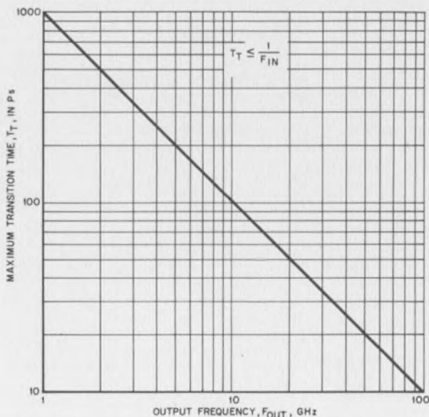
Fig. 2. Maximum diode transition time compared to output frequency of multiplier.
