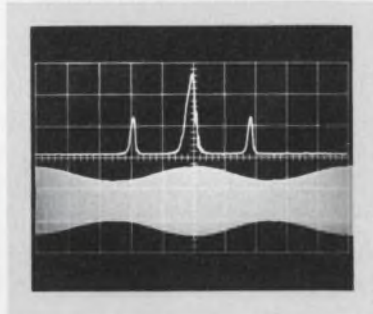
Stored time and frequency display of an AM signal using the 549 Storage Oscilloscope and 1L5 Analyzer.
