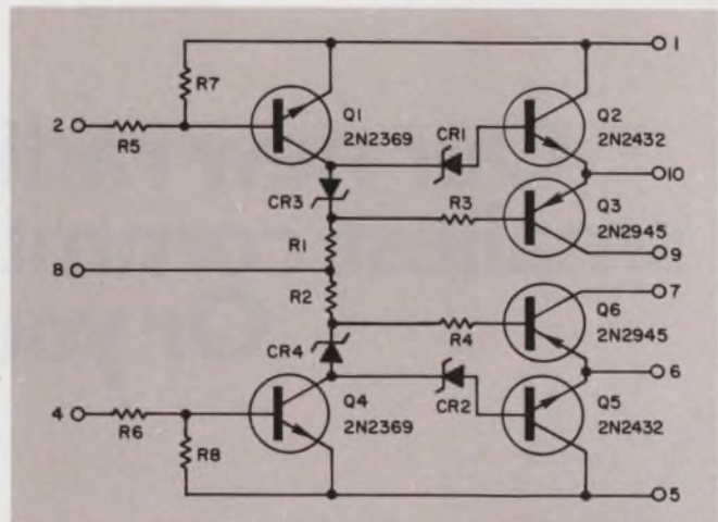
5. Parallel switching for each bit is required for high-speed d/a conversion. This hybrid 2-bit switch combines both high speed with low offset voltage. The response time is limited by the speed of the switch.
