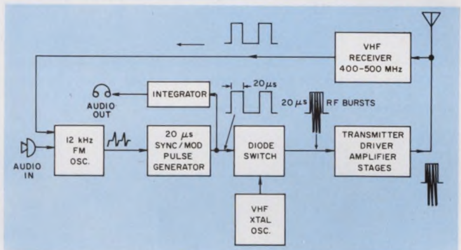
1. In the new Bendix vhf transceiver, the 12-kHz oscillator is frequency-modulated by local voice or received signals, producing a time-varied string of 20- \mu s pulses that are demodulated by an integrator.
