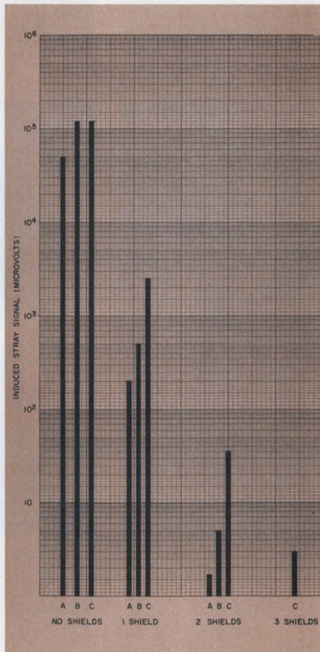
1. Shields help cut stray signal pickup, but it's not the whole solution. Superior core-coil construction makes unit A least sensitive to external fields, while unit C suffers from poor shield design.
