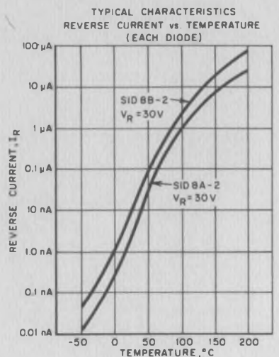
Fig. 2. Typical characteristics of diode arrays.
