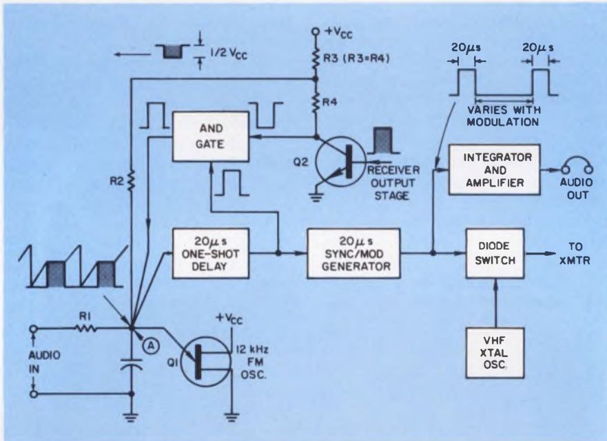
2. A unique feature of the Bendix system is the manner in which the 12-kHz FM oscillator is synchronized with its own transmitter pulses or with received pulses by feeding back the receiver's output to Q_1 .
