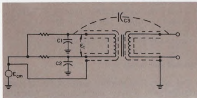
3. External wiring capacitance can defeat the best shielding design. Error voltage E_1 appears across the primary unless all leads are routed and terminated properly.
