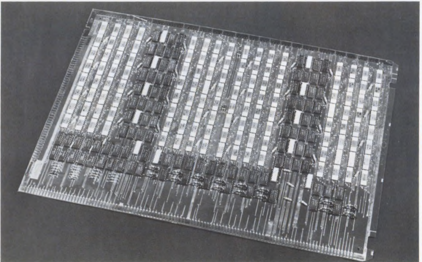
One of four memory boards, each containing 2 K words x 16 bits, is used in the Illiac IV memory system designed and manufactured by Fairchild Semiconductor for
