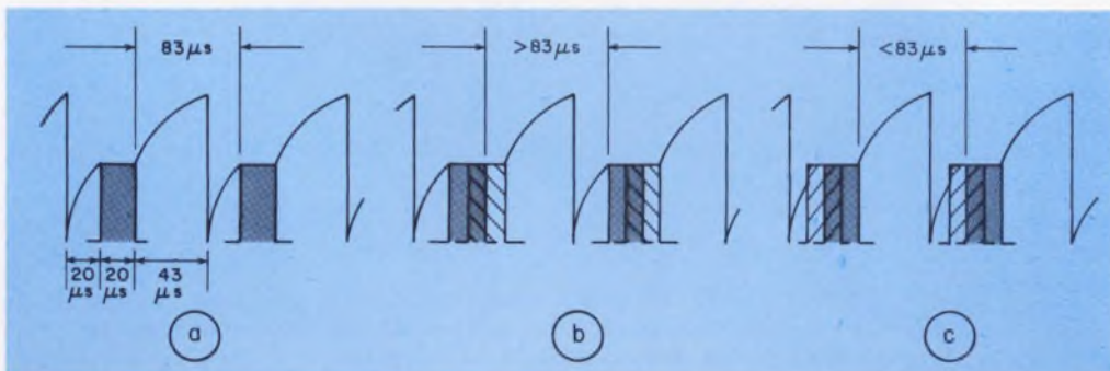
2. A unique feature of the Bendix system is the manner in which the 12-kHz FM oscillator is synchronized with its own transmitter pulses or with received pulses by feeding back the receiver's output to Q_1 .
