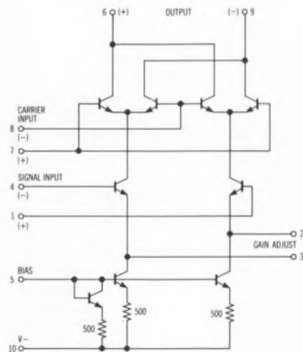
\mu A796 DOUBLY BALANCED MODULATOR/DEMULATOR
