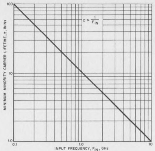
Fig. 1. Minimum minority carrier lifetime compared to multiplier input frequency.
