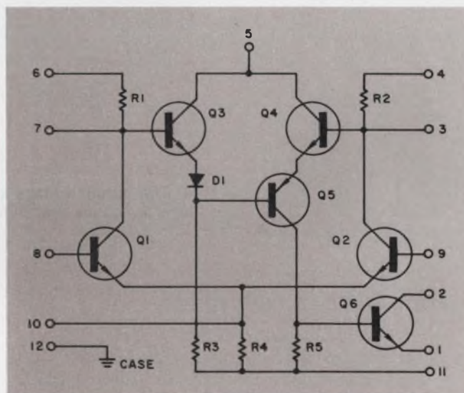
2. This wideband operational amplifier has a slew rate of 100 V per microsecond, which is difficult to obtain with monolithic op amps.
