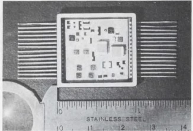
1. Hybrid technology as a packaging technique for monolithic chips is demonstrated by this one-inch-square ceramic flat pack. The circuit contains 10 monolithic chips five diode chips, four capacitors and two high-performance transistor chips.
