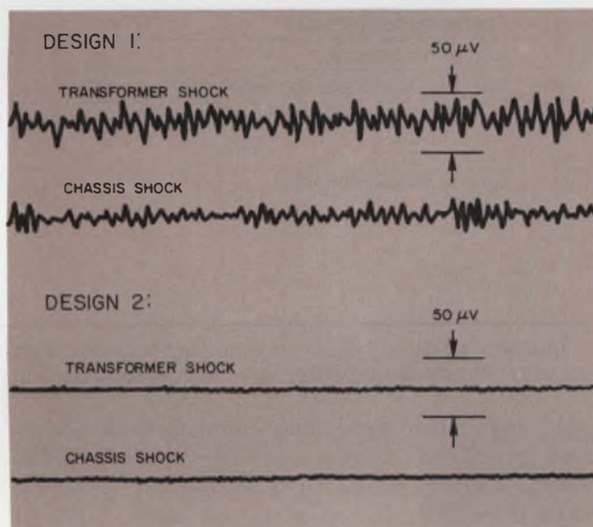
2. Shock and vibration can generate unwanted signals inside the transformer or along the leads. Vibration voltage is a problem under severe environments or when the transformer input voltage is small and easily masked by noise.
