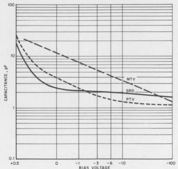
Fig. 3. Capacitance characteristics of three types of microwave diodes.
