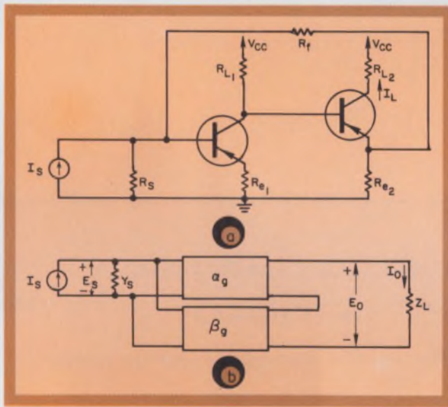
2. Typical series-shunt configuration (a) is best analyzed using h parameters (b) since I_s is common to both the forward and reverse networks and E_o is across both networks.
