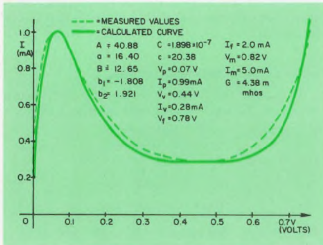
6. Static V-I characteristic for 1N2929 tunnel diode illustrates the closeness to fit that can be obtained by the curve-fitting method.
