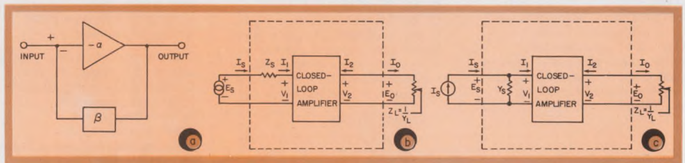
1. The general feedback amplifier (a) may be considered as a two-port network driven from a voltage source (b)
