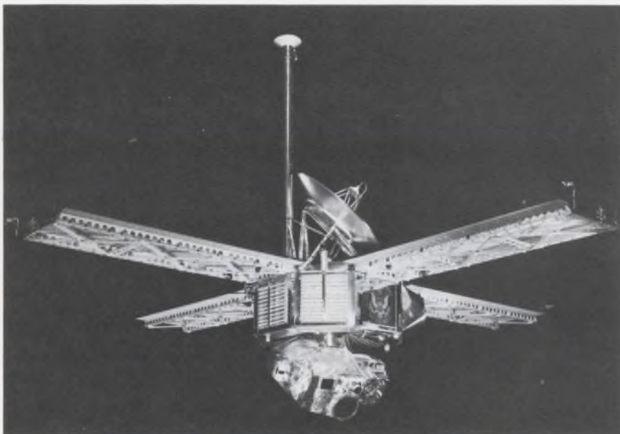
Mariner 6, fully extended , its high-gain antenna on top and its cameras pointed downward at a slant. The spacecraft flew successfully past Mars last July.
