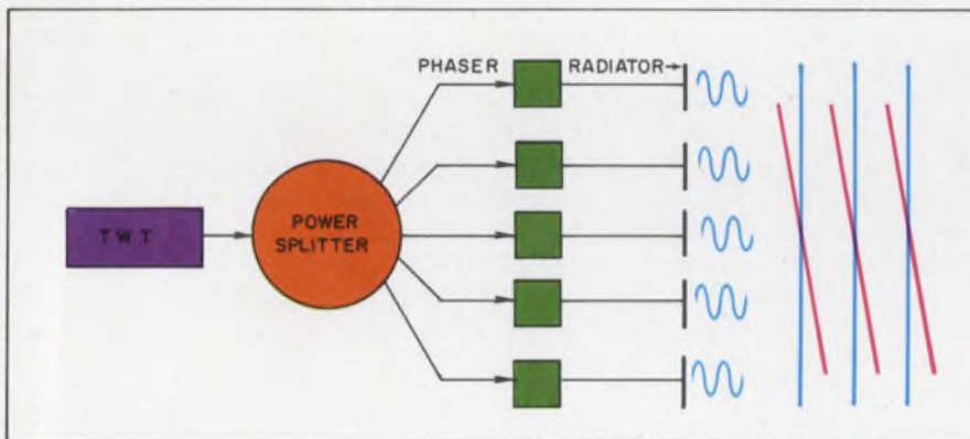
2. A phased-array antenna aims its beam by changing the relative phase of the signal applied to each radiator. When the phases are all the same, the resultant beam moves to the right, as shown by the blue constant-phase lines. By progressive delay of the phase (from top to bottom), the beam can be tilted up, as shown by the red lines.
