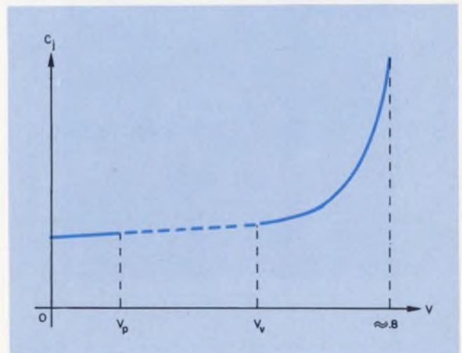
3. Capacitance characteristic of tunnel diode resembles that of an ordinary diode but is difficult to measure within the negative resistance region.
