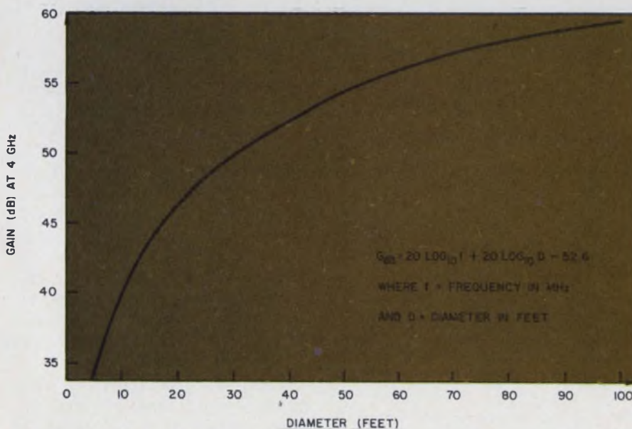
1. The point of diminishing returns is reached when it no longer pays to double the diameter of a parabolic reflector for 6 dB of additional gain. This occurs at about 85 feet for international stations.
