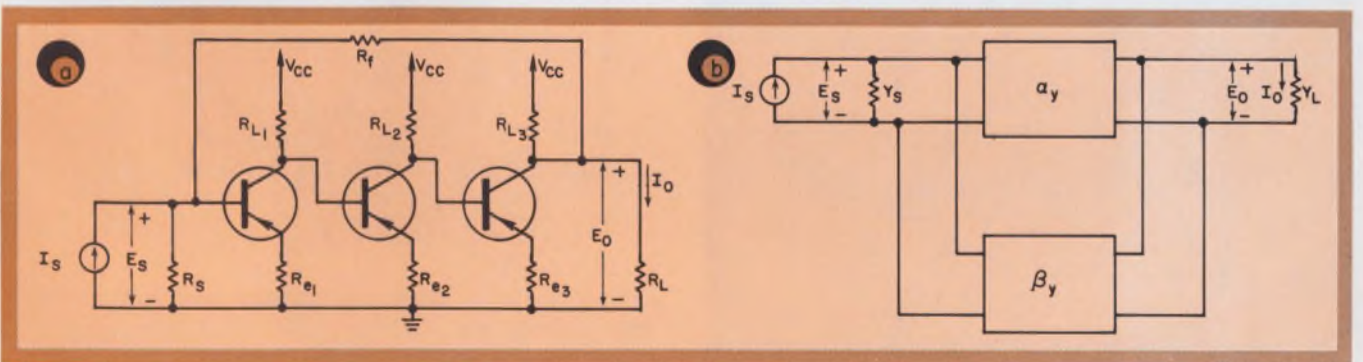
4. Typical shunt-shunt configuration (a) is best analyzed using y parameters (b). This selection of parameters is
