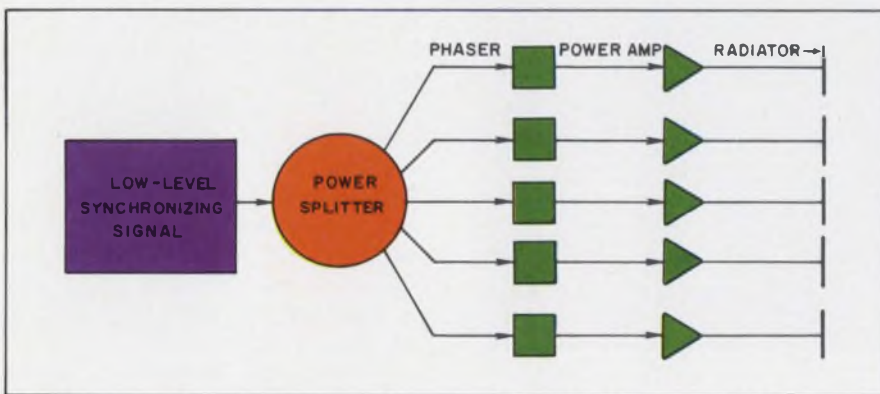
3. Phaser losses can be made unimportant through use of a separate power amplifier for each radiator. The amplifiers can be true amplifiers, or perhaps oscillators that are phase-locked to the input signal. In any event, this approach won't be practical until very lightweight reliable solid-state amplifiers are made available.
