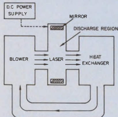
Desk-sized CO 2 laser contains a closed-cycle gas cooling system.
