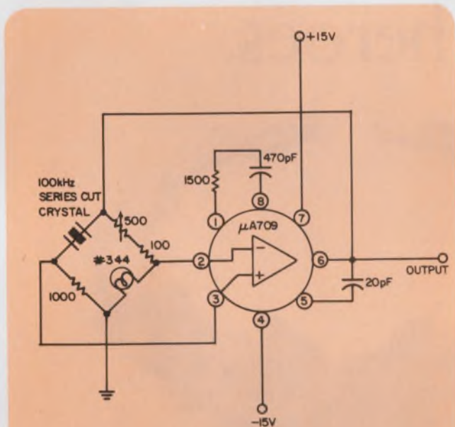
1. No transformer is used in this Meacham Bridge. An IC op amp is combined with a light bulb to keep the crystal drive level fixed.
