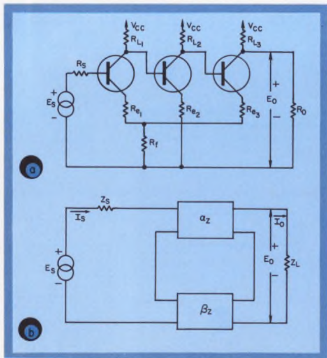
5. Typical series-series configuration (a) is best analyzed using z parameters (b) since I_s and I_o both flow through the forward and reverse networks.
