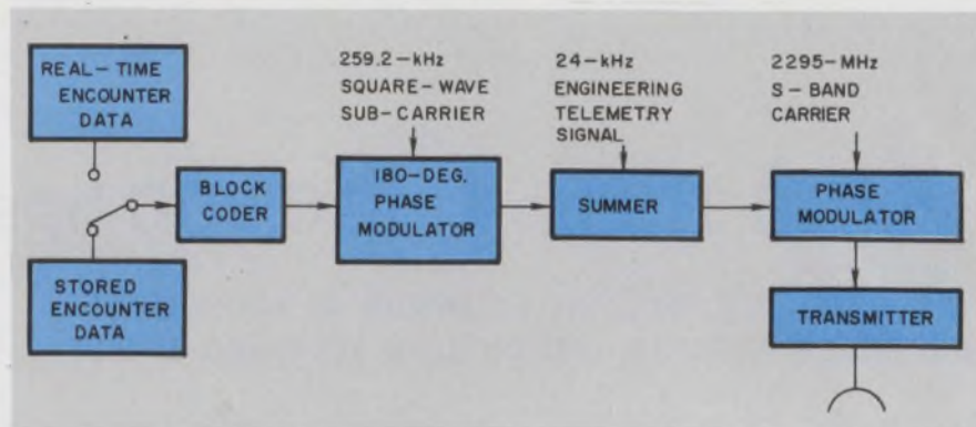
Block diagram of the 16,200-bit-per-second Mariner data-transmission system.
