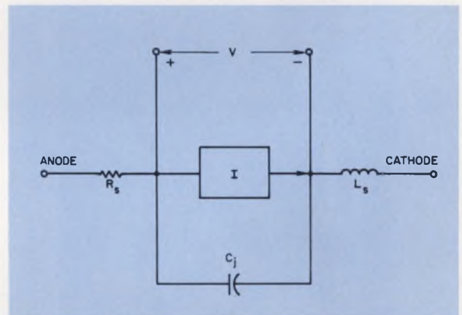
2. Topology of tunnel diode depicts the lumped parameters that must be evaluated.
