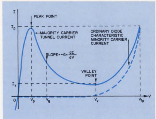
1. Static V-I characteristic of typical tunnel diode defines the curve that must be matched mathematically.
