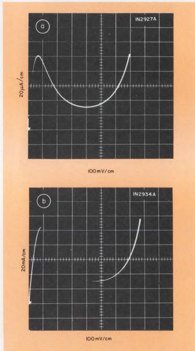
4. Oscilloscope traces of tunnel-diode characteristics facilitate measurement of peak, and valley points. The loss of detail in the negative resistance region of the IN2934A makes measurement of V_g difficult.
