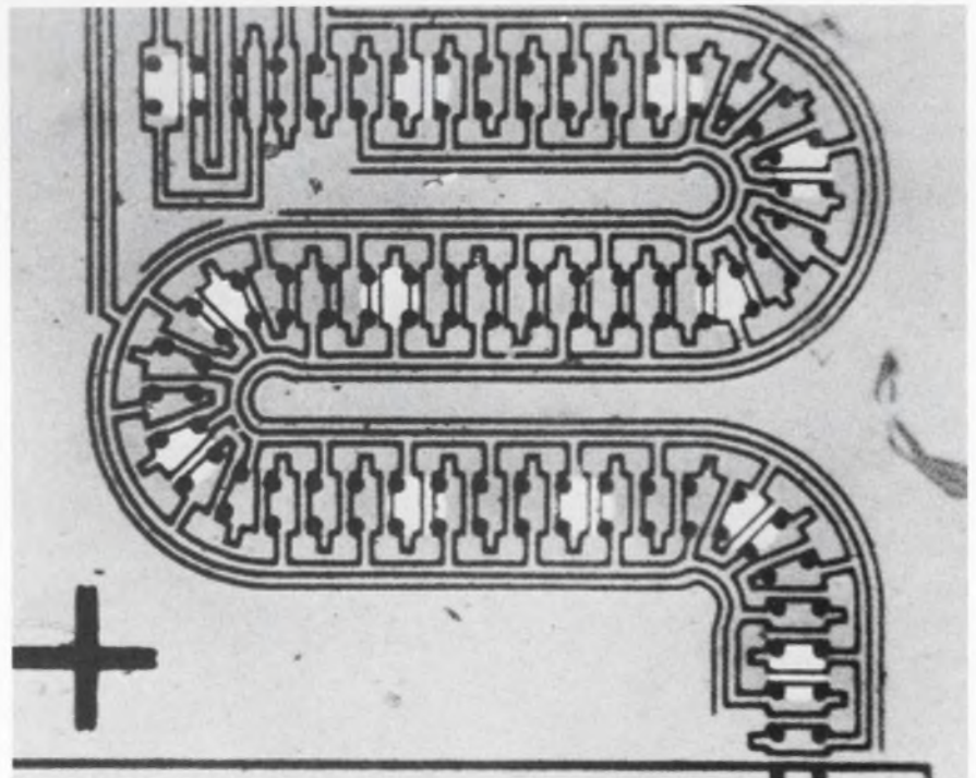
Travelling bubbles (the white dots) can move through conductor circuits at data rates of three megahertz.
