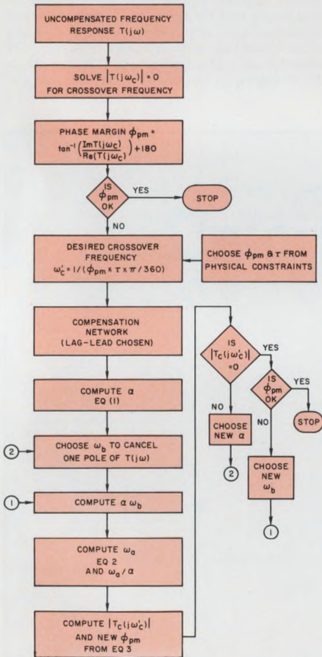
7. Flow chart shows steps in designer/computer interaction during programming.
