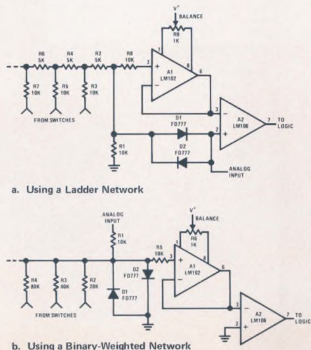
FIGURE 1. Comparator Circuits for Fast A/D Converters
