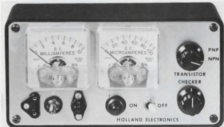
Battery-operated transistor tester can check unknown transistors for shorts, opens and gain, p. 115.
