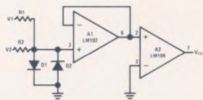
a. Comparator for Signals of Opposite Polarity
