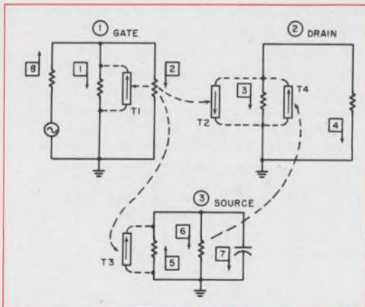
6. All capacitive elements except C_s are excluded in this ac model.
