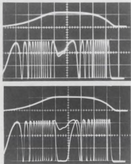
Oscilloscope records compare voltage-divider and laser measurements of same pulses. At top, pulses of 142.30 kV and 142.35 kV are superimposed on both divider and laser traces, while at bottom voltages are 142.30 kV and 142.80 kV.
