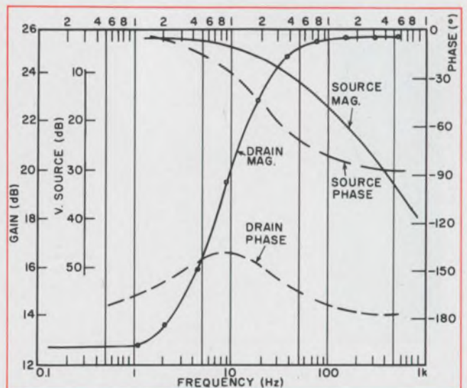
7. Curves show the analysis results of the ac model depicted in Fig. 6.
