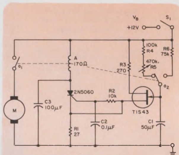
The OFF time of the motor being controlled can be varied between 5 and 35 seconds by potentiometer R_5 . The motor ON time is constant at 5 seconds.
