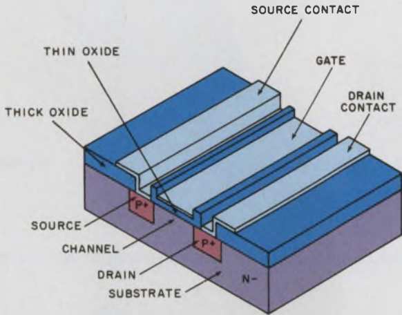
A. The MOS transistor: a simple configuration of source, drain and gate electrodes.
