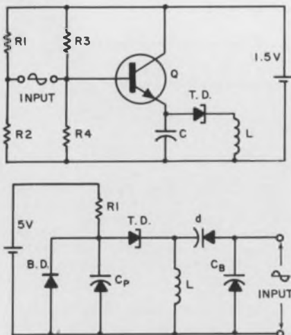
4. Two single-channel biotelemetry transmitters developed by Case Institute of Technology are an advance over previous all-transistor models. The circuits use tunnel, backward and varicap diodes. The lower circuit has the same sensitivity as the upper, but it has greater temperature stability and a higher input impedance of 100 megohms.
