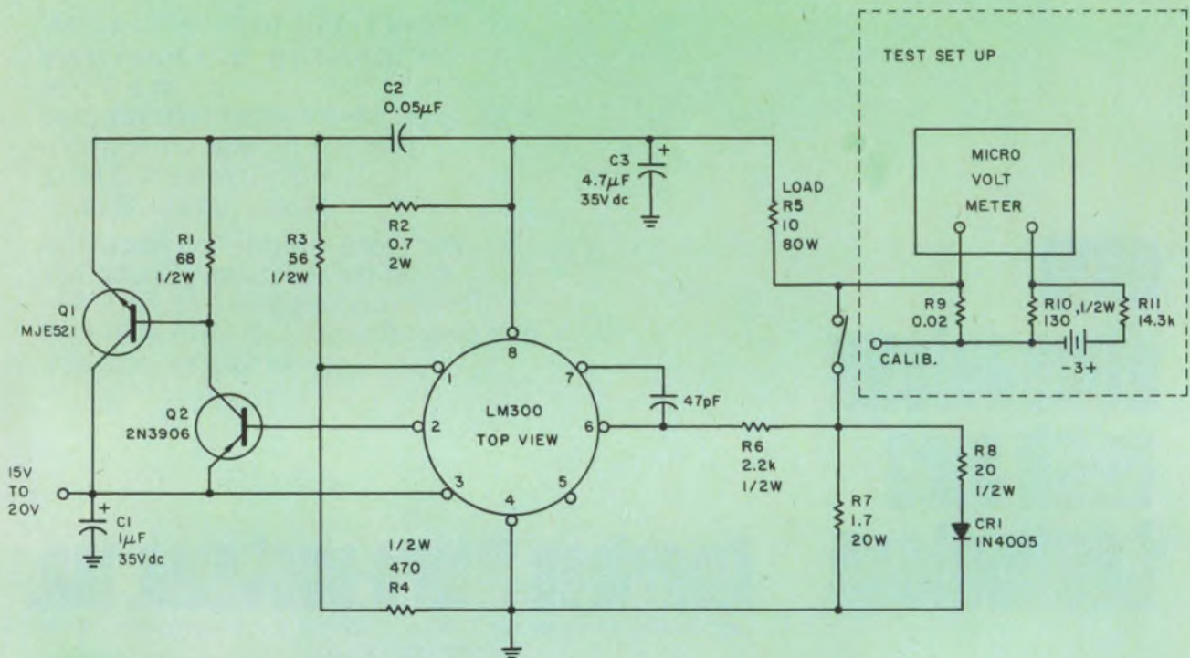
Constant current of 1 A is maintained through the load, despite changes in load resistance or supply voltage.
