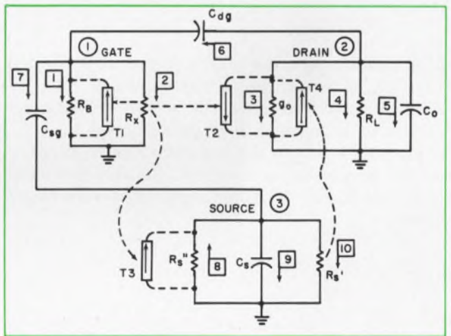
4. General FET model for ac requires two additional current sources, T_3 and T_4 .
