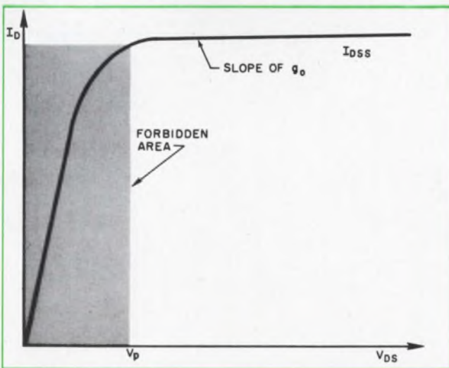
2. Plot shows good linear performance of the FET model. The shaded area indicates the portion of the model's range that is not suitable for linear representation.
