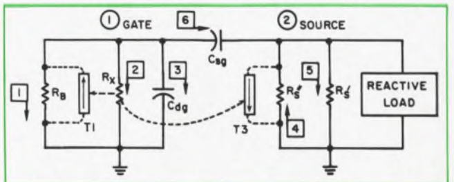
5. Reduce current sources by using this source follower version of the model. Only two current sources are required here, rather than four as in other versions.
