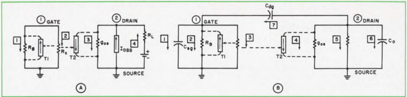
1. Dependent current sources are key elements in this linear FET model for use with ECAP. The basic dc model
