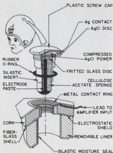
2. "Sponge" helmet electrodes developed by NASA at its Ames Research Center for brain-wave measuring telemetry system.
