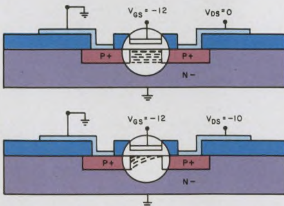
C. The saturation phenomenon: drain-to-source voltage effects are limited by channel pinch-off.
