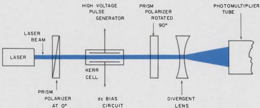
Laser and Kerr-cell pulse-voltage measuring system sends the laser beam through the first polarizer and then the Kerr cell, in which beam polarization is rotated by rising (or falling) voltage across the cell. As the beam rotates, the second polarizer output is a sequence of bright maxima and dark minima, occurring each 90 degrees. For each pulse, the photomultiplier output gives sine-traces such as shown at left, on the oscilloscope screen. The system was developed by National Bureau of Standards and Sandia Corp.
