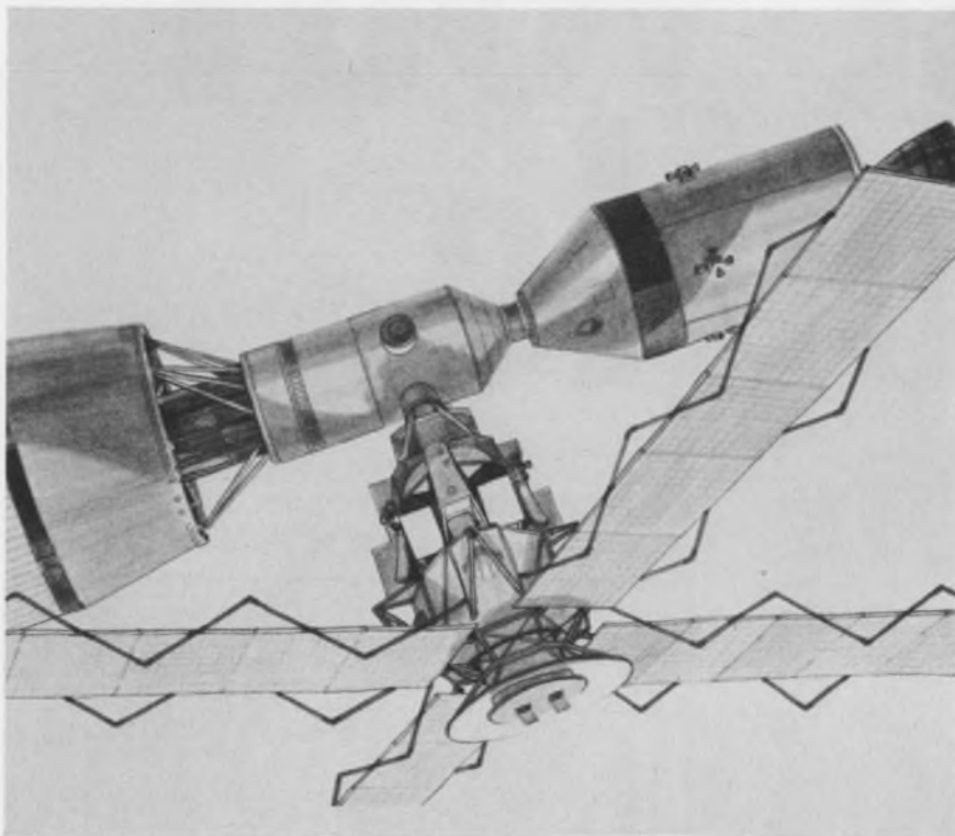
Telescope for earth-orbit or lunar station. Attached are solar astronomy experiment equipment, solar arrays, and control moment gyroscopes. Telescope will gather data on physical characteristics of the sun.
