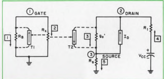
3. Resistor stabilizes the operating point. Selection of the proper value for stabilizing resistor R_s can be done graphically or with a curve tracer.
