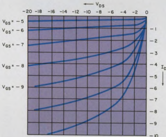
B. The dc characteristic: channel conductance is determined by the gate-to-source voltage.
